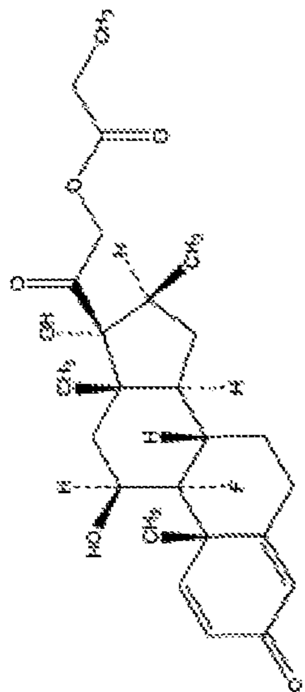
Impurity B (Betamethasone 21-propionate)
