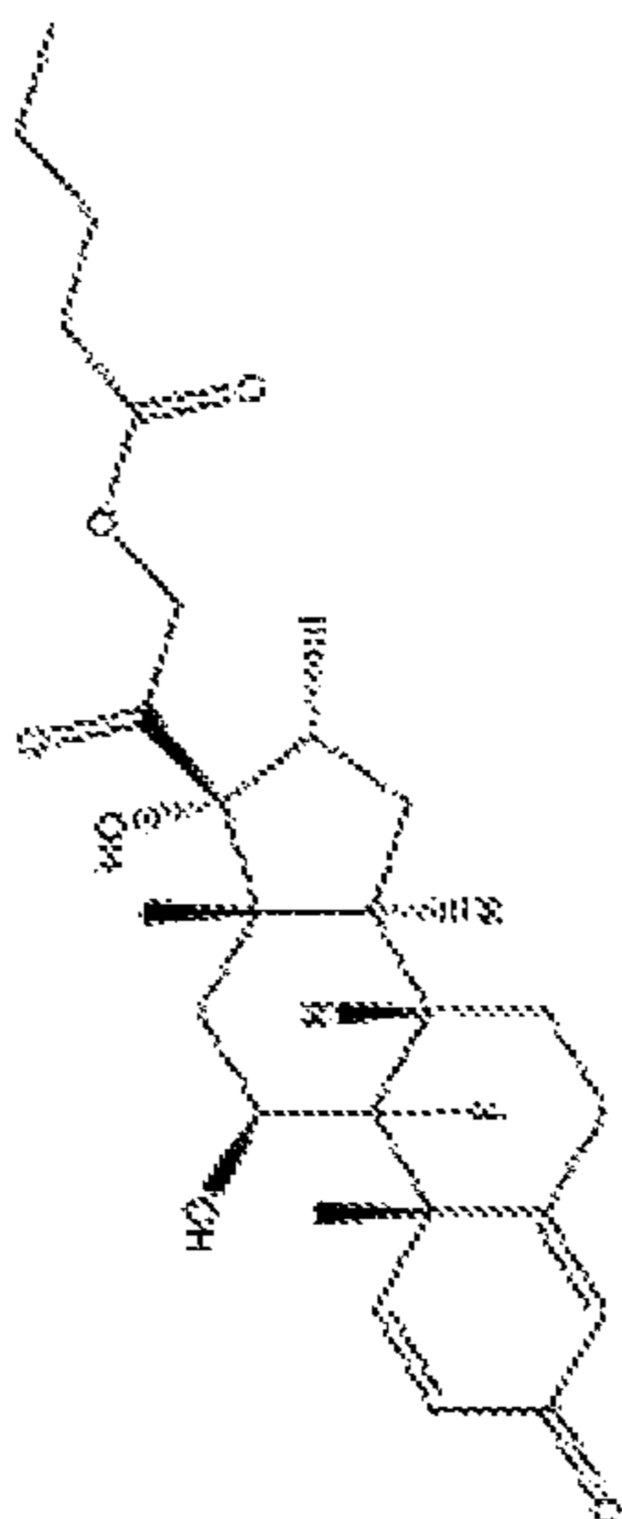
Impurity D (Betamethasone 21-valerate)
