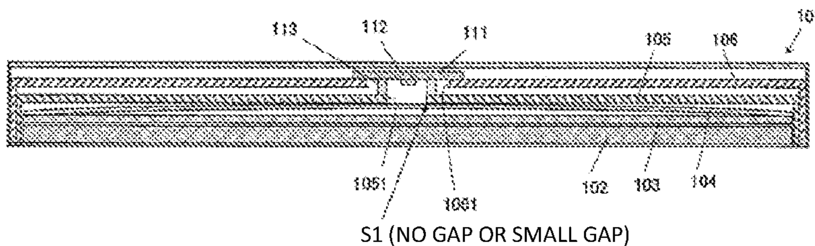
Fig. 22 PRIOR ART
