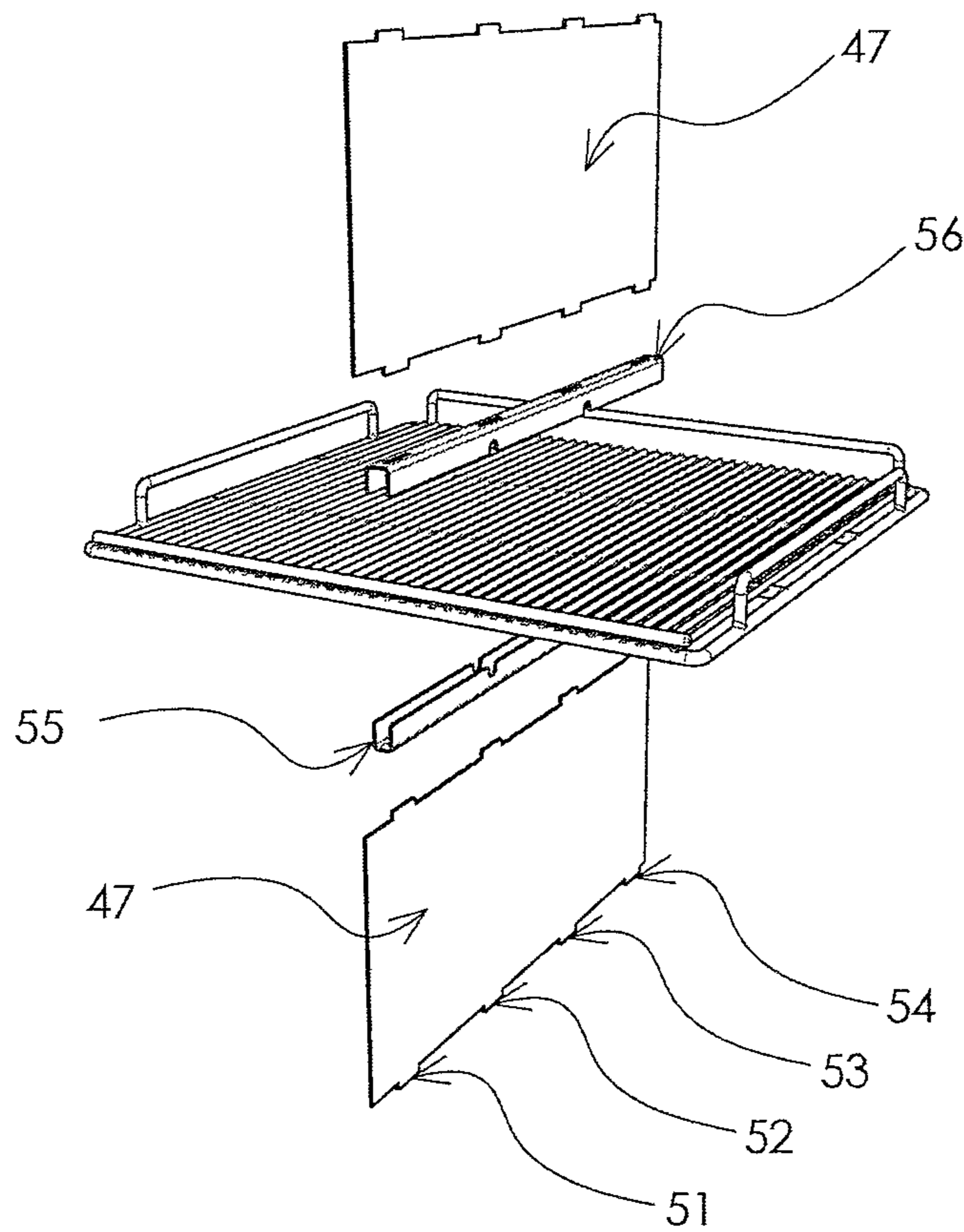
EXPLODED VIEW
