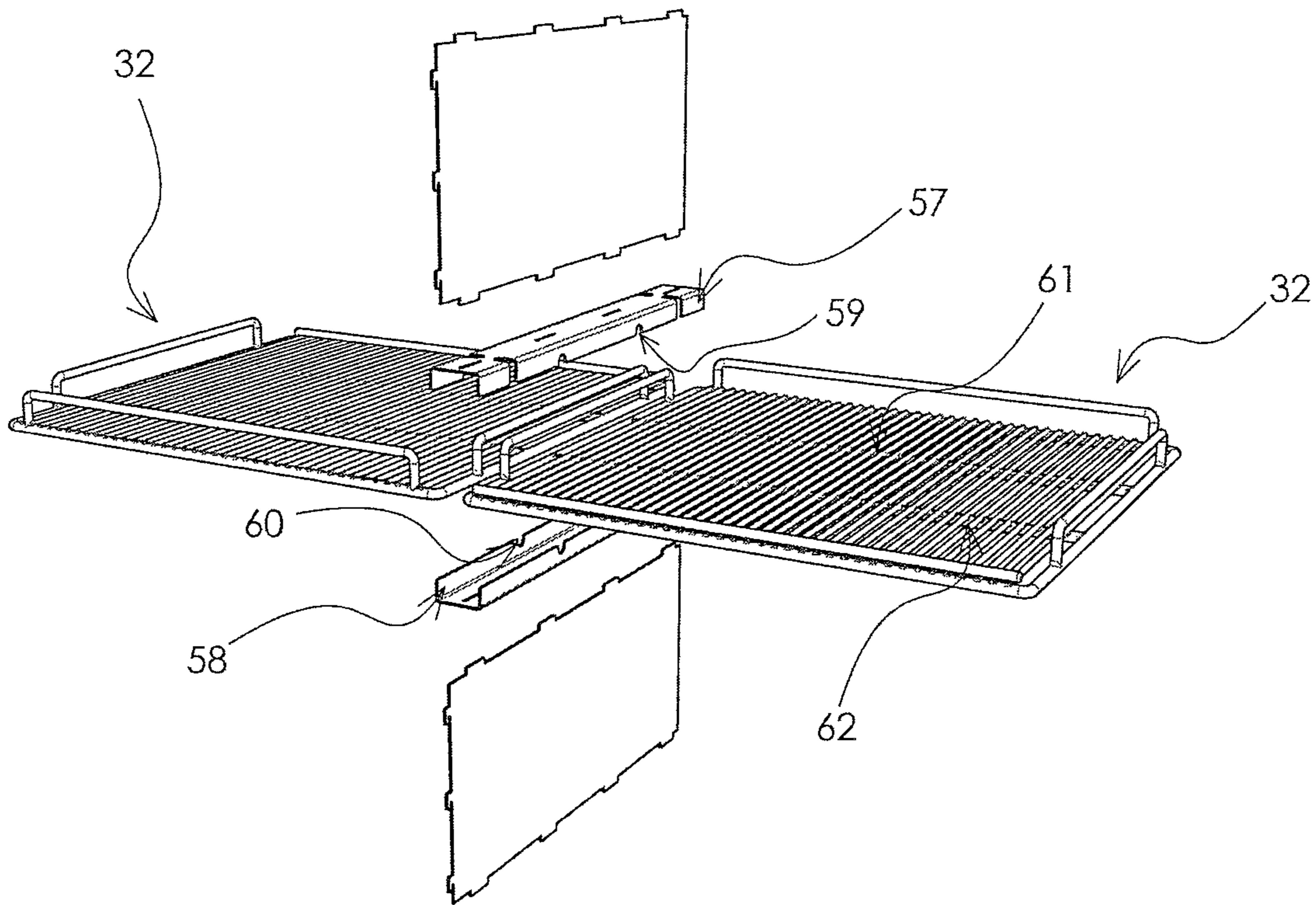
EXPLODED VIEW
