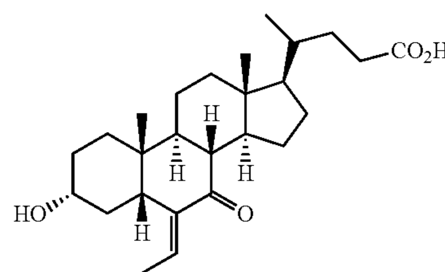
3 \alpha -hydroxy-6-ethylidene-7-keto-5 \beta -cholan-24-oic acid 5
