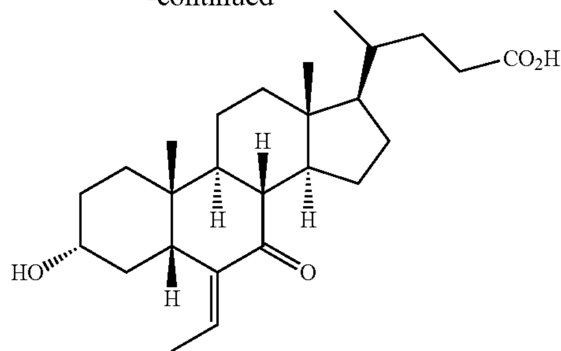
3 \alpha -hydroxy-6-ethylidene-7-keto-5 \beta -cholan-24-oic acid 5
