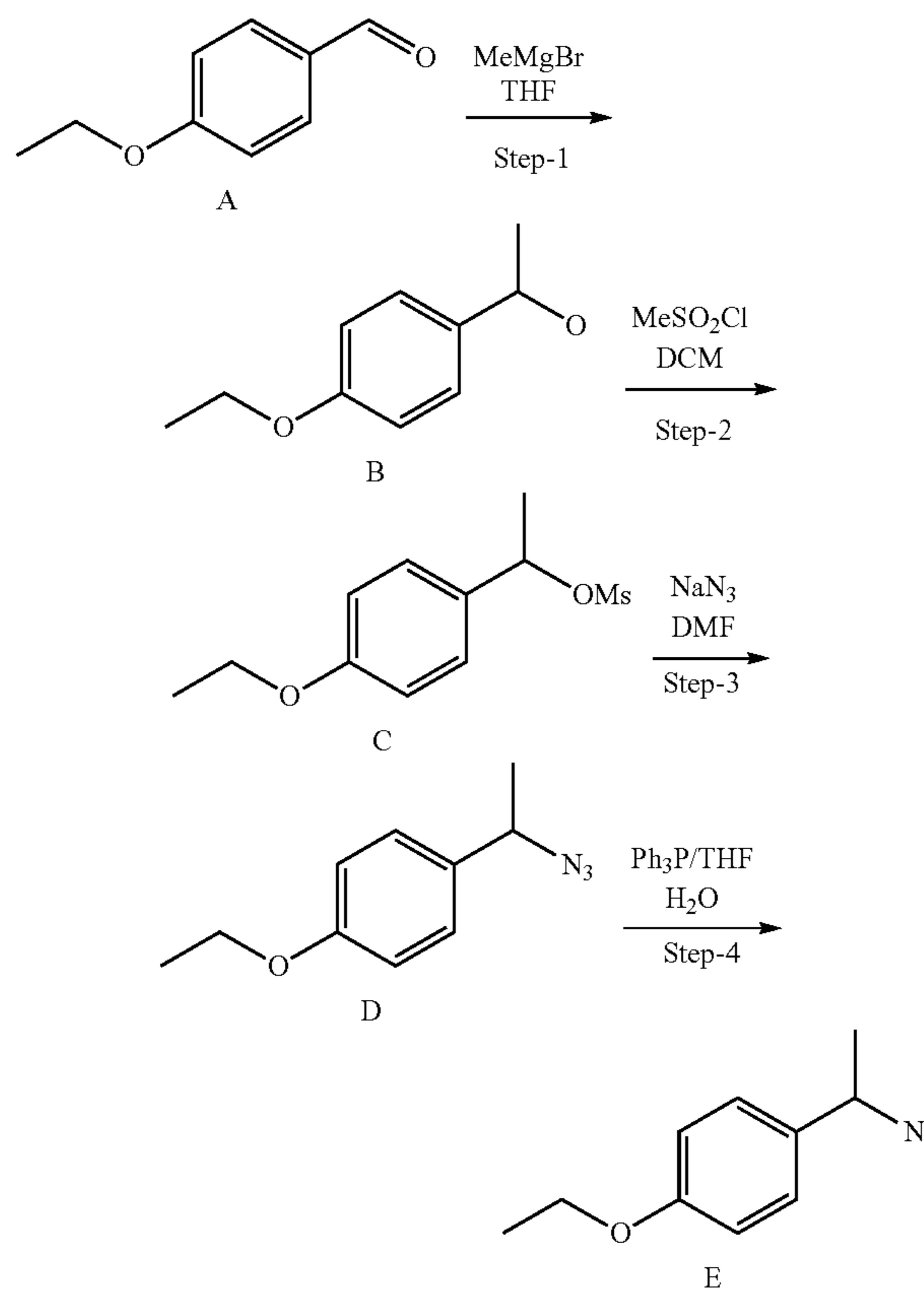
SCHEME-11: Synthesis of 1-(4-Ethoxy-phenyl)-ethylamine
