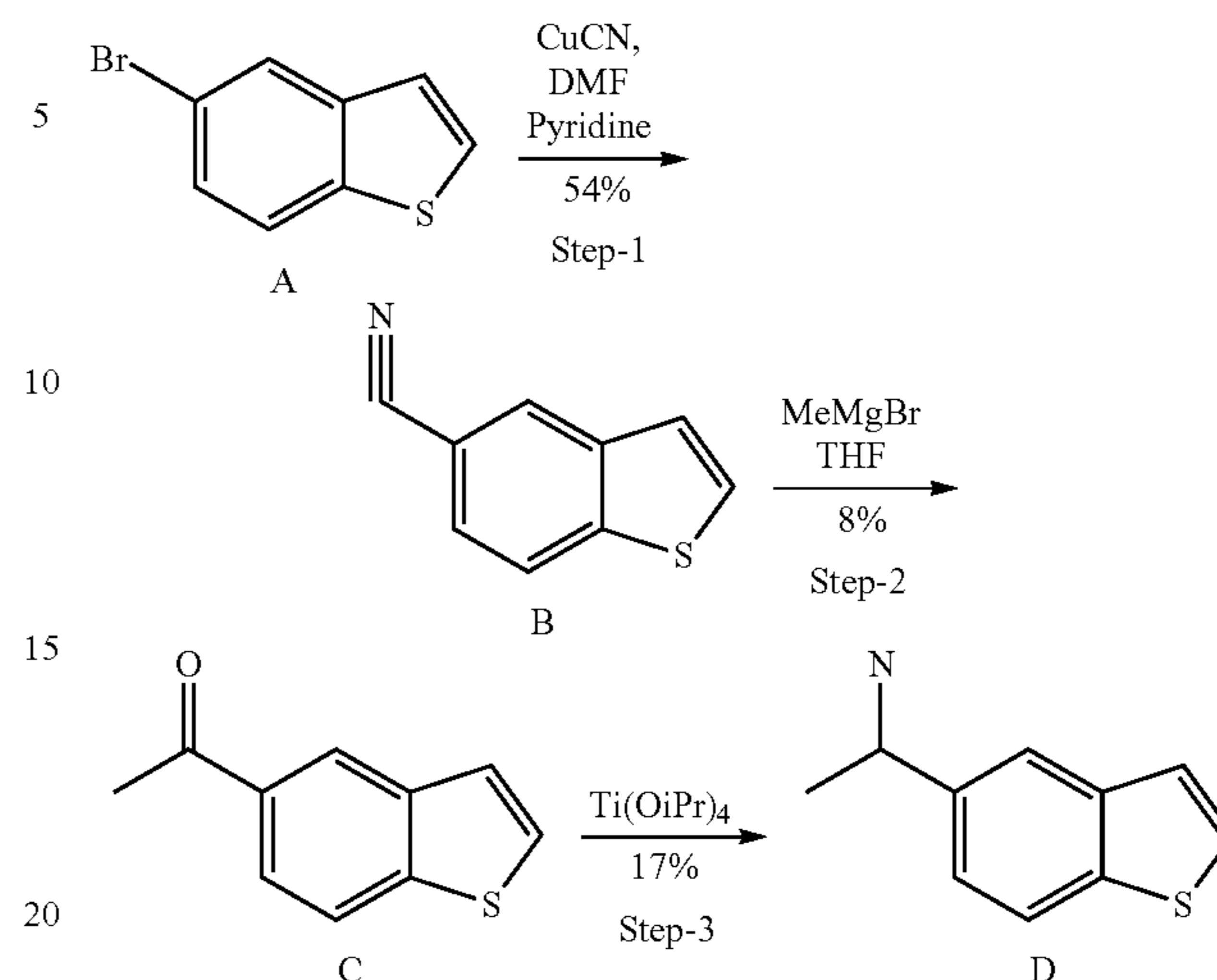
SCHEME-10: Synthesis of 1-Benzo[b]thiophen-5-yl-ethylamine
