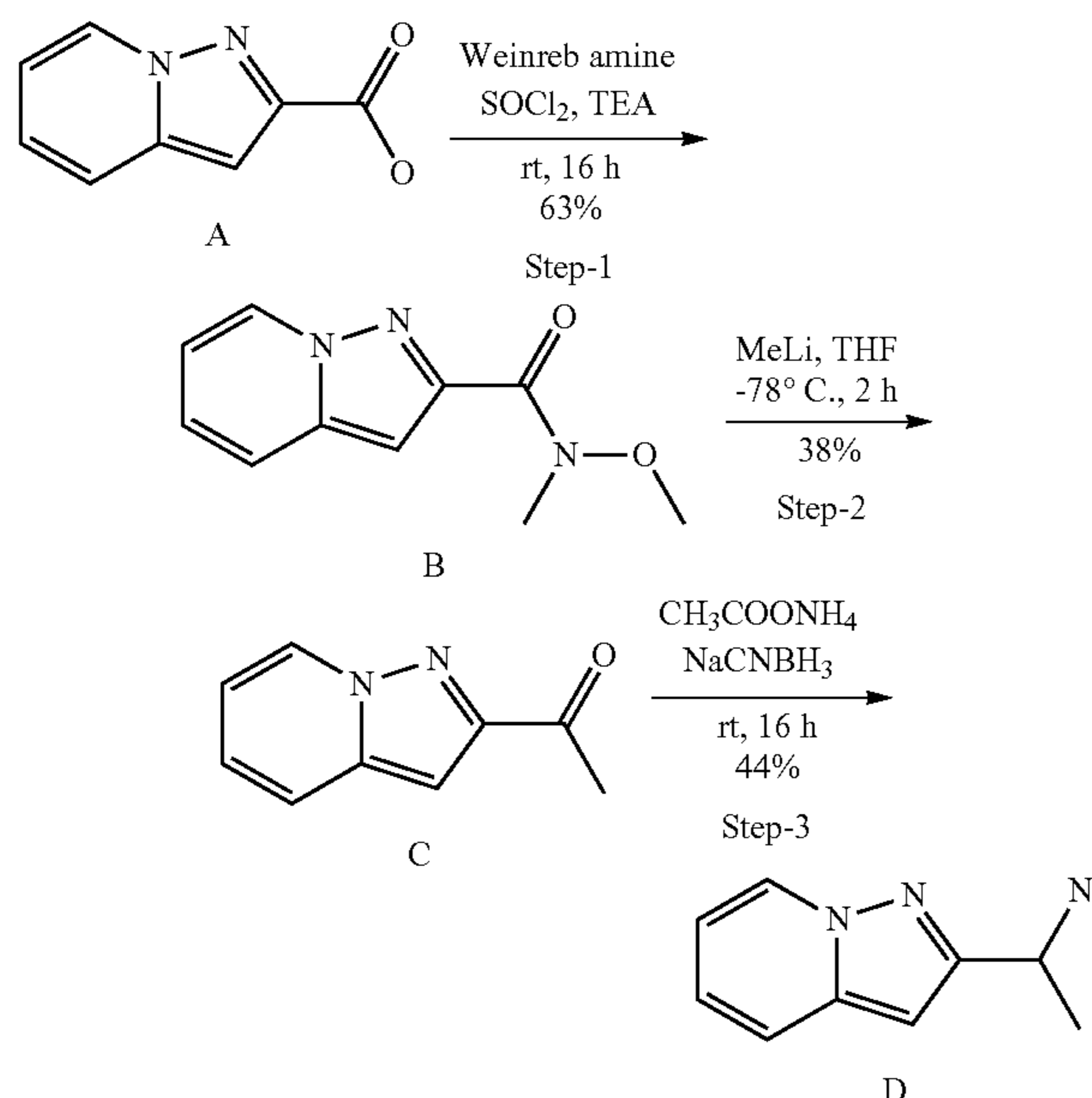
SCHEME-15: Synthesis of 1-Pyrazolo[1,5-a]pyridin-2-yl-ethylamine
