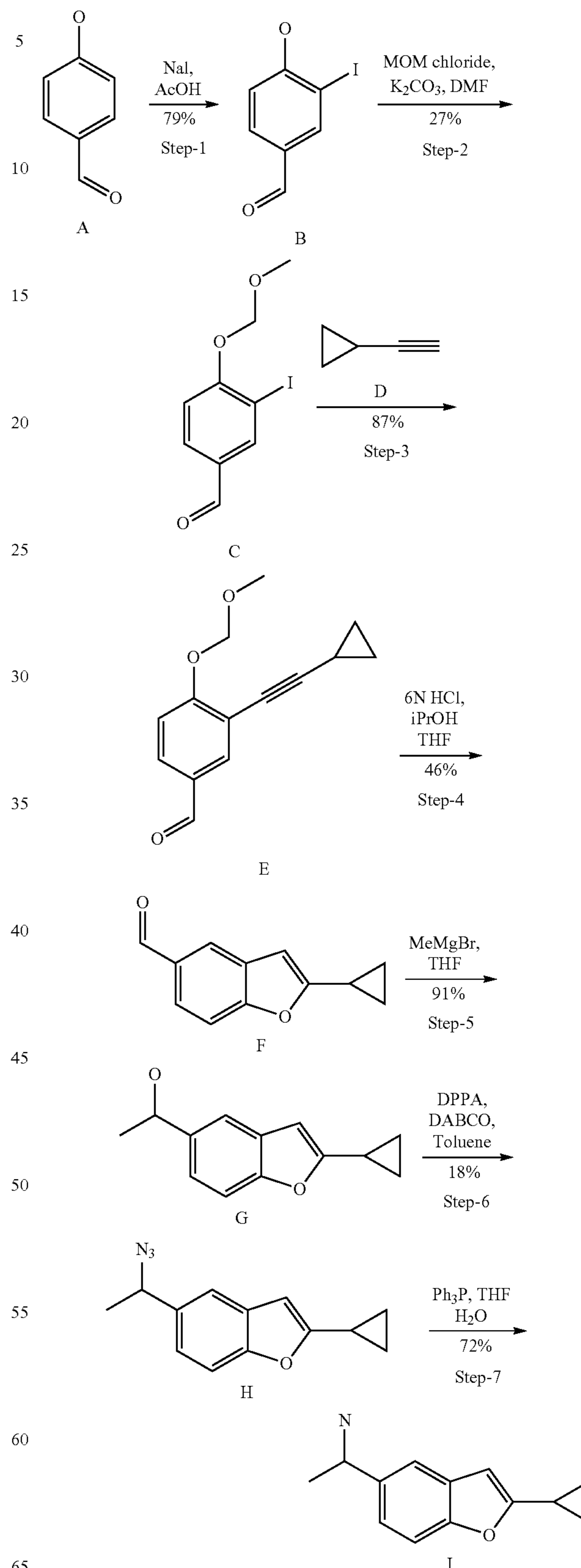
SCHEME-4: Synthesis of 1-(2-Cyclopropyl-benzofuran-5-yl)-ethanamine
