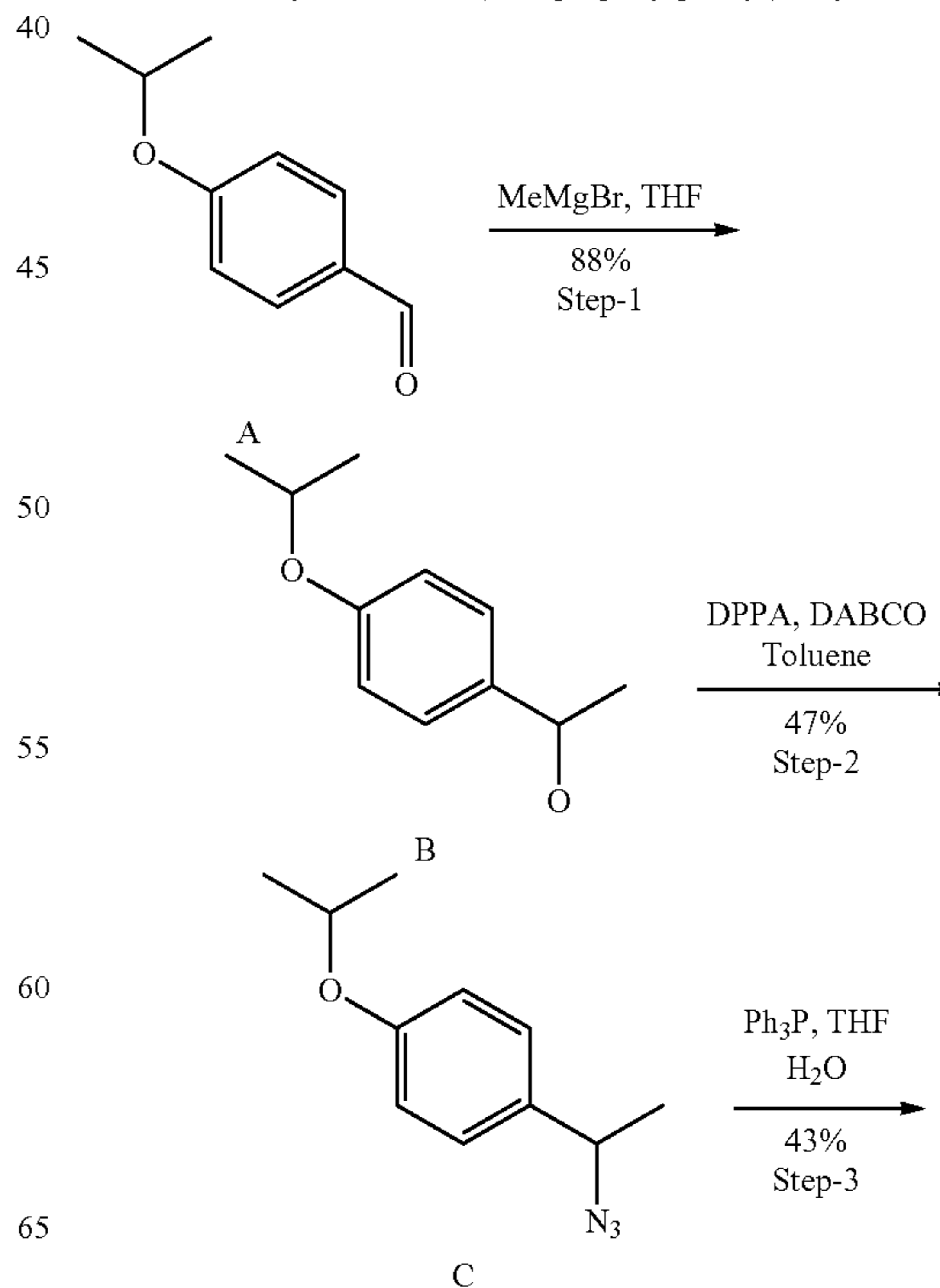
SCHEME-3: Synthesis of 1-(4-Isopropoxy-phenyl)-ethylamine
