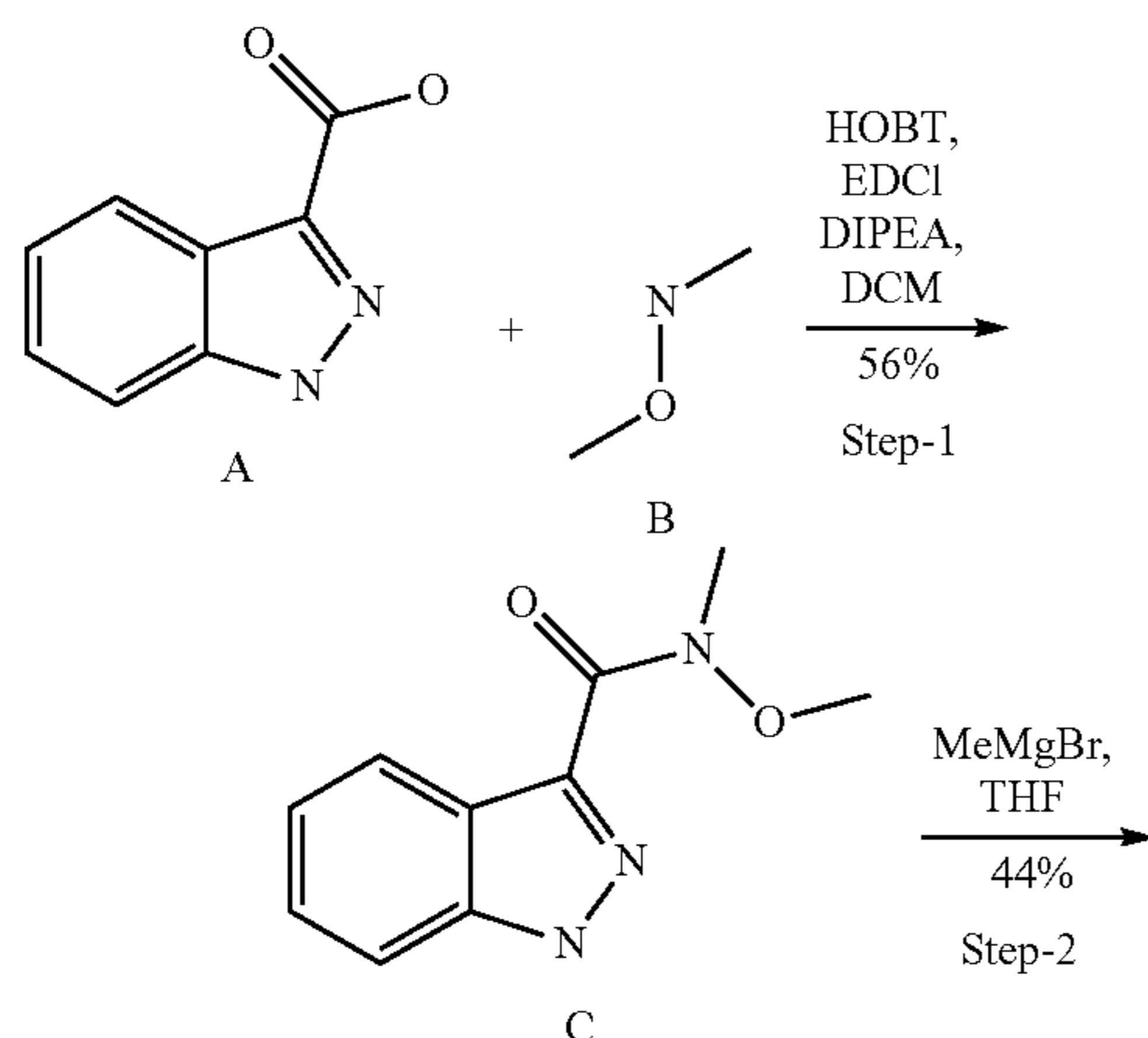
SCHEME-6: Synthesis of 1-(1H-Indazol-3-yl)-ethylamine
