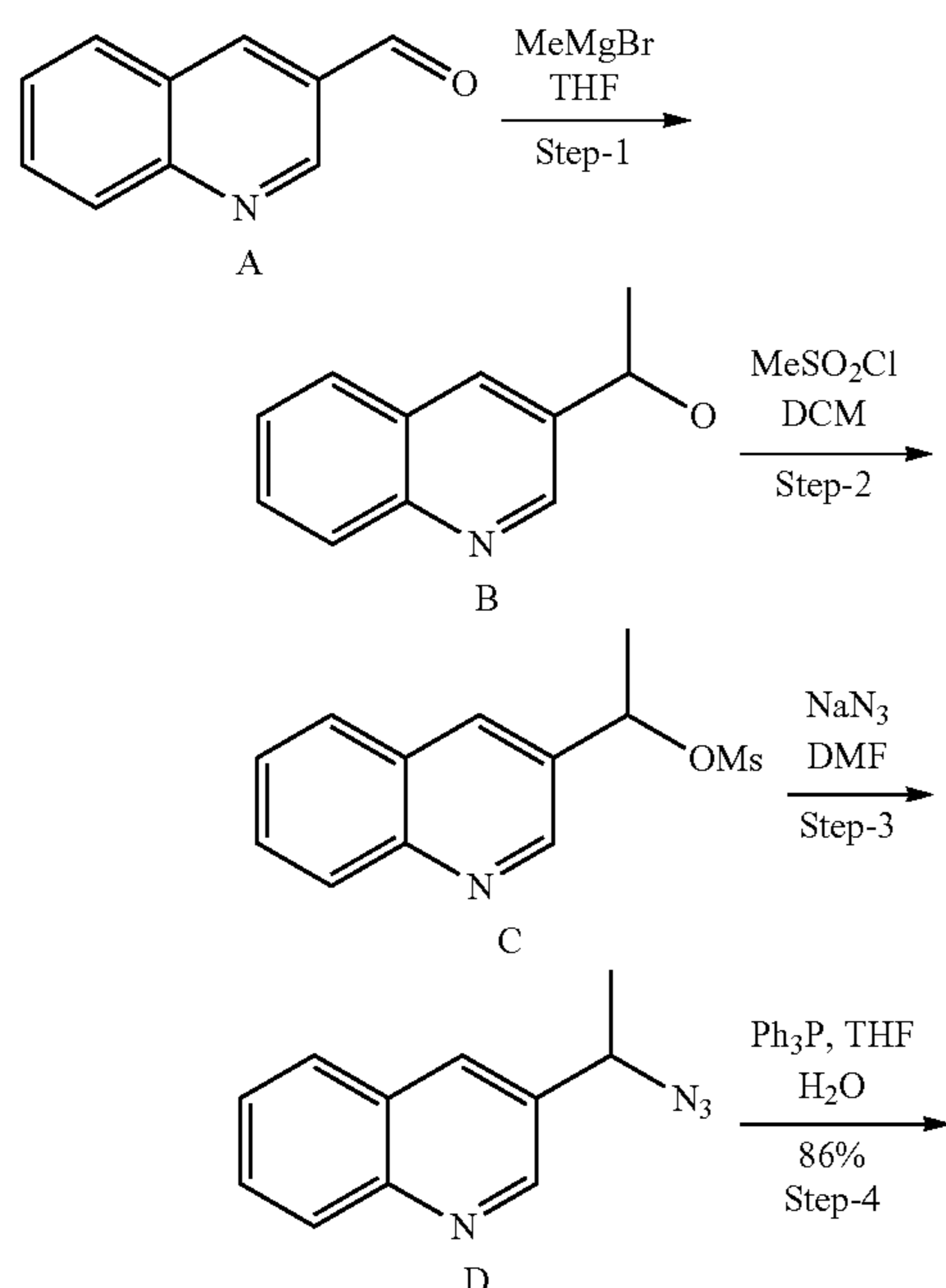
SCHEME 17: Synthesis of 1-Quinolin-3-yl-ethylamine
