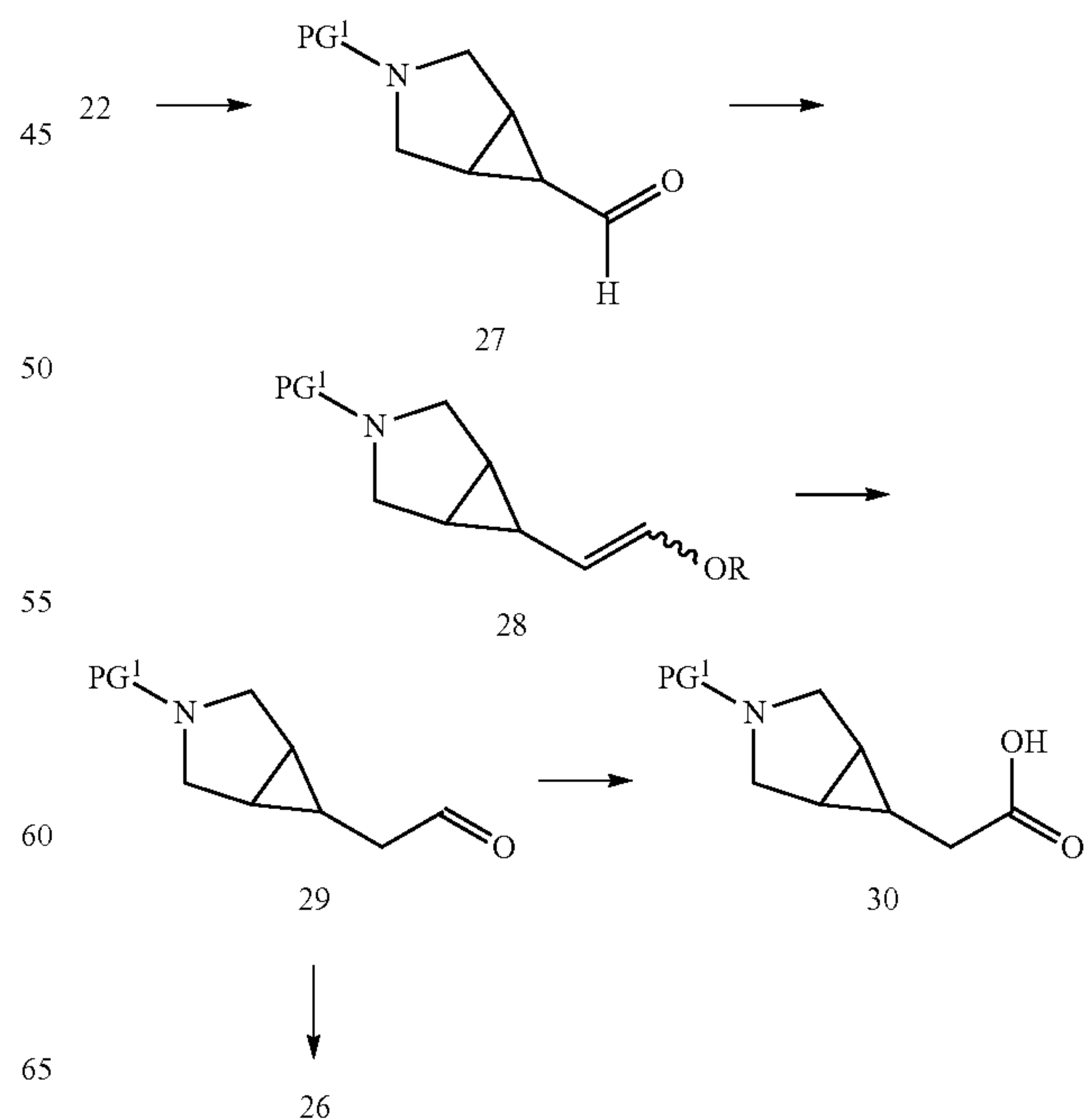
Scheme 3B
