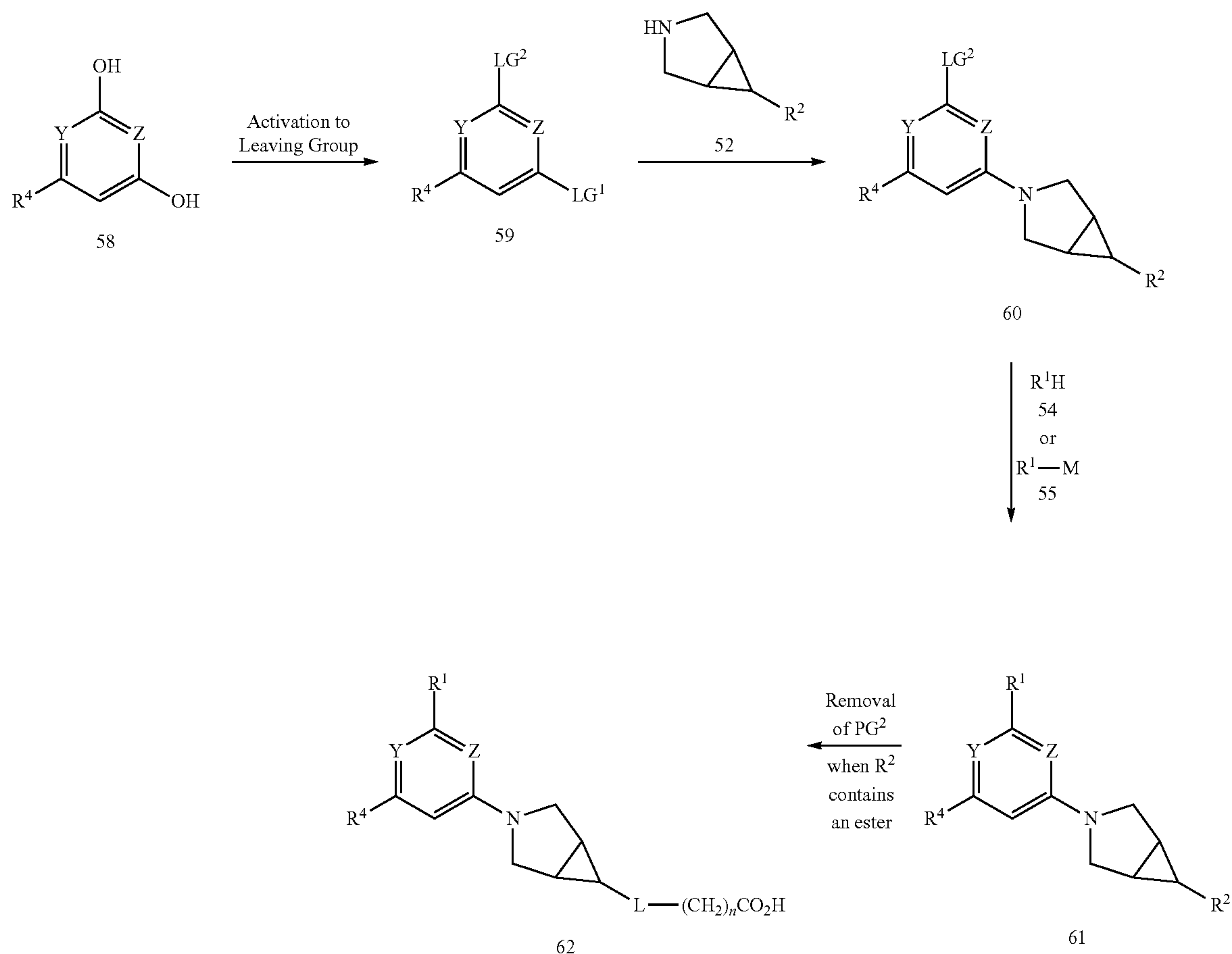
Scheme 6A
