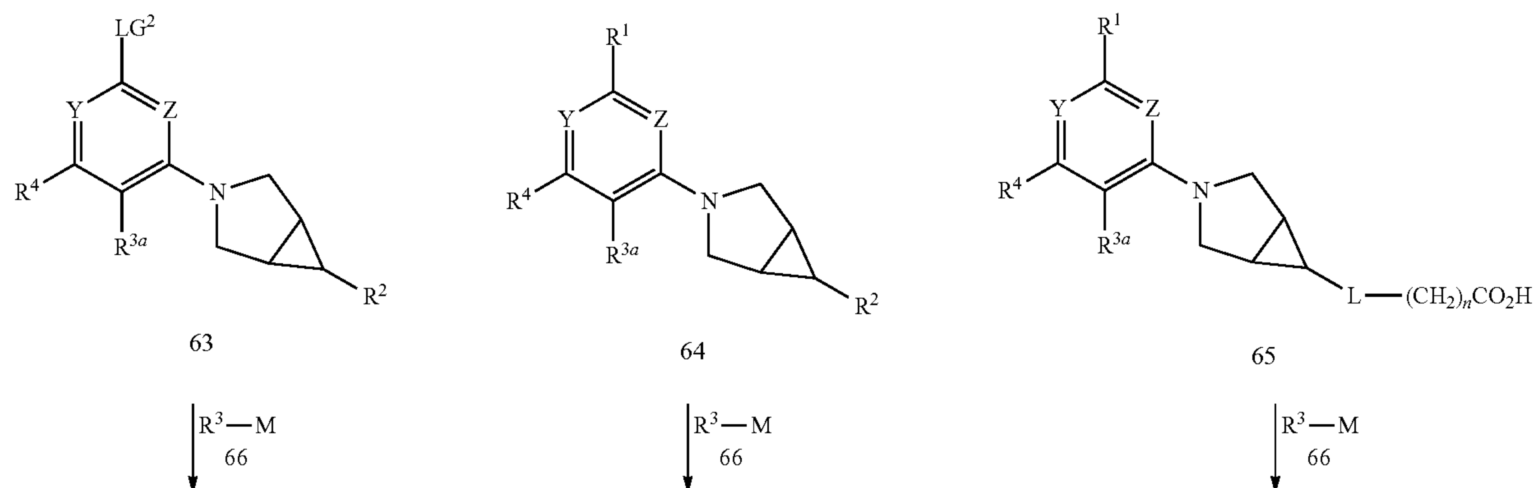
Scheme 6C
