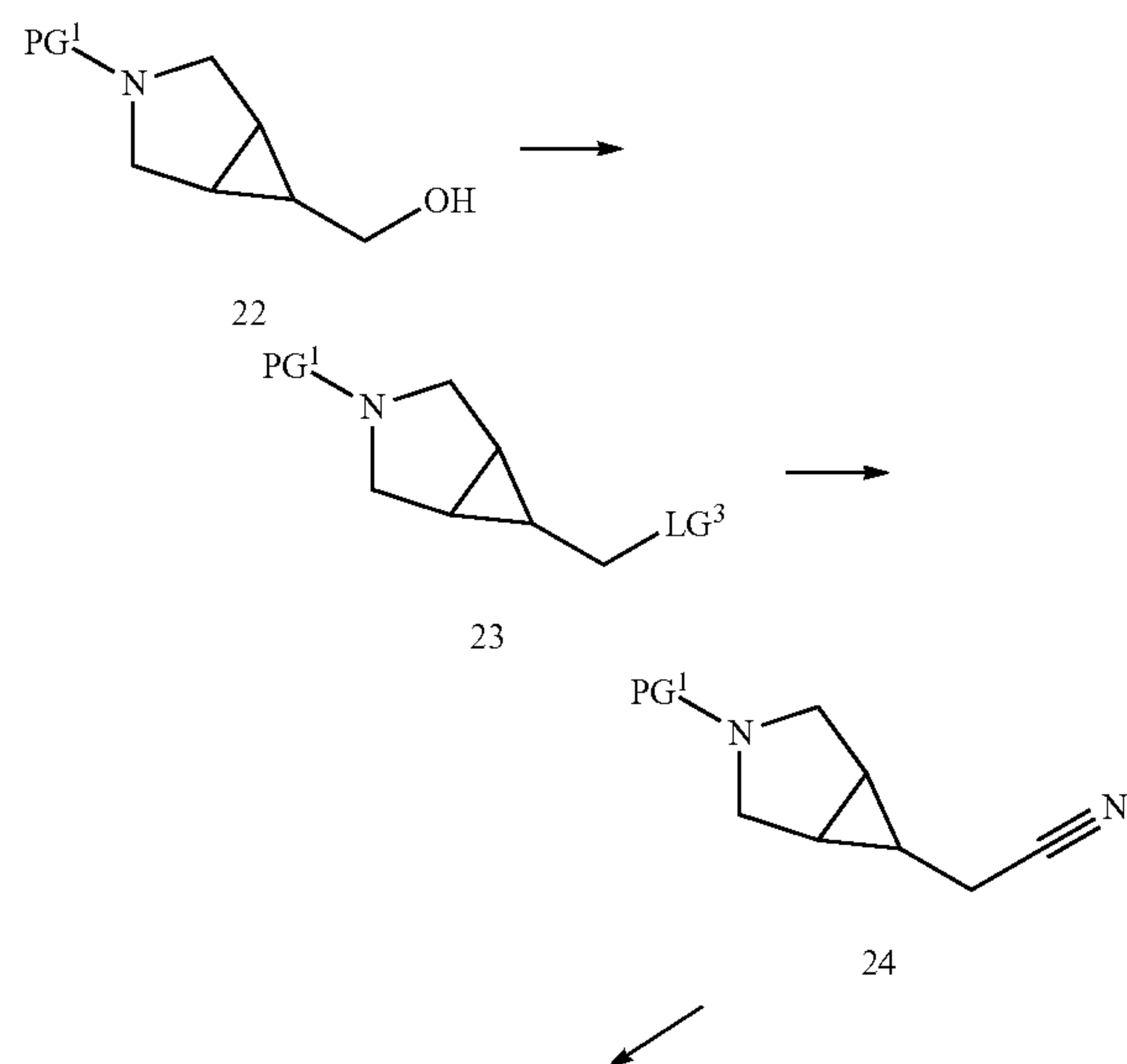
Scheme 3A
