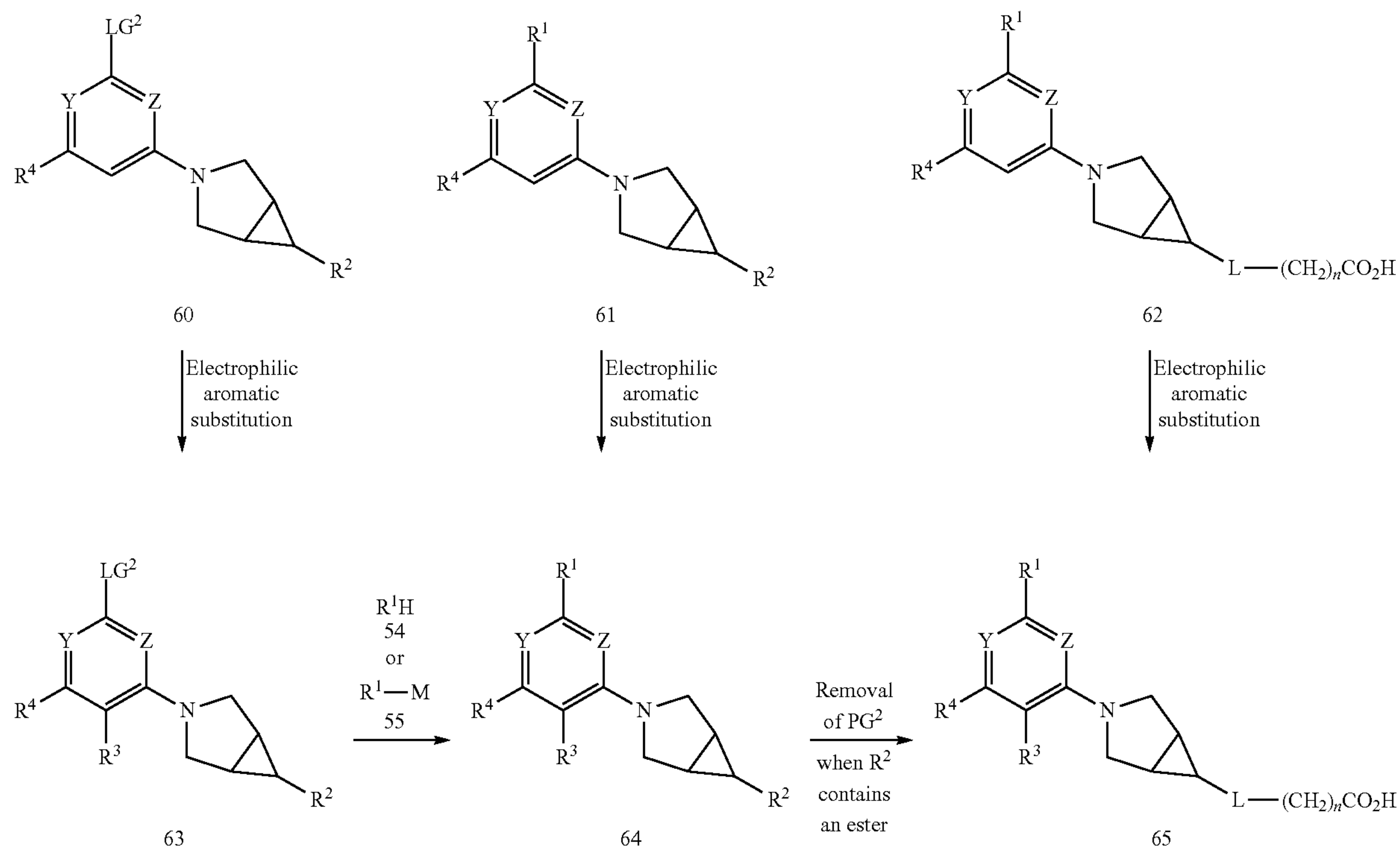
Scheme 6B
