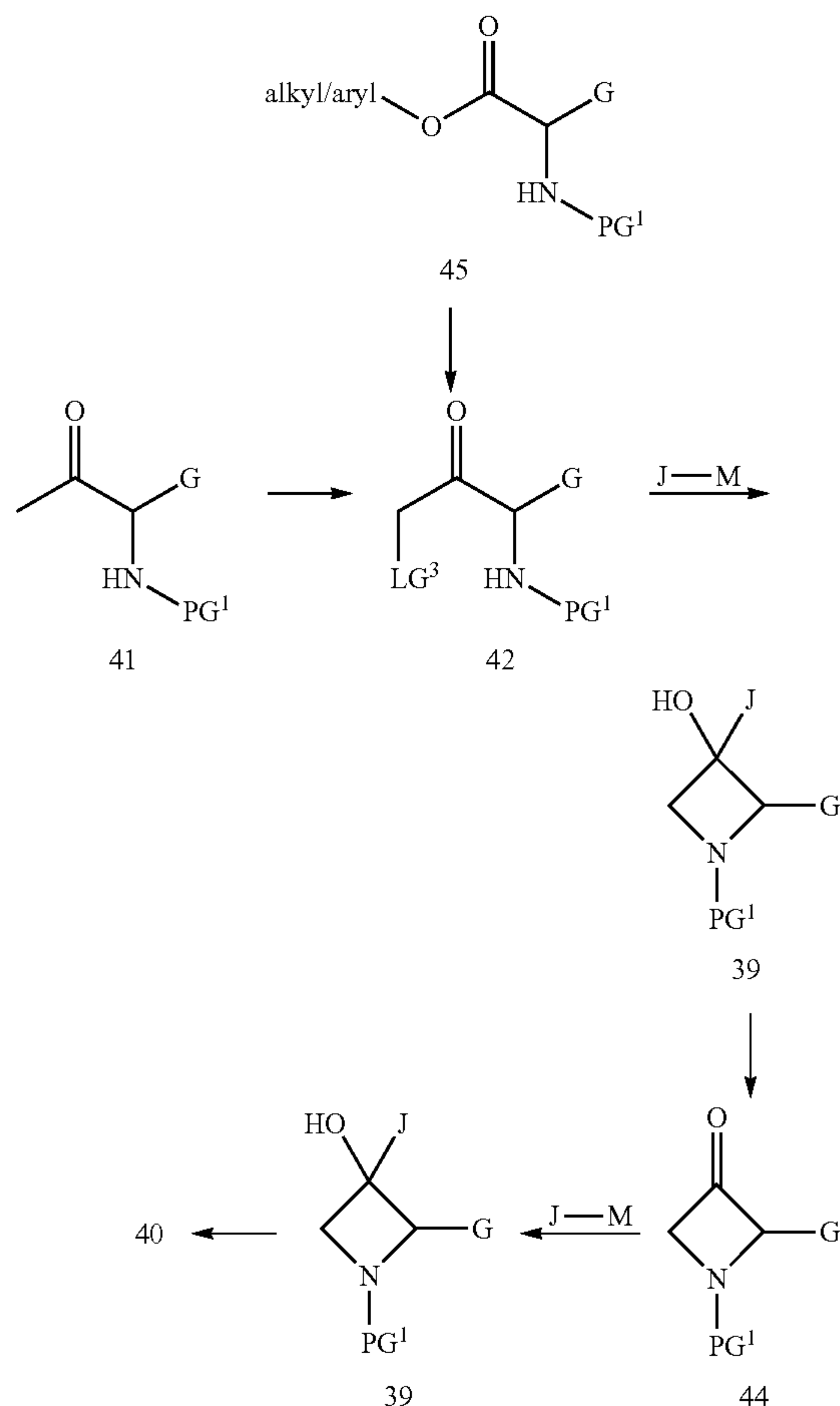
Scheme 4B
