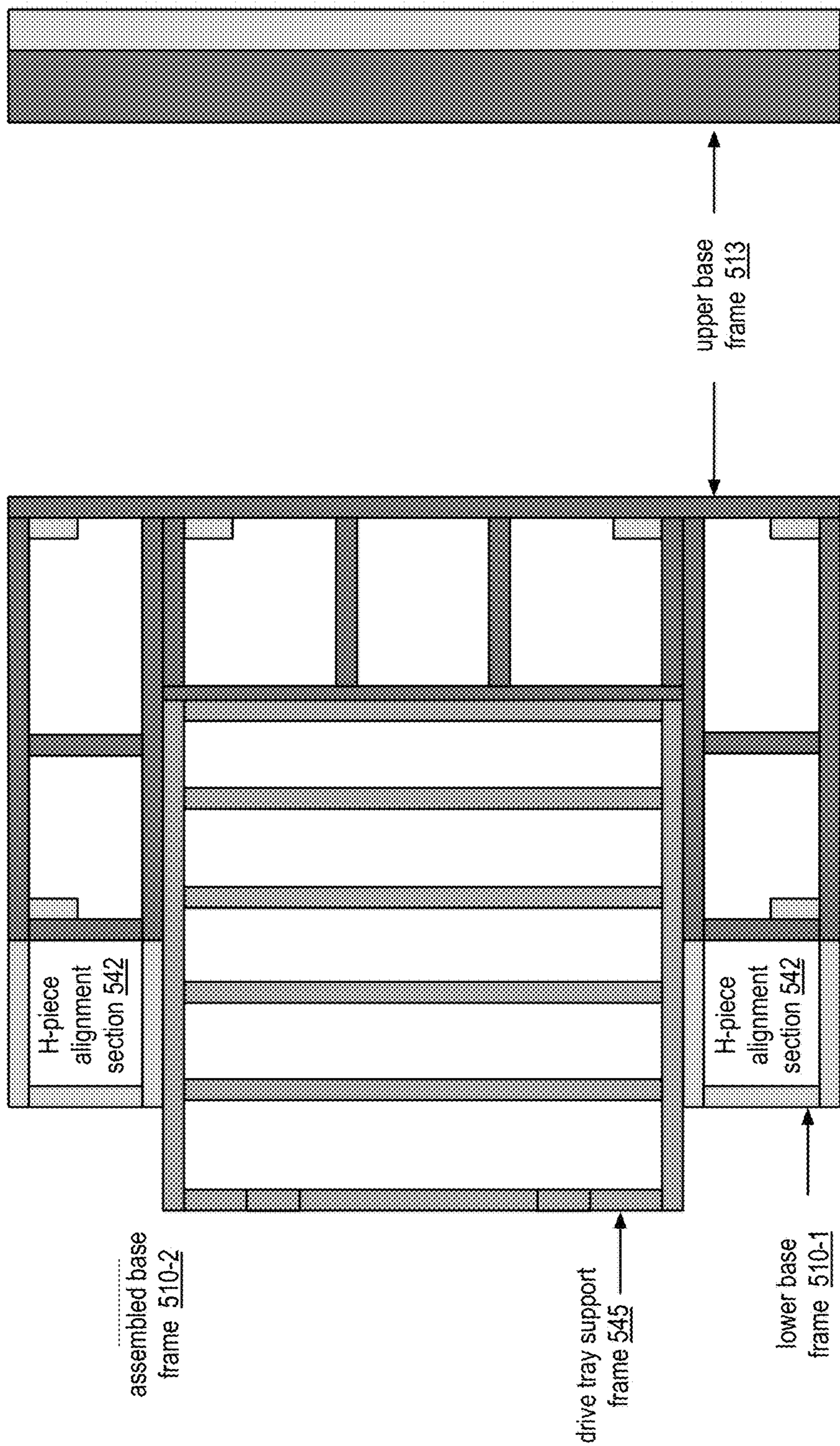
rear view FIG. 2J
