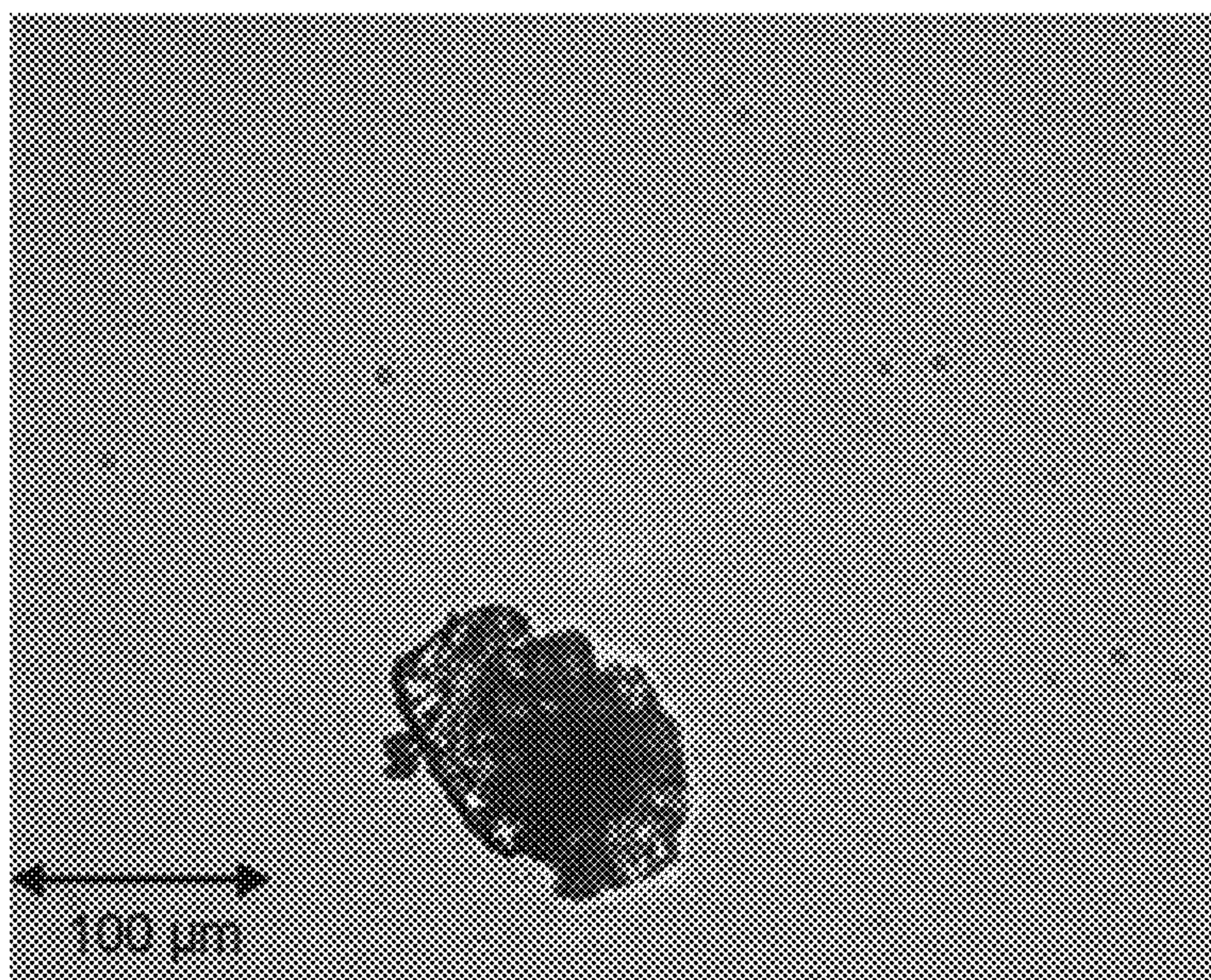
Unpolarised light
