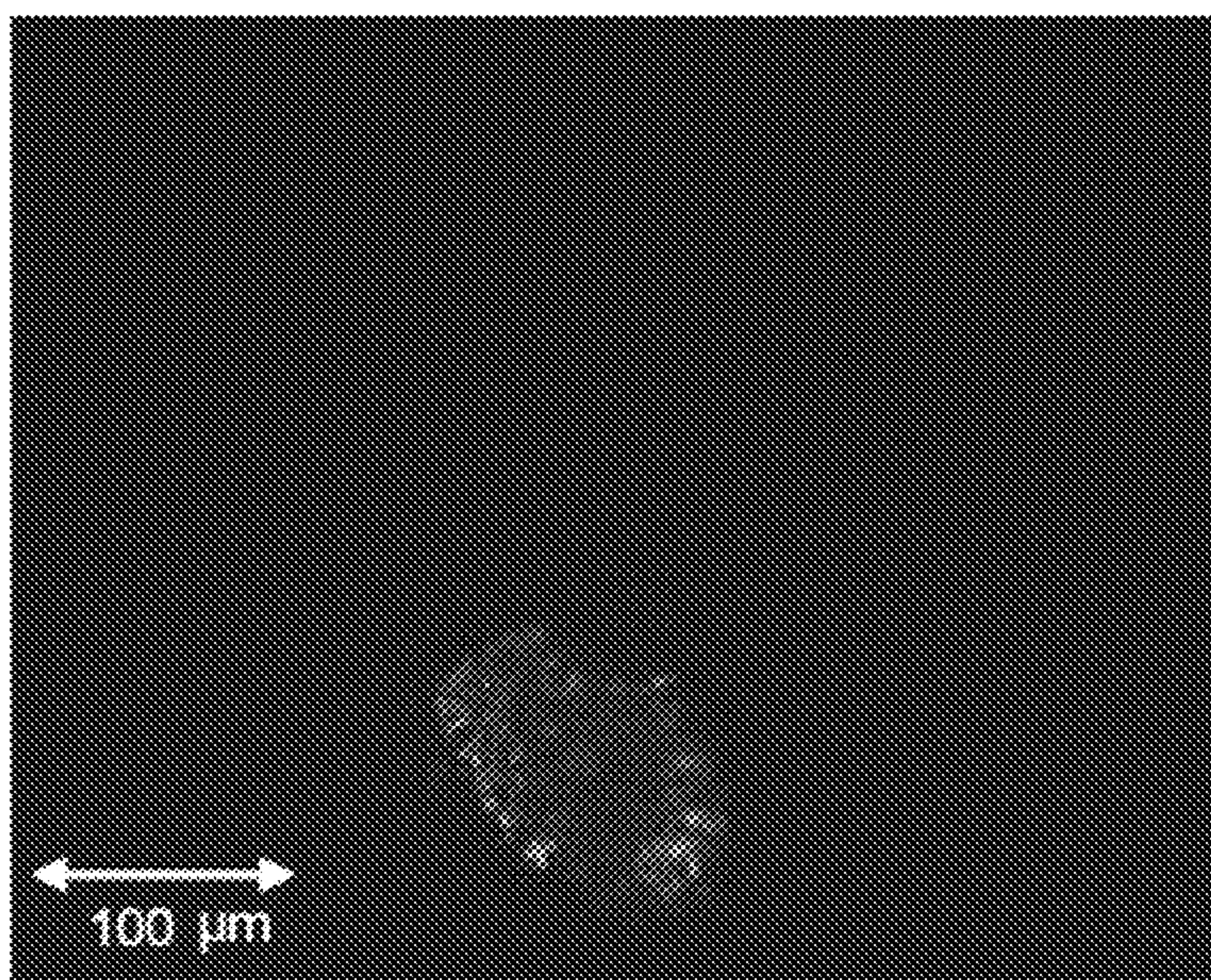
Polarised light
