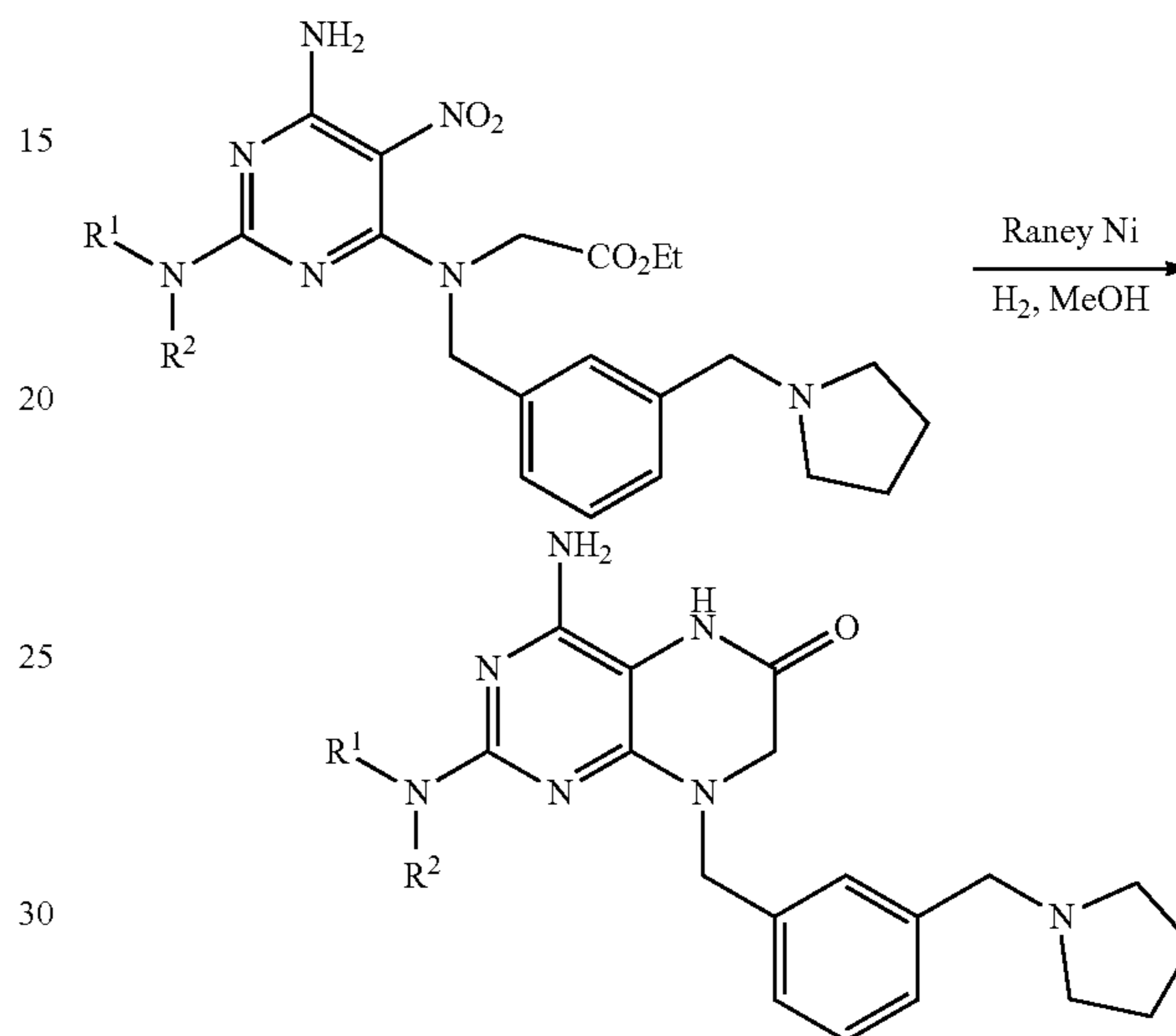
Scheme 17
