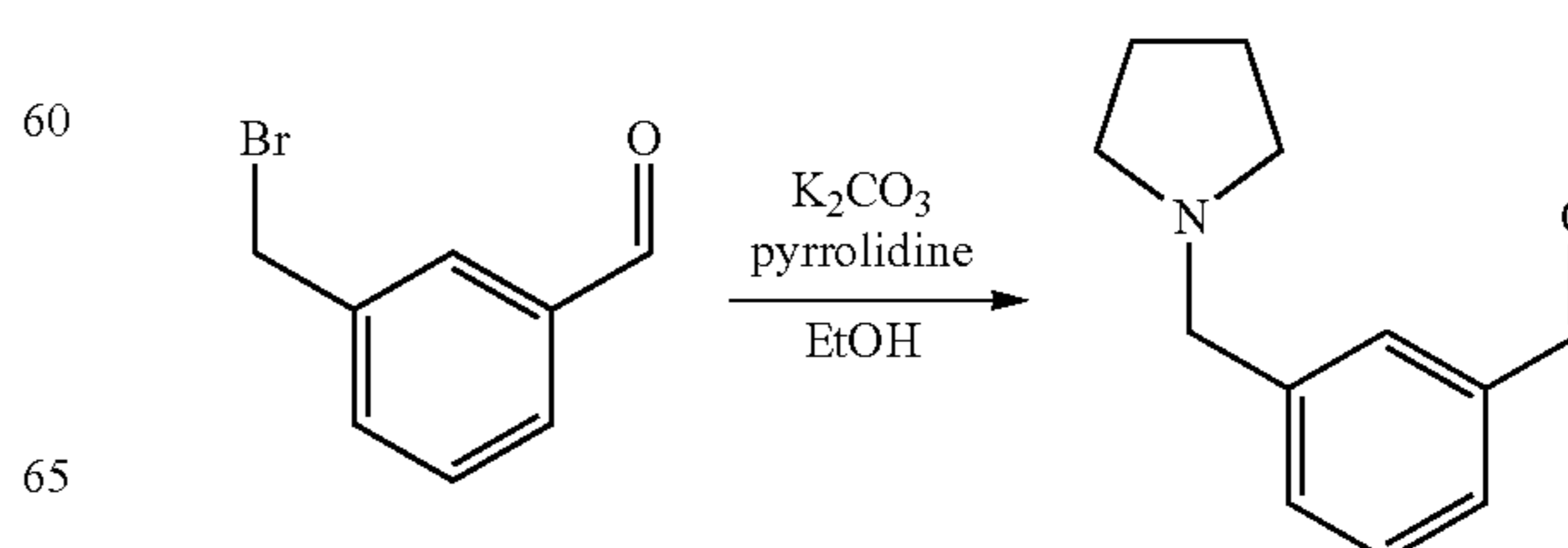
Scheme 4
