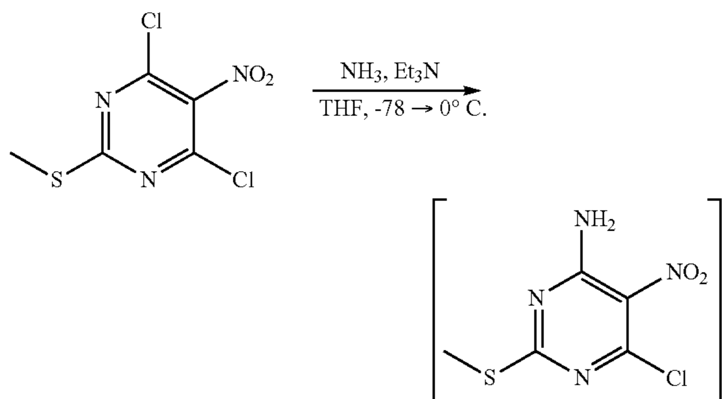
Scheme 34
