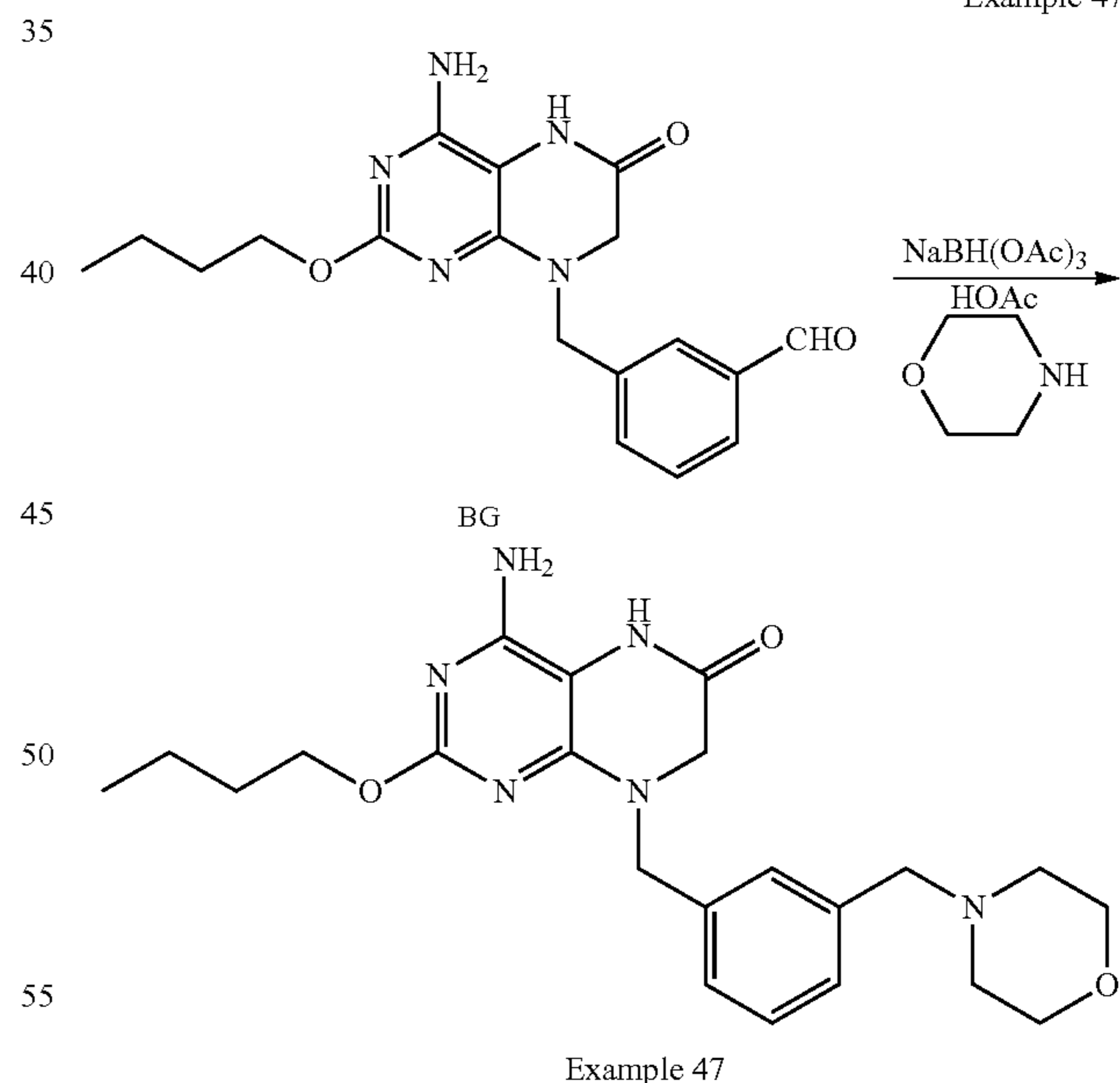
Scheme 25
