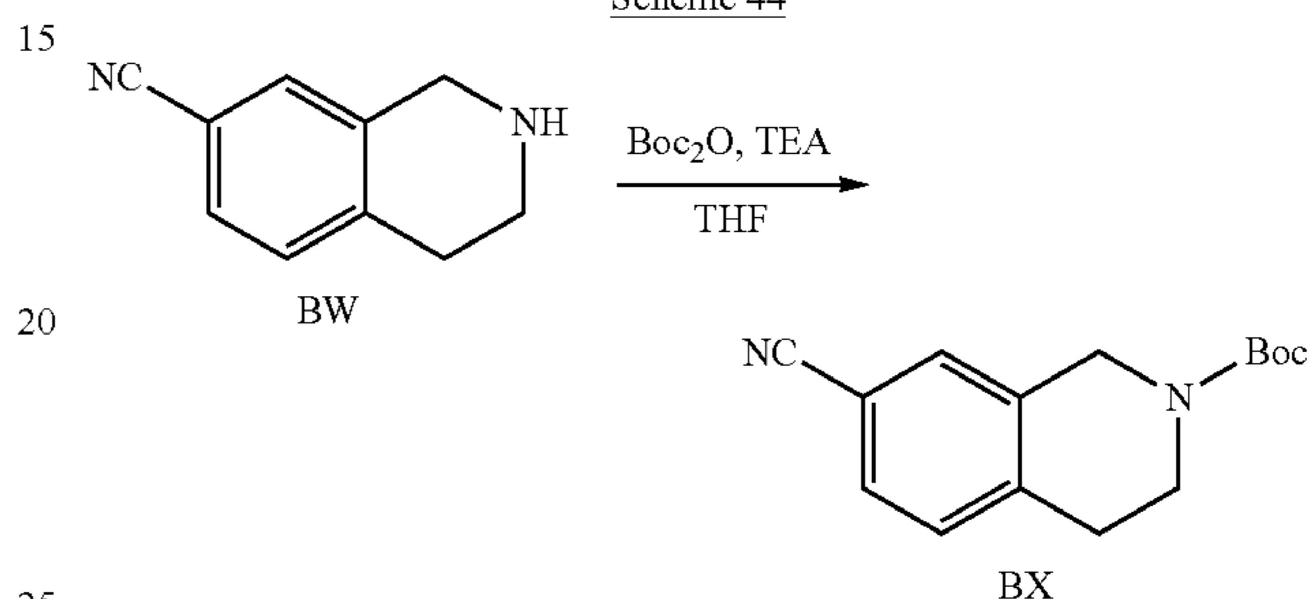
Scheme 44
