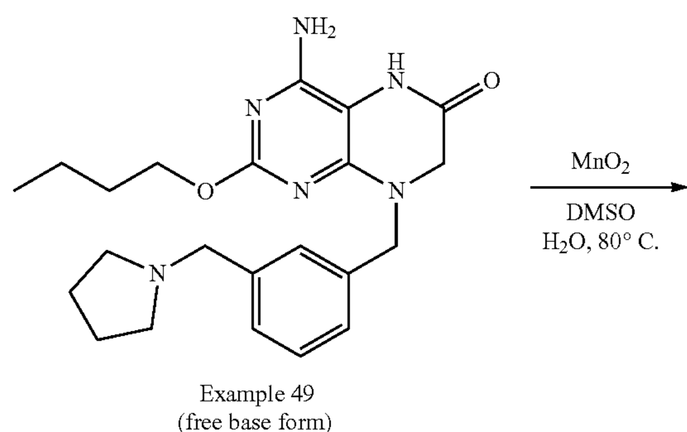
Scheme 87
