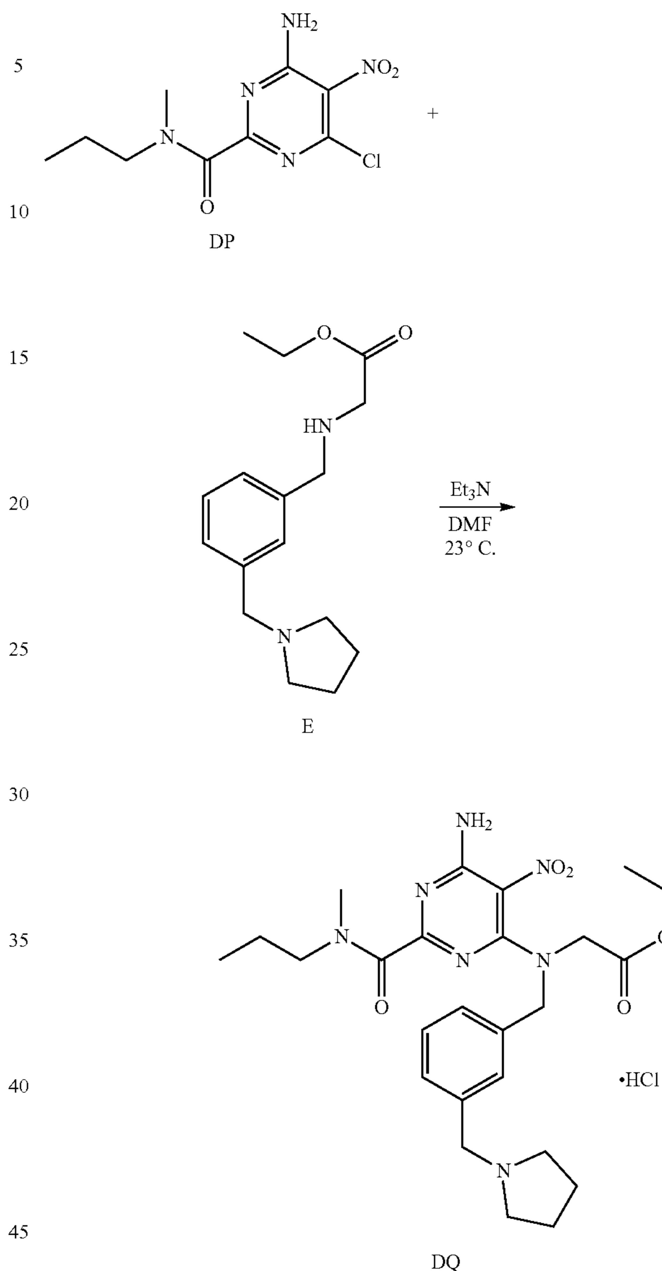
Scheme 83:
