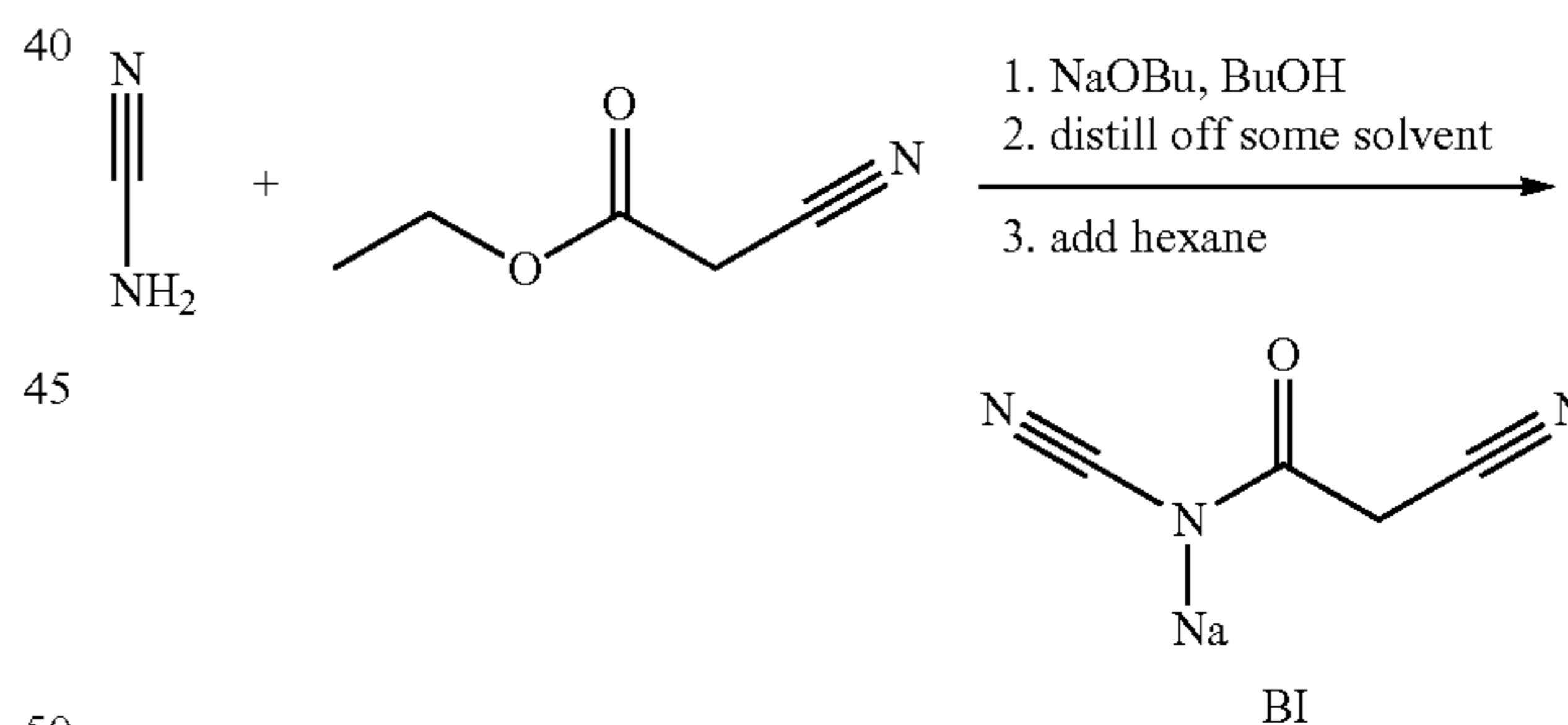
Scheme 27
