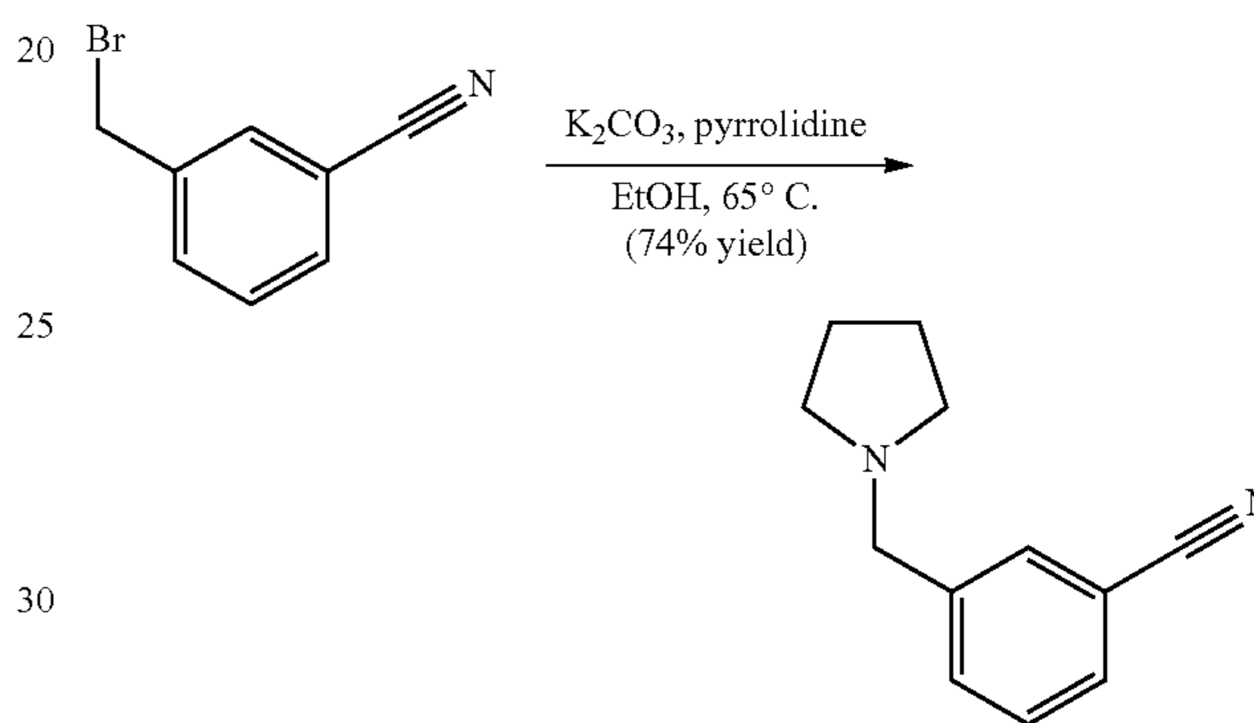
Scheme 3
