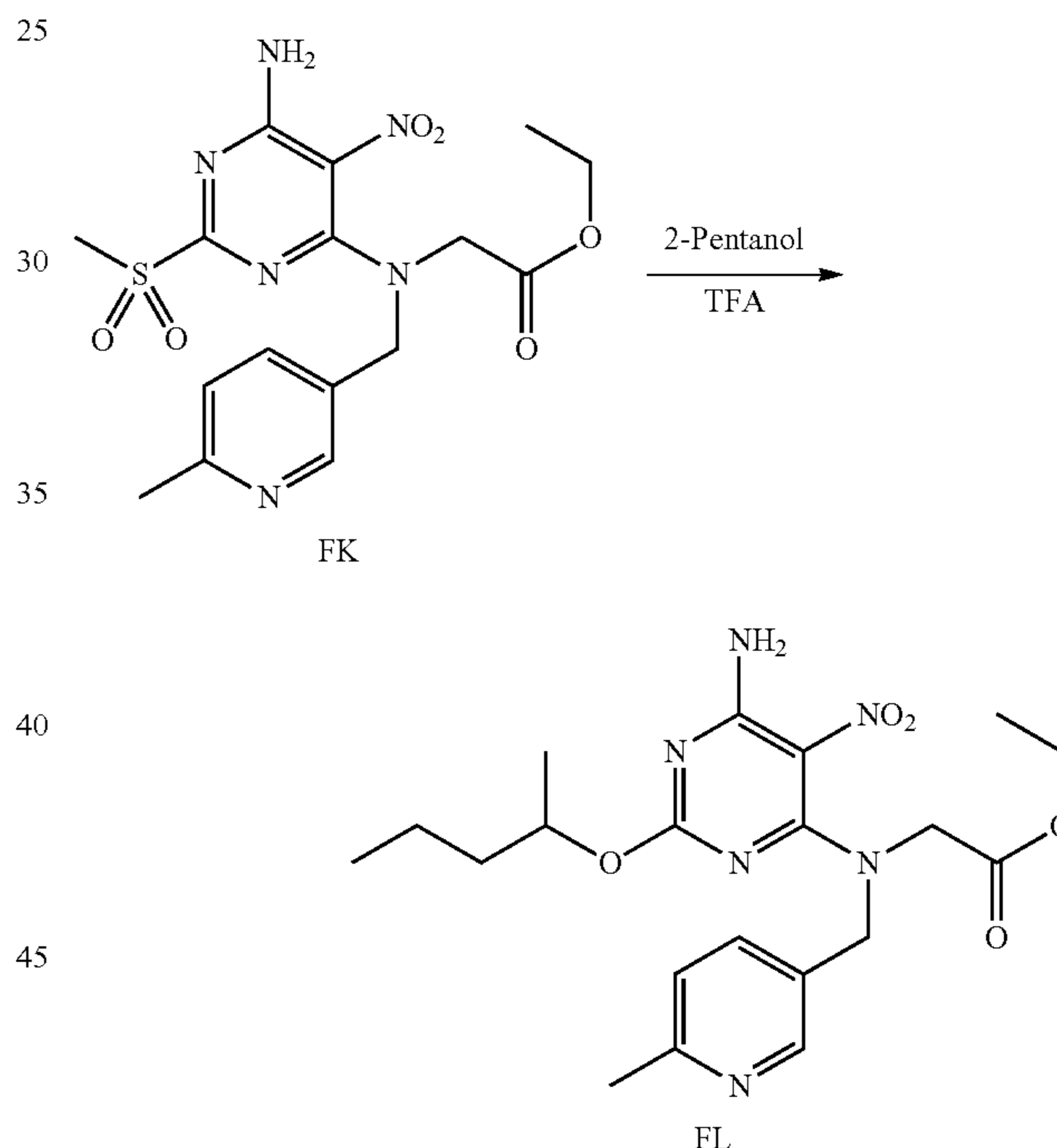
Scheme 100:
