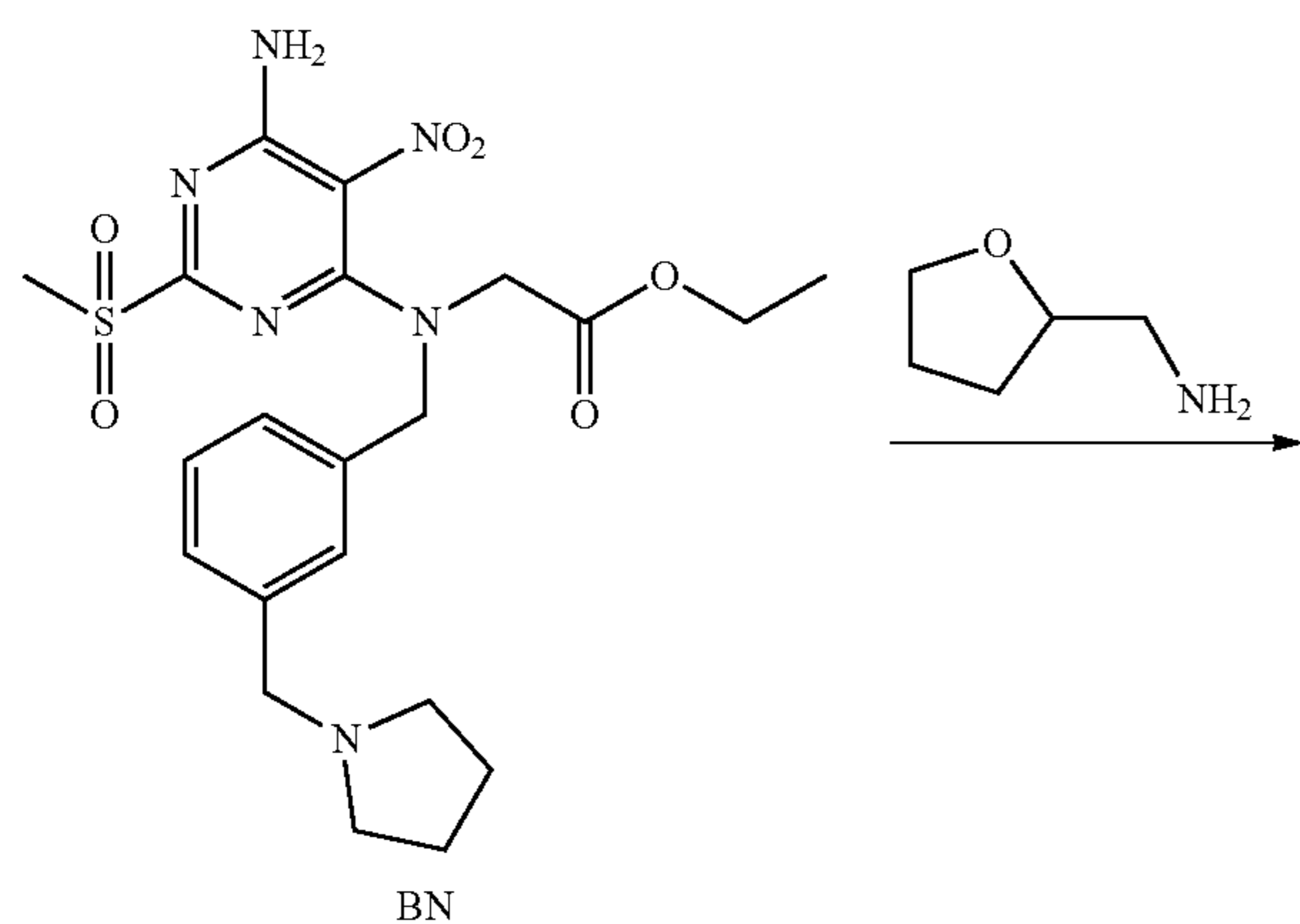
Scheme 68: Compound DE Prepared Via Method XIII
