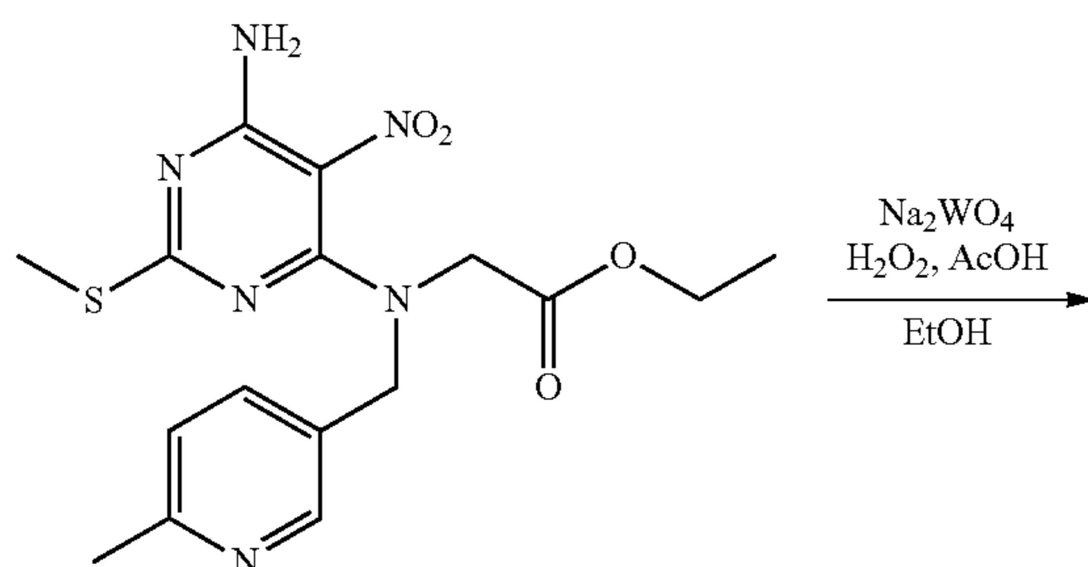
Scheme 99:
