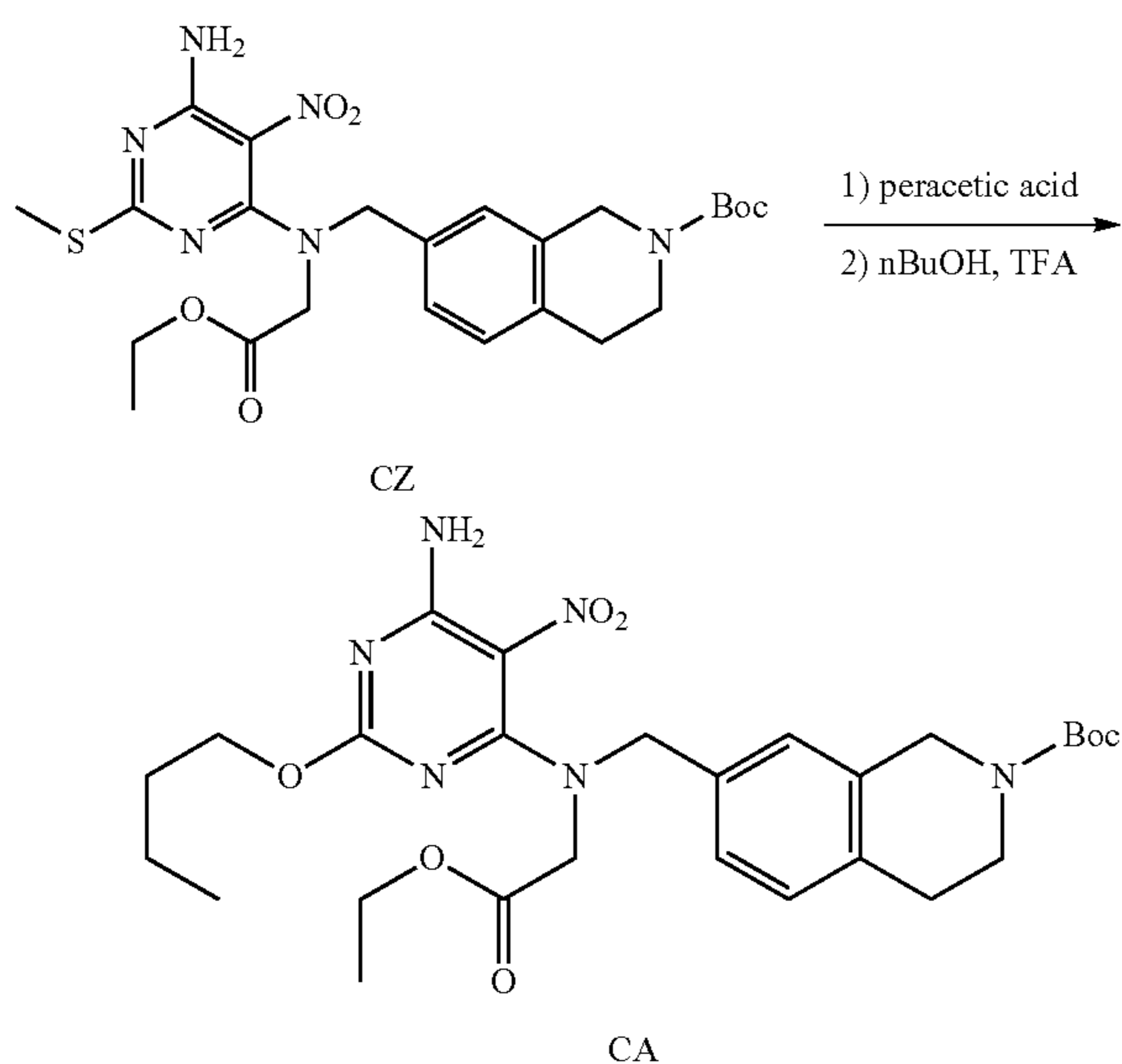
Scheme 60: Compound CA Prepared Via Method XVIII:
