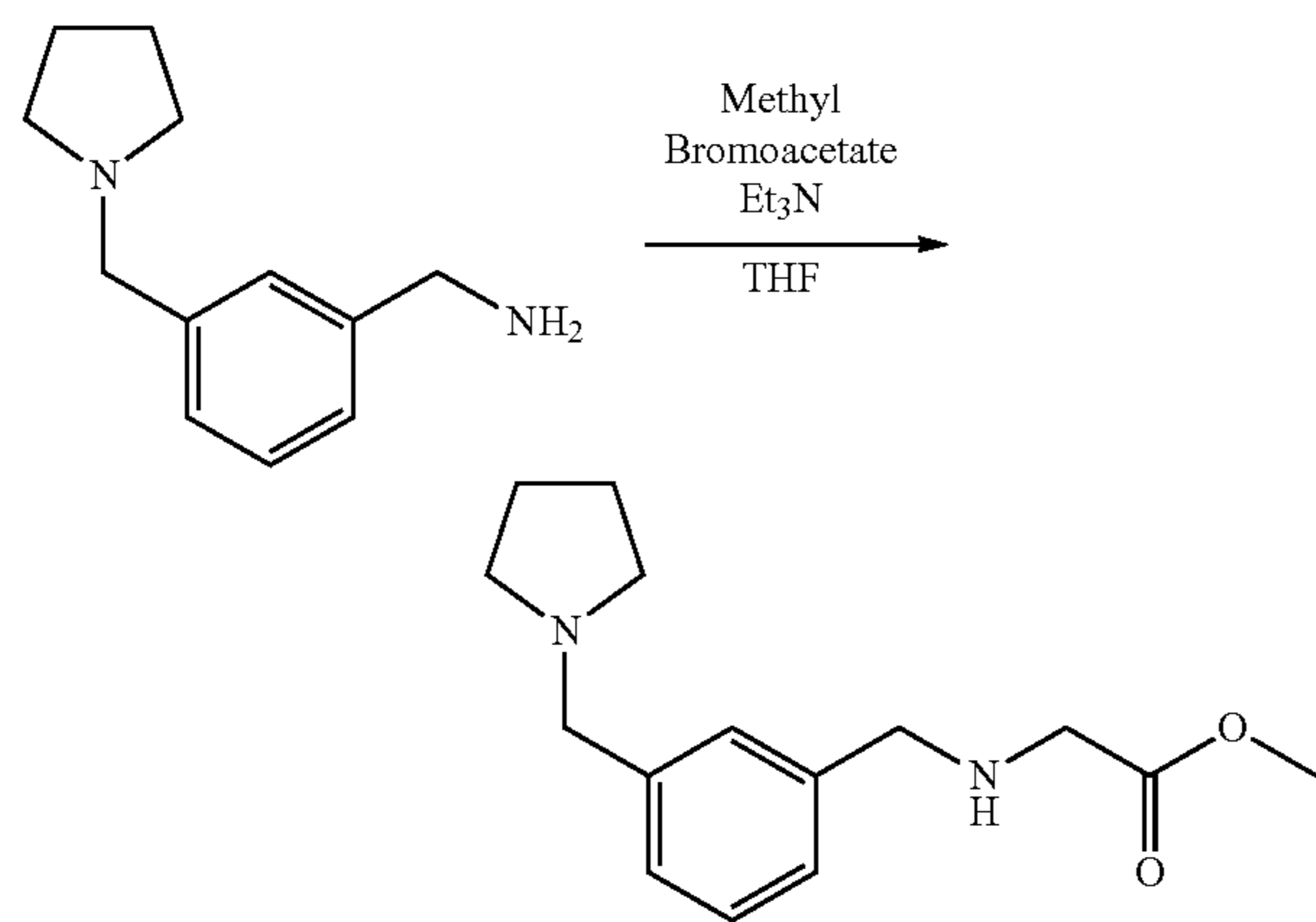
Scheme 20
