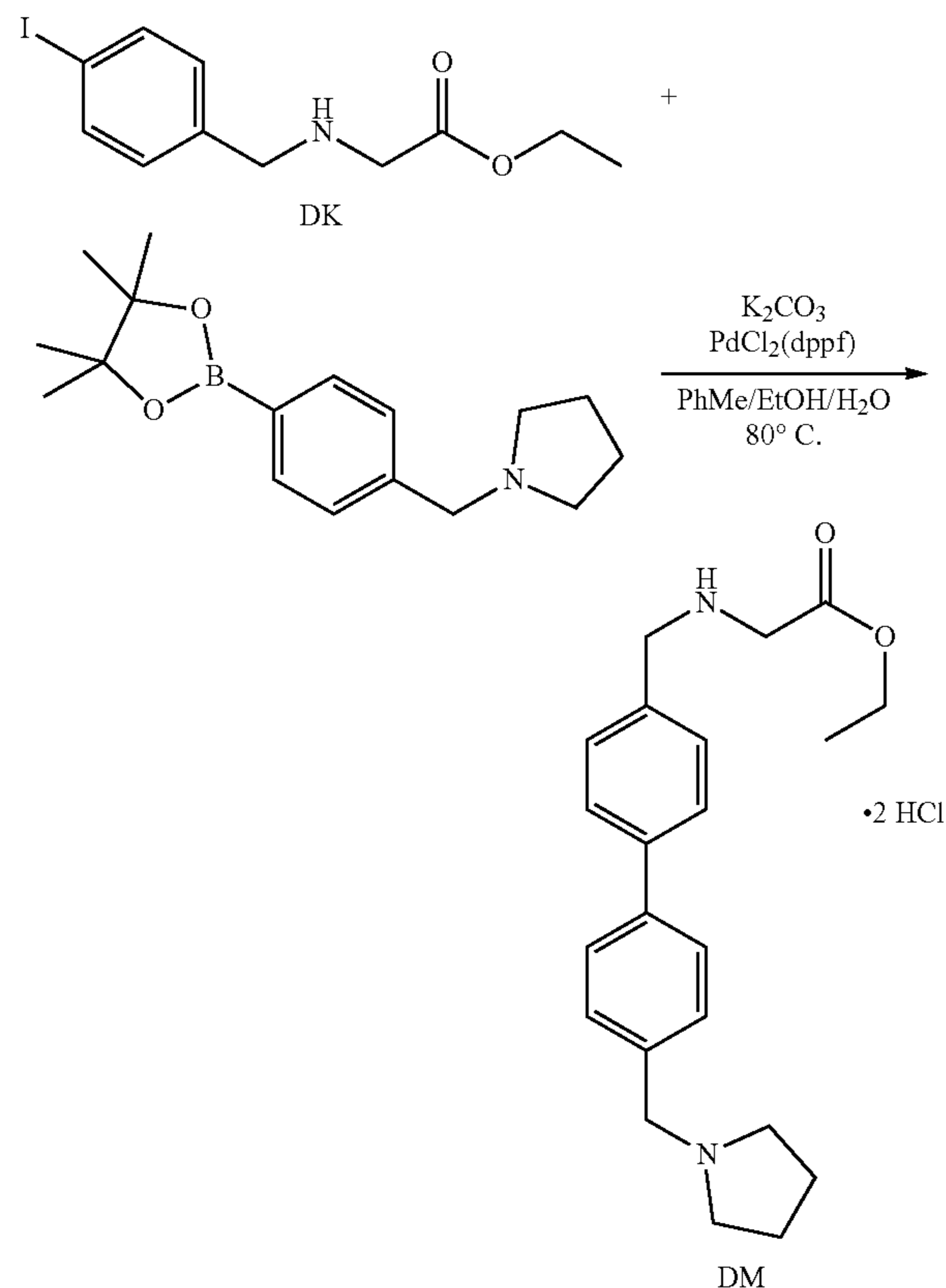
Scheme 79
