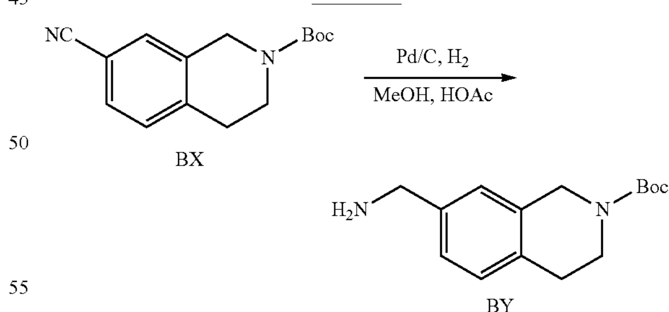
Scheme 45
