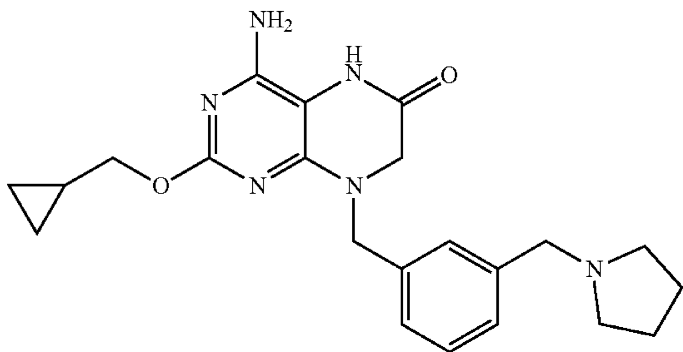
4-amino-2-((cyclopropyl)methoxy)-8-(3'-(pyrrolidin-1-ylmethyl)-benzyl)-5,6,7,8-tetrahydropteridin-6-one
