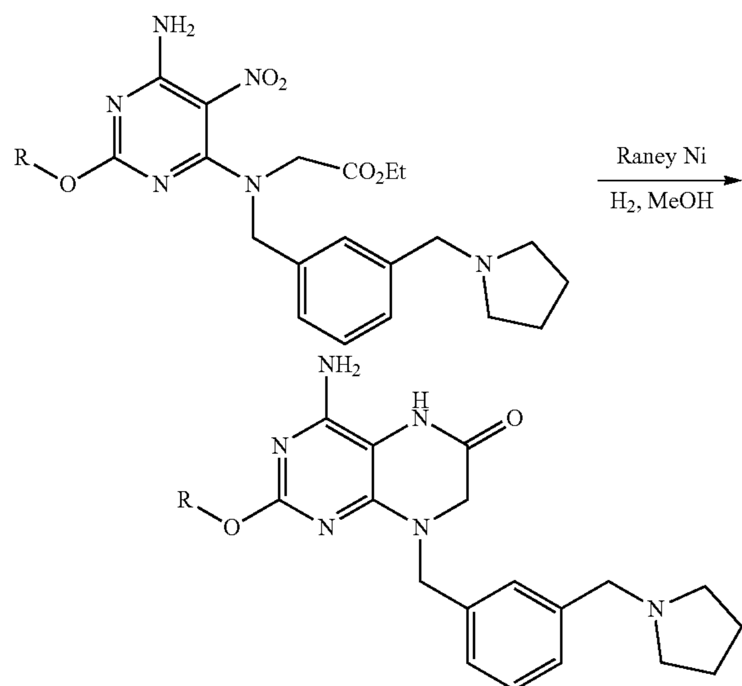
Scheme 15
