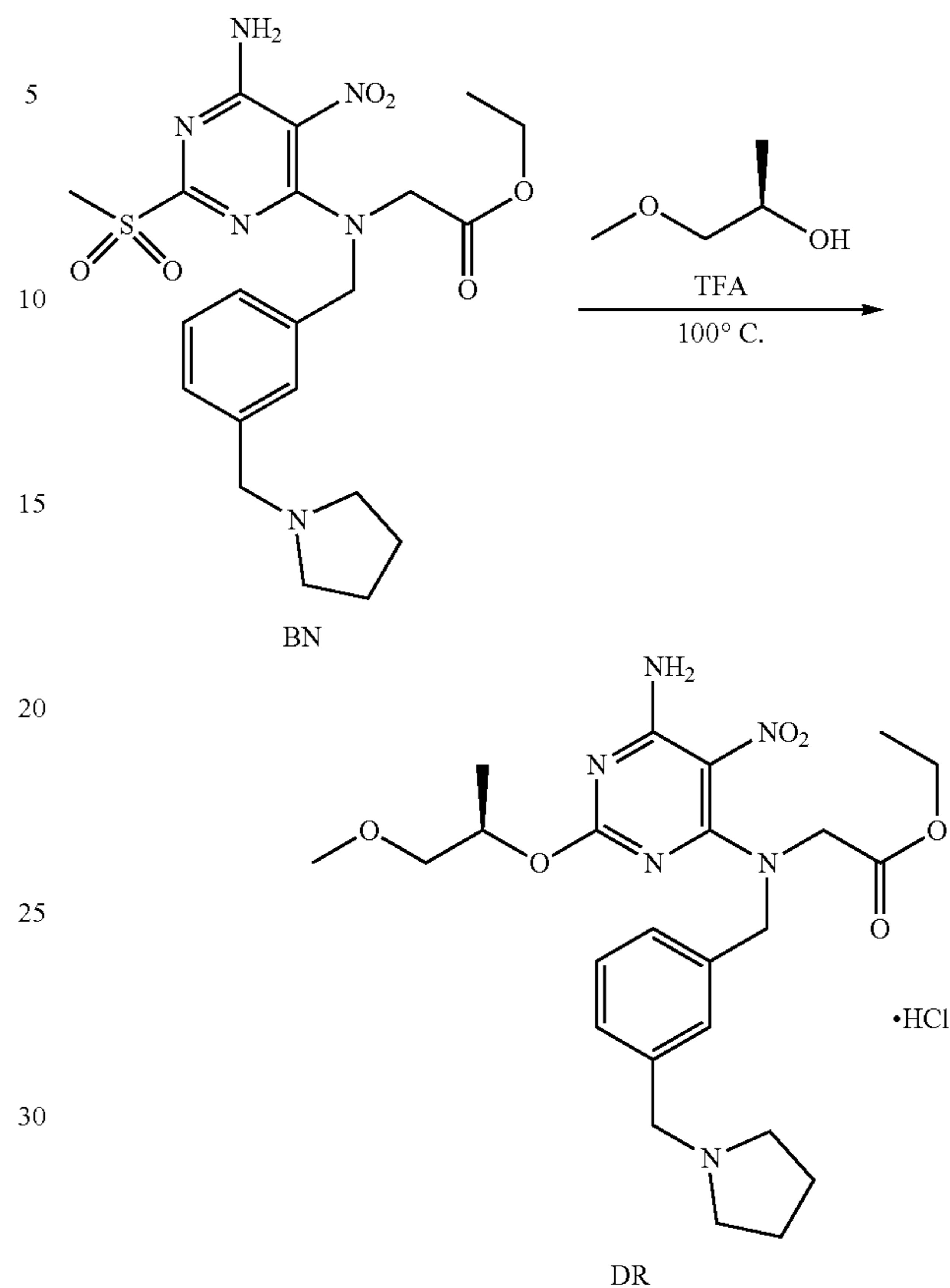
Method LXII: Compound ZZ
