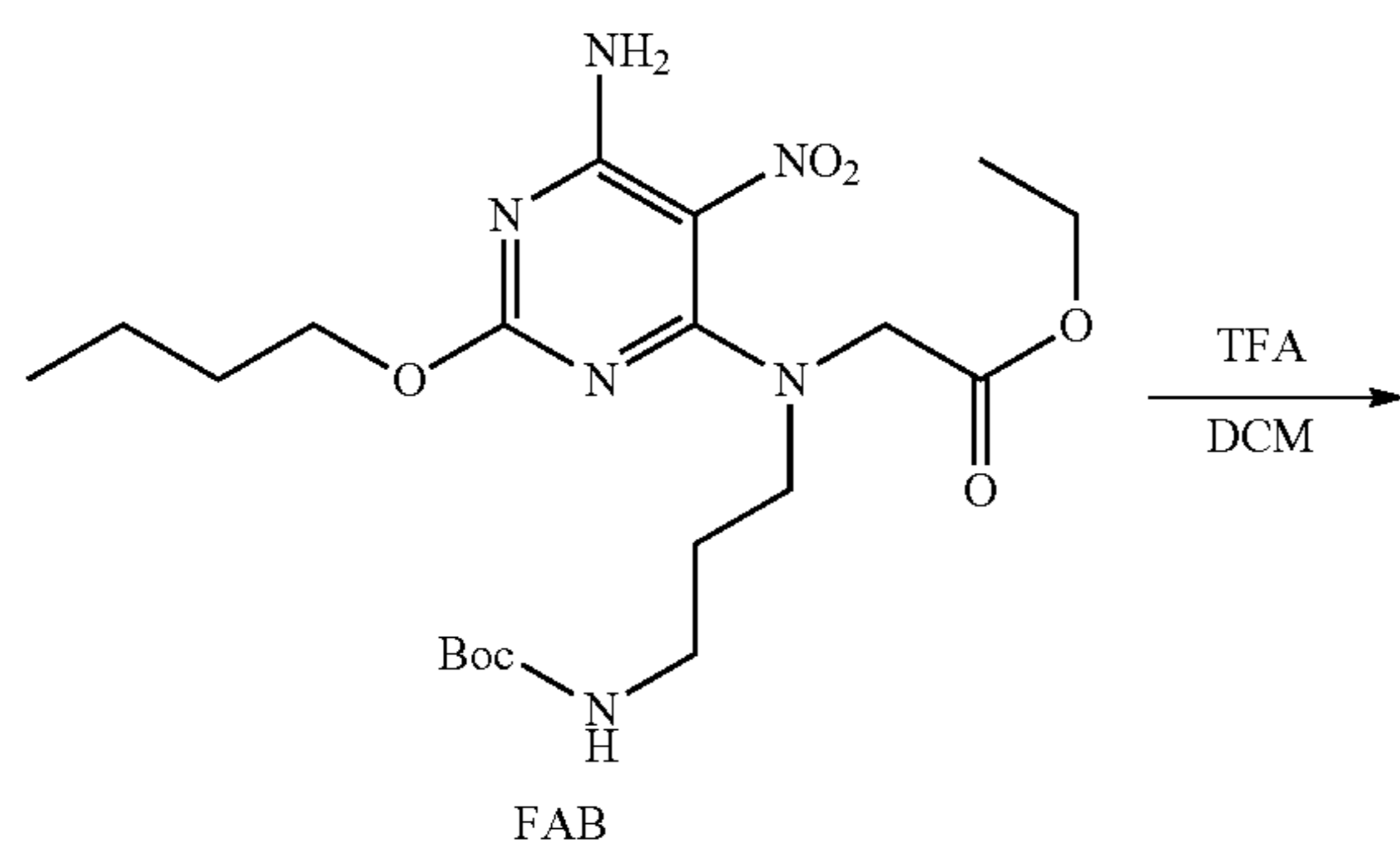
Scheme 105:
