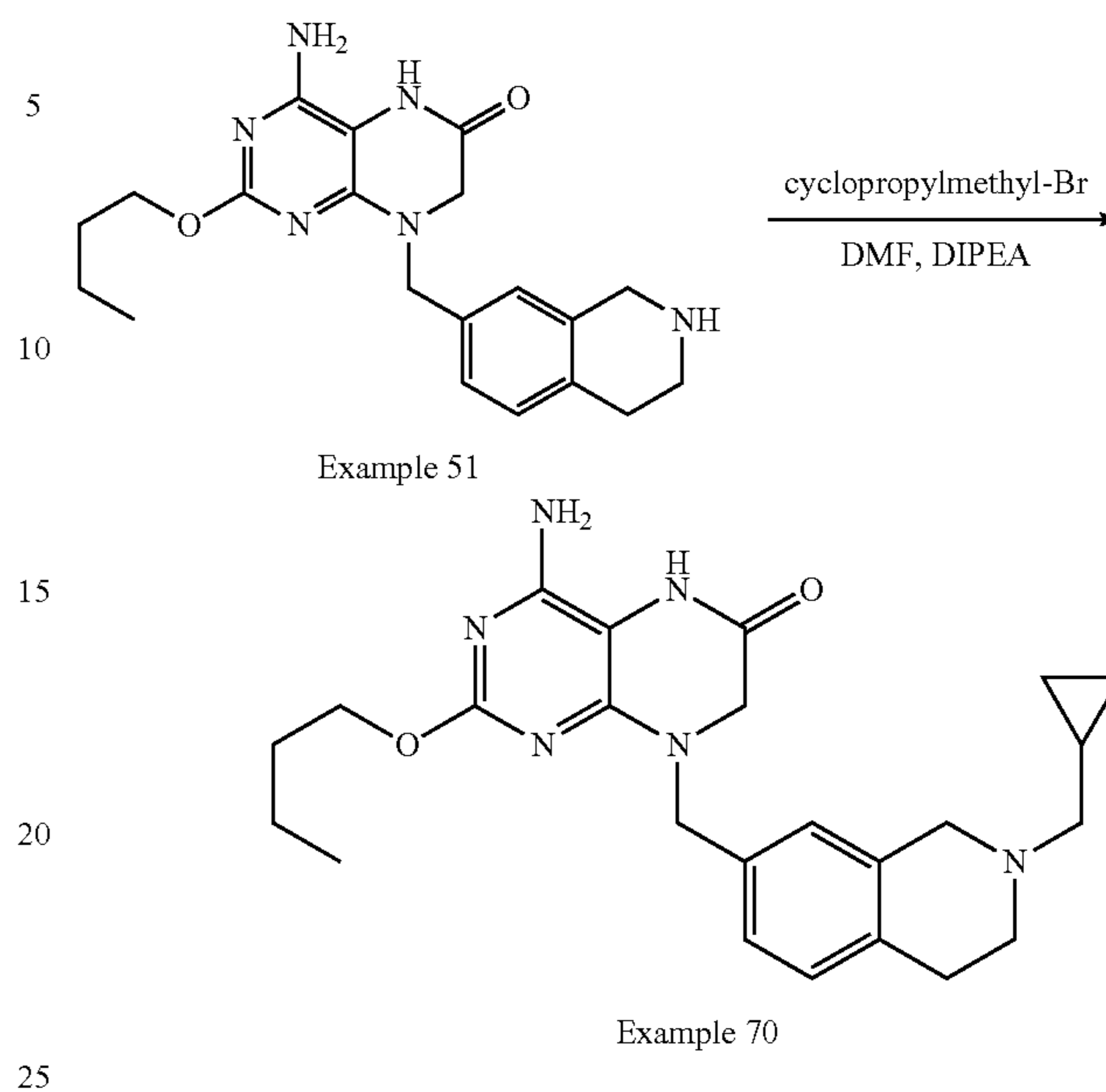
Scheme 61: Example 70, Method XLVIII
