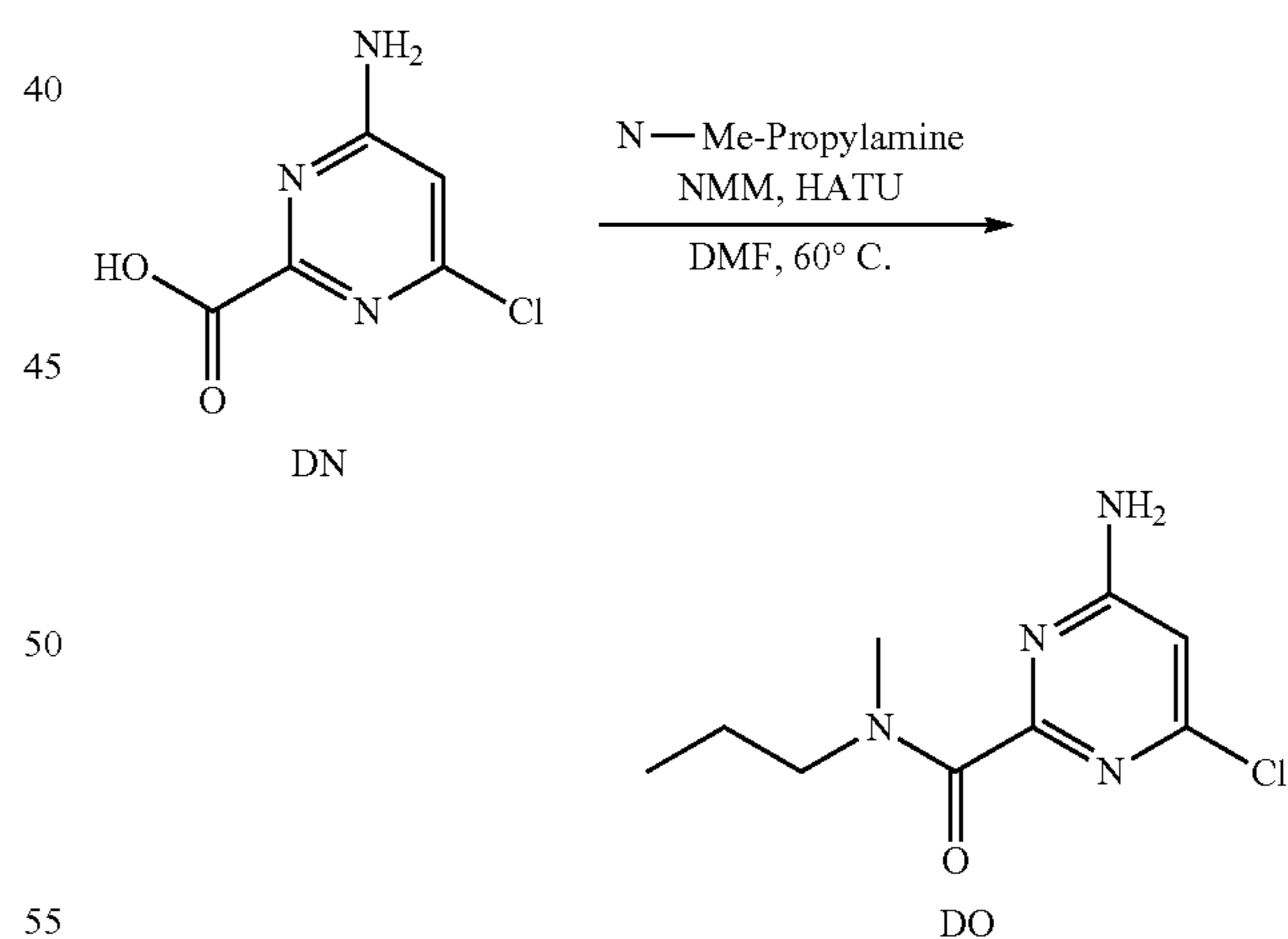
Scheme 81:
