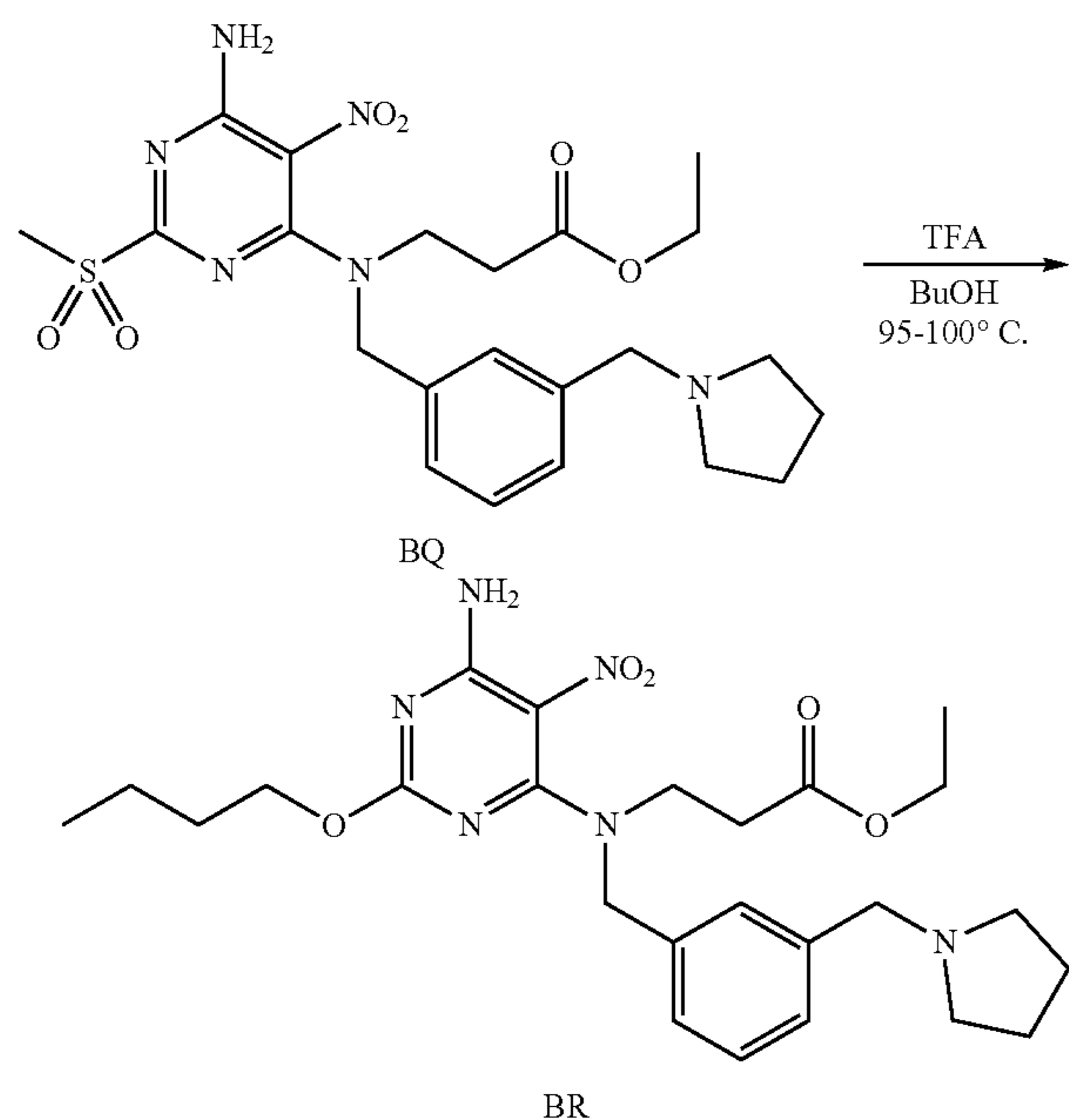
Scheme 37
