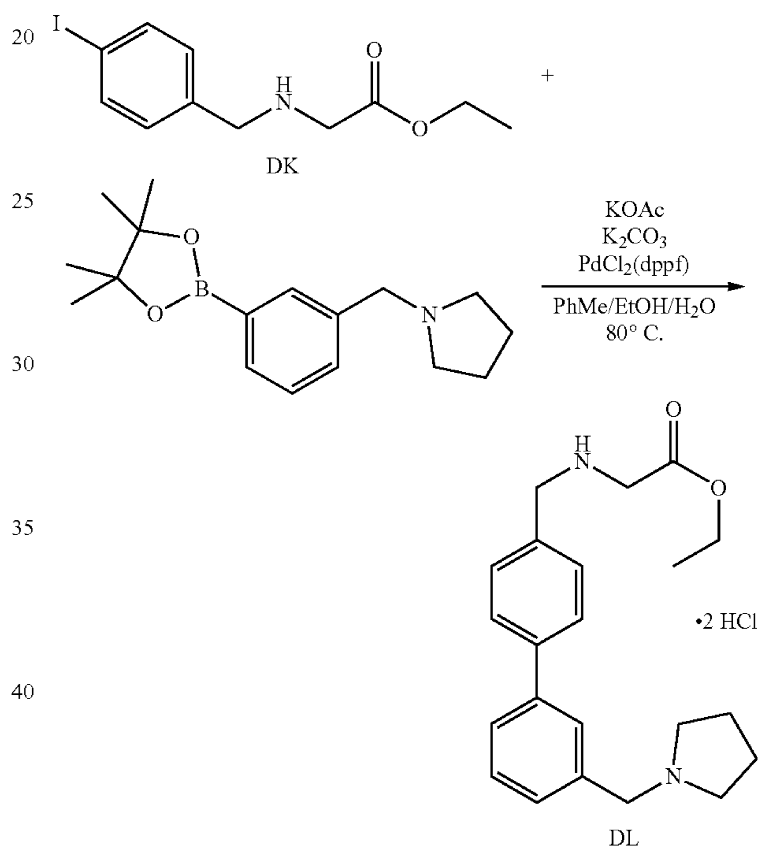
Scheme 78
