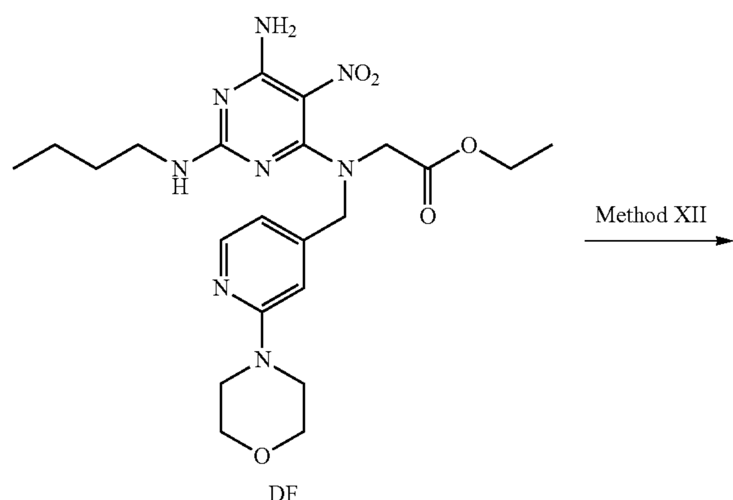
Scheme 71: Example 78, Method XII
