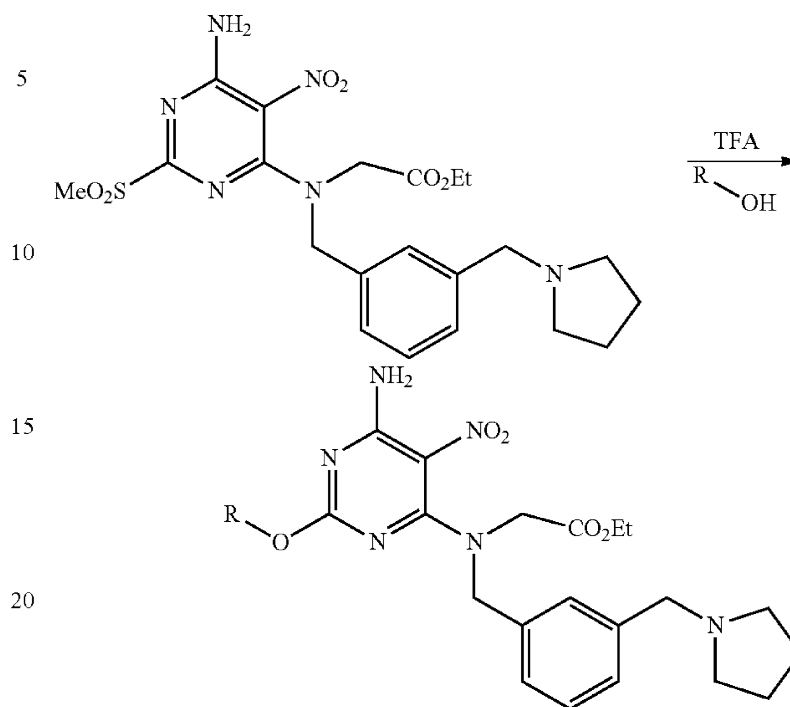
Scheme 13
