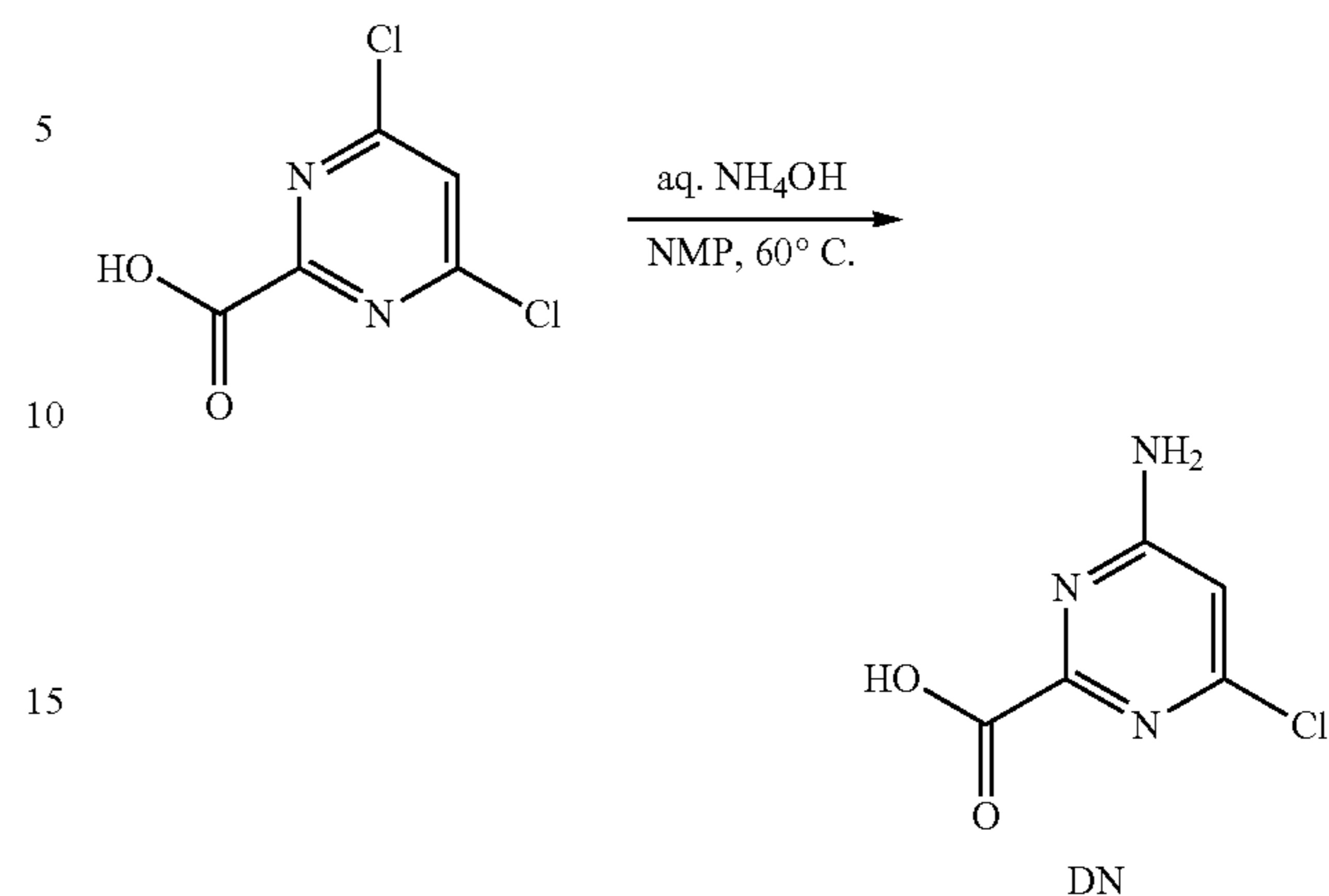
Scheme 80
