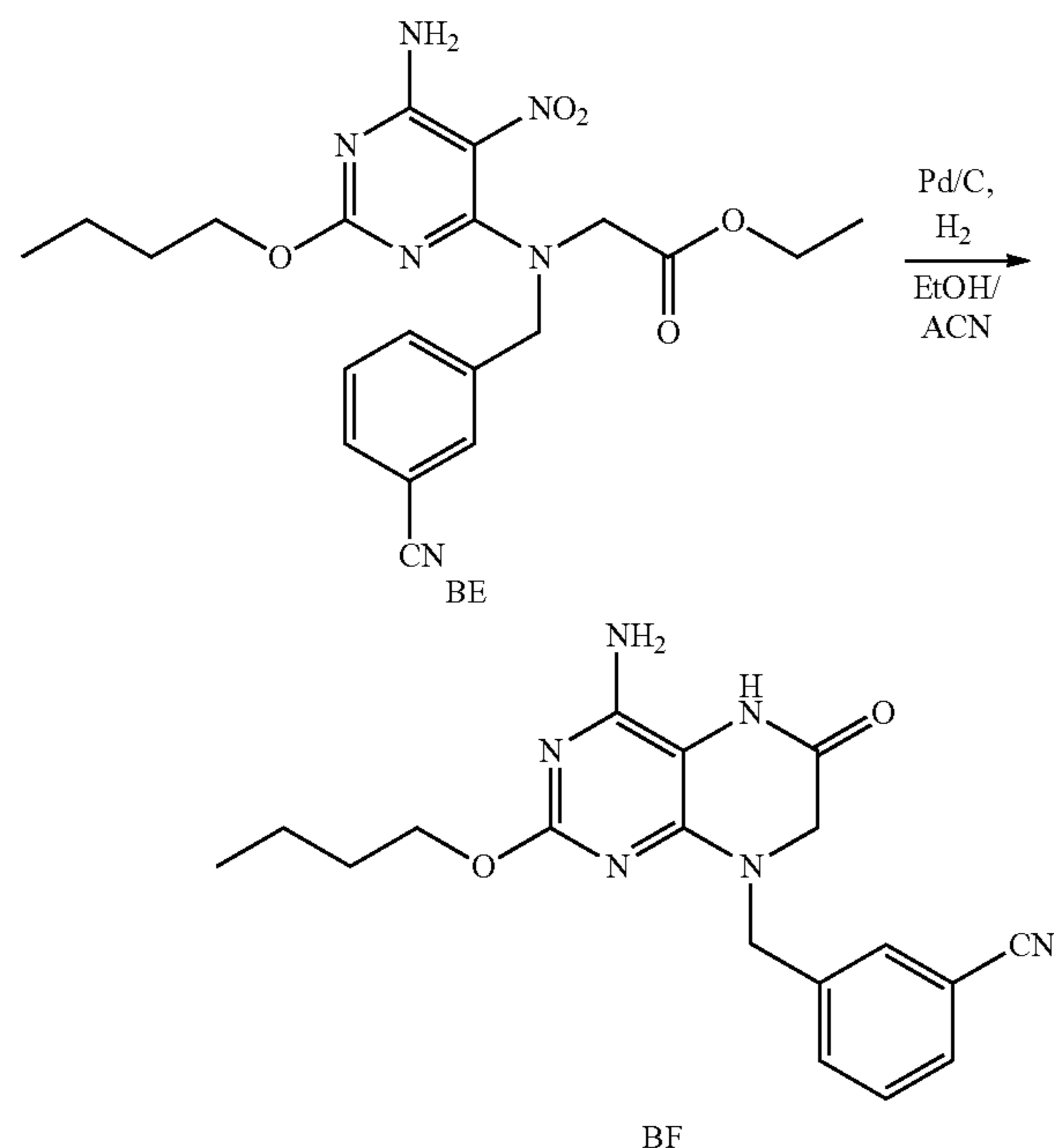
Scheme 23
