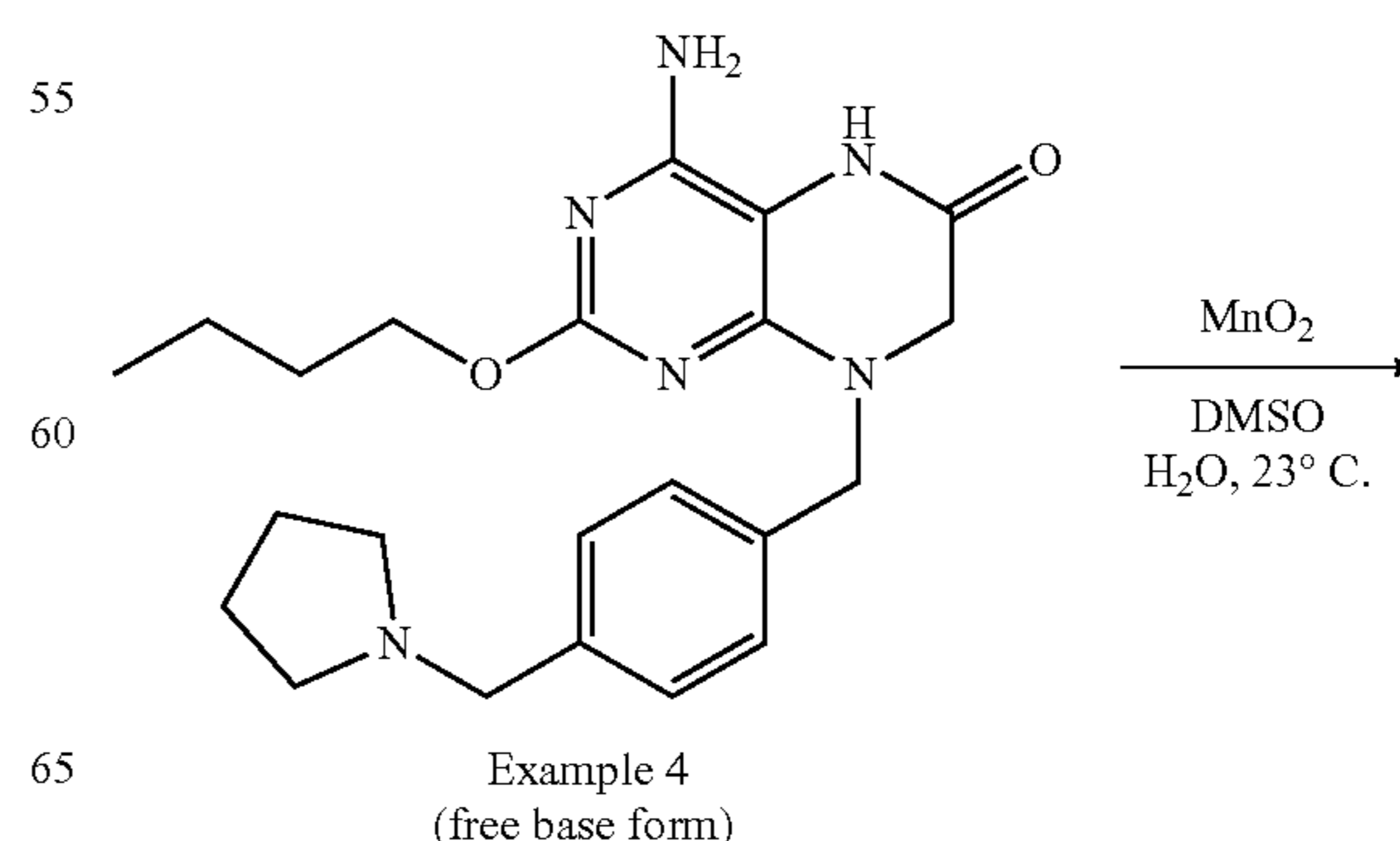
Scheme 88:
