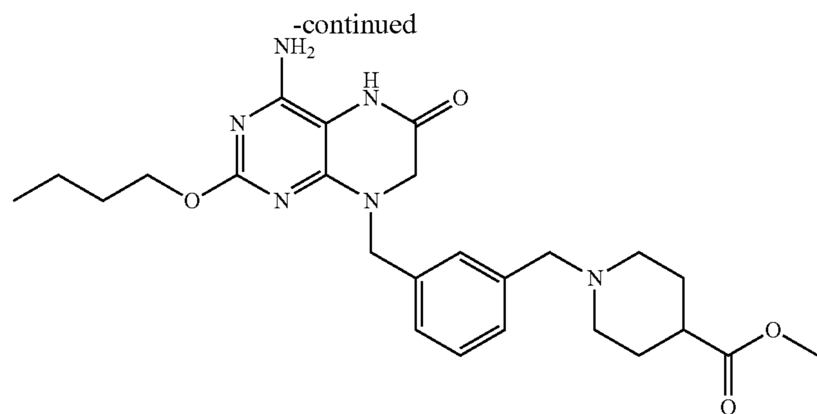
Example 54
