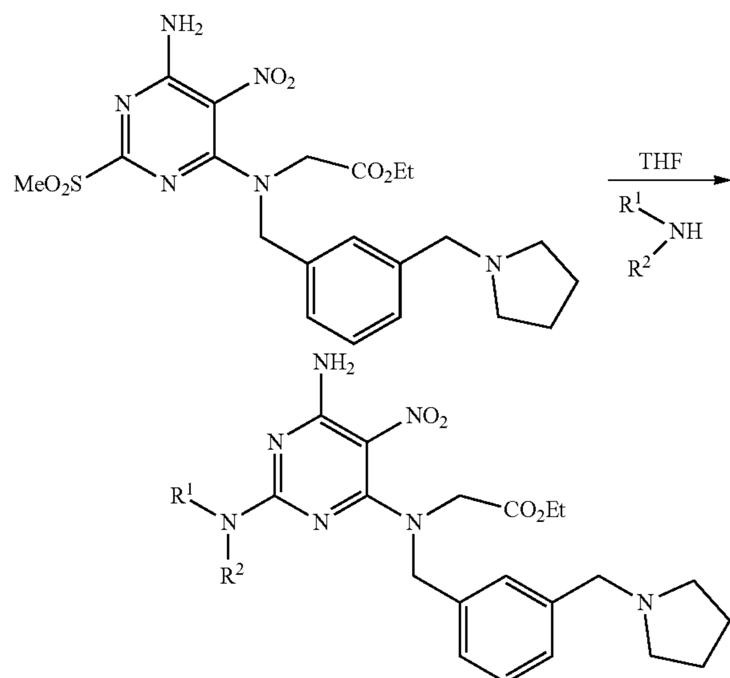
Scheme 16
