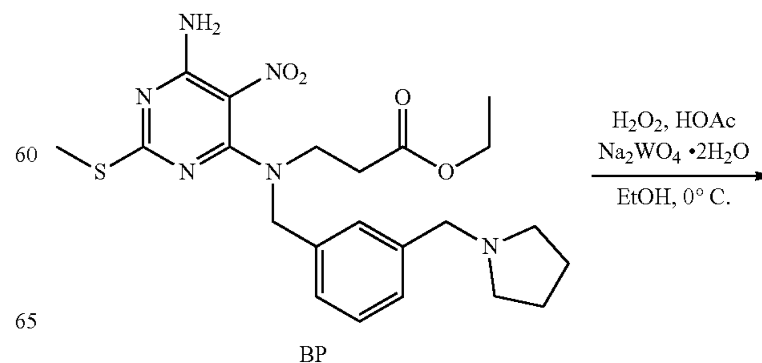
Scheme 36
