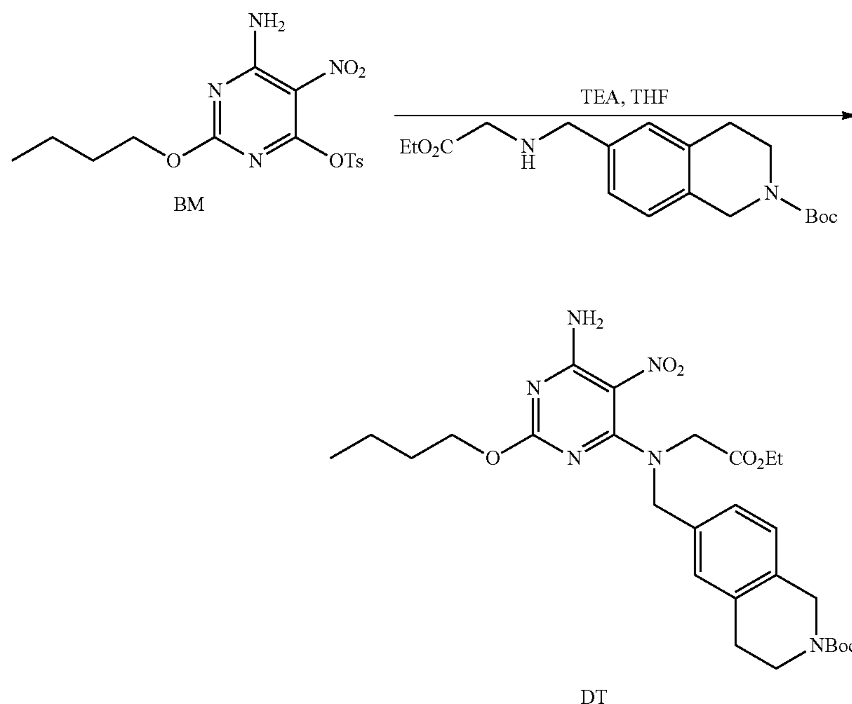
Scheme 89:
