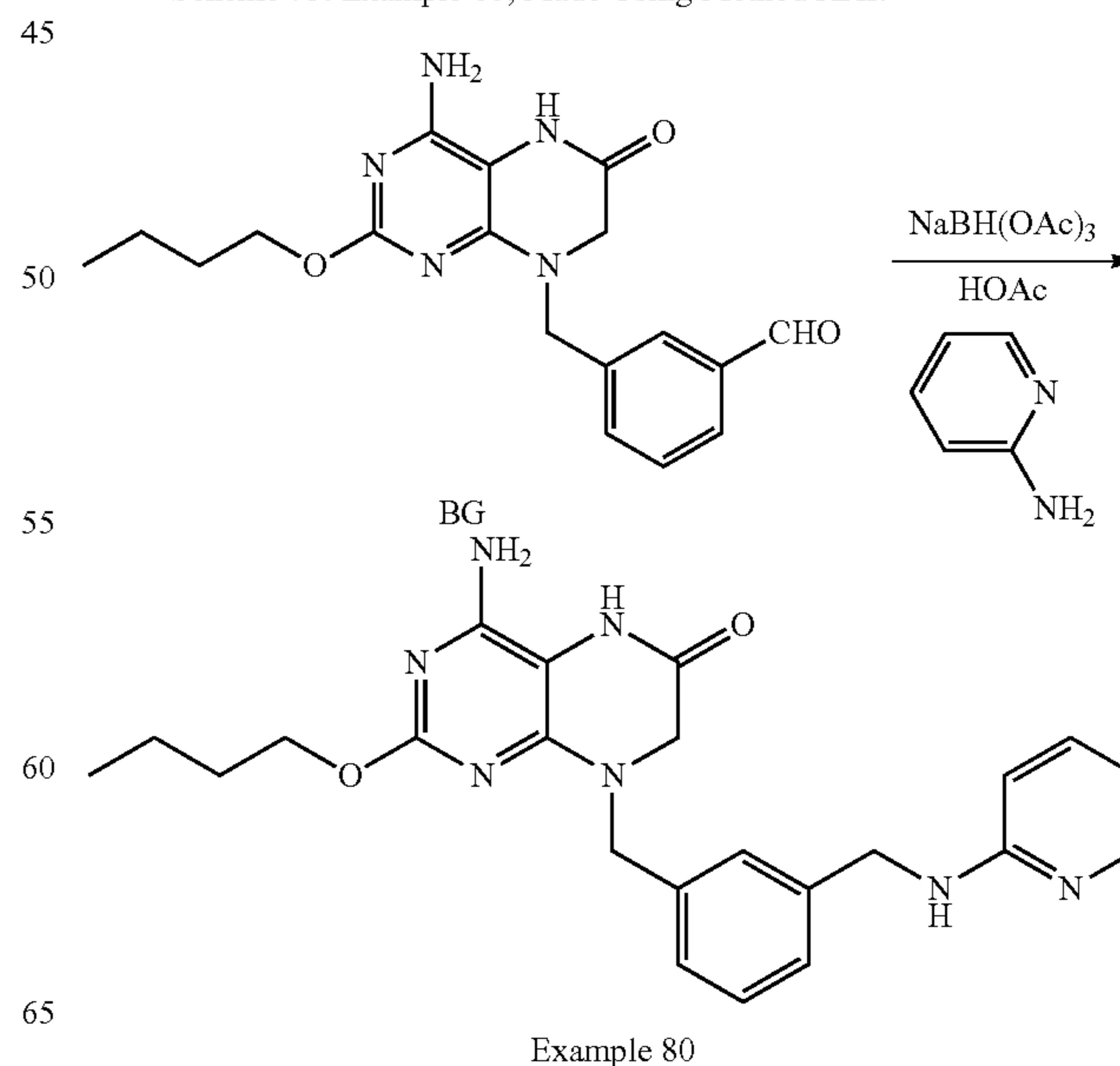
Scheme 73: Example 80, Made Using Method XXI:
