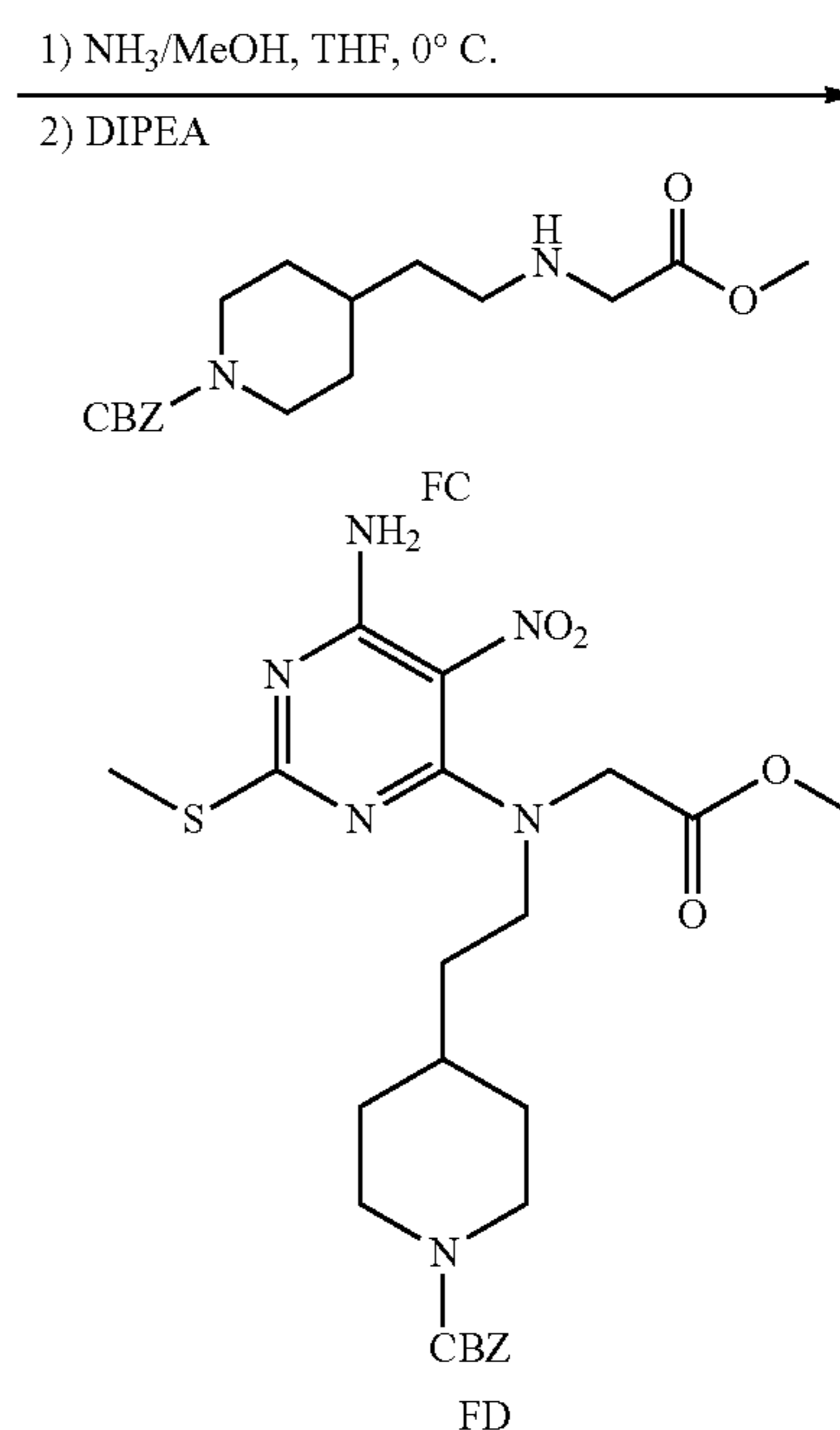
Scheme 92
