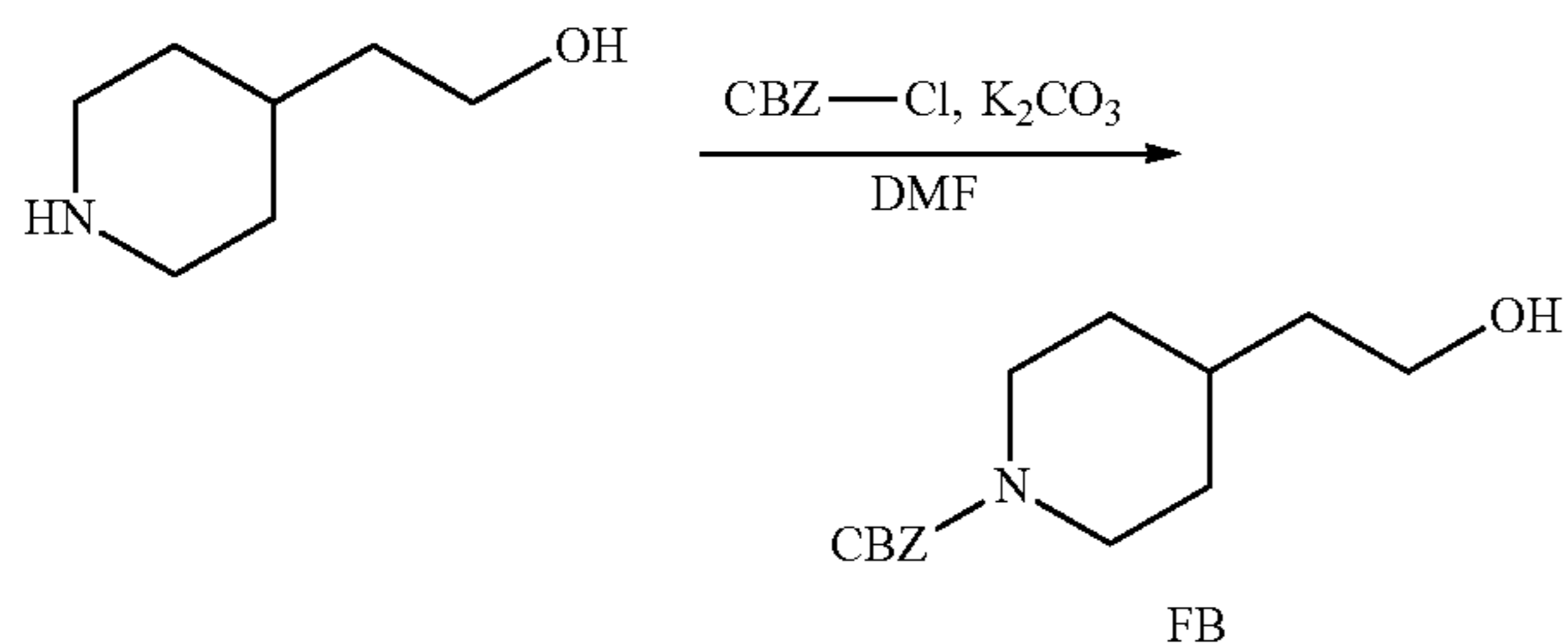
Scheme 90
