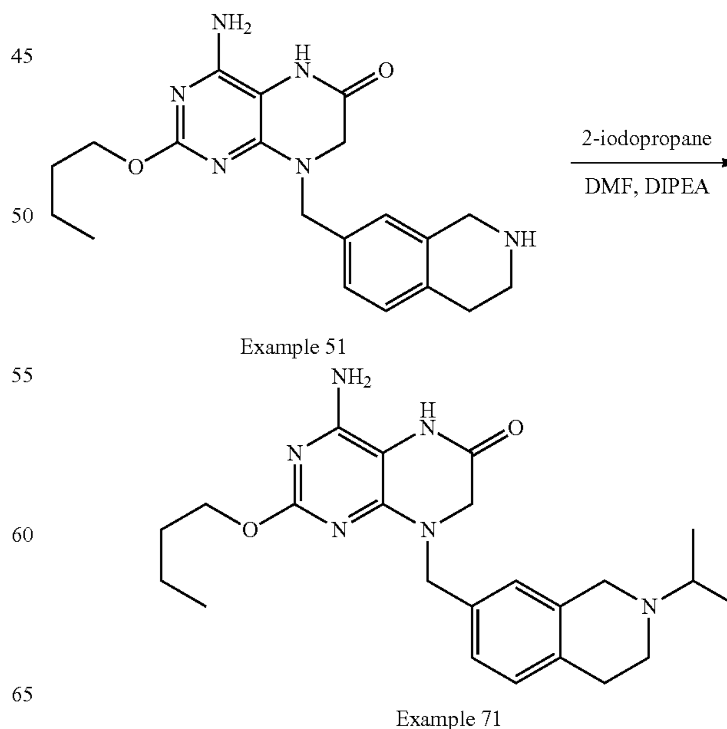
Scheme 62: Example 71, Method XLVIII:
