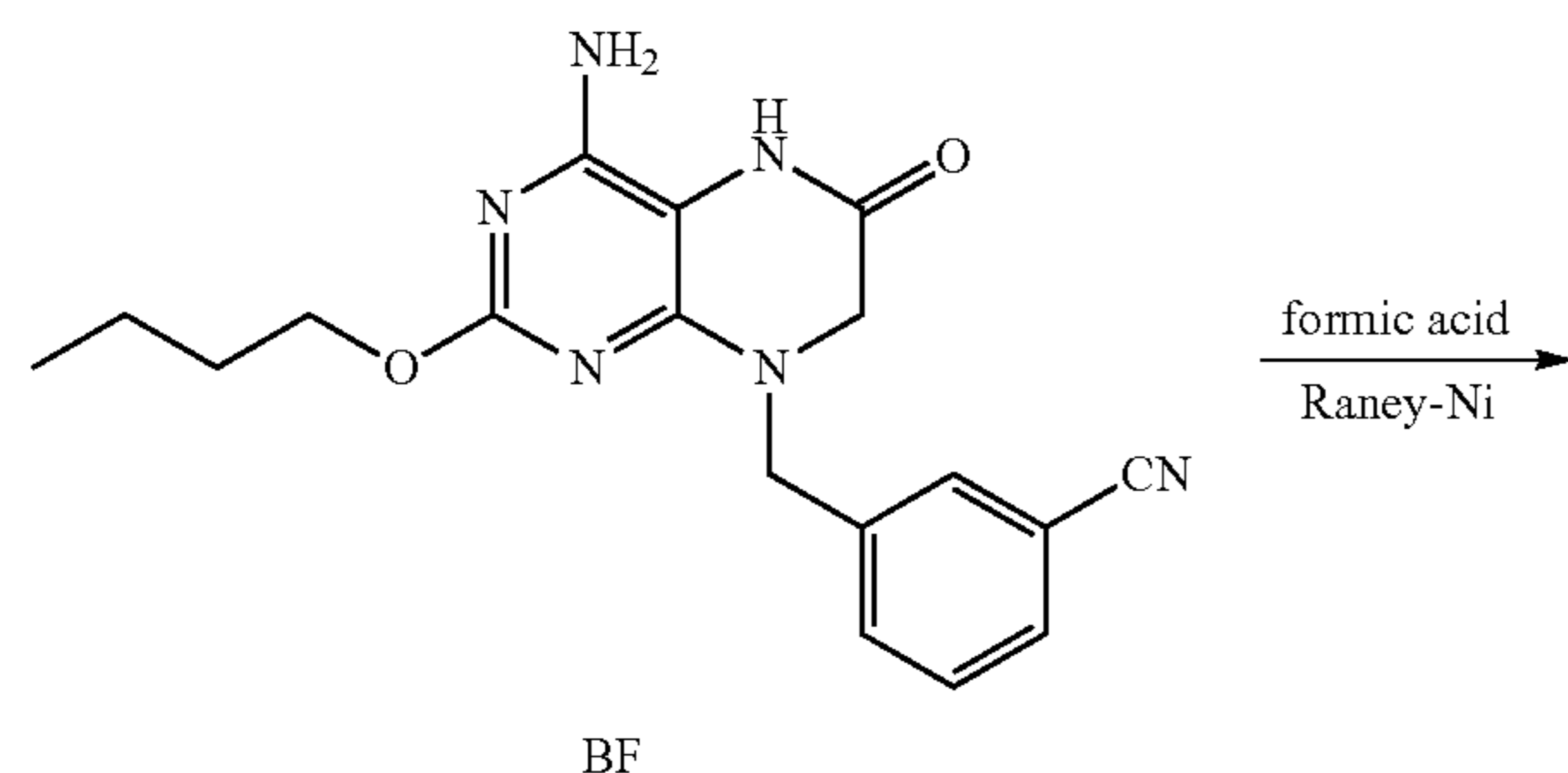
Scheme 24
