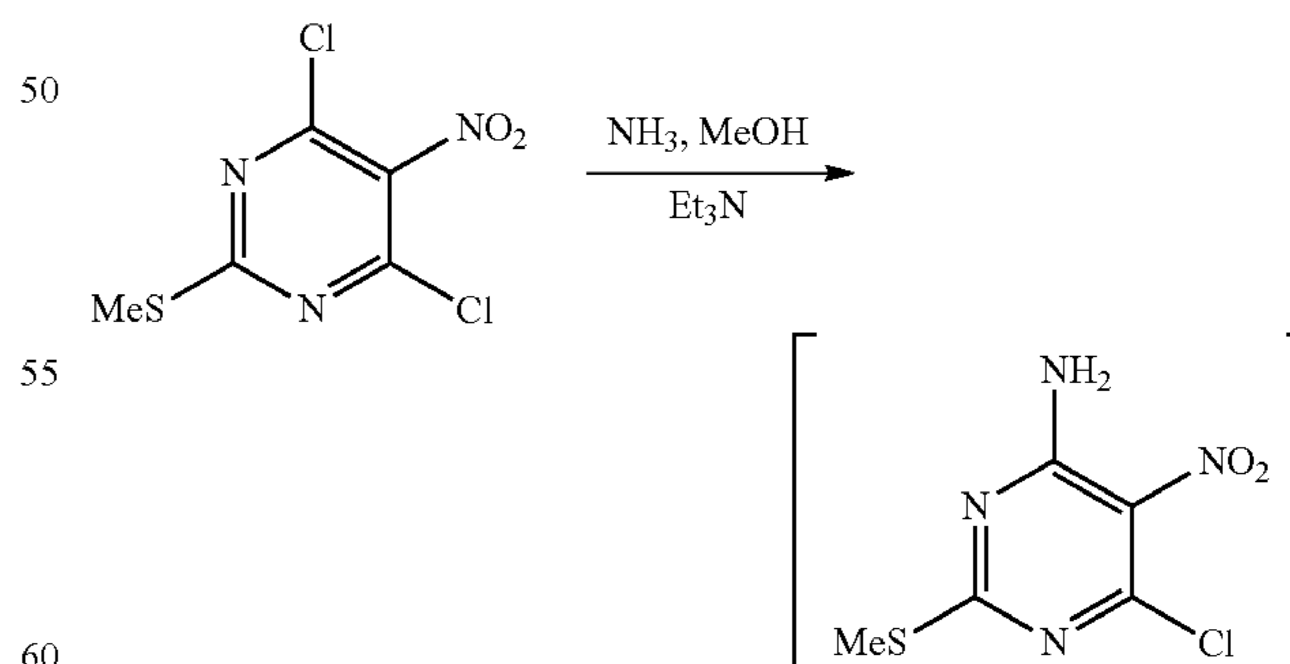
Scheme 18
