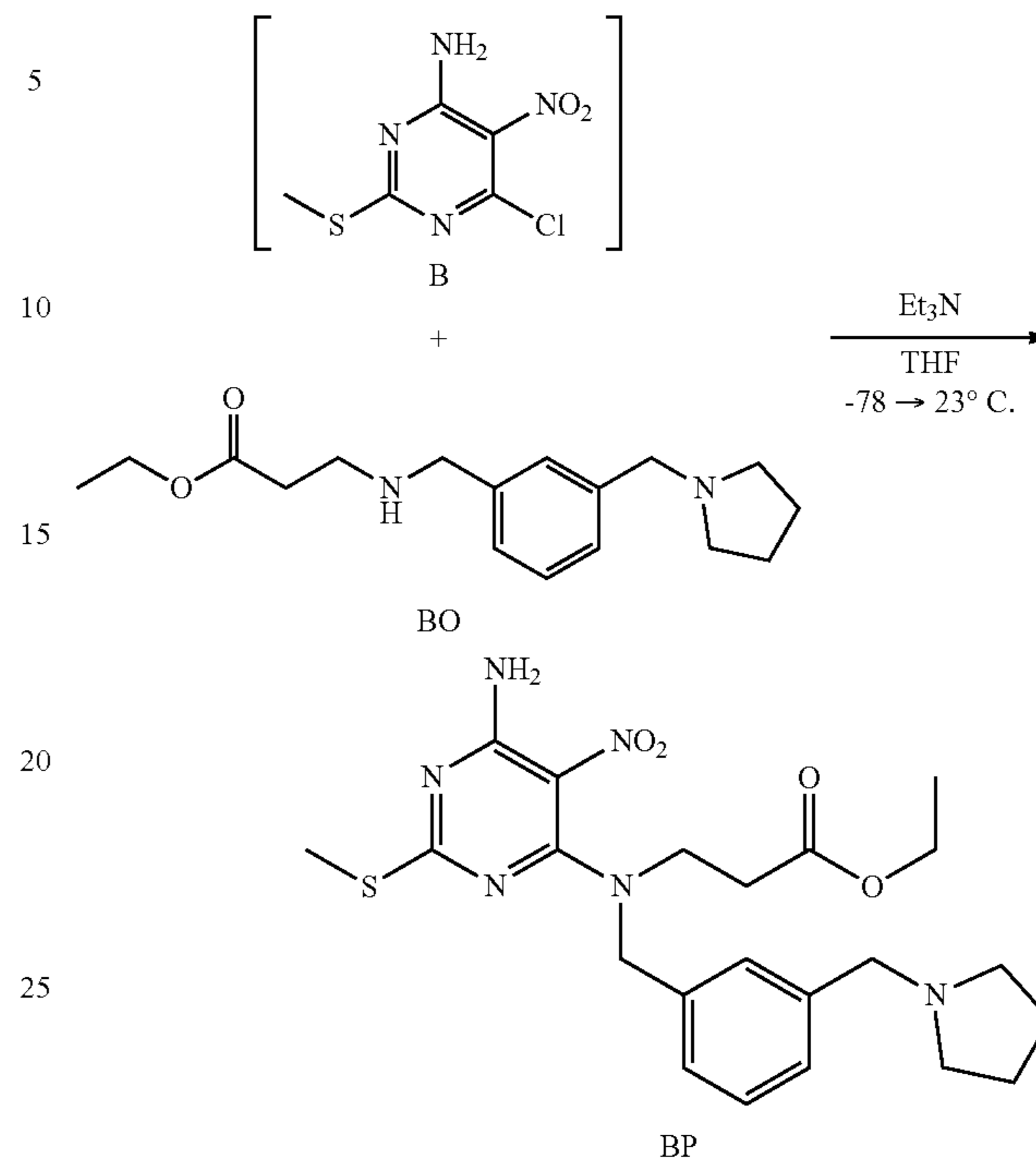
Scheme 35
