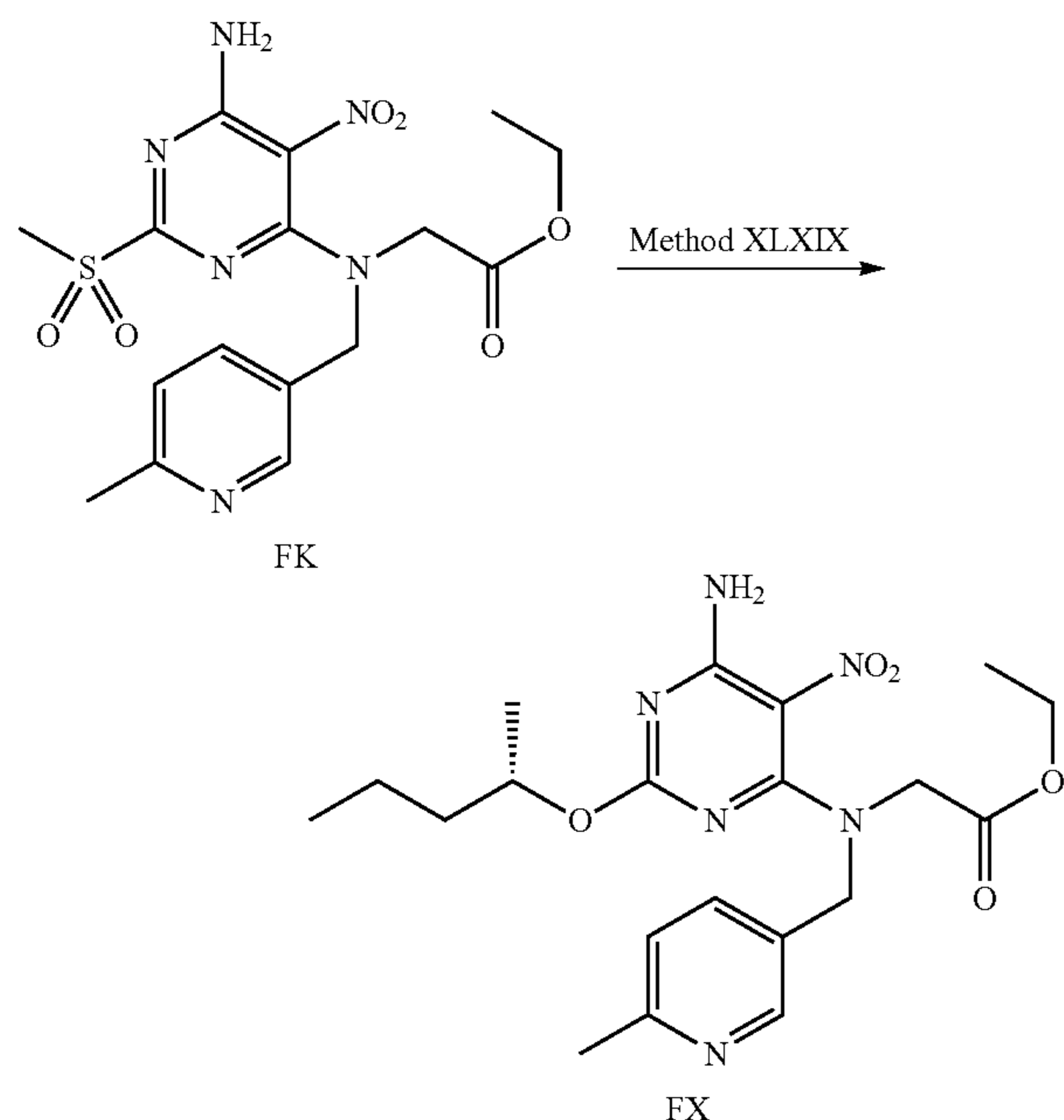
Scheme 116: Prepared Via Method XLXIX
