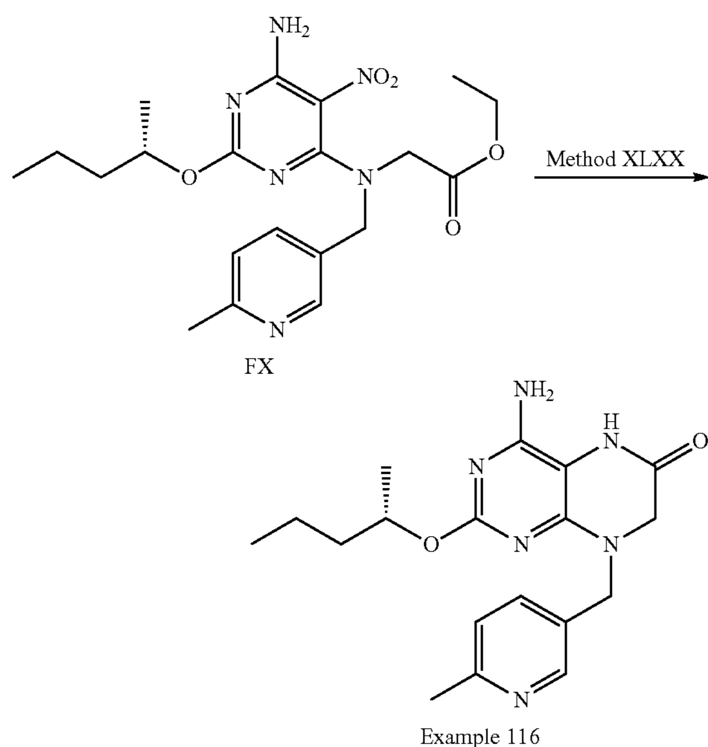
Scheme 117: Example 116, Method XLXX
