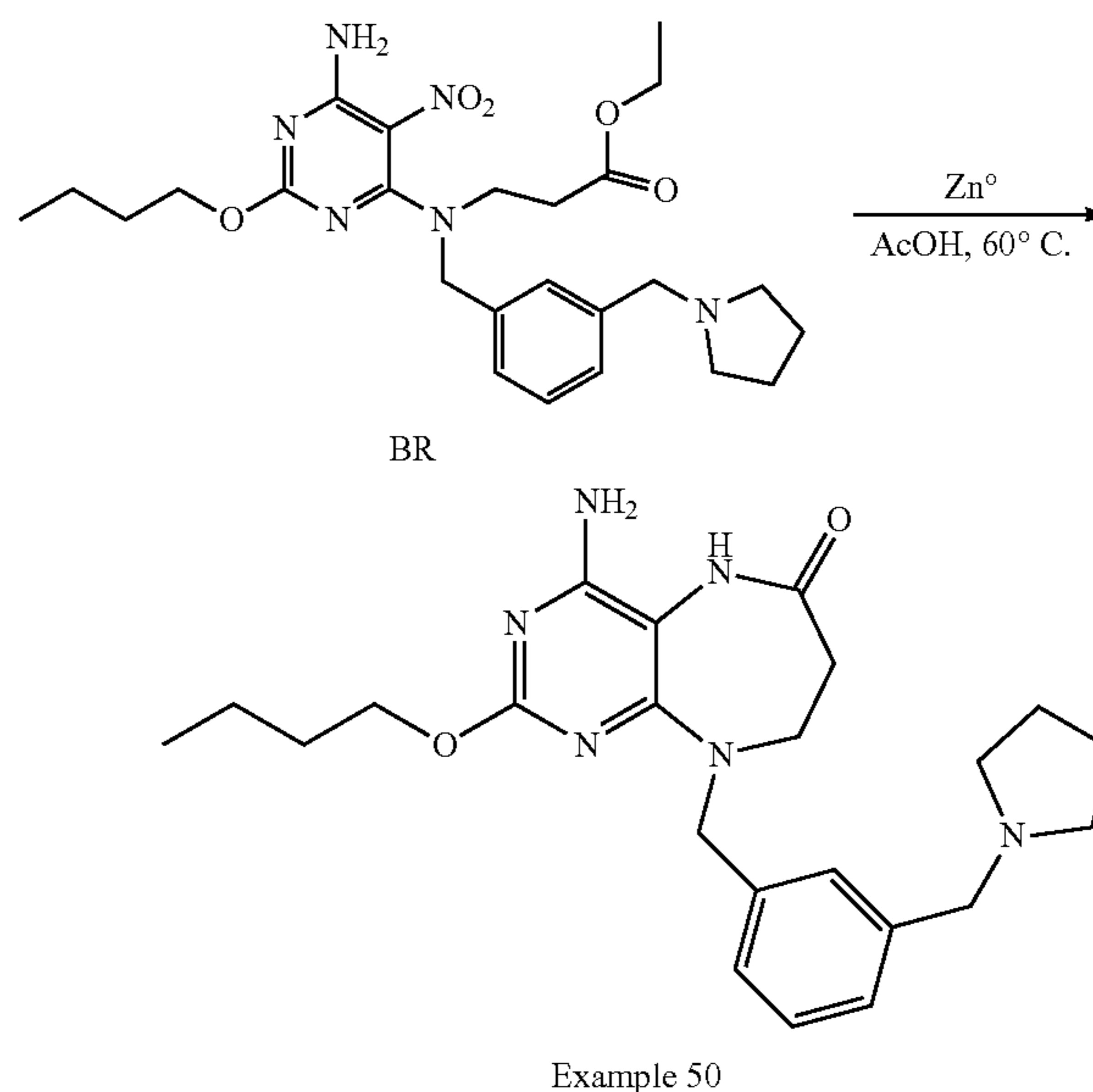
Scheme 38: Example 50
