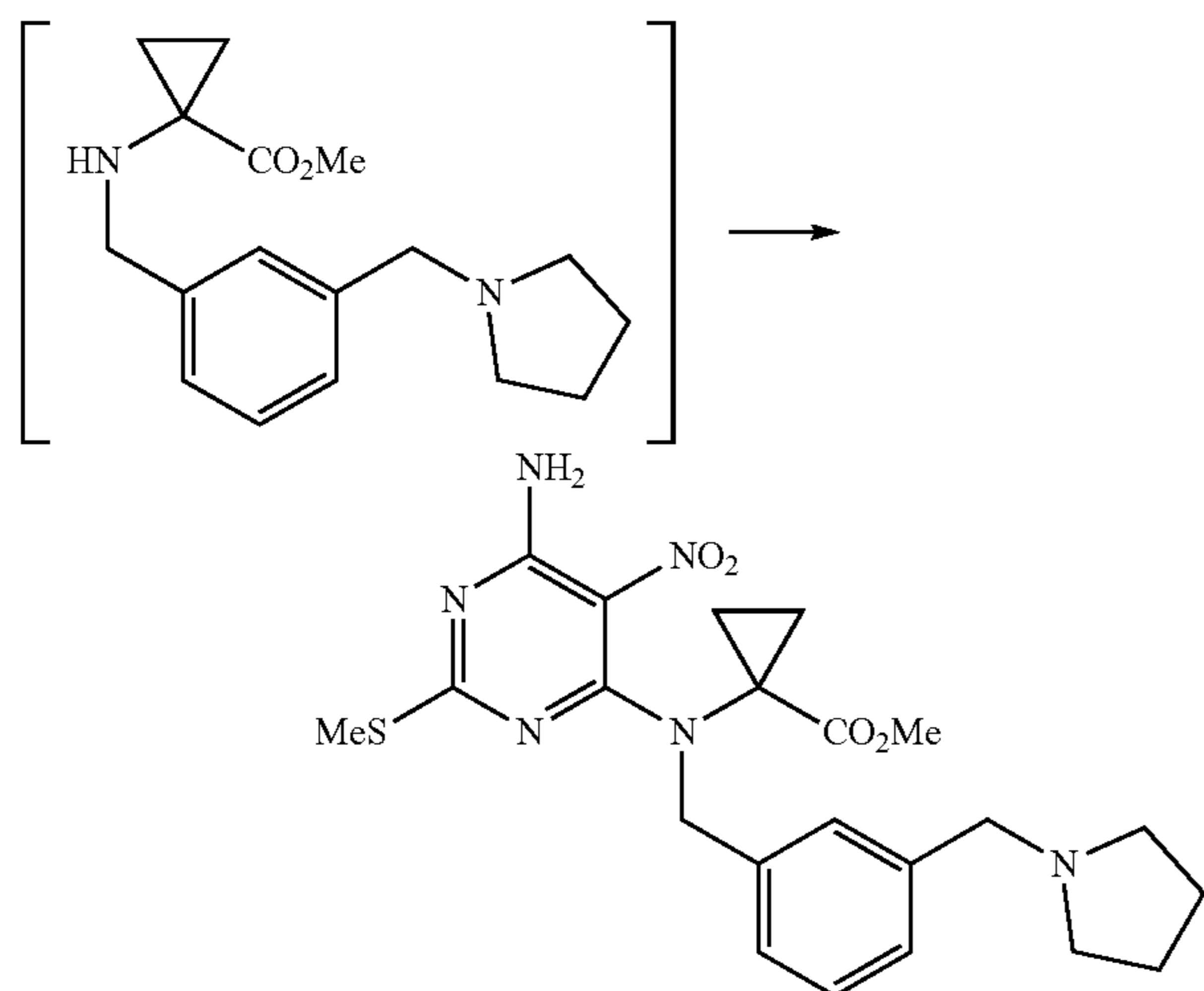
Scheme 19
