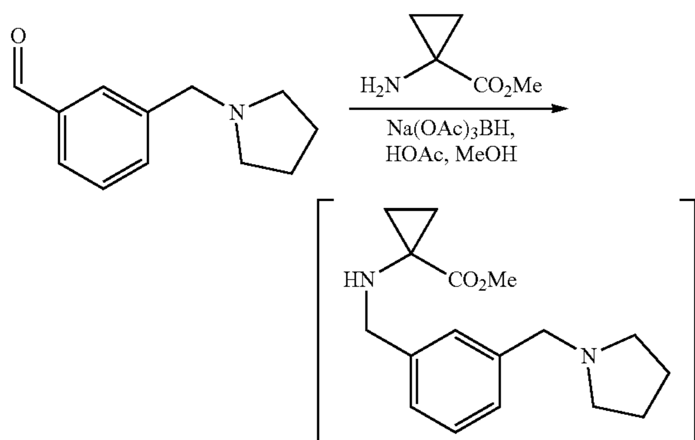
Scheme 12
