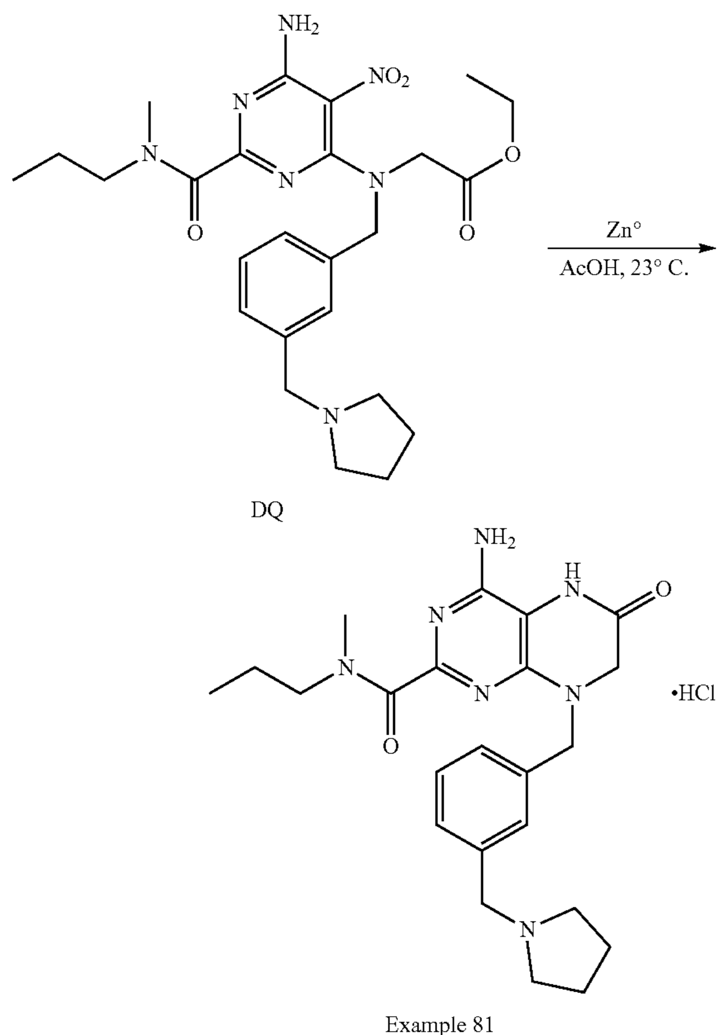
Scheme 84: Example 81
