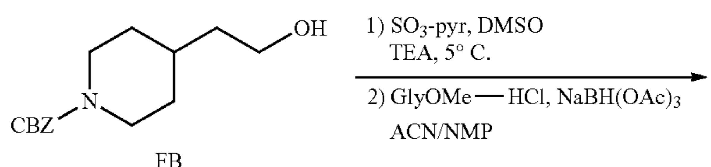
Scheme 91
