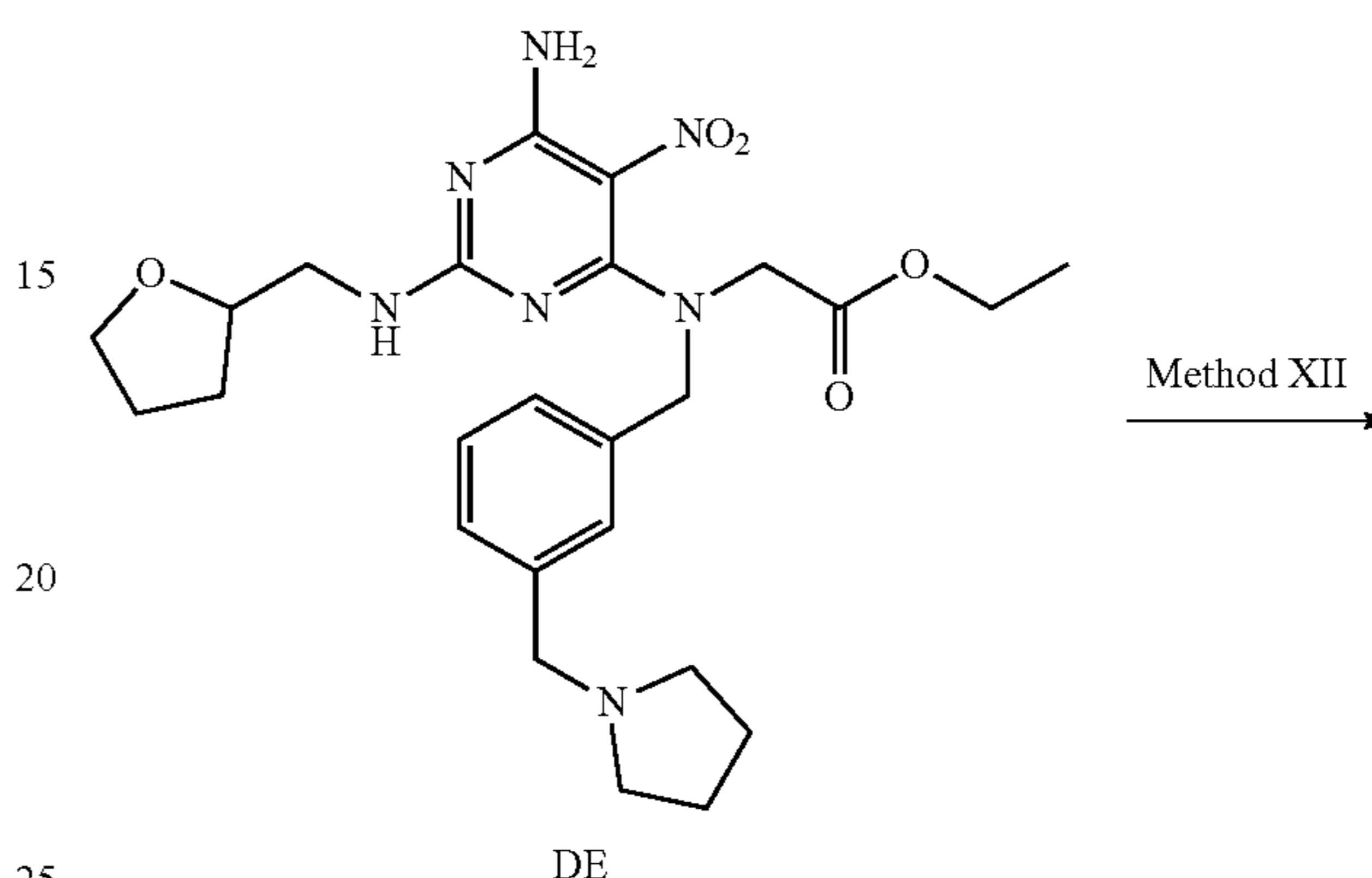
Scheme 69: Example 77, Method XII
