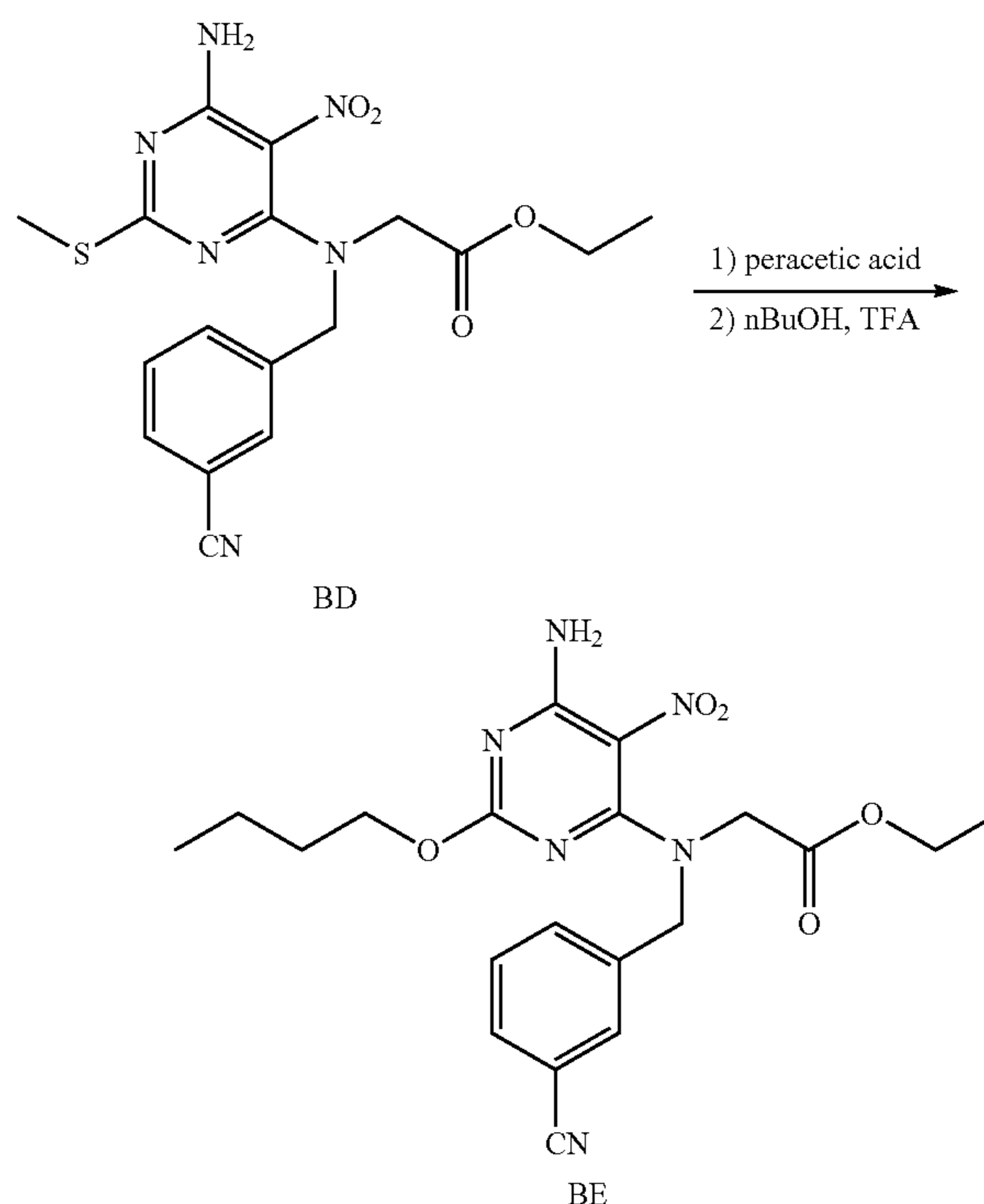
Scheme 22
