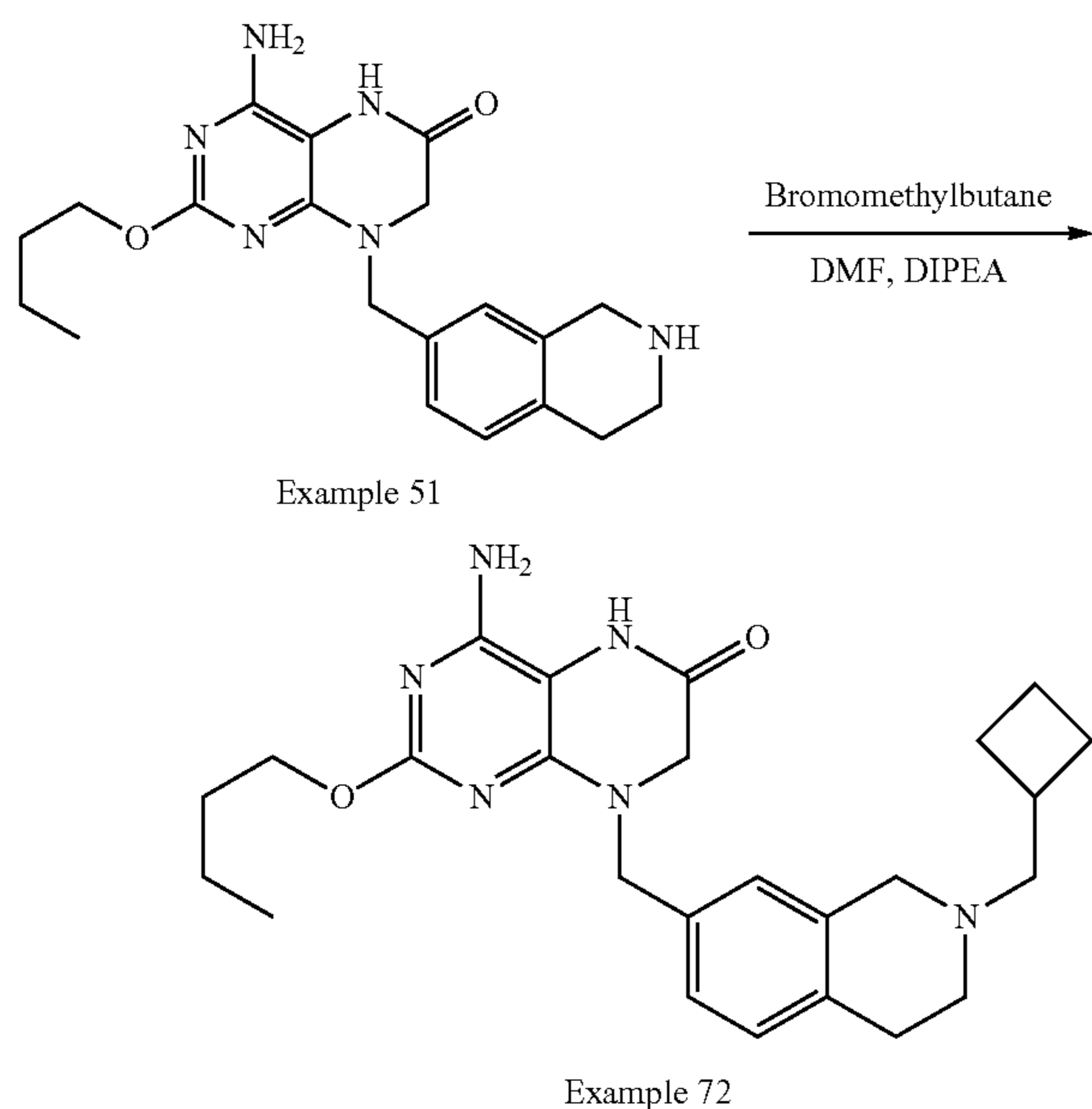
Scheme 63: Example 72, Method XLVIII:
