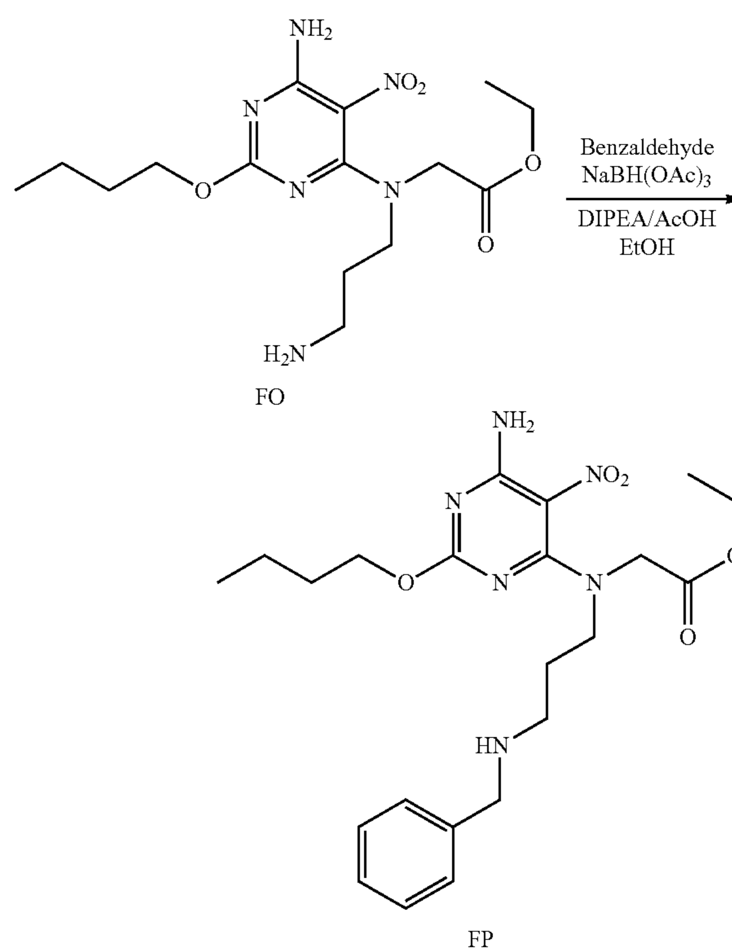
Scheme 106:
