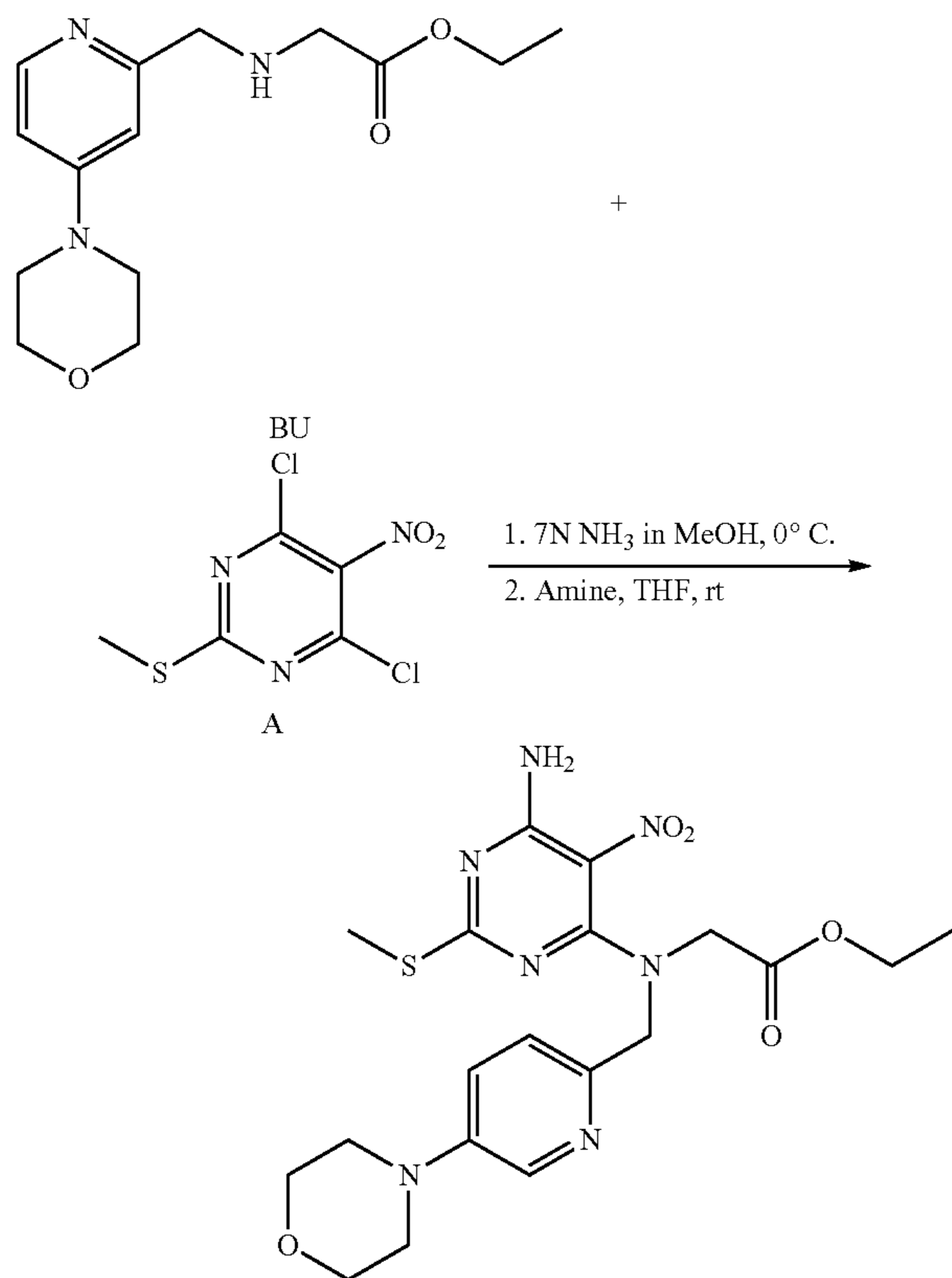
Scheme 43
