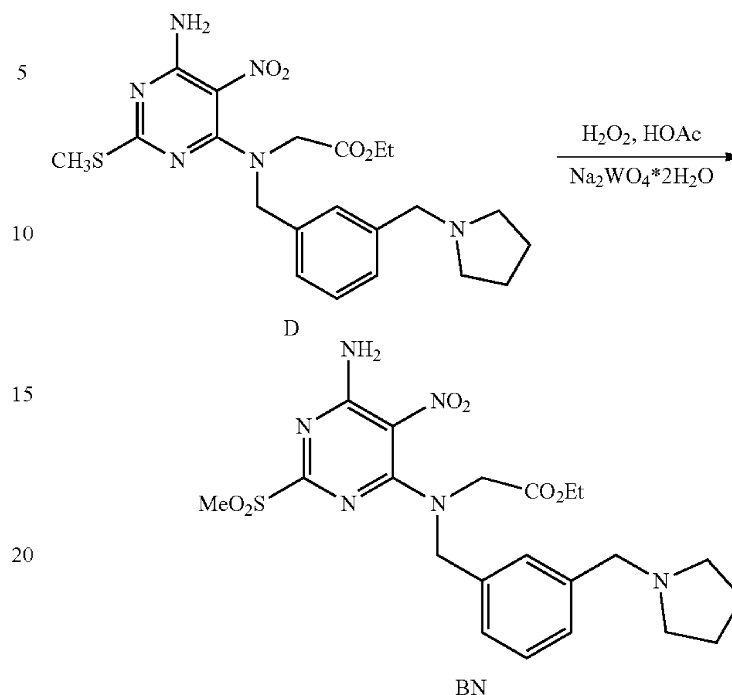
Scheme 32
