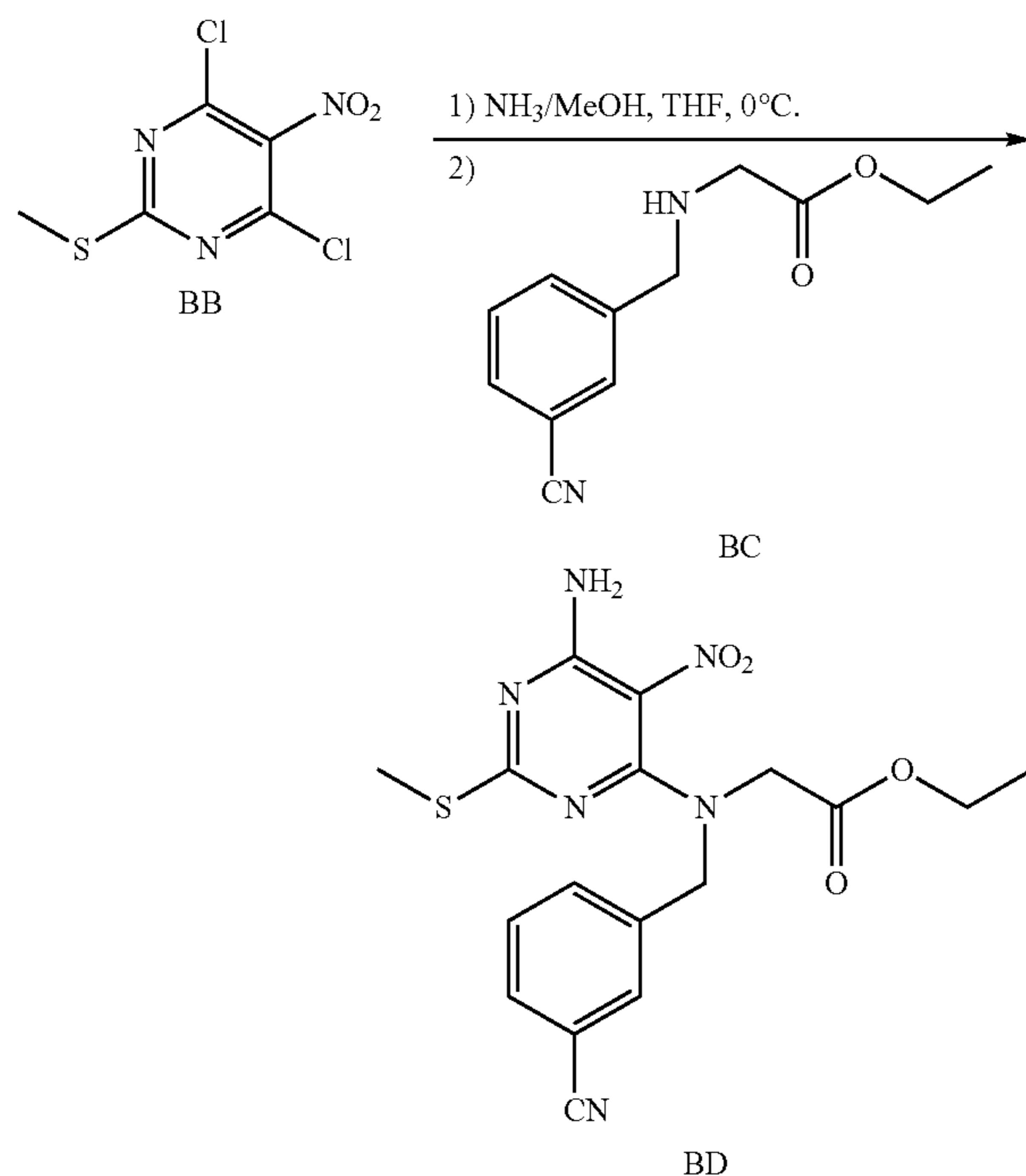
Scheme 21
