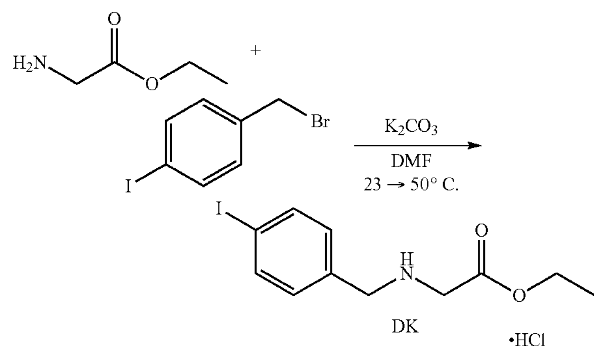
Scheme 77
