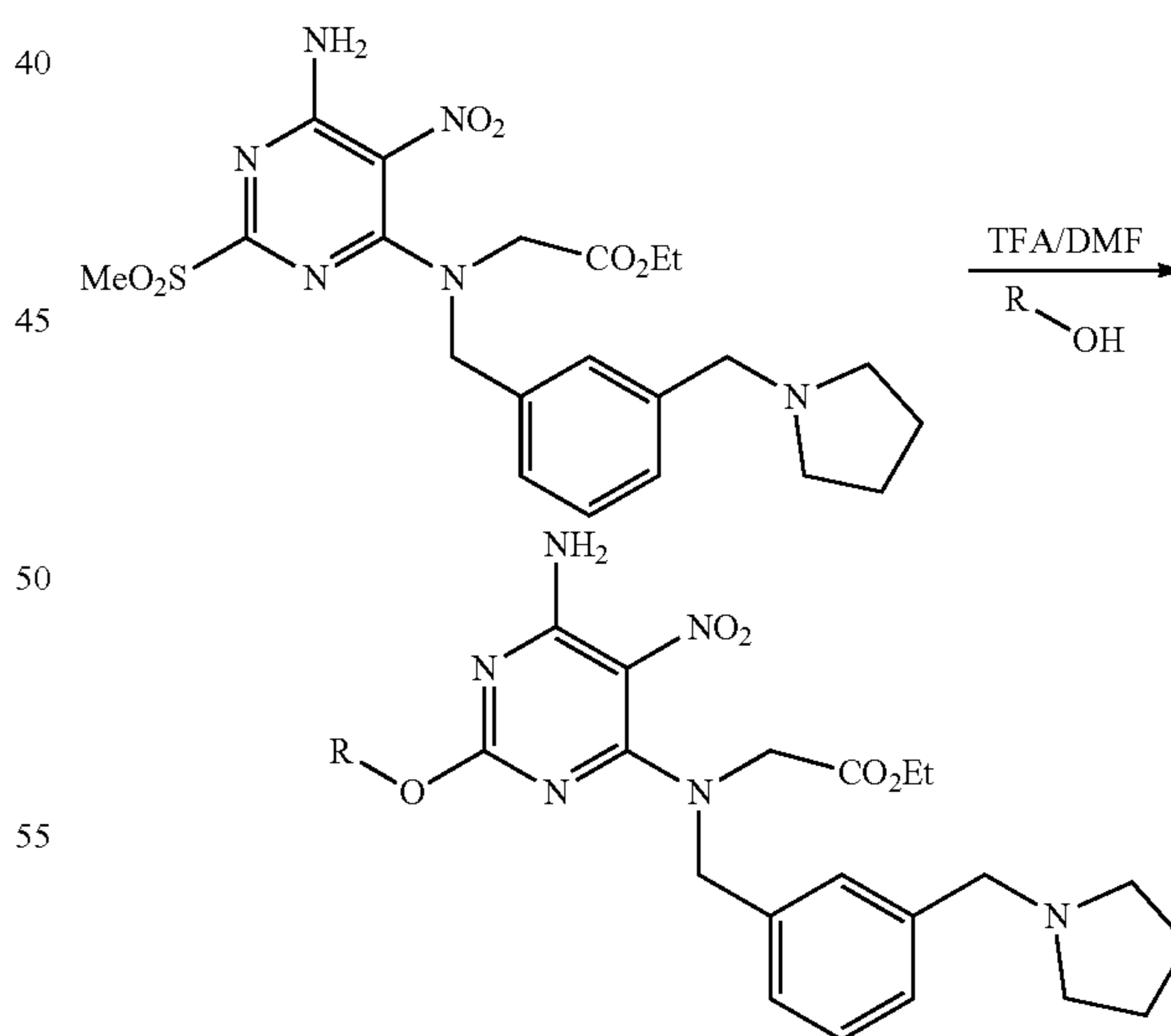
Scheme 14
