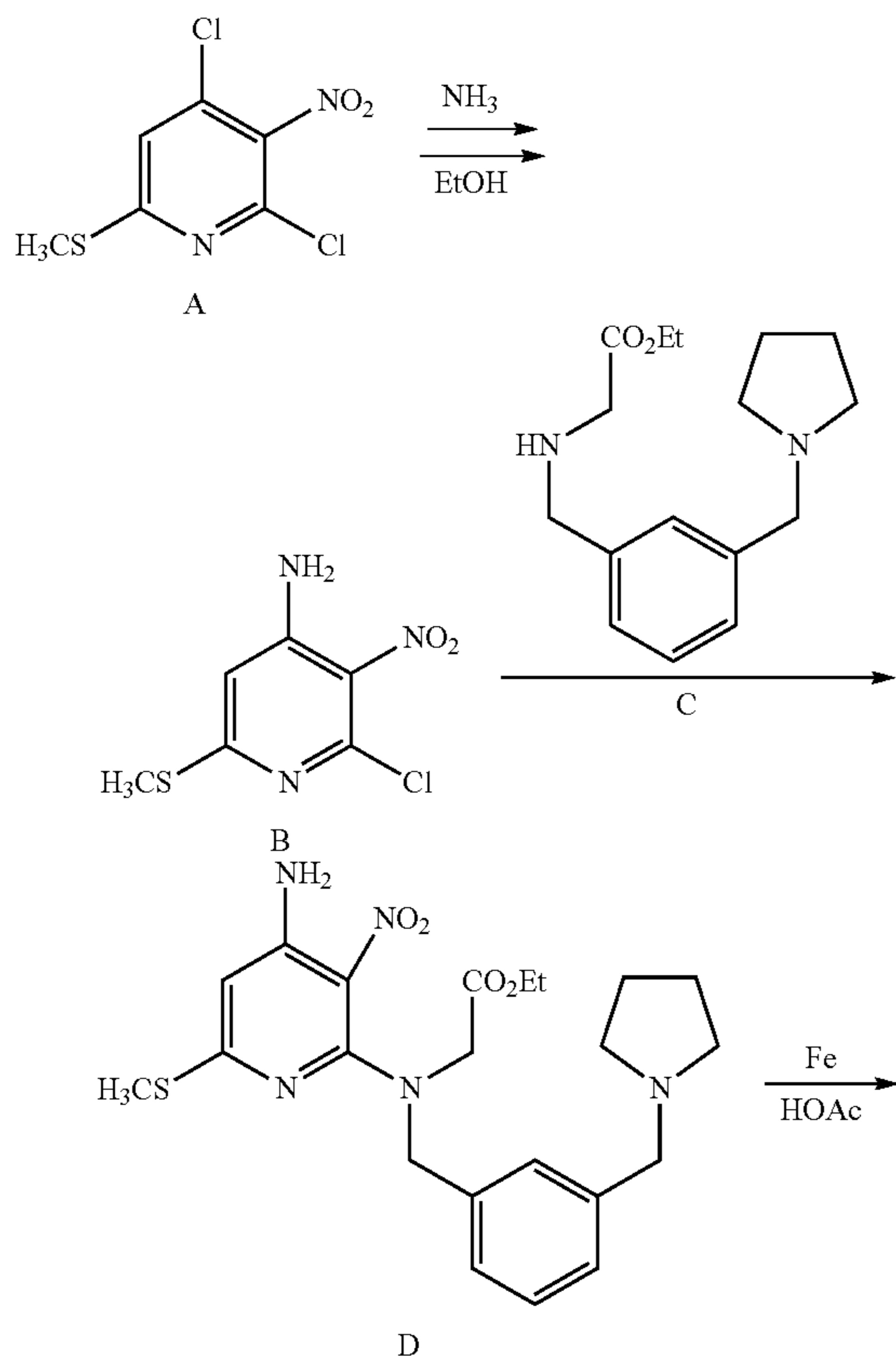
Scheme 1
