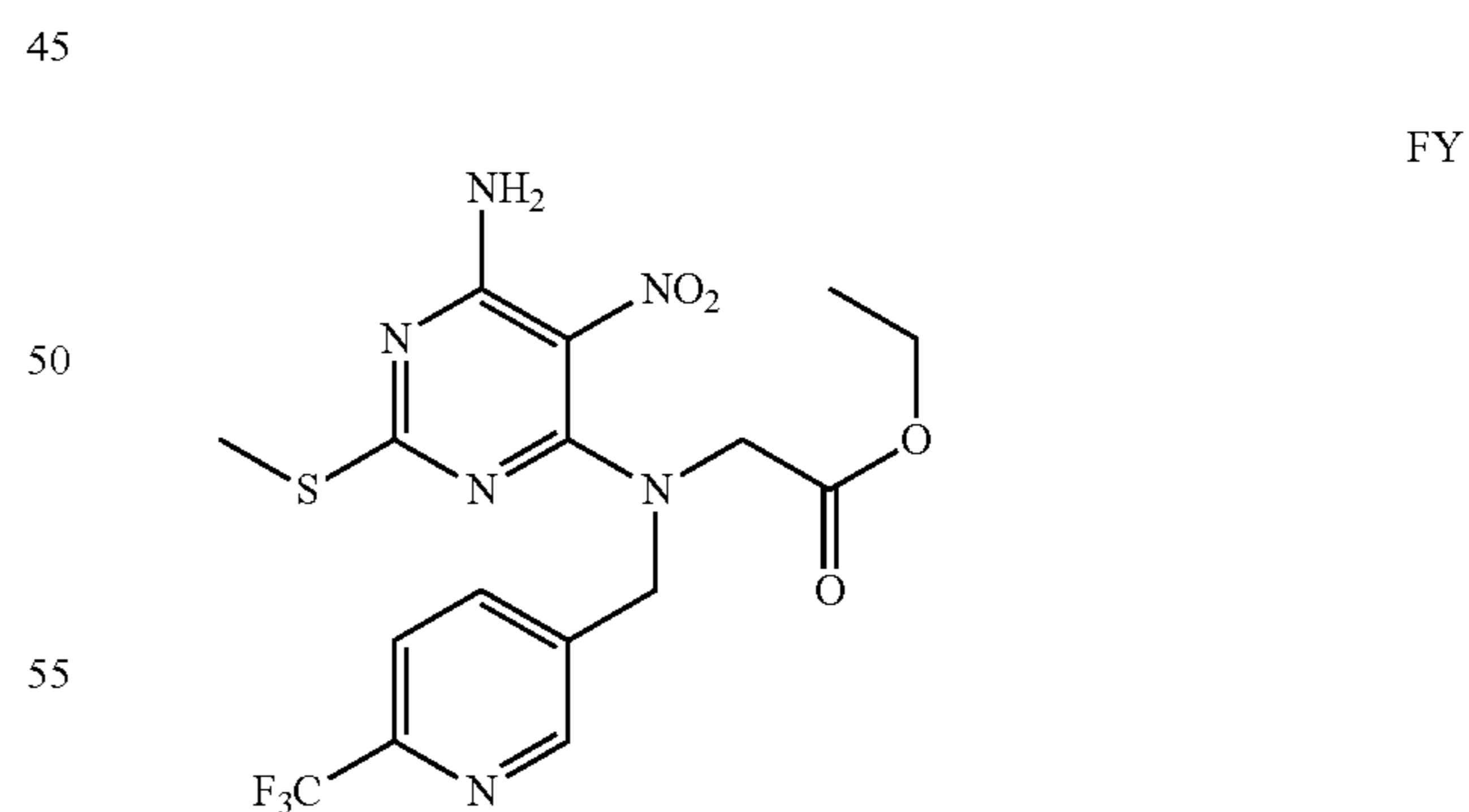
Compound FY: Prepared by Method XLXVII
