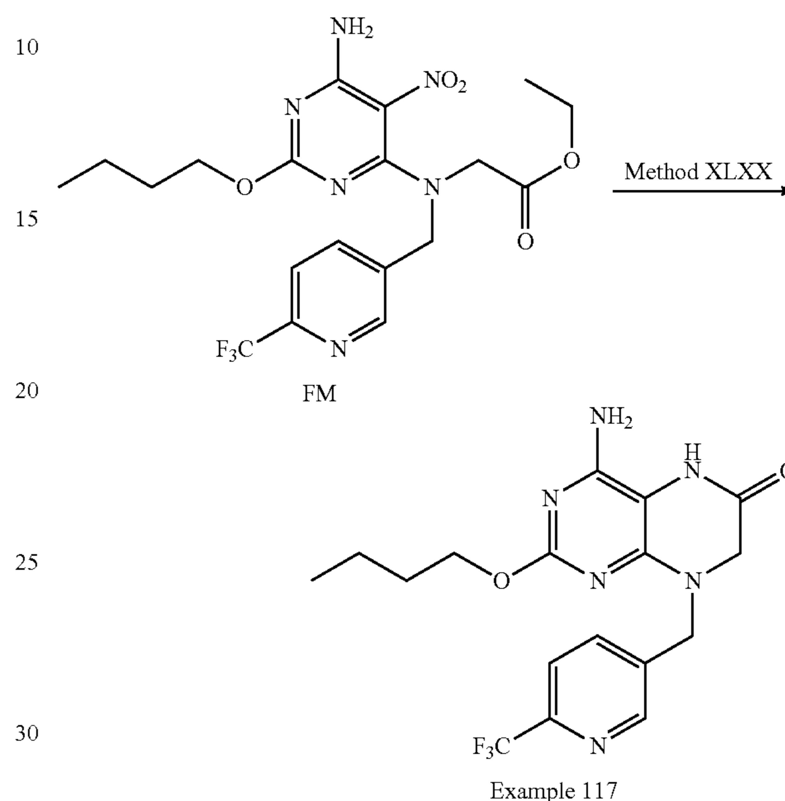
Scheme 118: Example 117, Method XLXX
