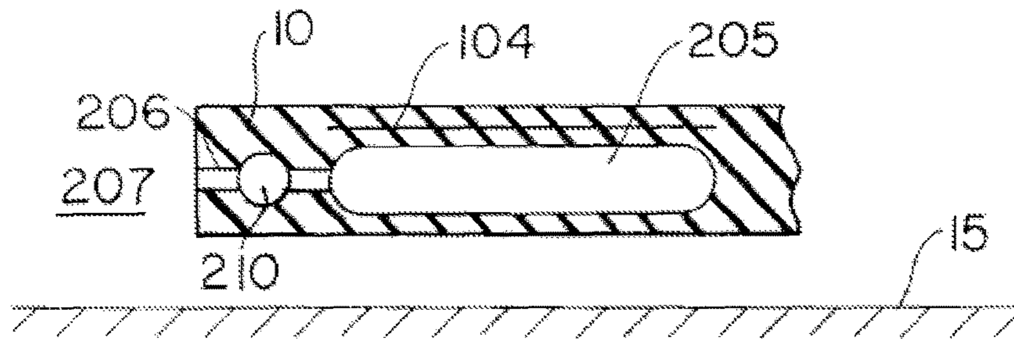
FIG. 10G PRIOR ART
