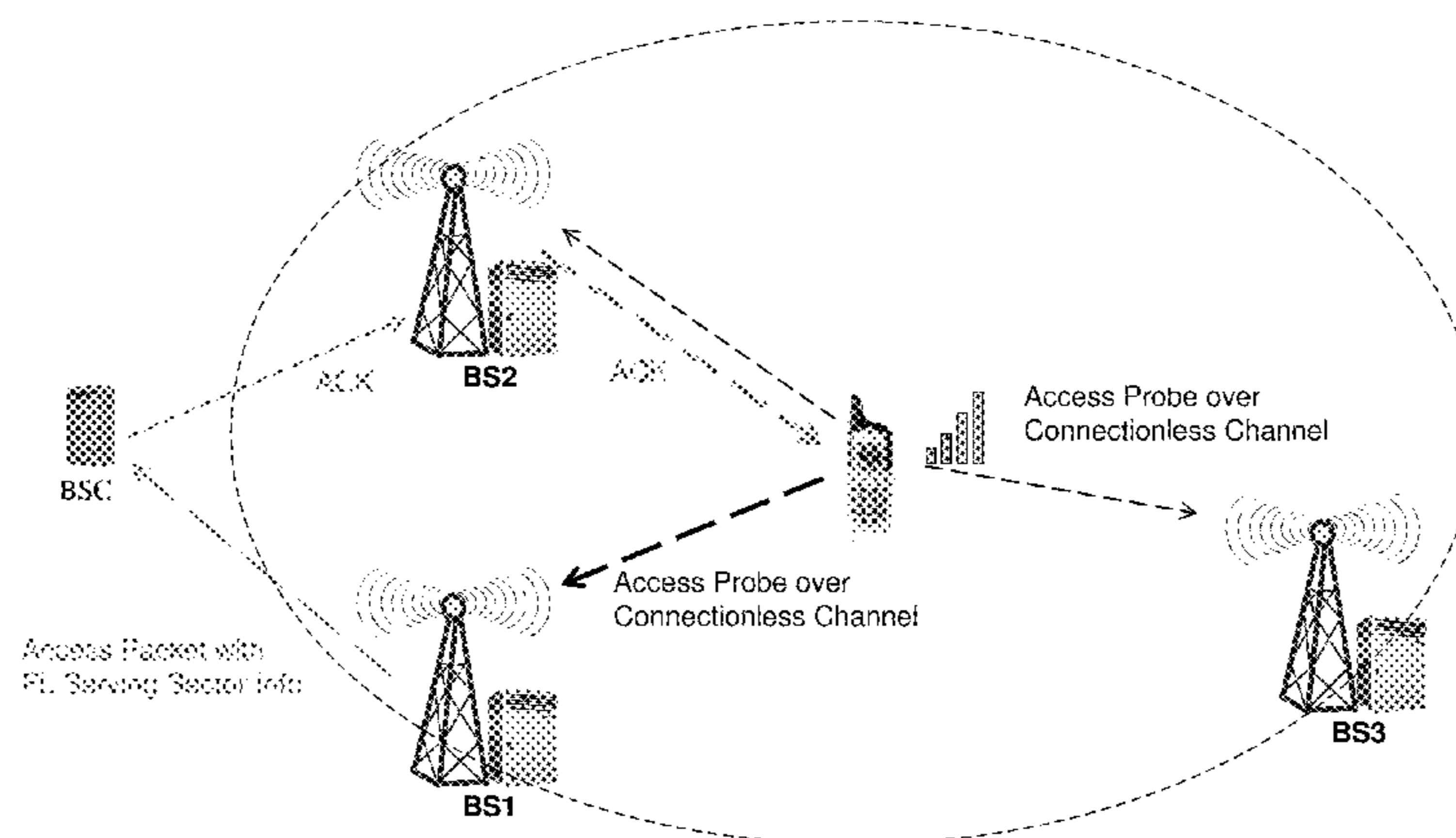
Connectionless Soft/Softer Handoff in RL Cellless Configuration
