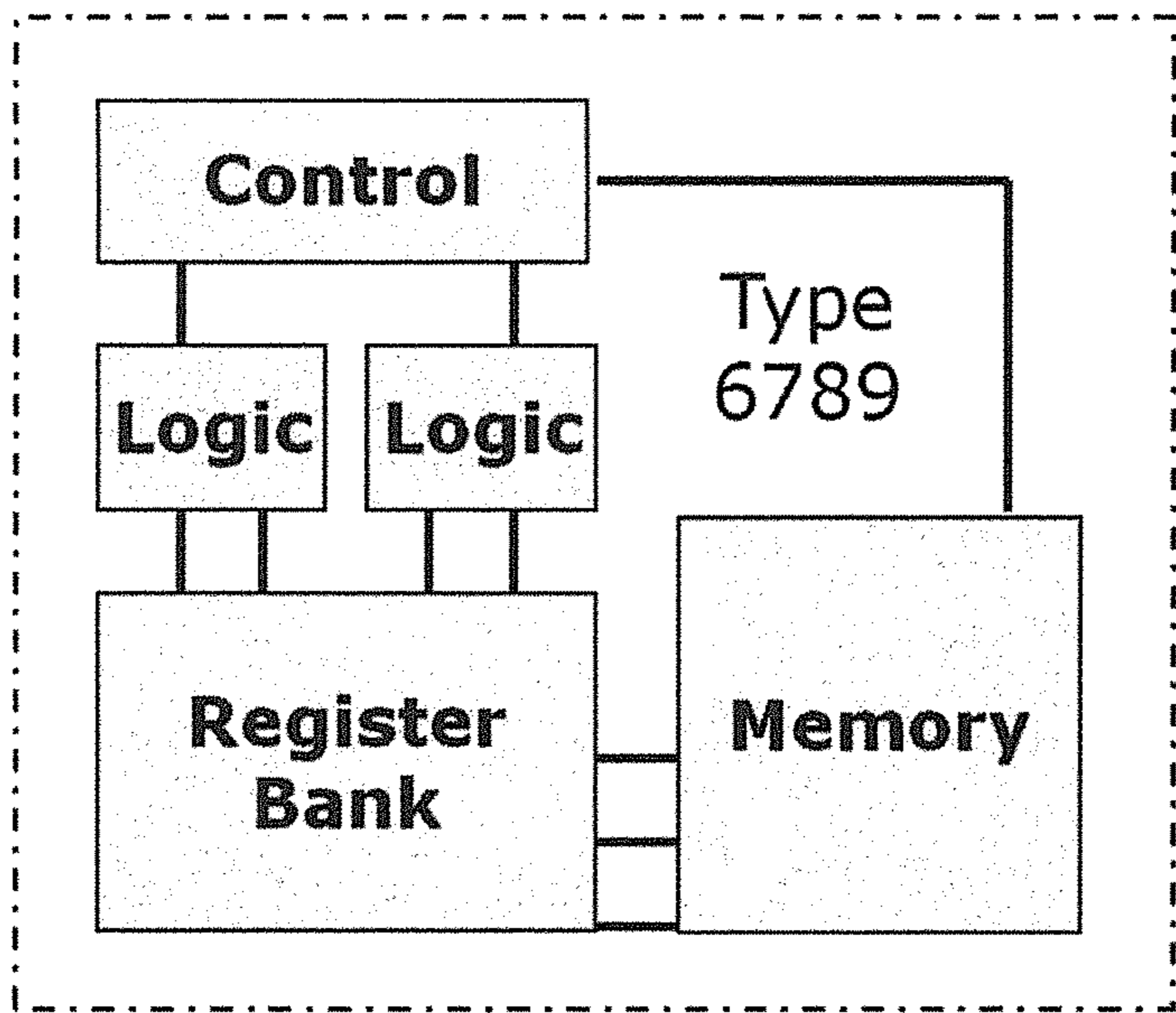
Figure 9: A single Processing Element (PE).
