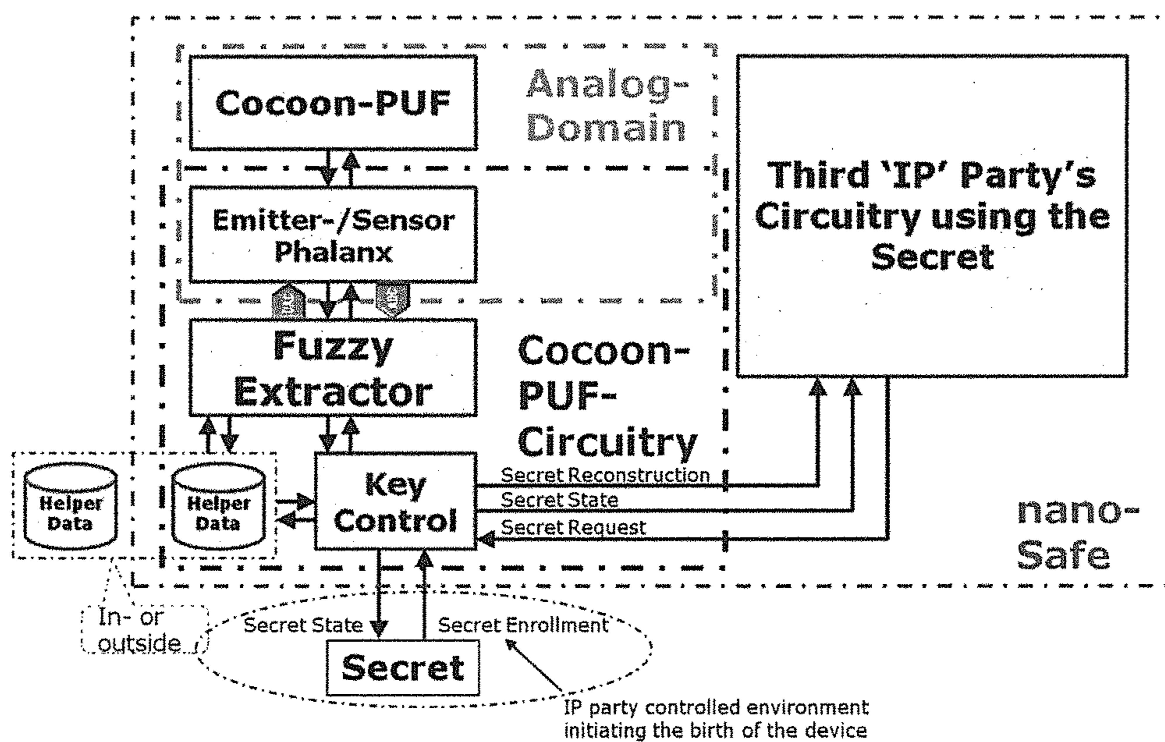
Figure 21: Block Diagram of a CASTOR.
