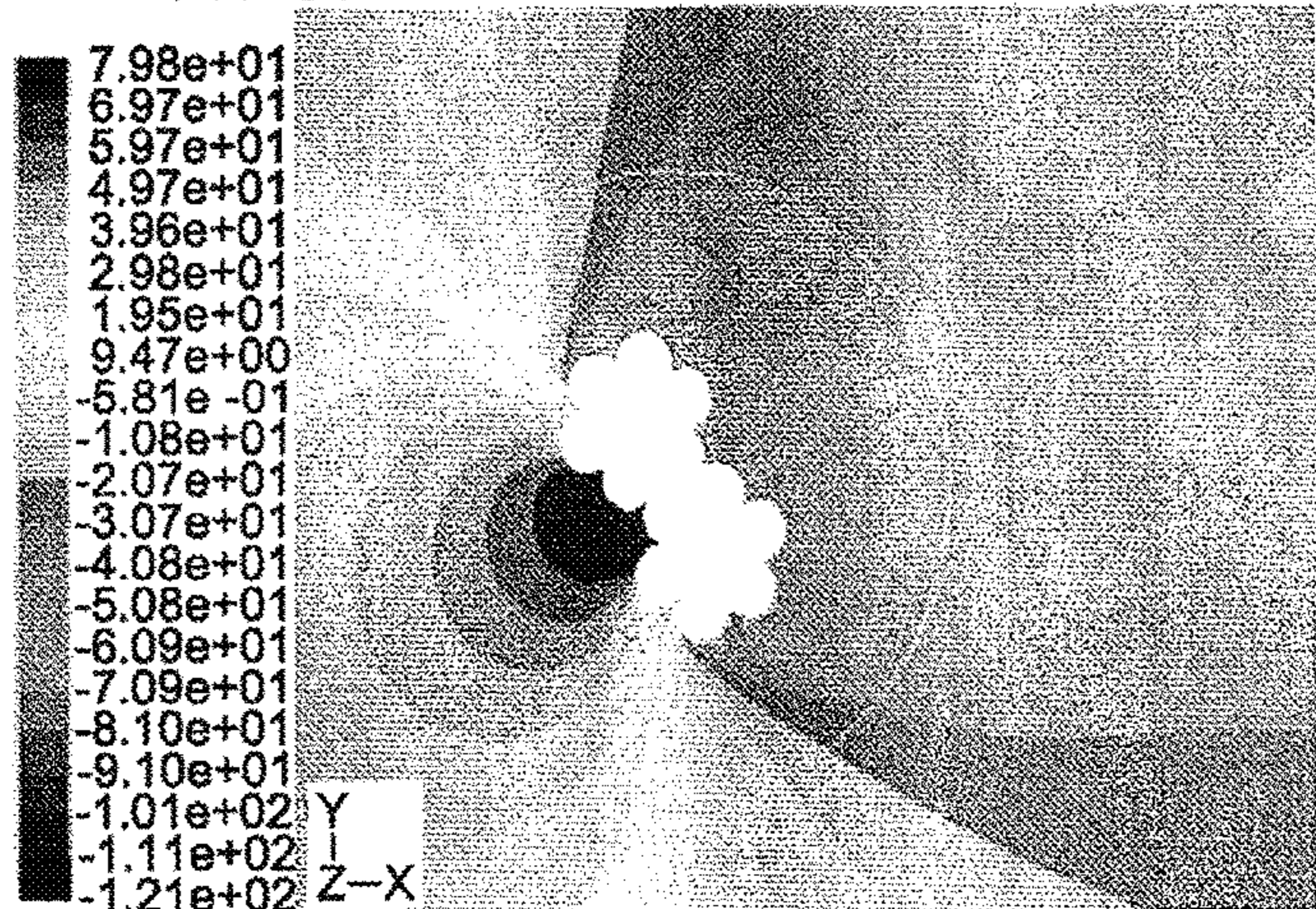
PRESSURE AT VARIOUS TIMES: 9FT LAY CABLE
