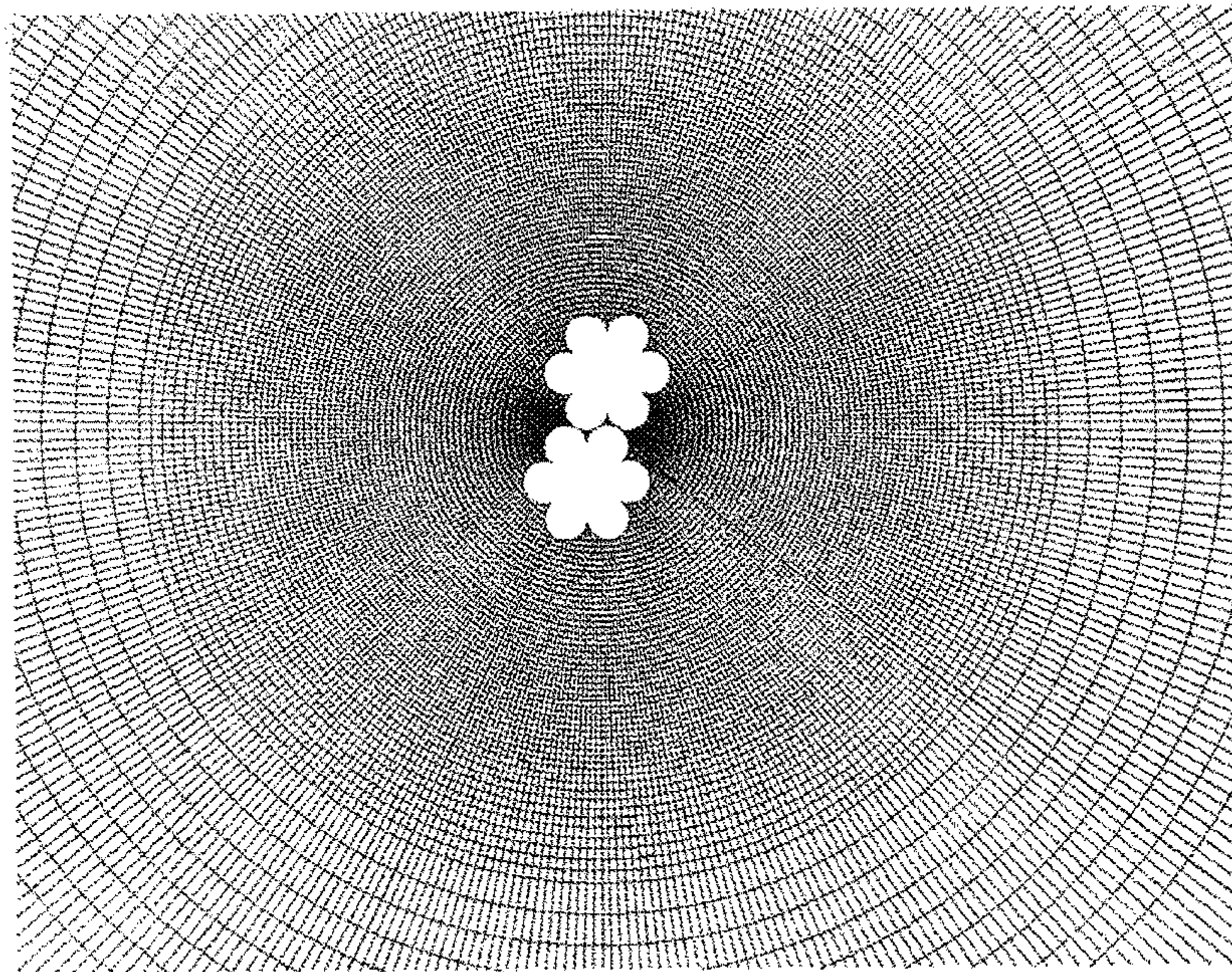
CLOSE-UP OF CABLE AND MESH
