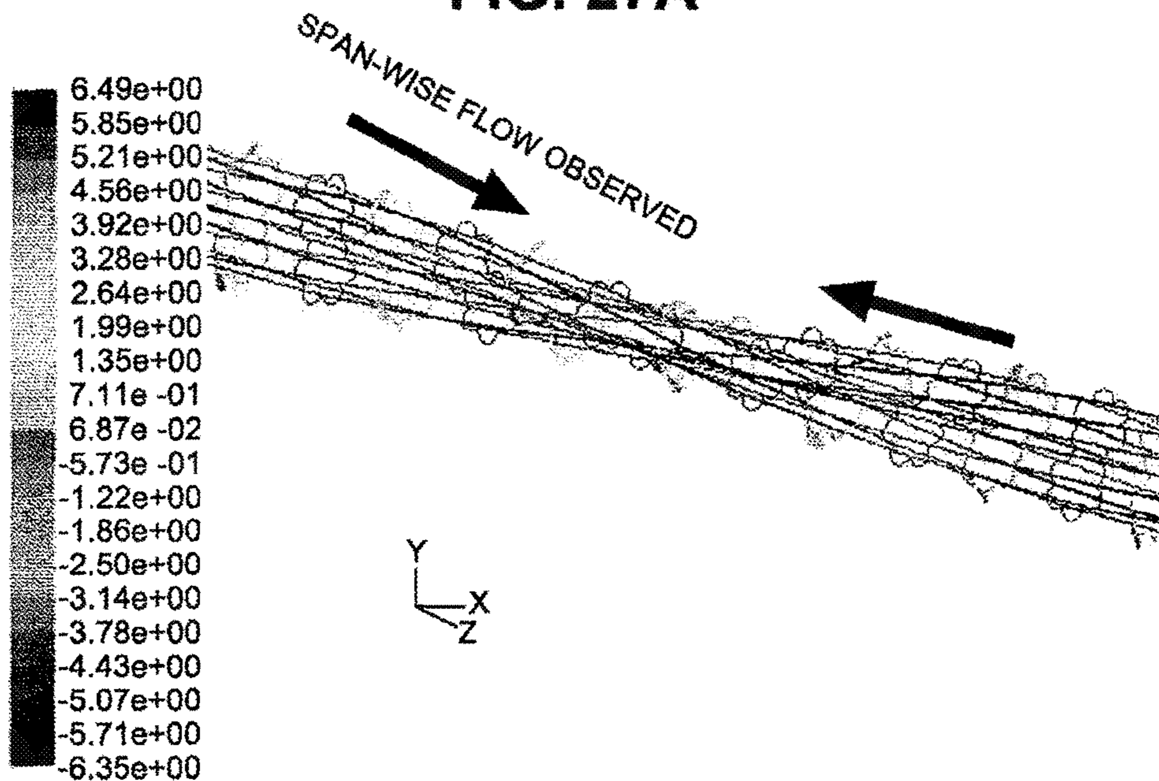
VELOCITY VECTORS COLORED WITH SPAN-WISE SPEED (m/s)
