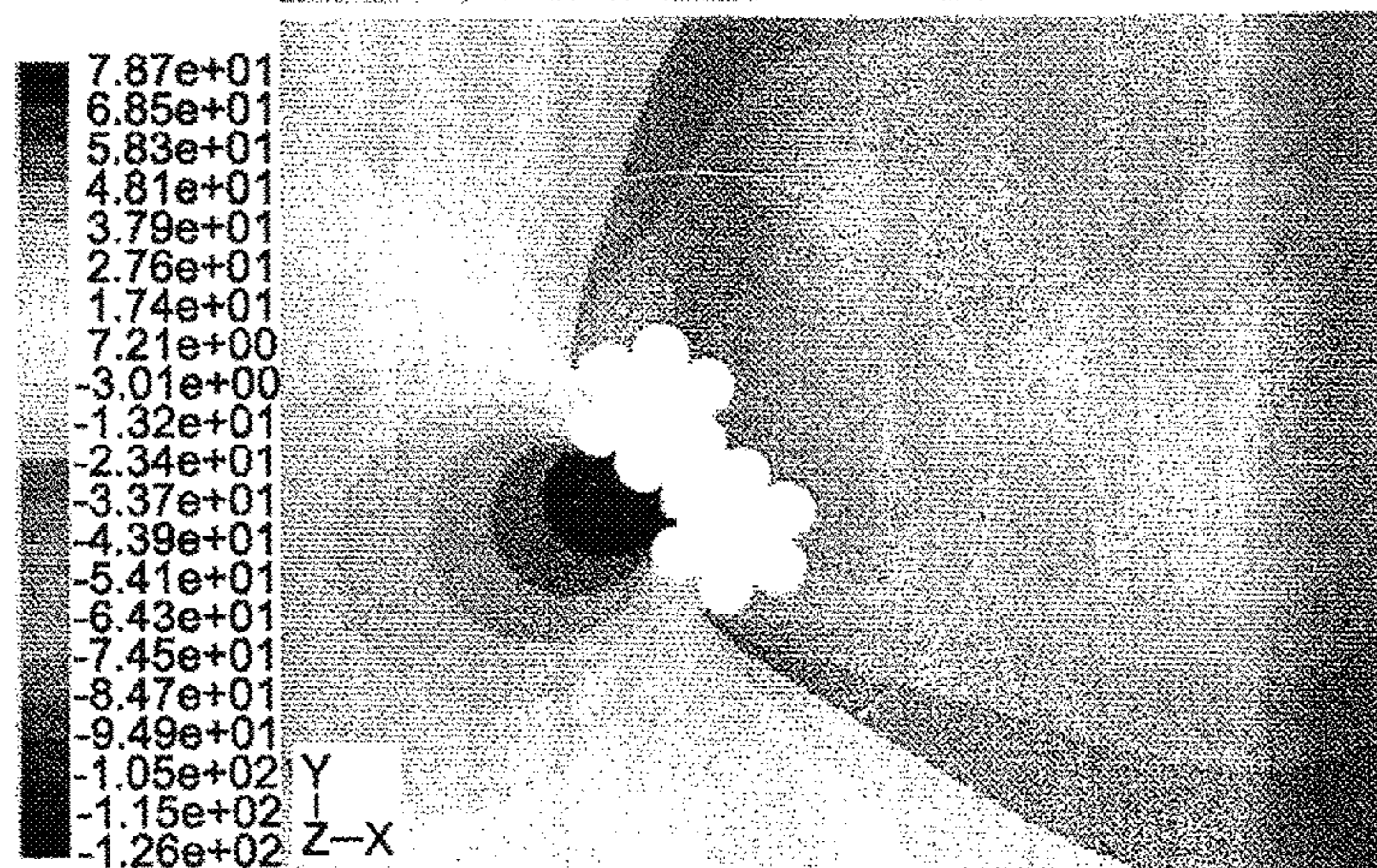
PRESSURE (Pa) ON PLANE 2 AT VARIOUS TIME-INSTANTS INDICATING THE CHAOTIC AND TIME-DEPENDANT NATURE OF THE FLOW BEHAVIOR
