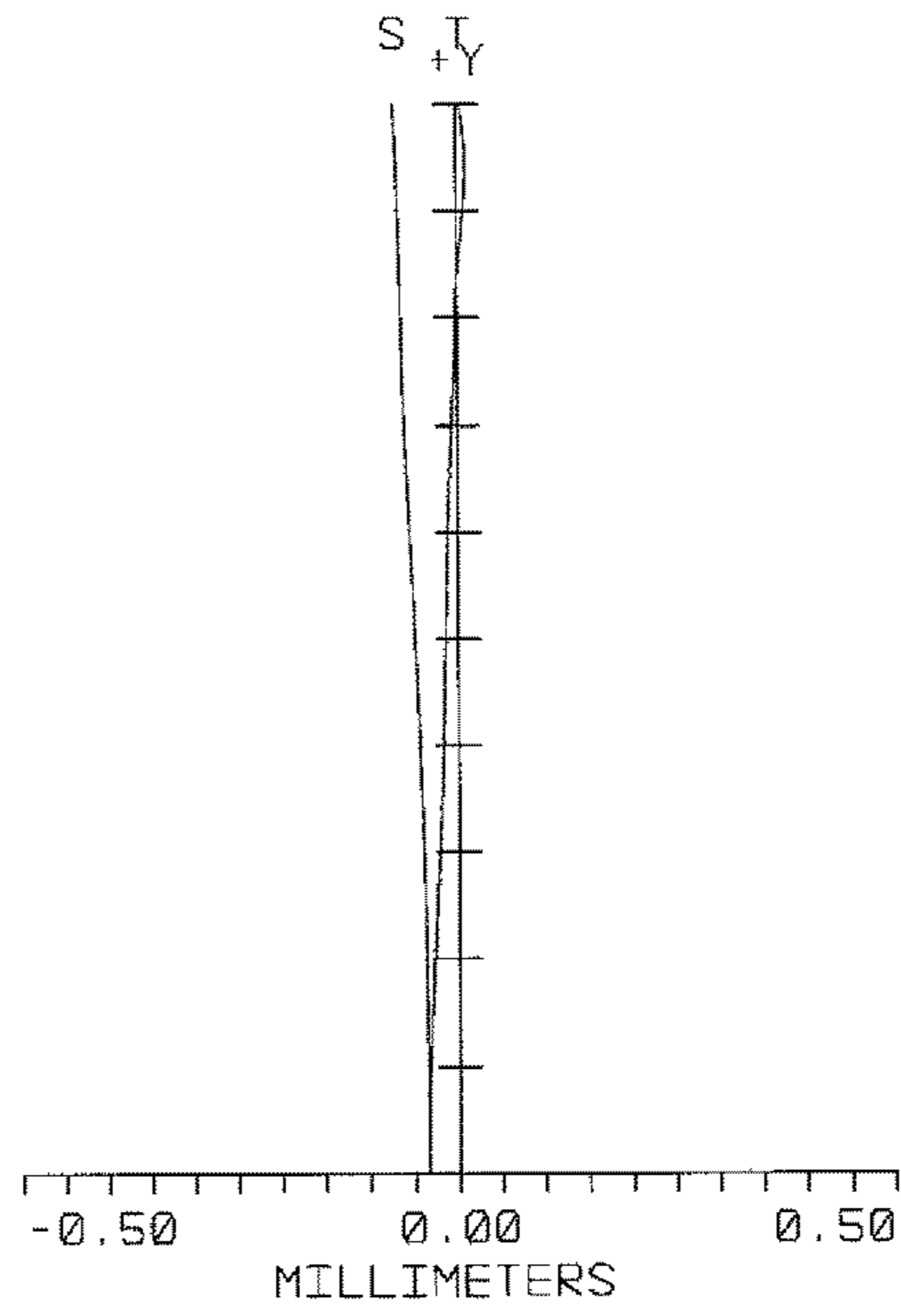
FIG. 6C FIELD CURVATURE
