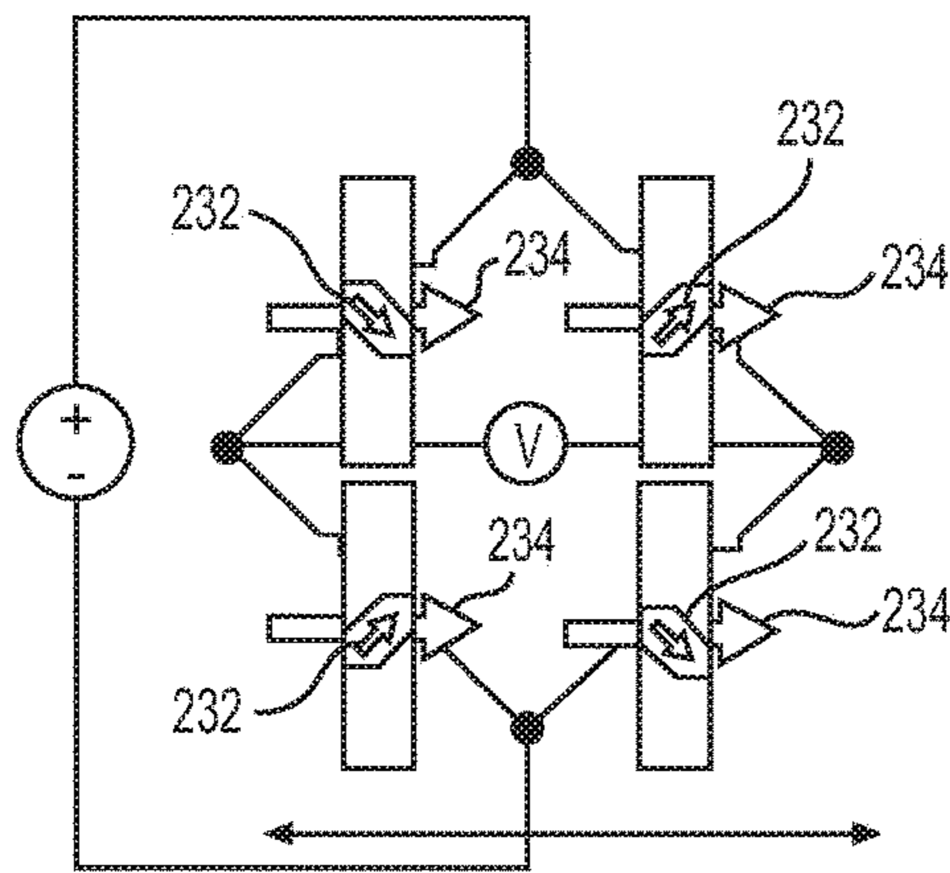
XY AXIS CONFIGURATION
