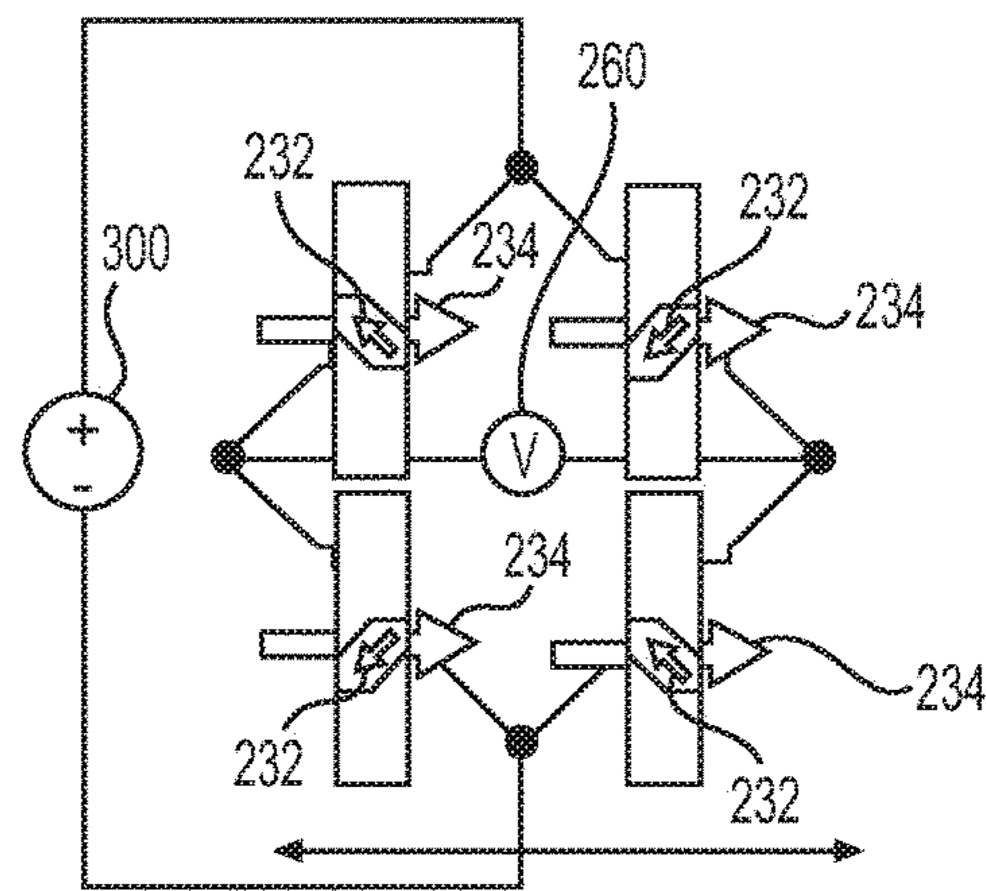
XY AXIS CONFIGURATION
