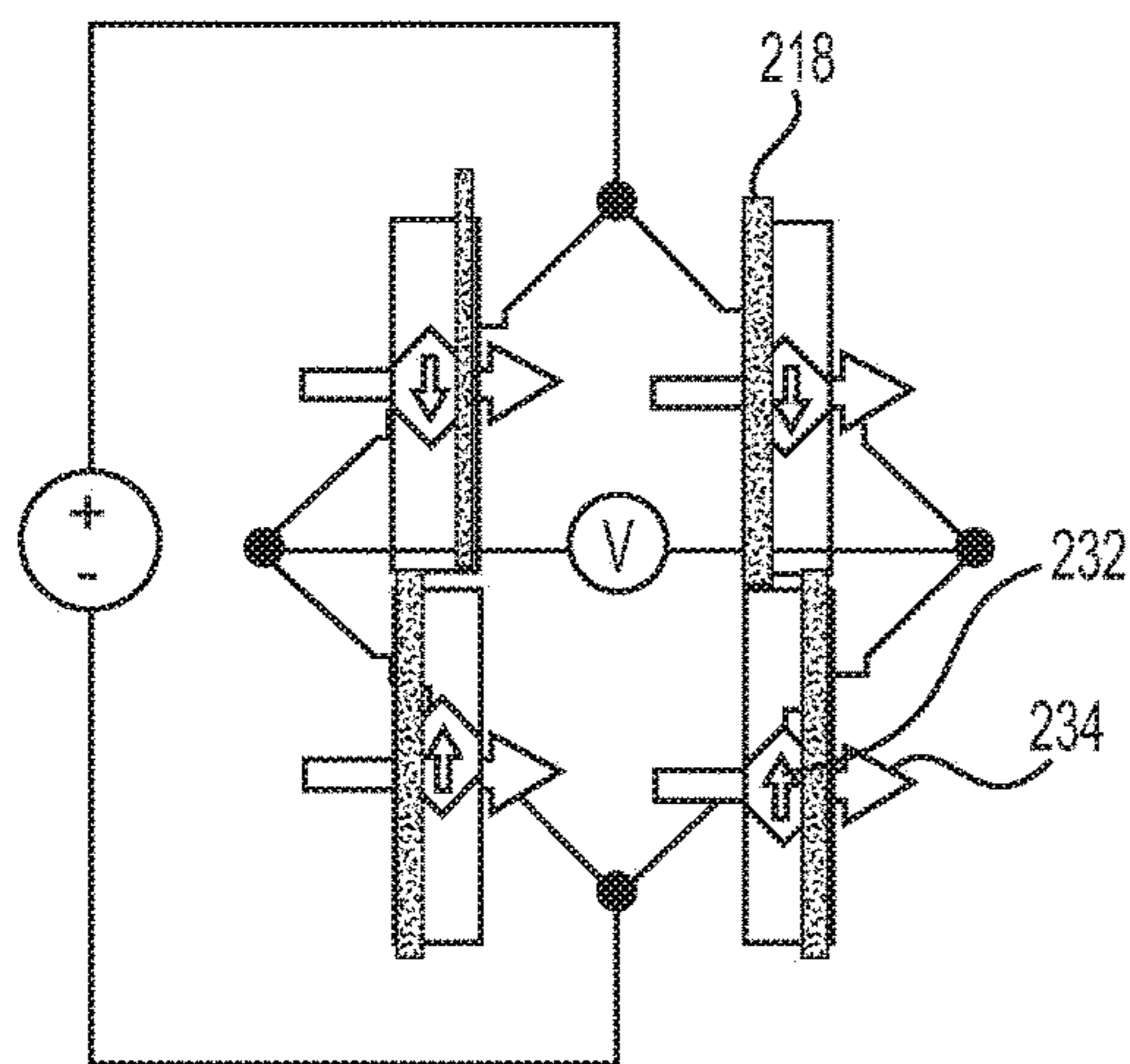
Z AXIS CONFIGURATION
