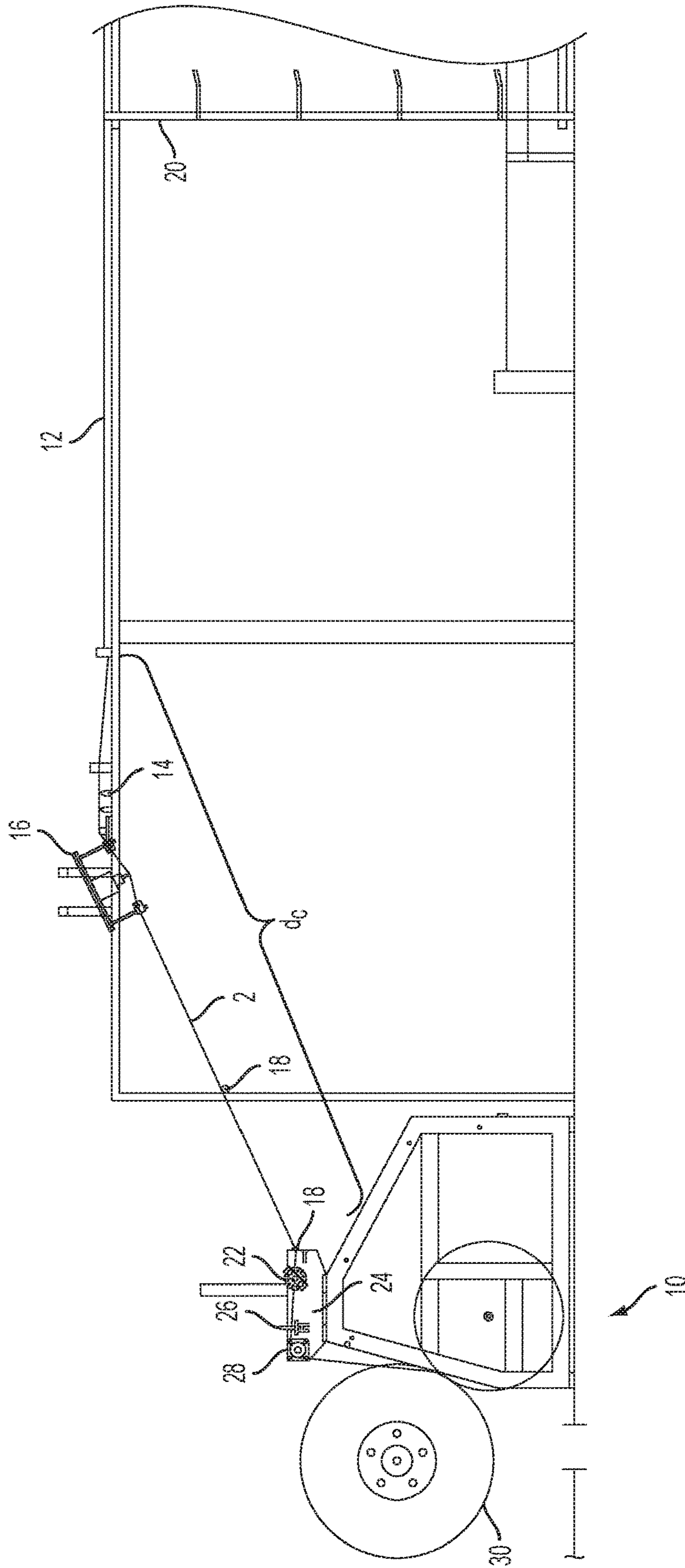
FIG. 1 PRIOR ART
