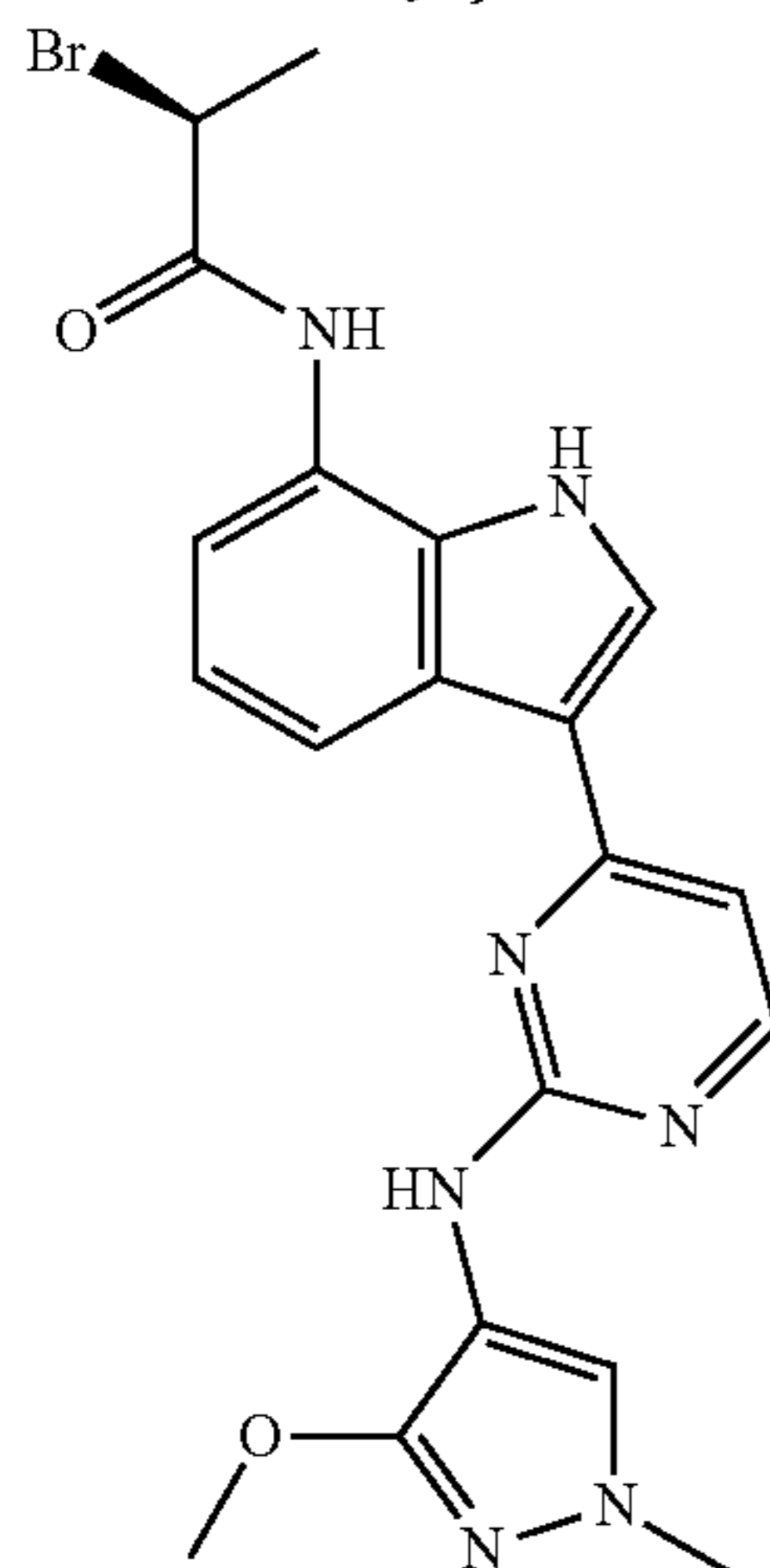
Intermediate 32: (2S)-2-Bromo-N-(3-{2-[(3-methoxy-1-methyl-1H-pyrazol-4-yl)amino]pyrimidin-4-yl}-1H-indol-7-yl)propanamide
