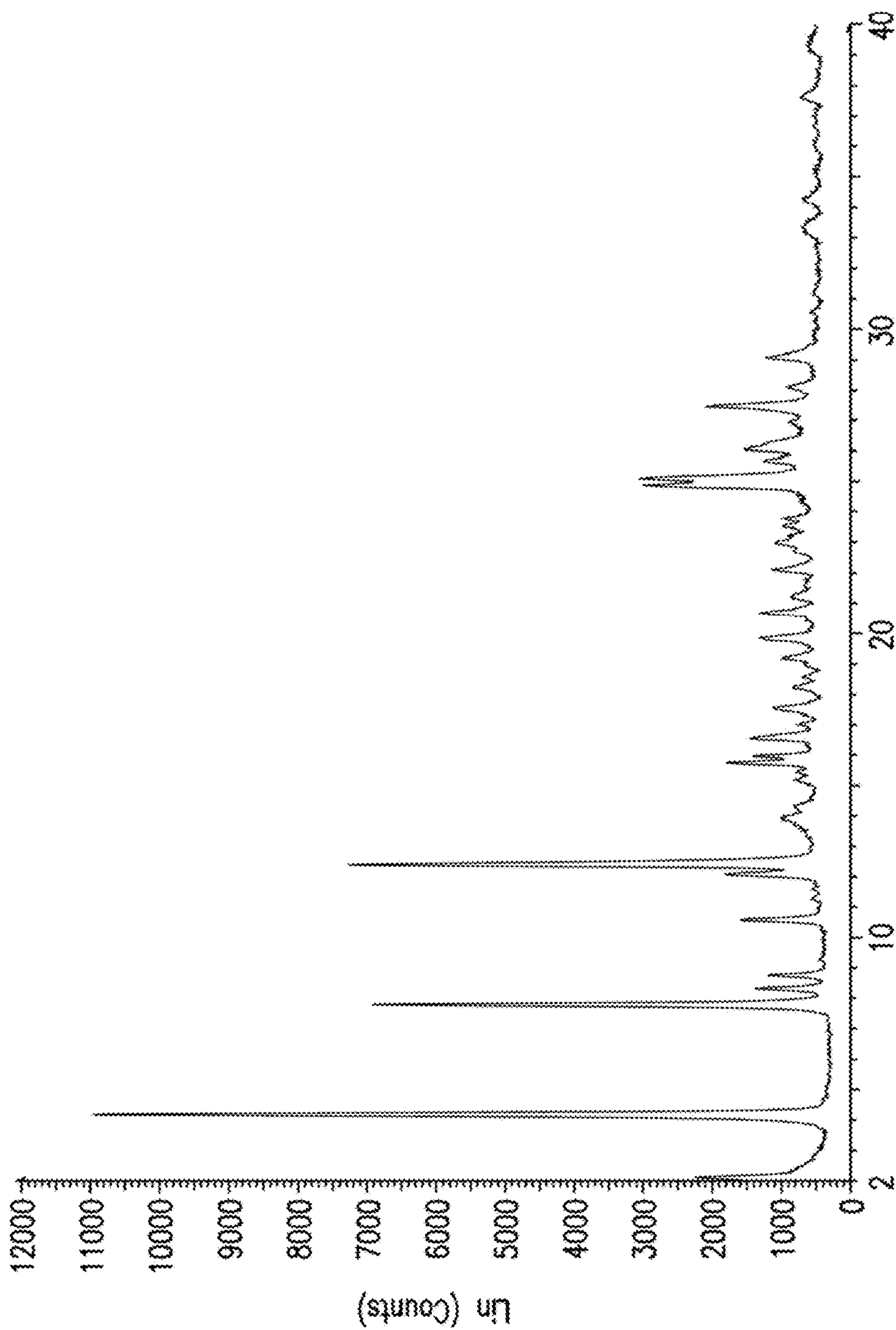
2-Theta - Scale
