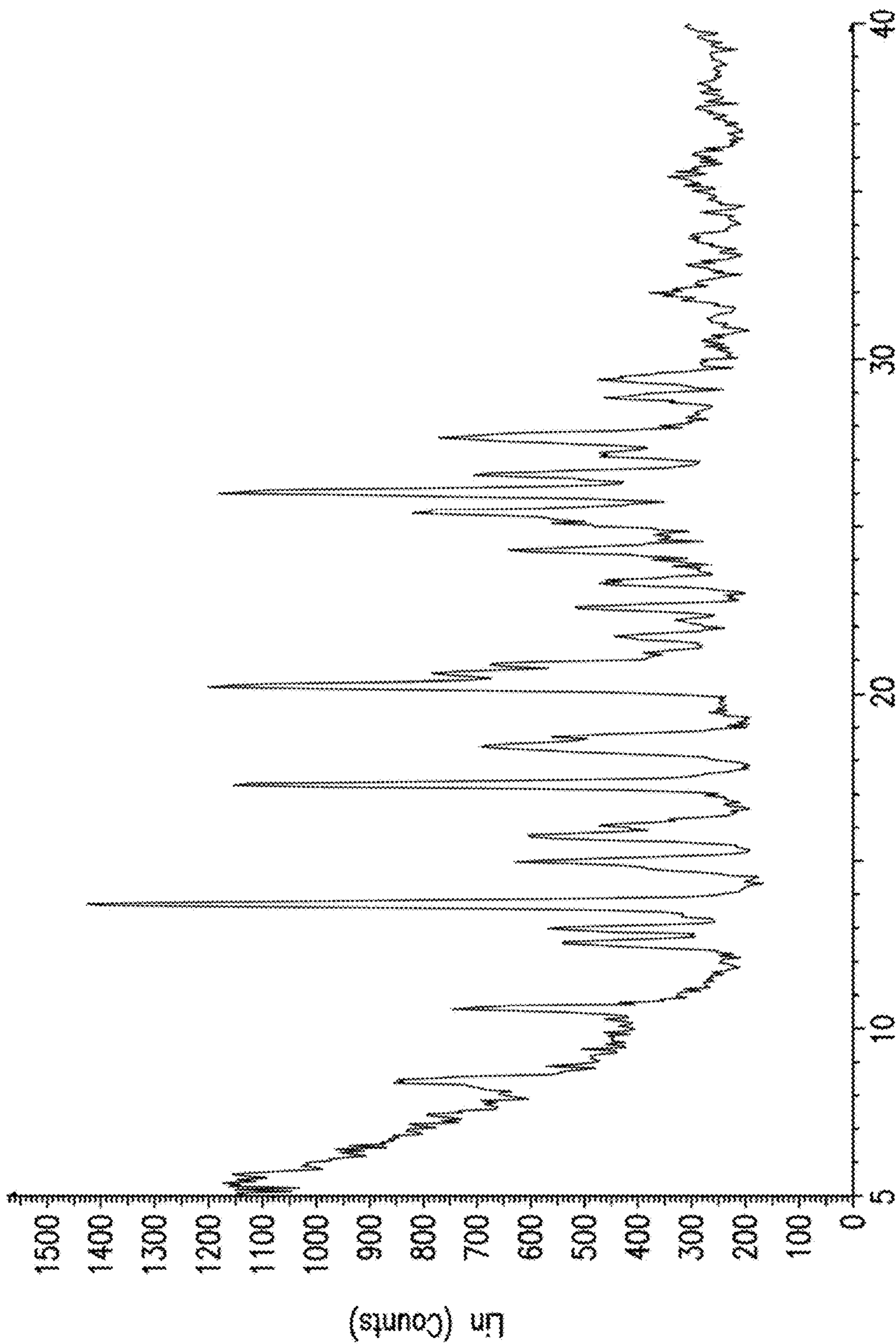
2-Theta - Scale
