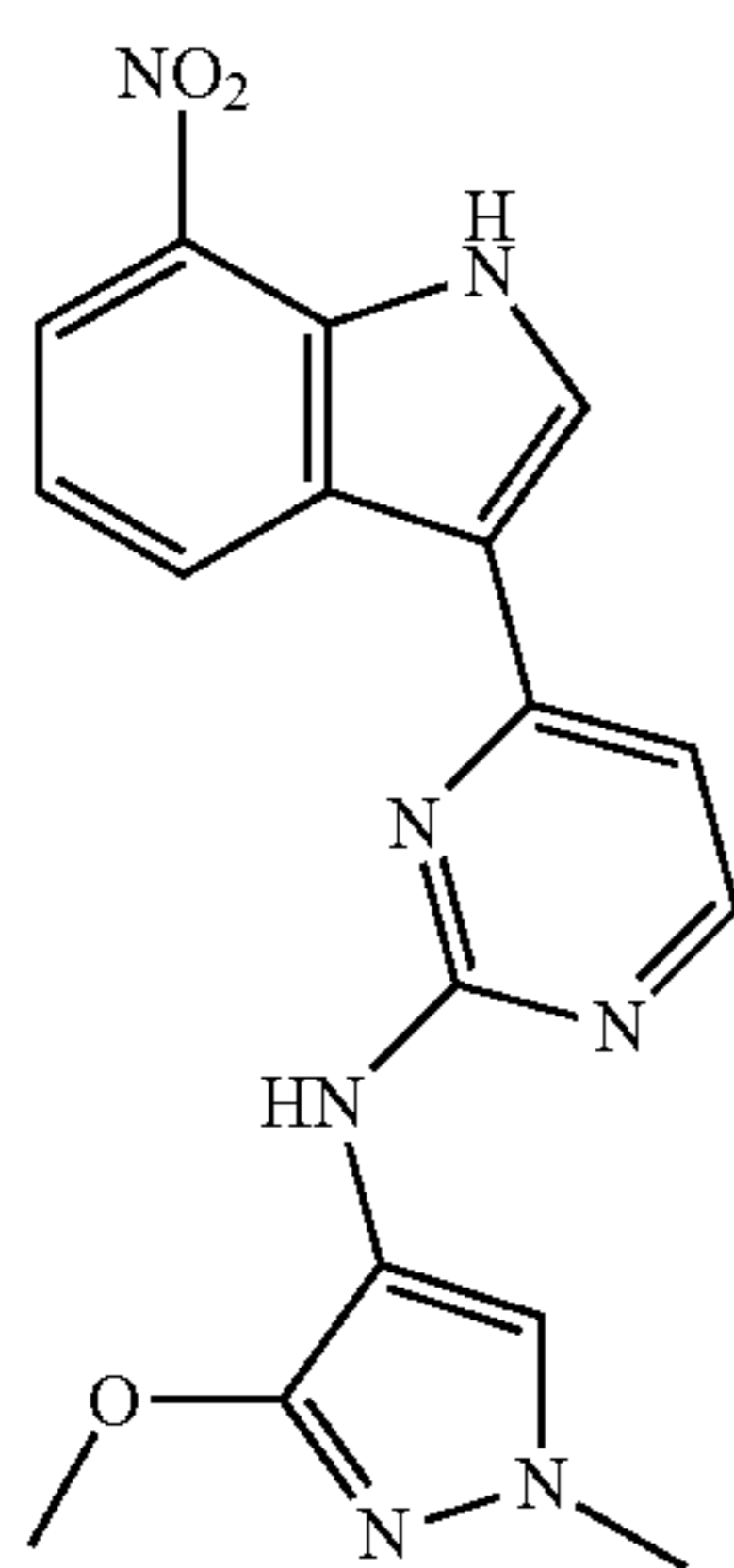
Intermediate 14: N-(3-Methoxy-1-methyl-1H-pyrazol-4-yl)-4-(7-nitro-1H-indol-3-yl)pyrimidin-2-amine
