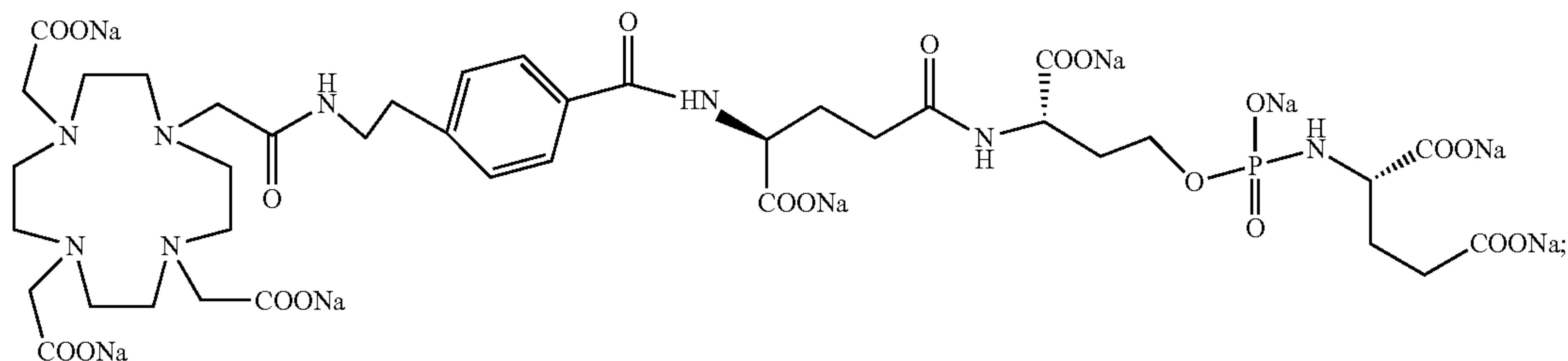
sodium (S)-2-(((S)-3-carboxylato-3-((S)-4-carboxylato-4-(4-(2-(2-(4,7,10-tris(carboxylatomethyl)-1,4,7,10-tetraazacyclododecan-1-yl)acetamido)ethyl)benzamido)butanamido)propoxy)oxidophosphoryl)amino)pentanedioate
