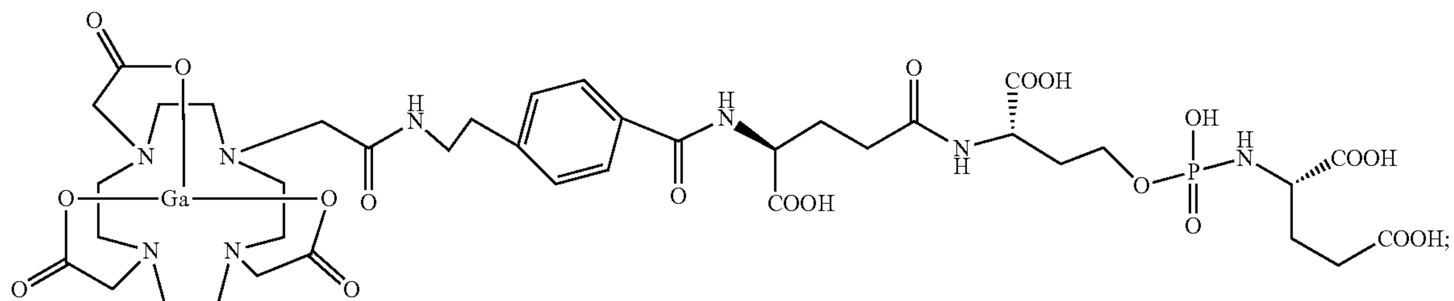
gallium 2,2',2''-(10-(2-((4-(((1S)-1-carboxy-4-(((1S)-1-carboxy-3-(((S)-1,3-dicarboxypropyl)amino)hydroxyl)phosphoryl)oxy)propyl)amino)-4-oxobutyl)carbamoyl)phenethyl)amino)-2-oxoethyl)-1,4,7,10-tetraazacyclododecane-1,4,7-triyl)triacetate
