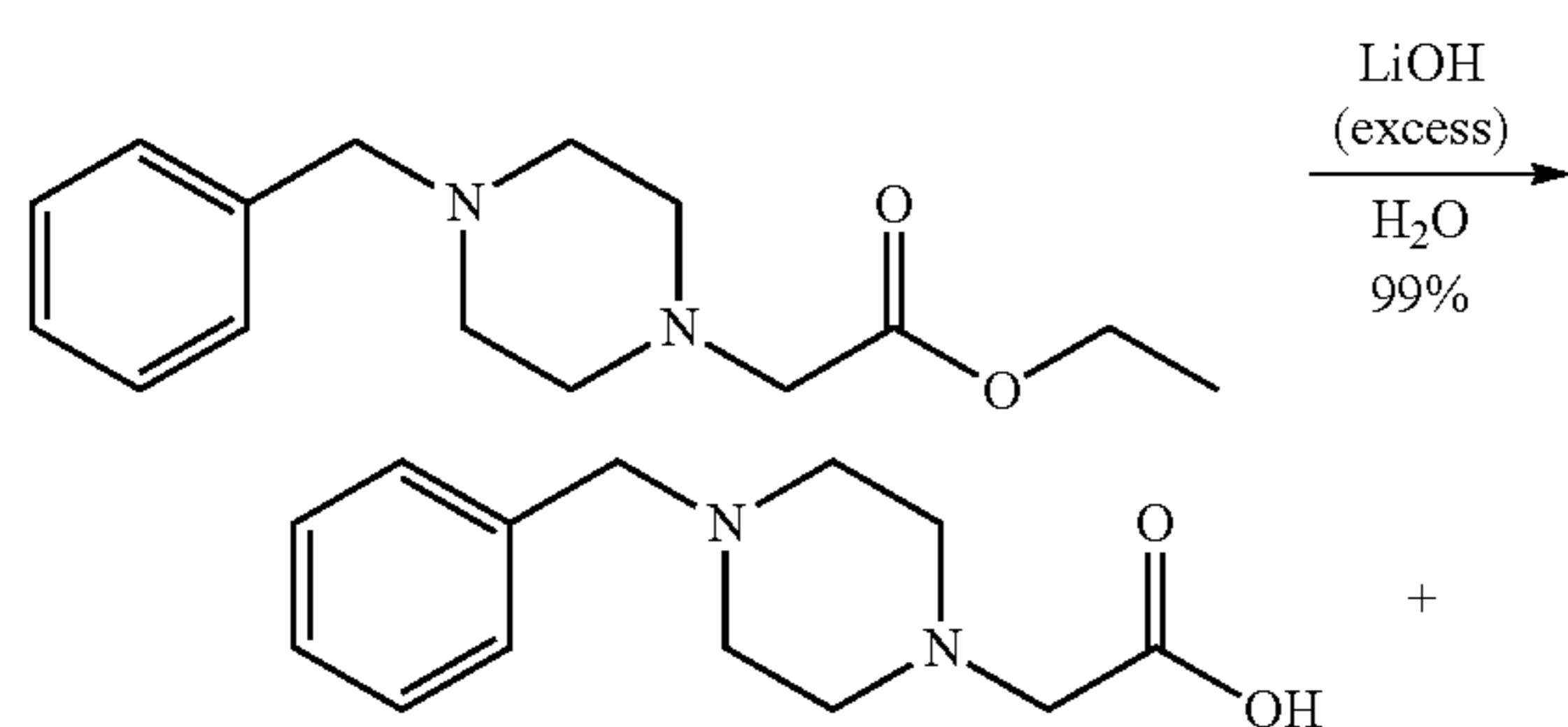
Scheme for DX16
