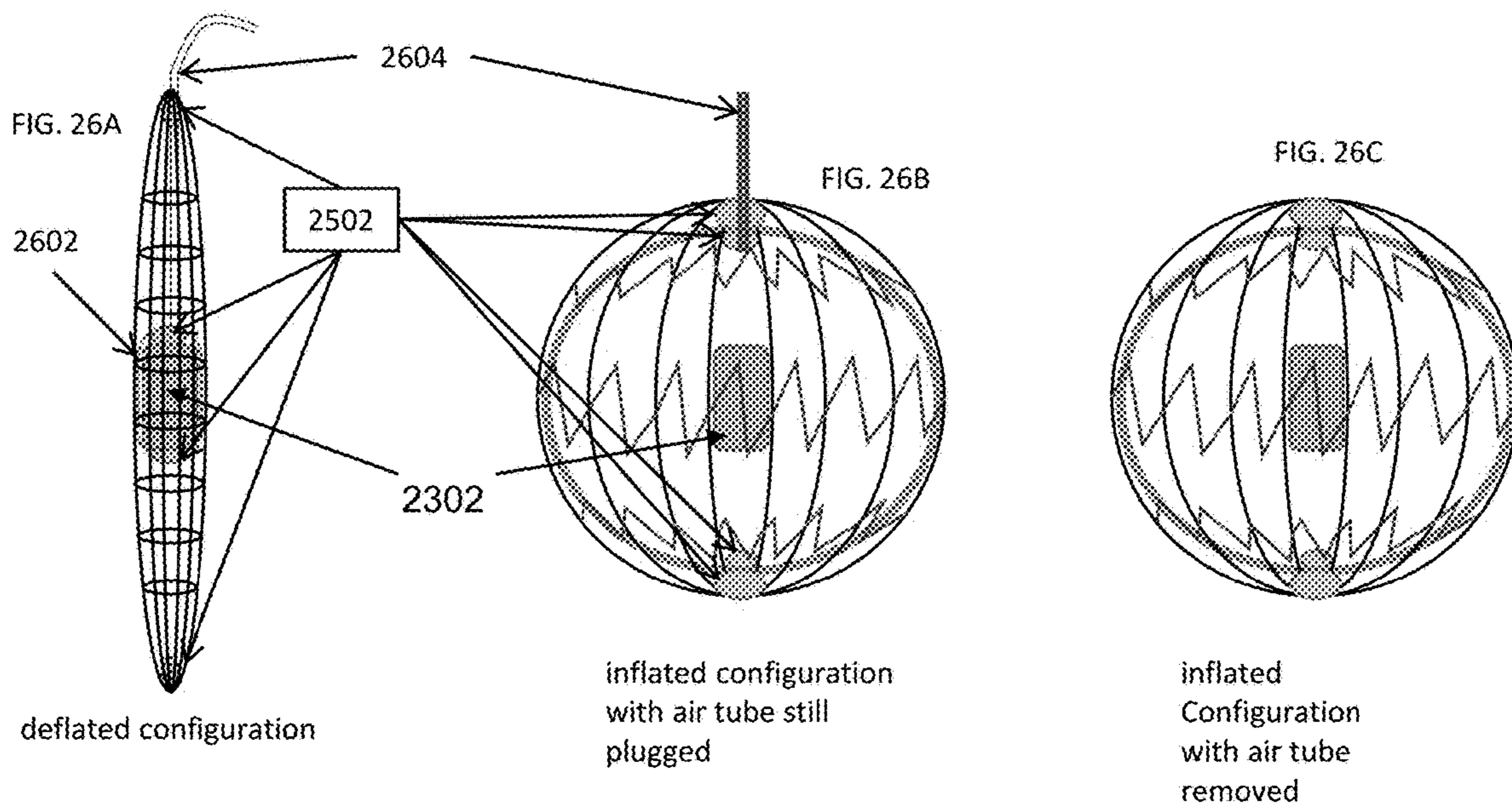
Magnet free-floating in a balloon inside the lantern-shaped structure
