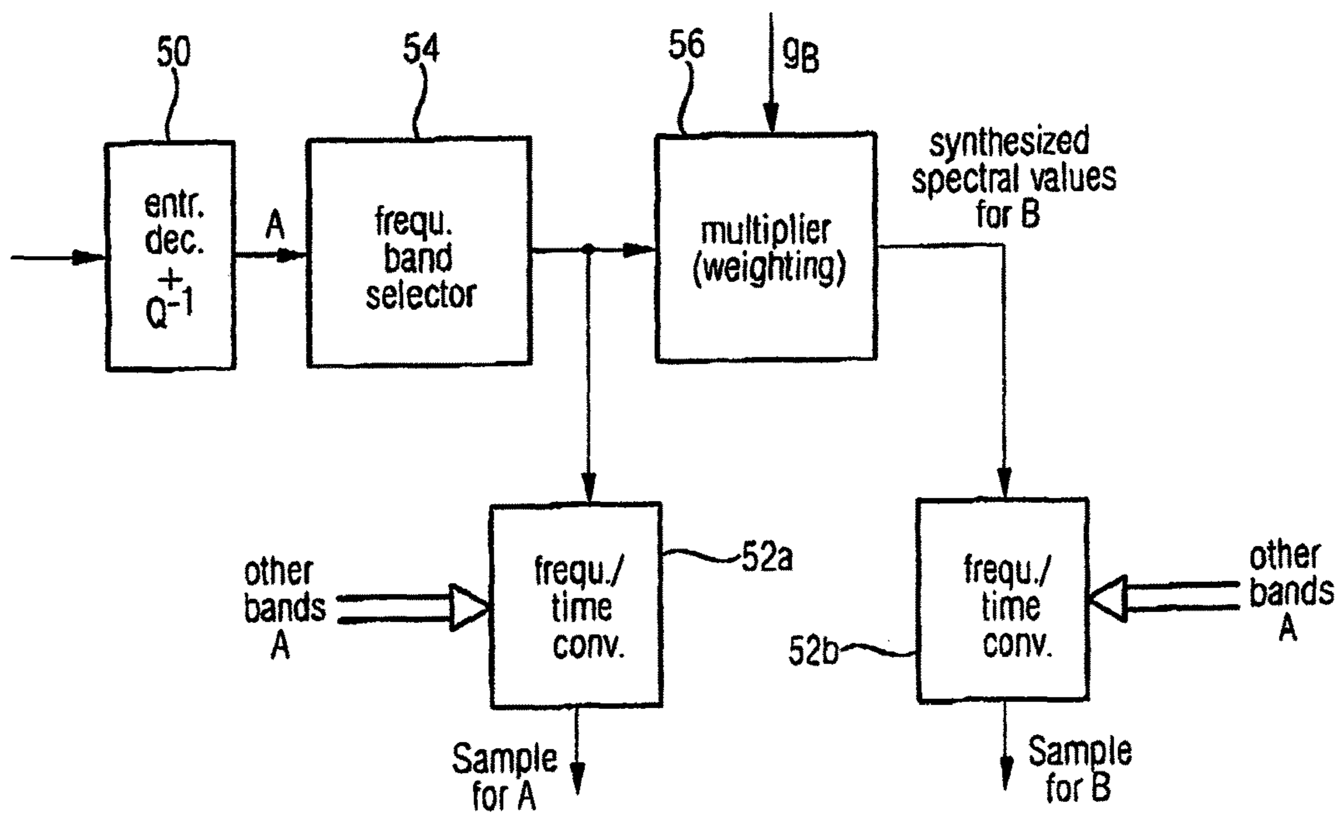
FIG 5 (decoder side)
