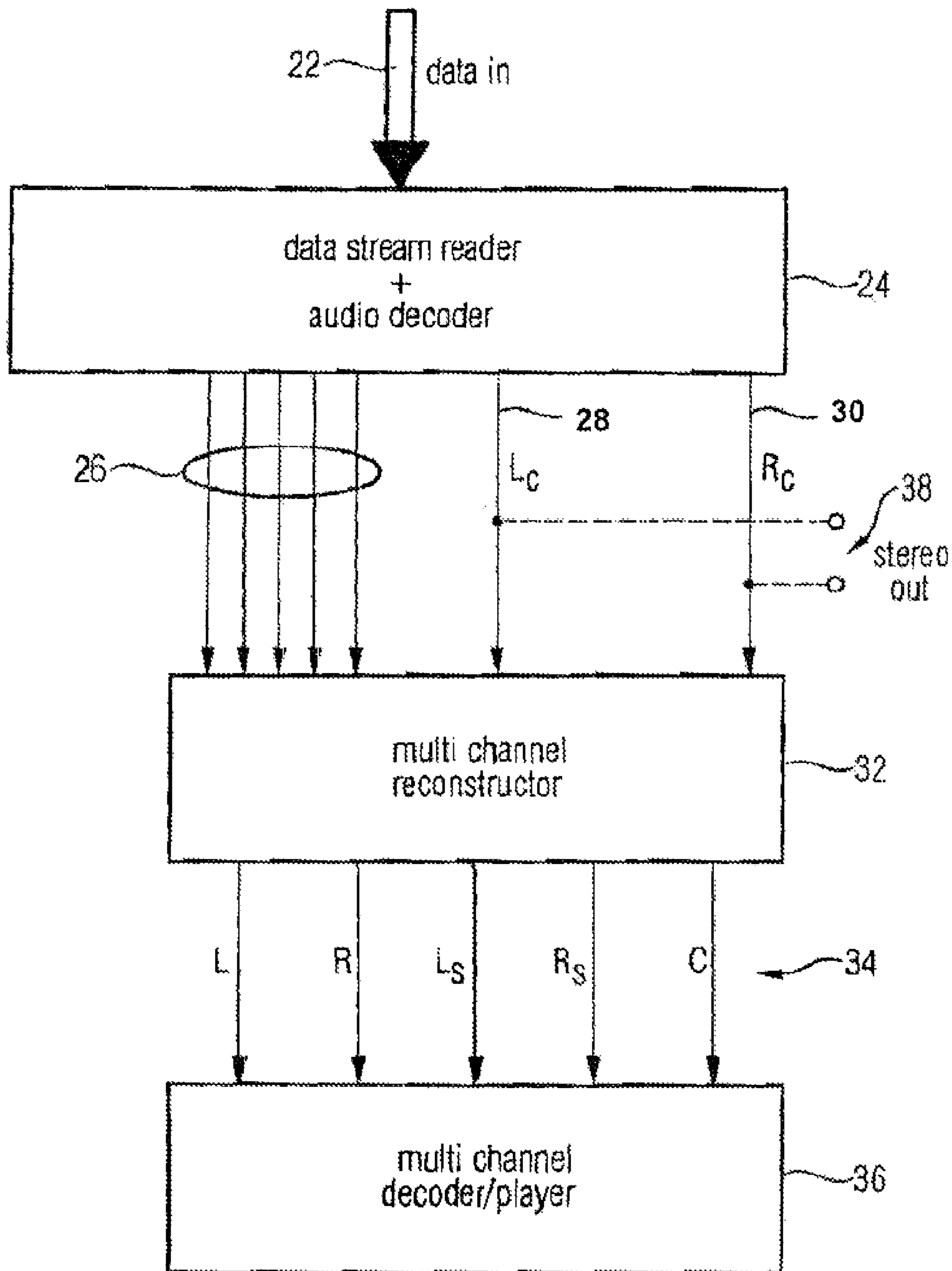
FIG 2 (Decoder)
