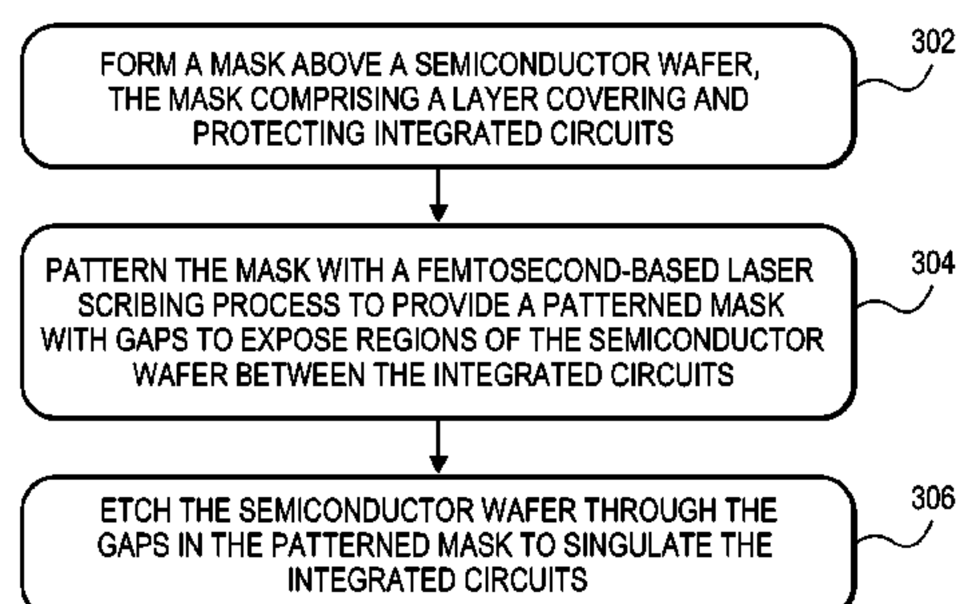
FLOWCHART 300
