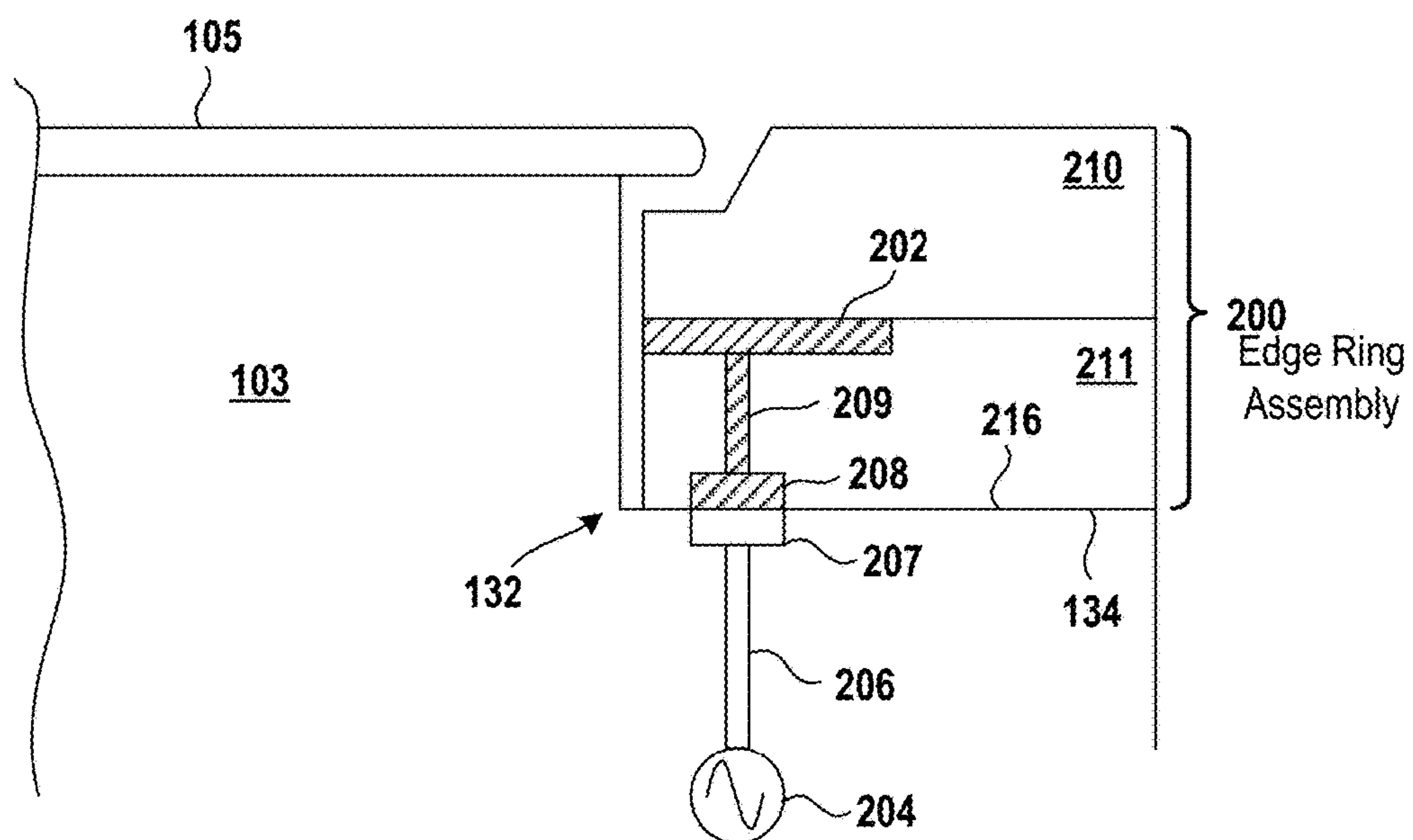
FIG. 2D
