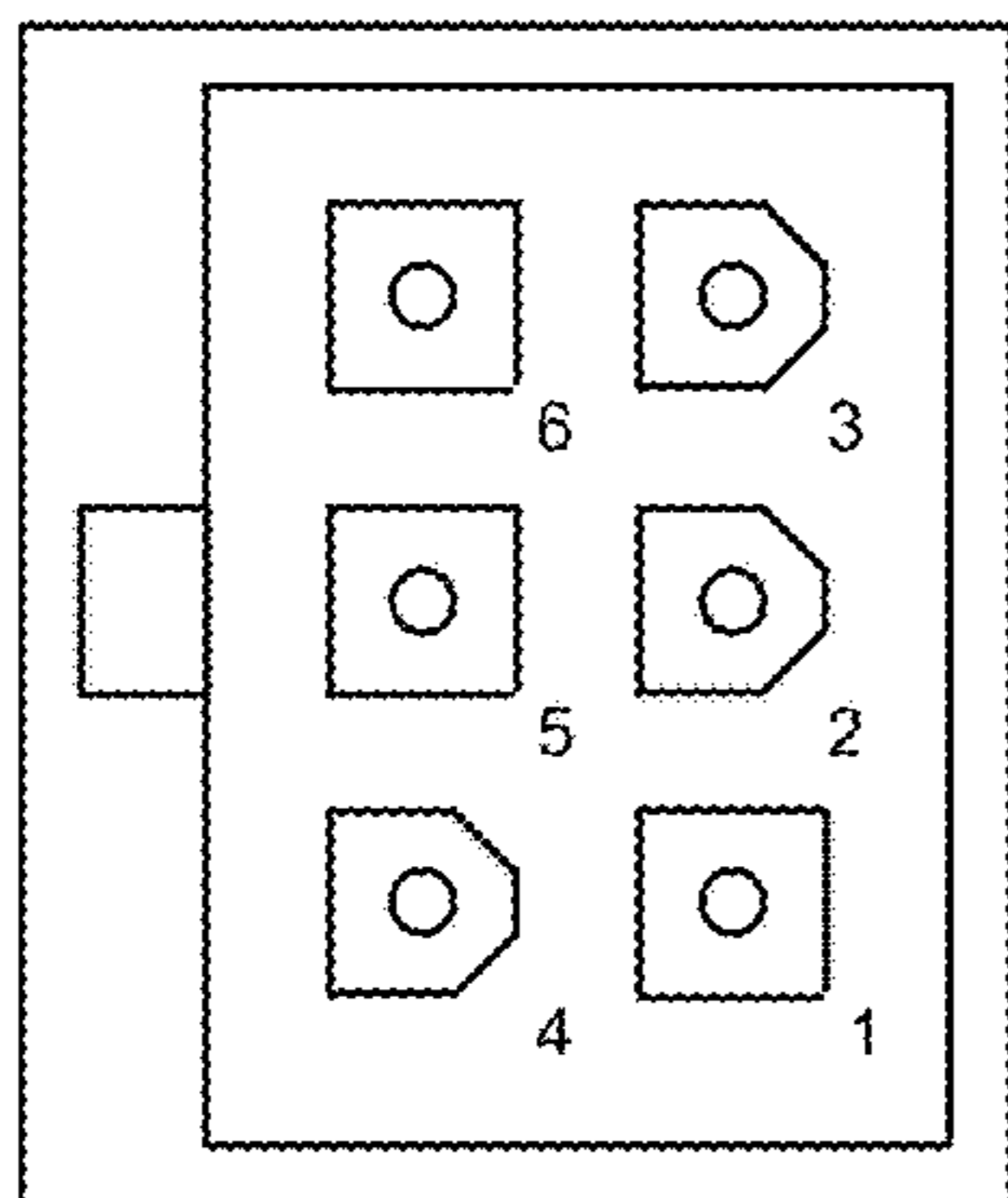
Peripheral Connector Face View Receptacle (Sockets)
