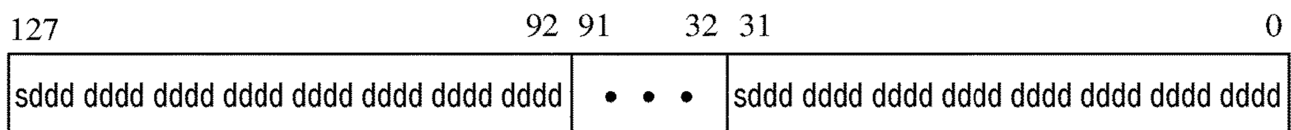
349 — SIGNED PACKED DOUBLEWORD REPRESENTATION
