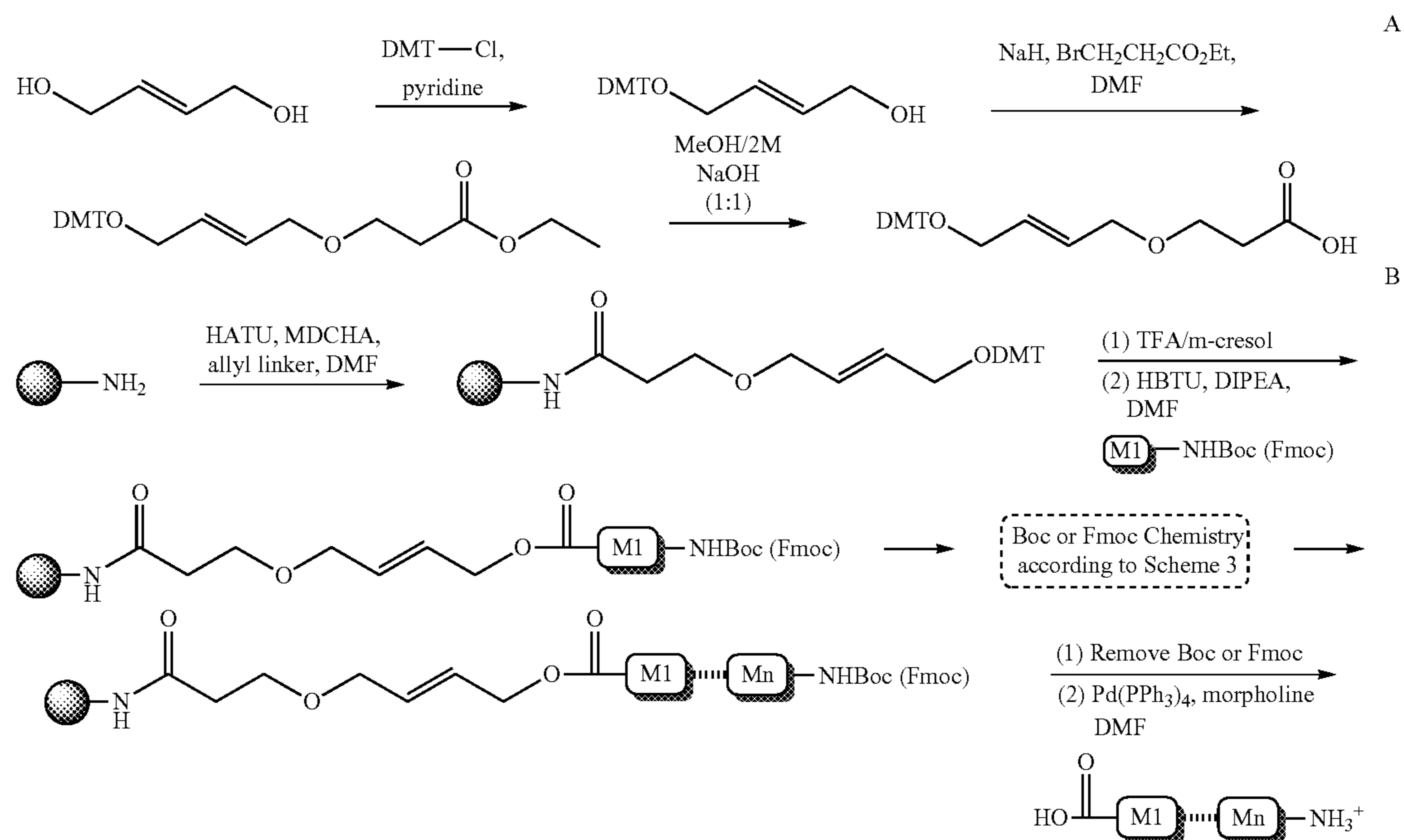
Scheme 4
