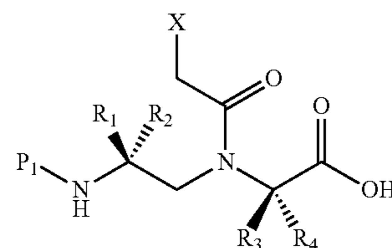
MONOMERS
