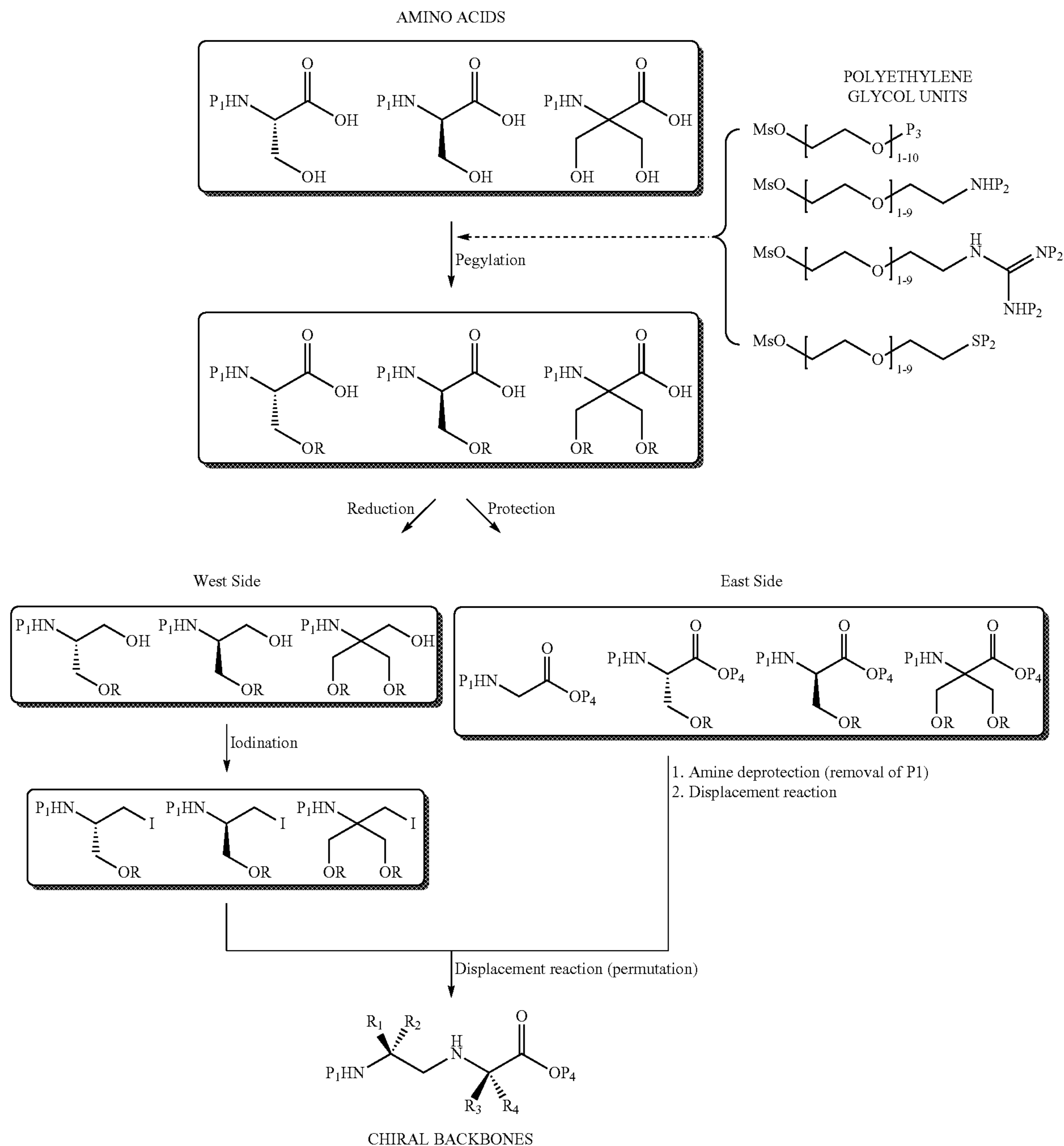
Scheme 2
