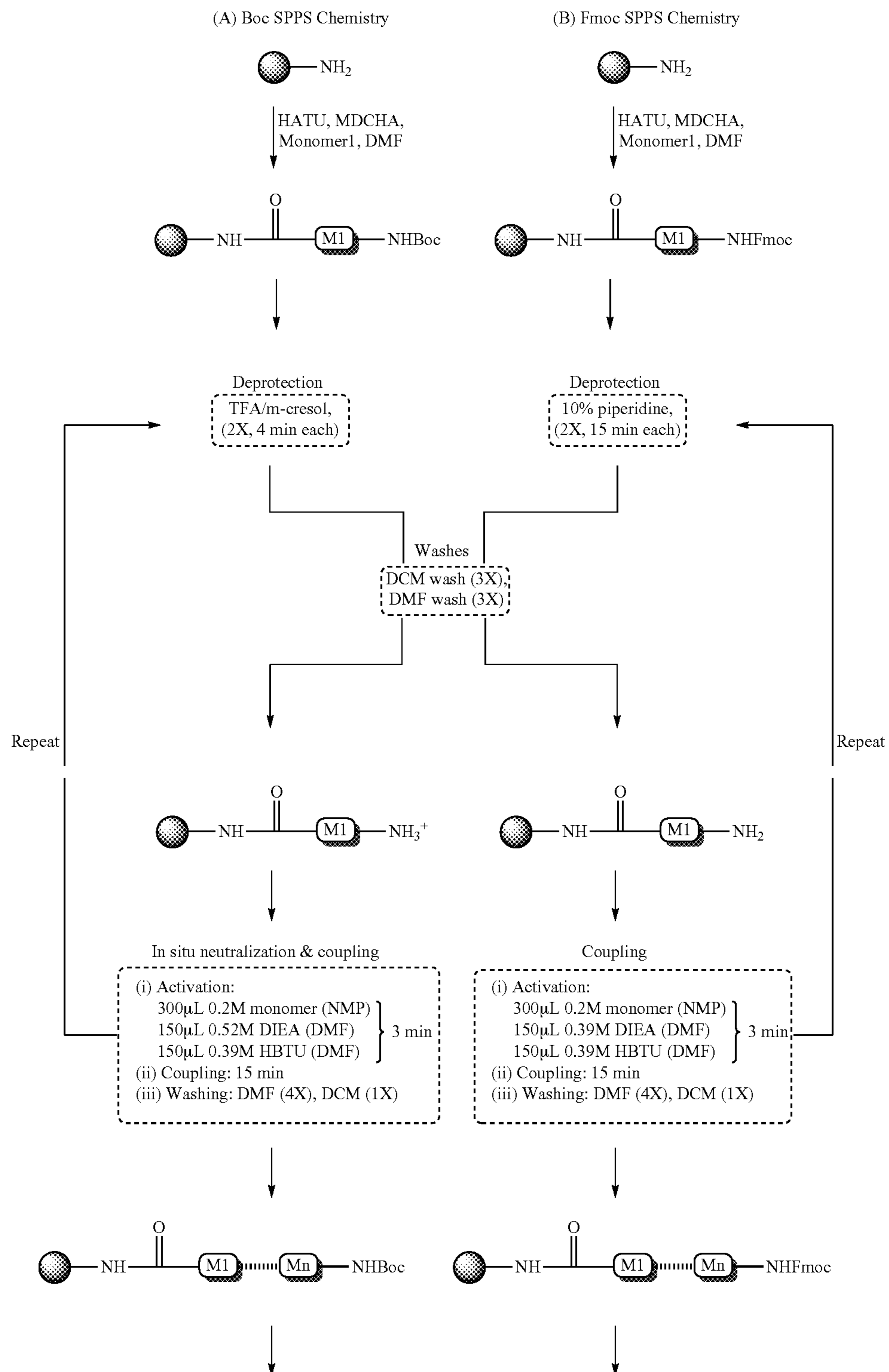
Scheme 3
