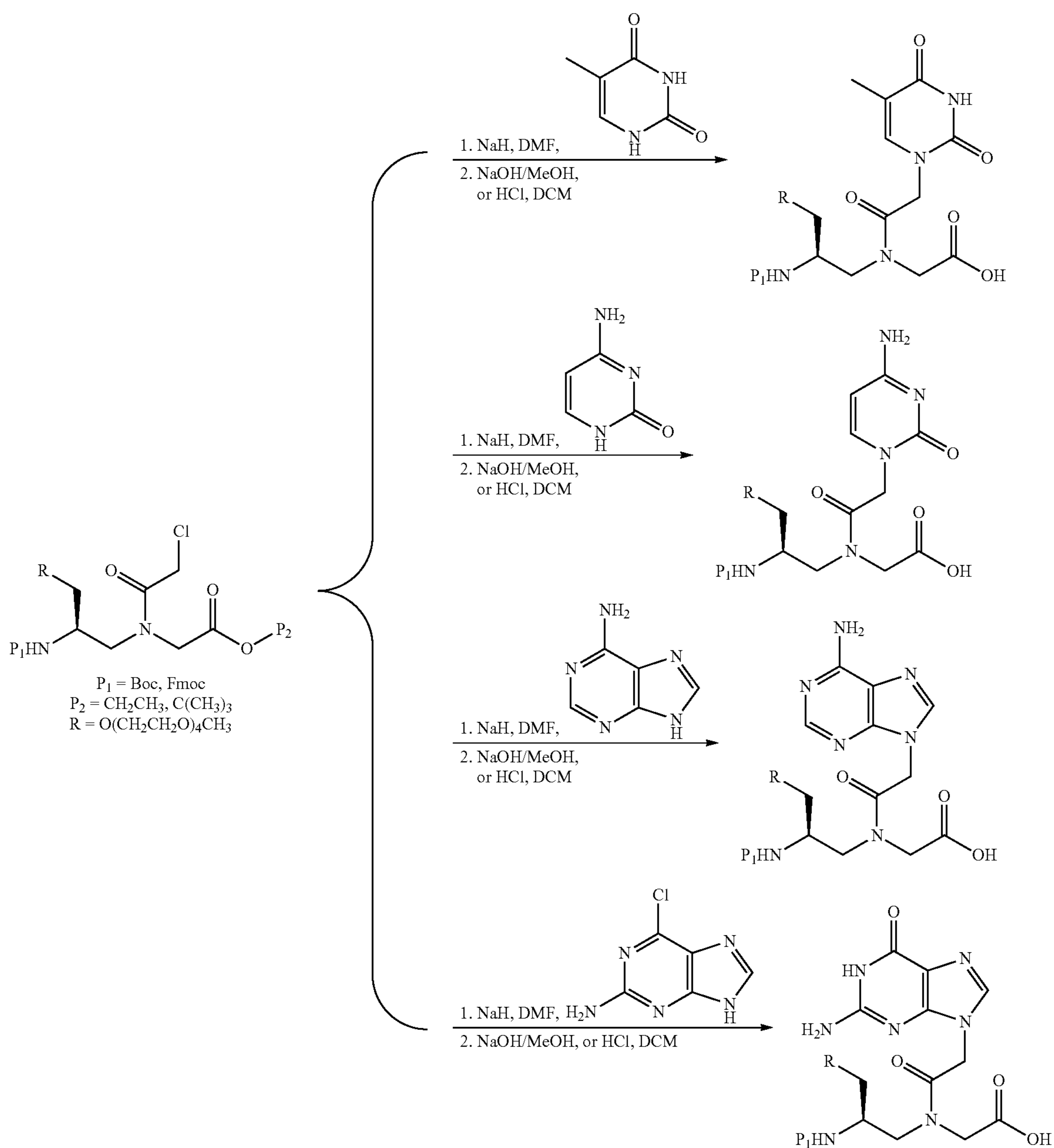
Scheme 1
