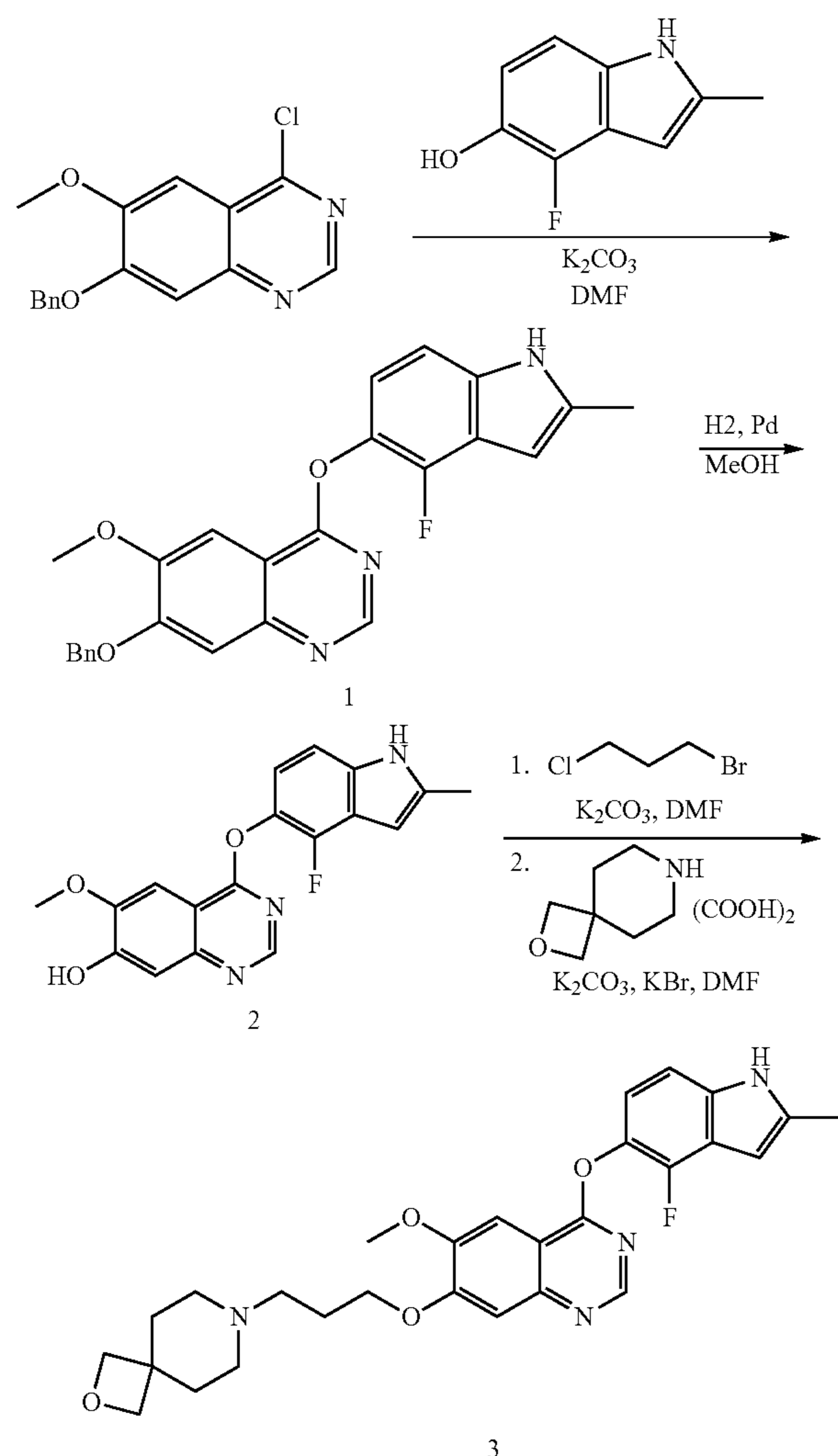
Scheme 1: Method A of synthesizing Compound 3.
