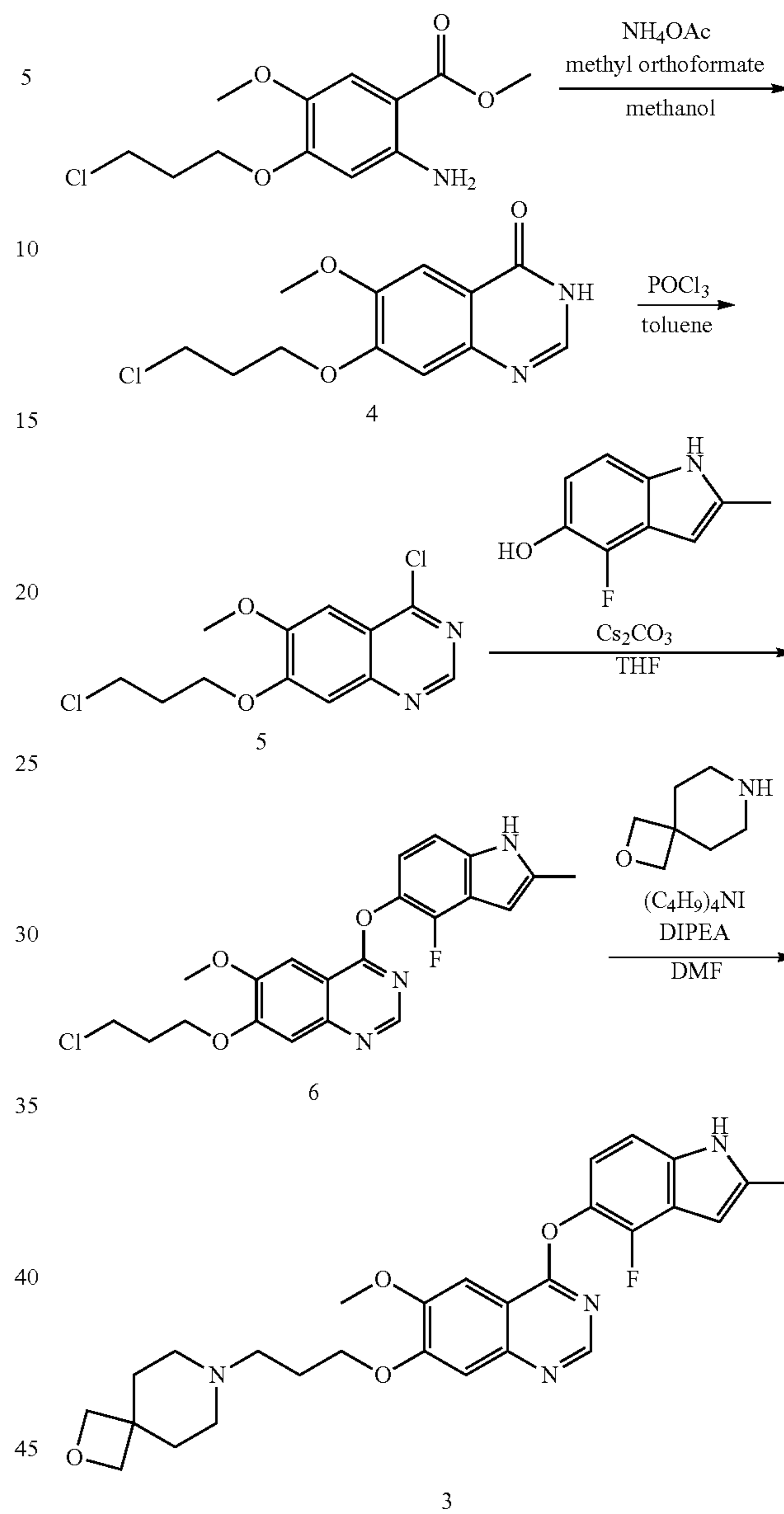
Scheme 2: Method B of synthesizing Compound 3.
