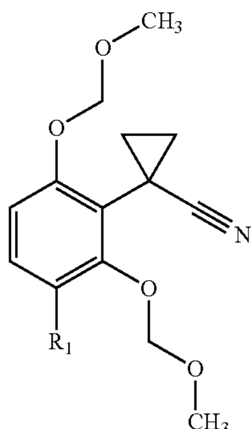
1-[2,6-bis(methoxymethoxy)-3-methyl-phenyl]cyclopropanecarbonitrile
