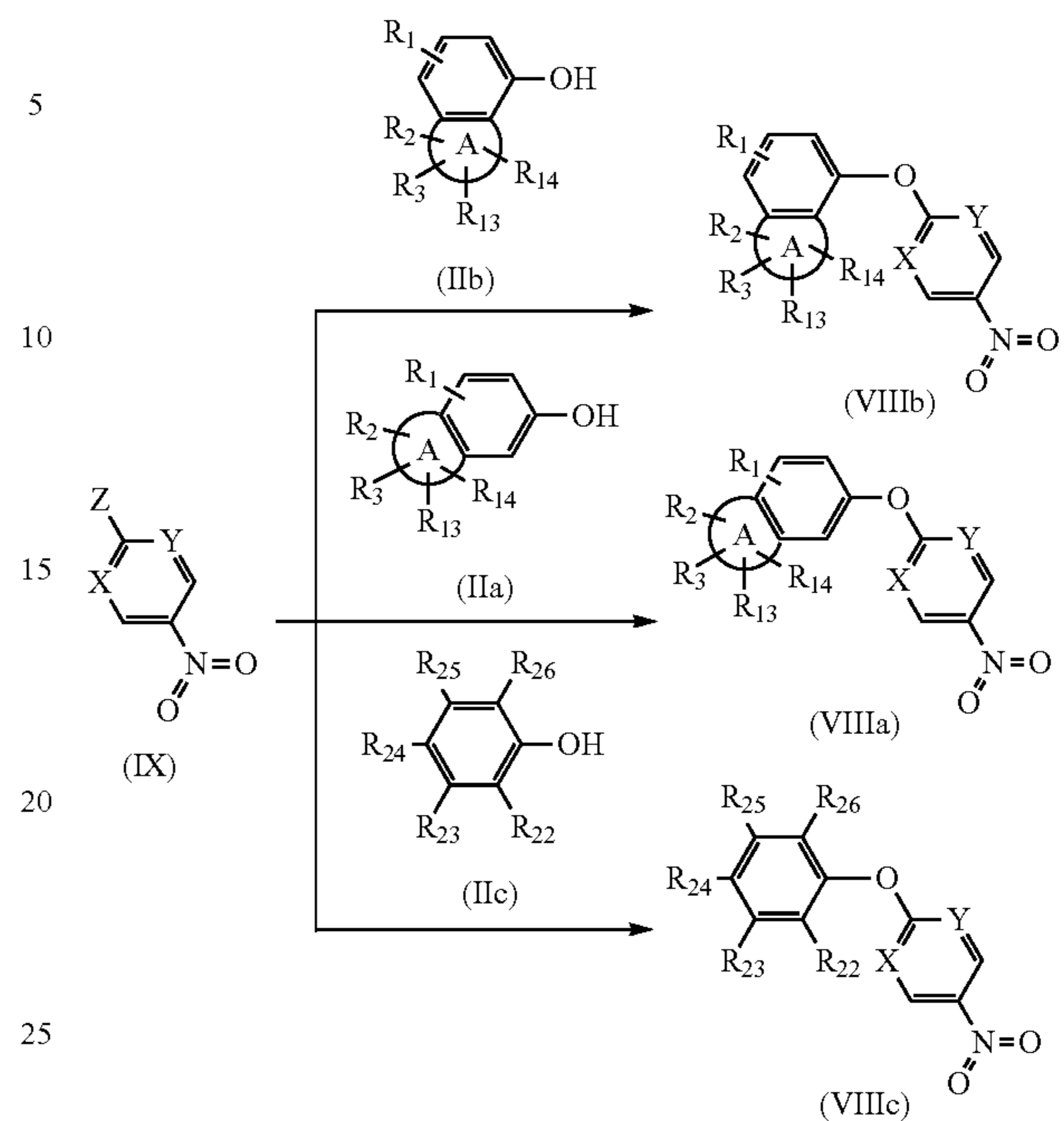
Scheme 4
