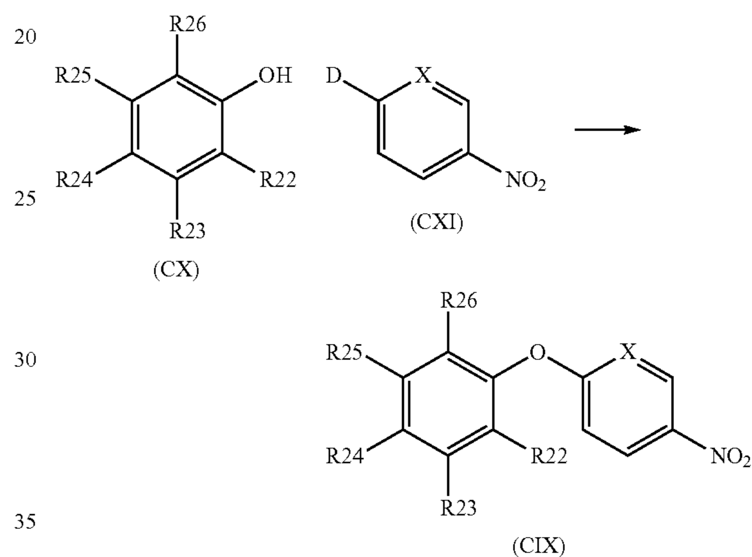
Scheme 14
