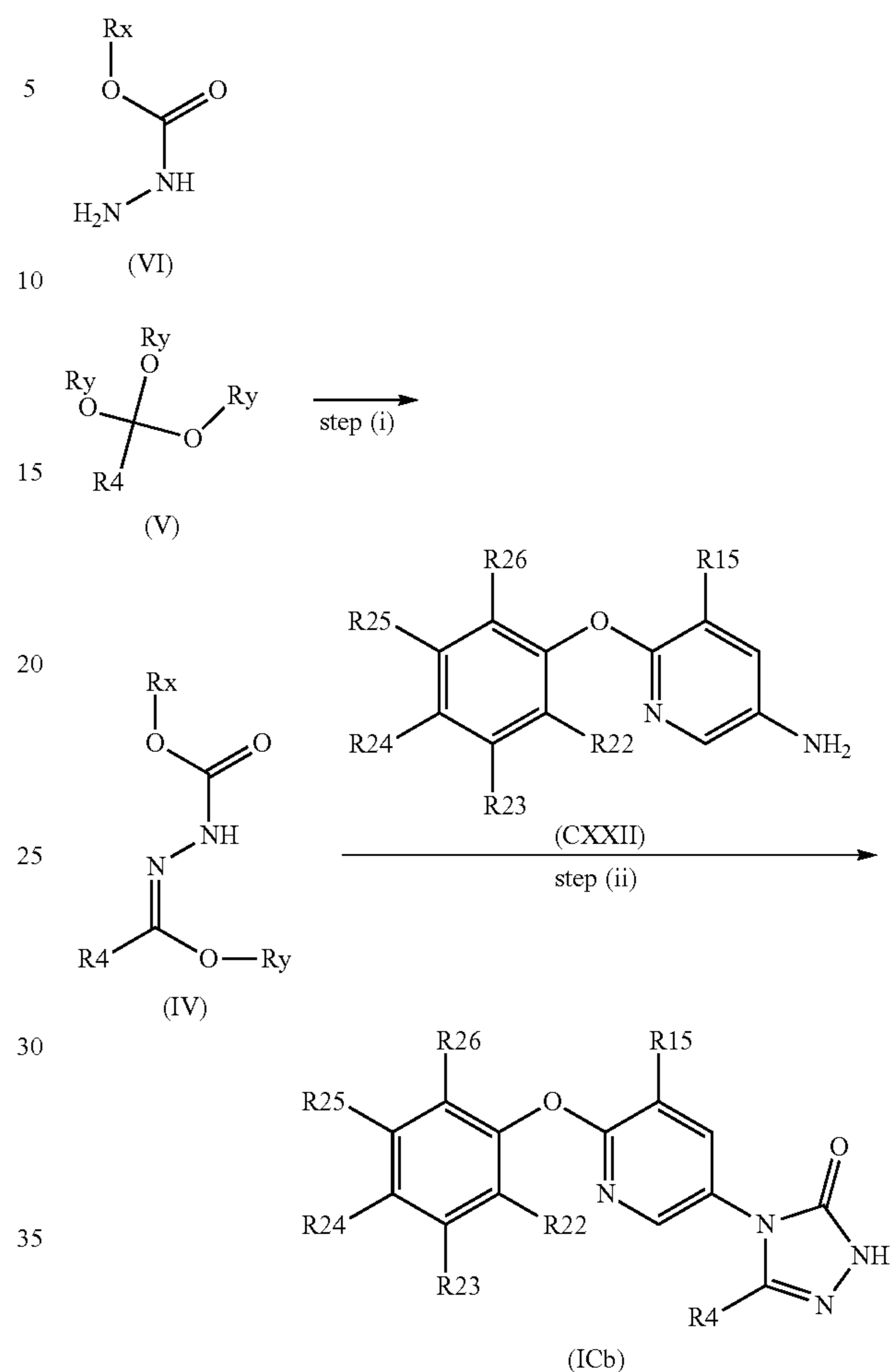
Scheme 23
