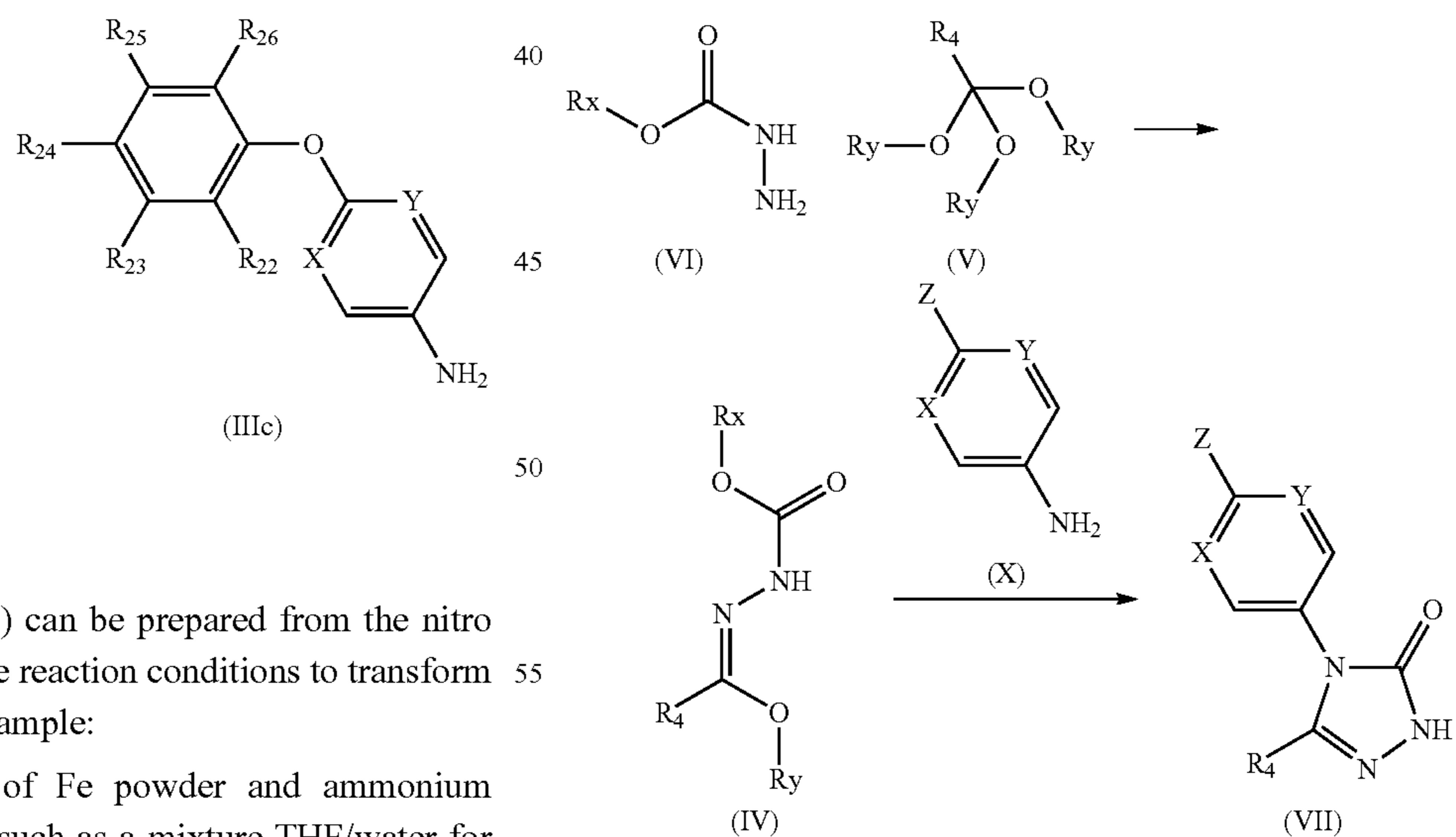
Scheme 5
