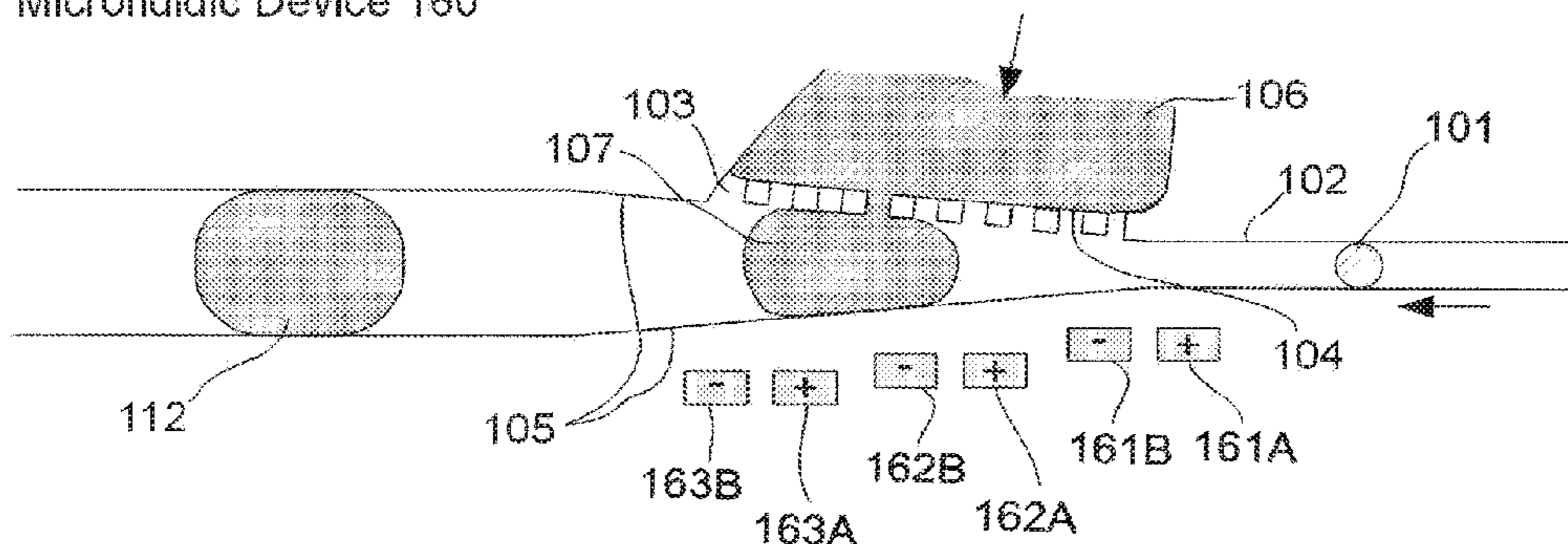
Microfluidic Device 160
