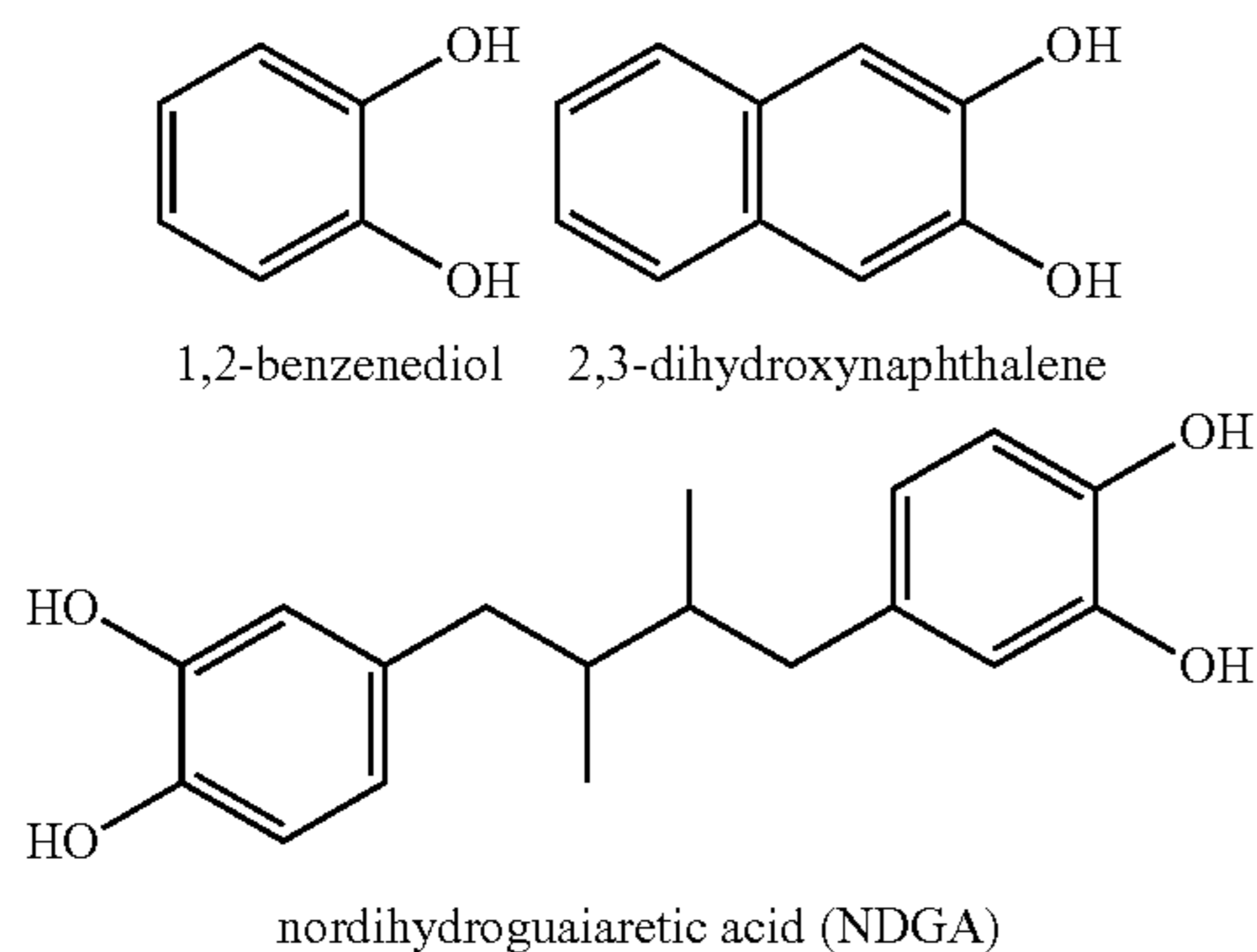
Scheme 2: Exemplary catechols.
