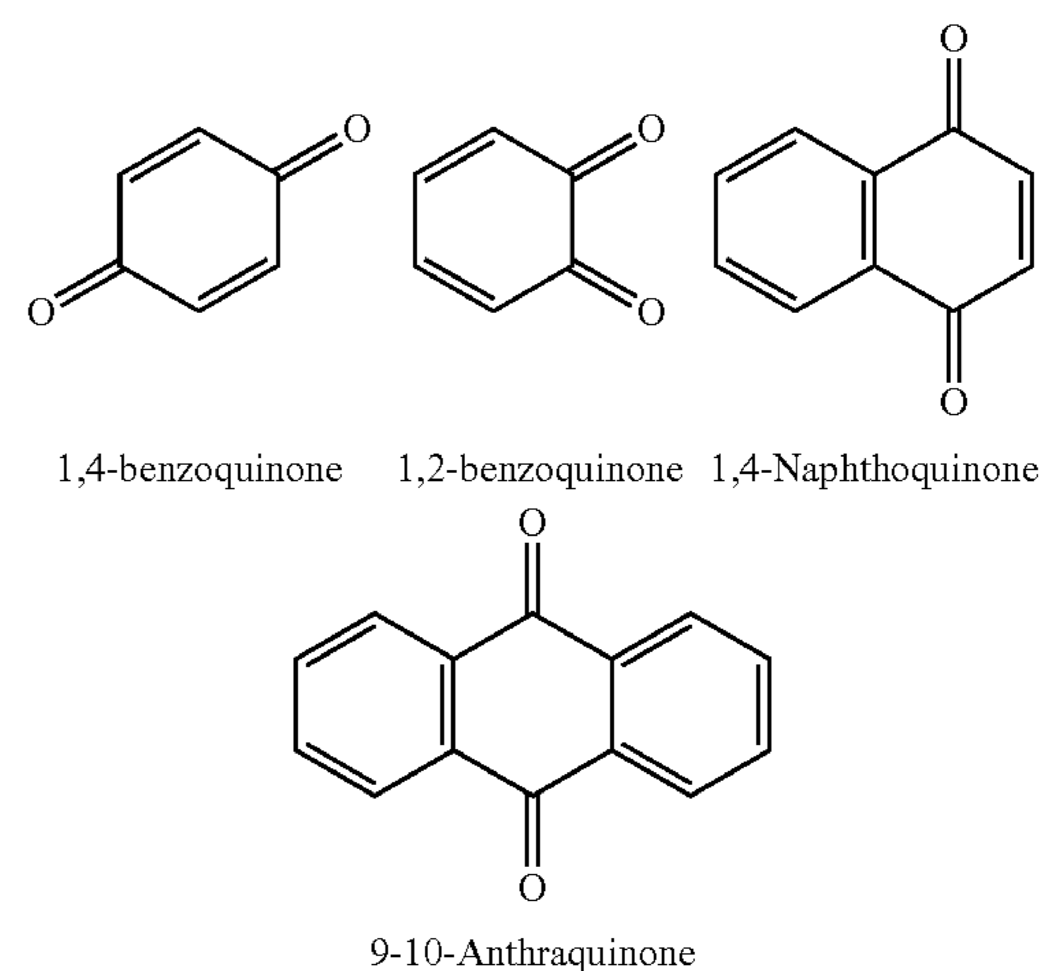
Scheme 1: Exemplary quinones.
