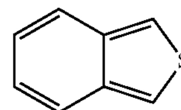
2-benzothiophene
