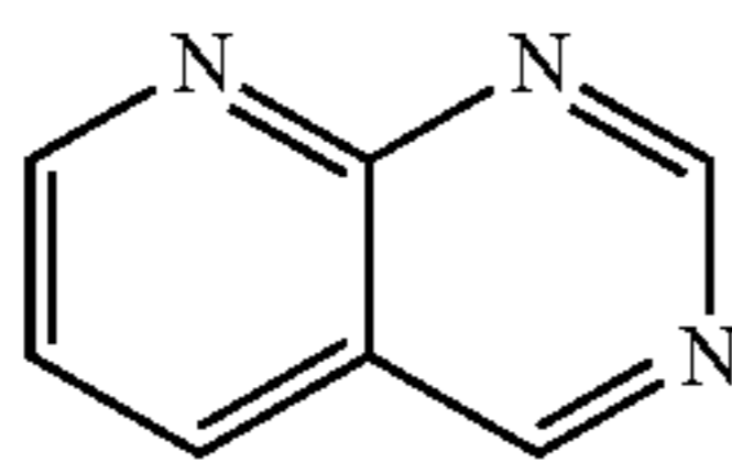
Pyrido[2,3- d]pyrimidine
