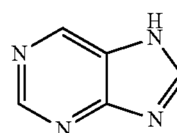
7H-purine
