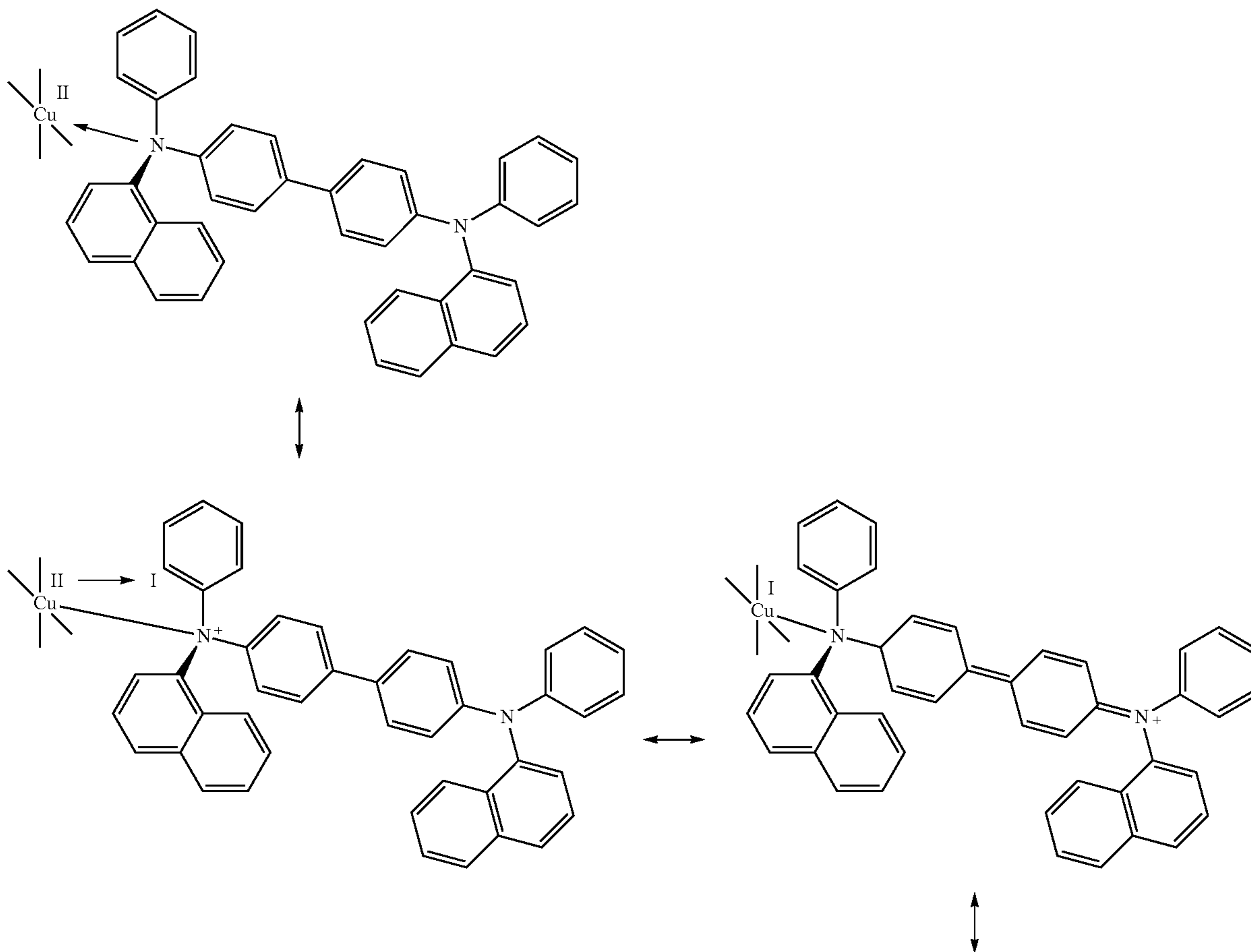
Scheme 1
