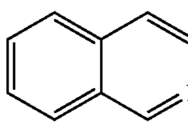
isoquinoline
