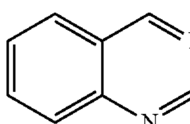
Quinazoline
