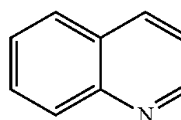
quinoline
