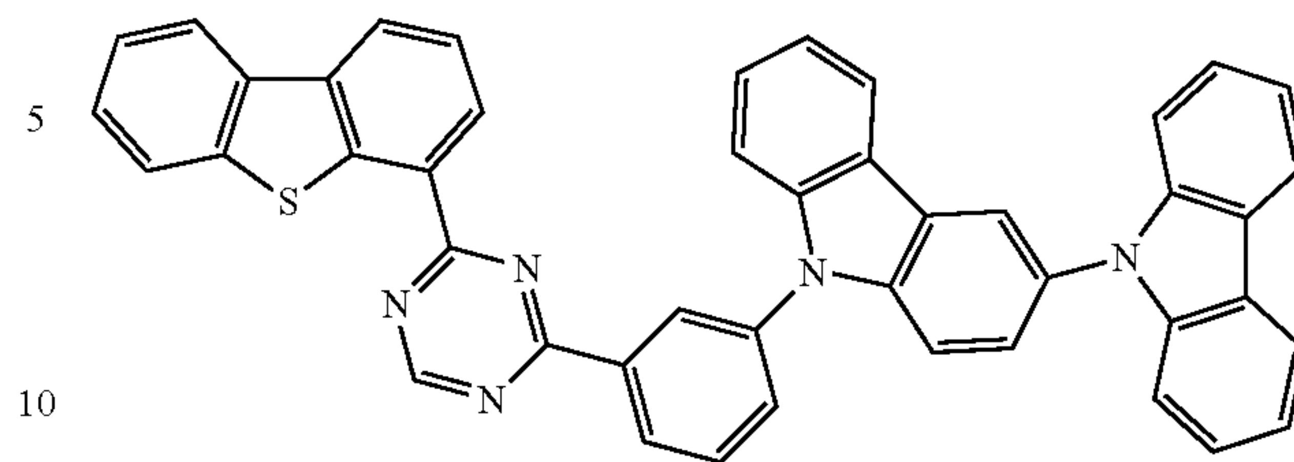
Compound A
