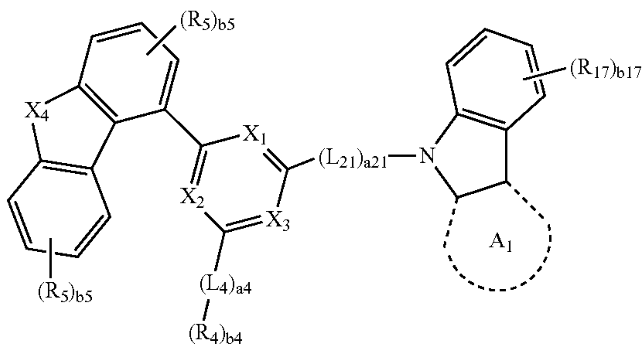
Formula 1A(4)
