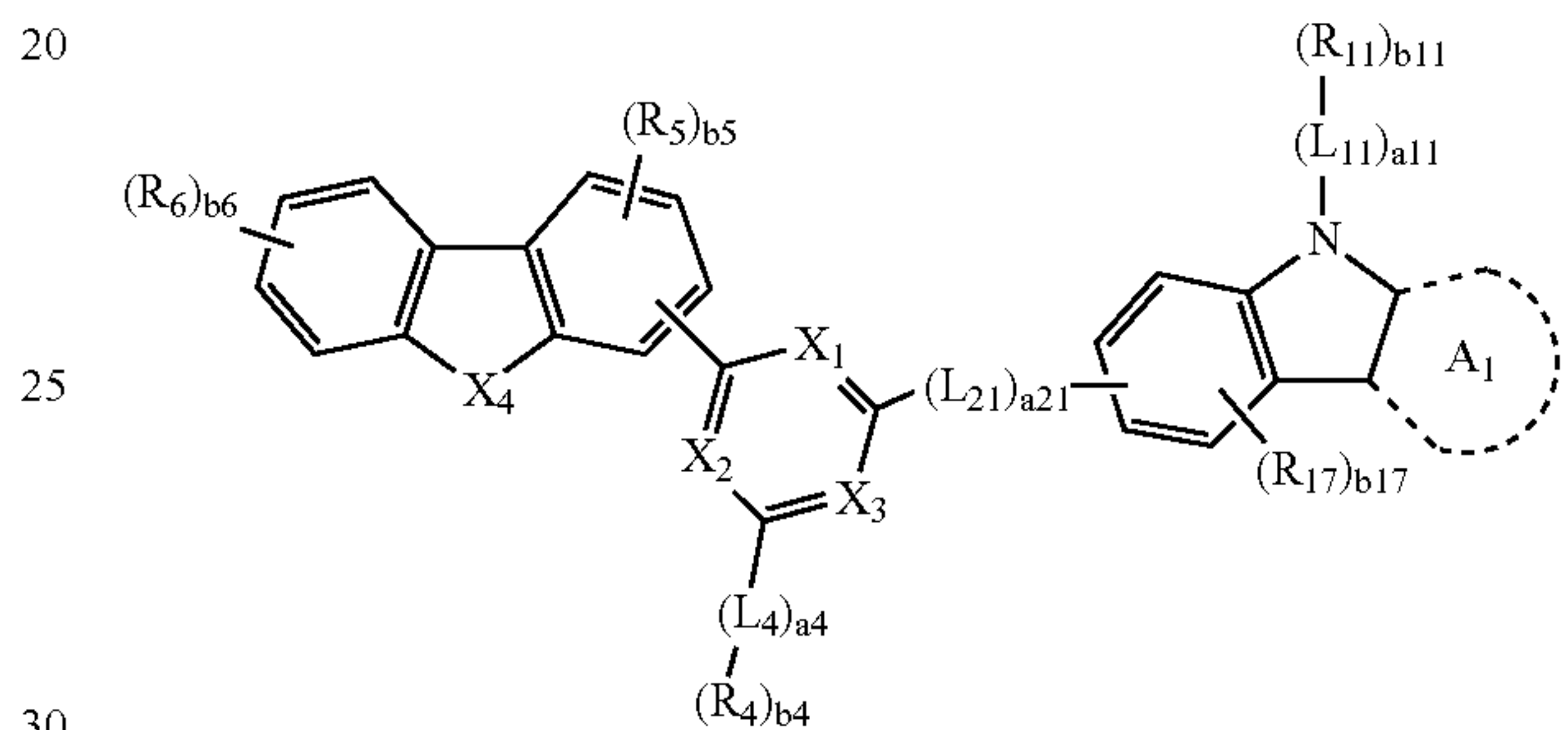
Formula 1B
