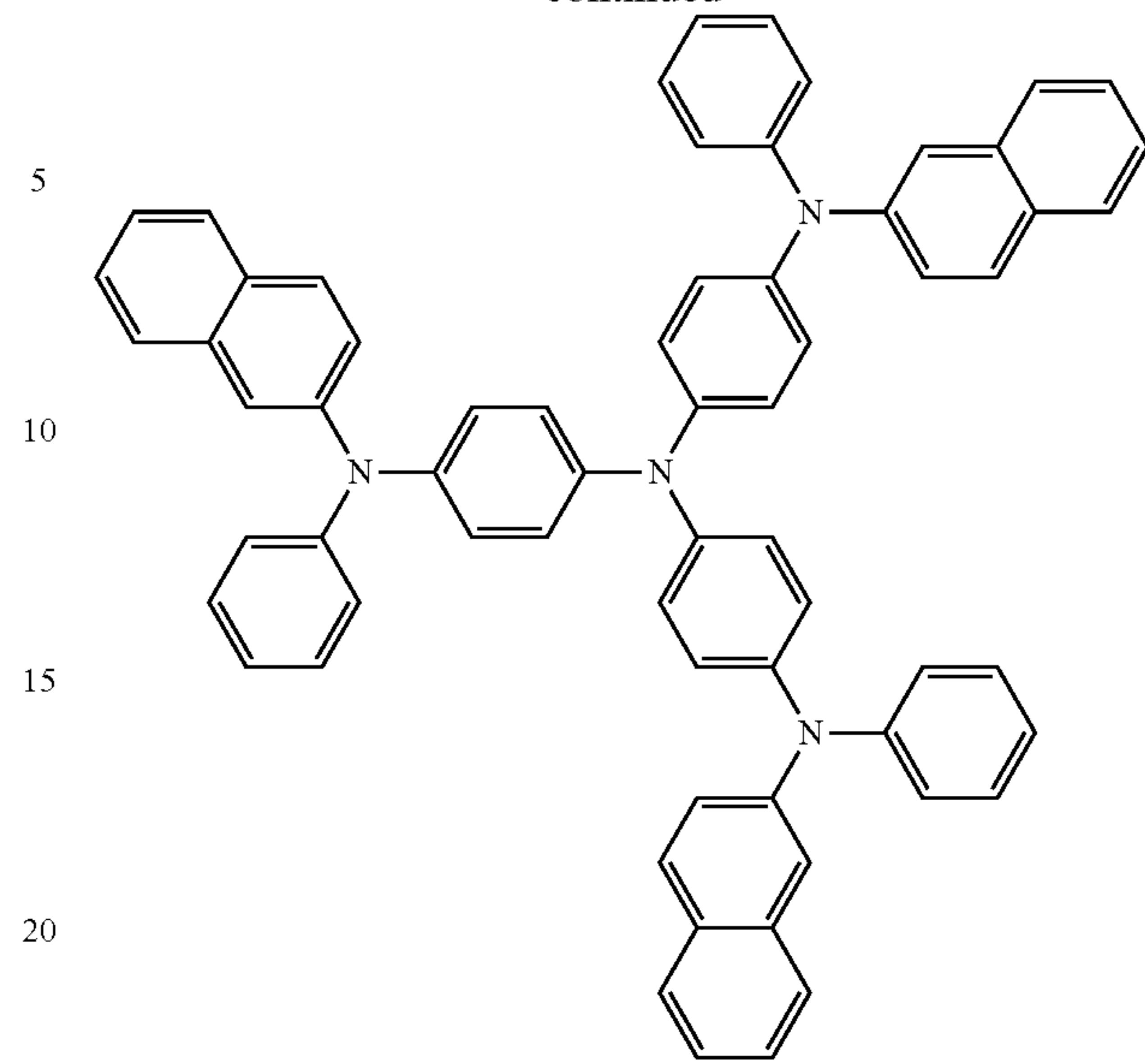
2-TNATA
