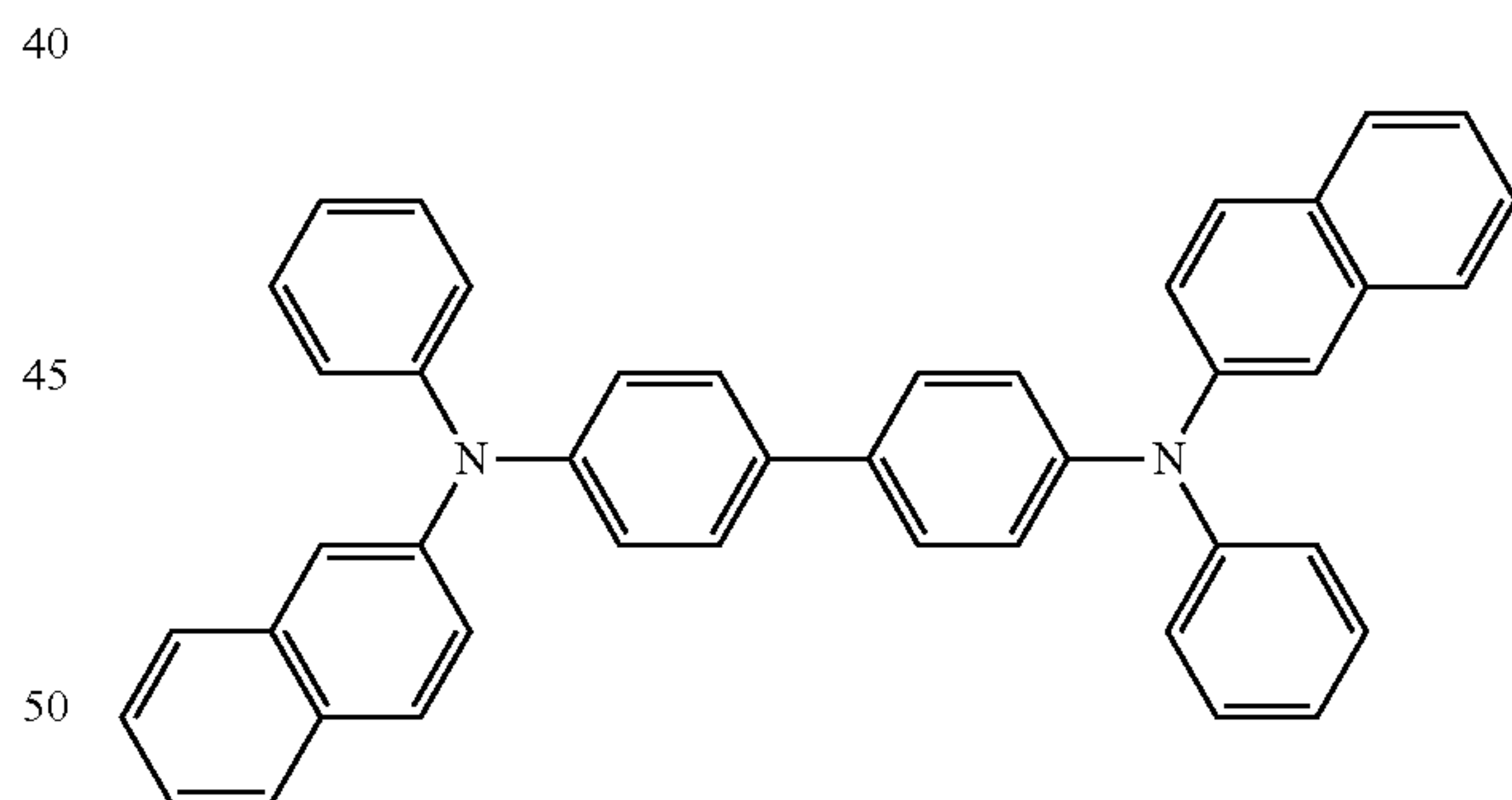
\beta -NPB
