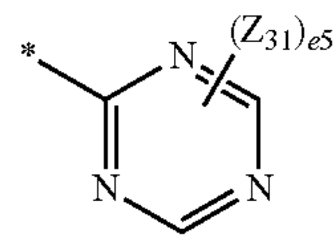
Formula 4-2 30
