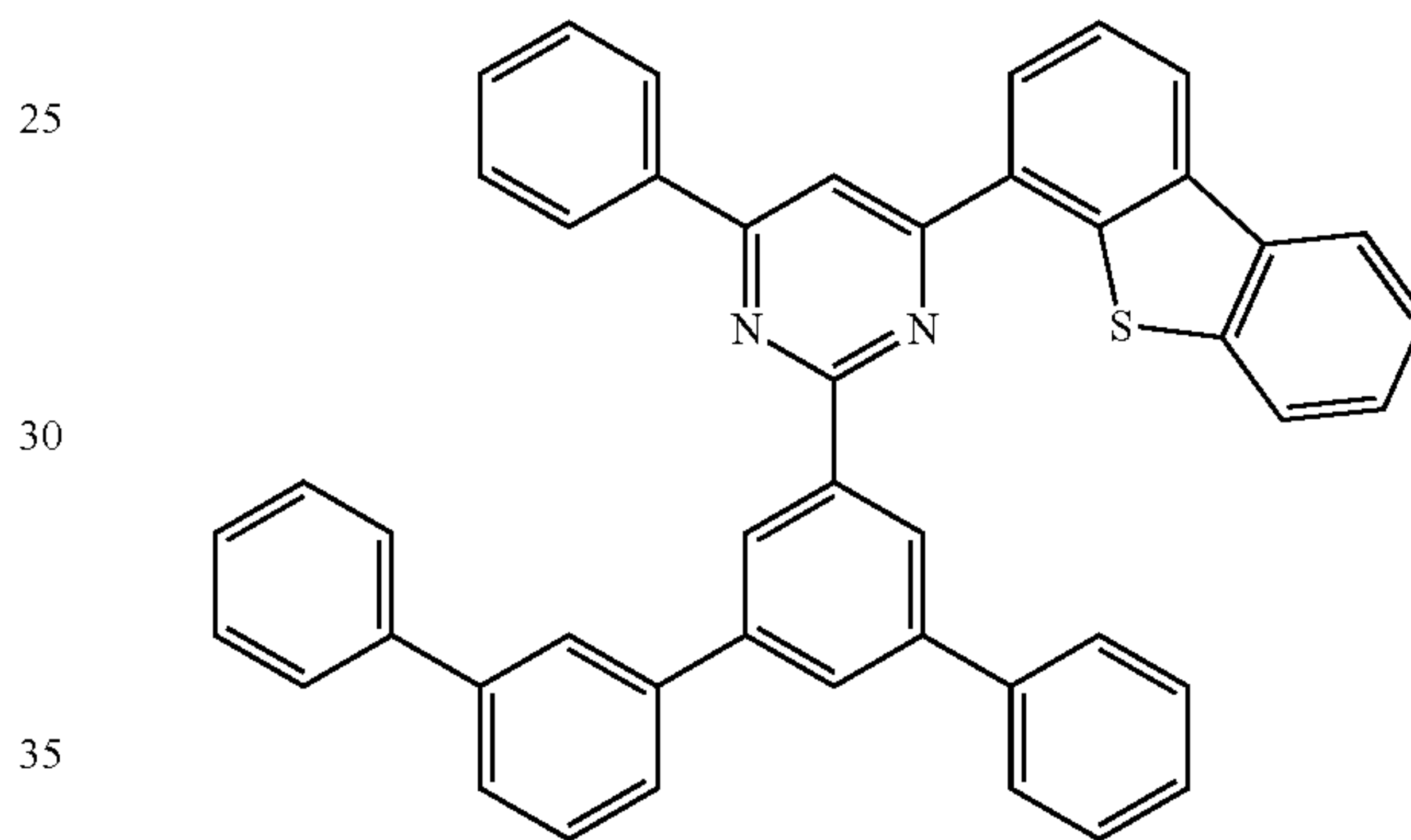
Compound B
