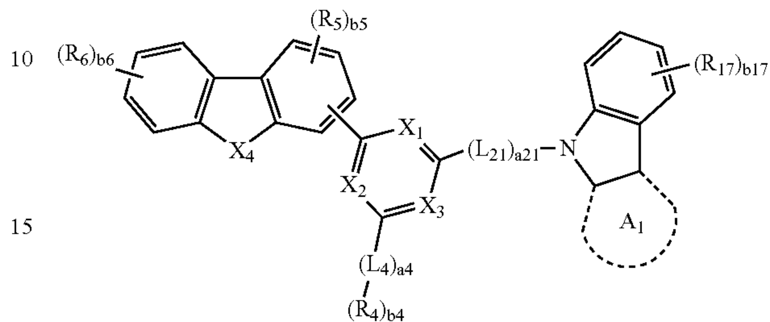
Formula 1B
