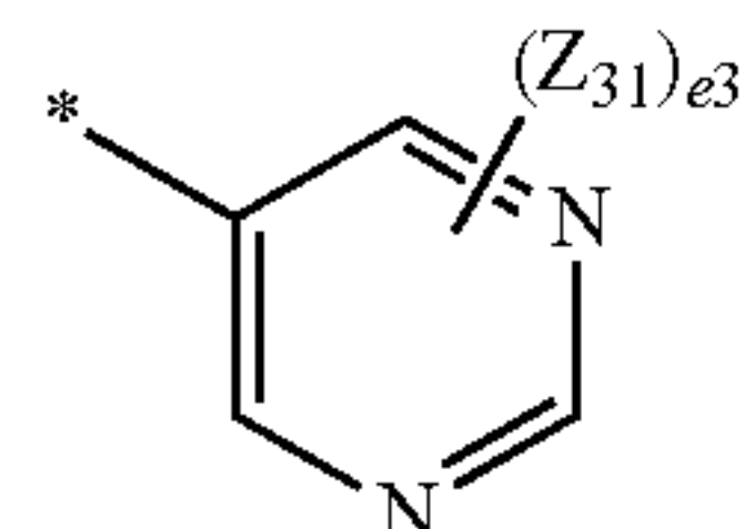
Formula 4-1 25
