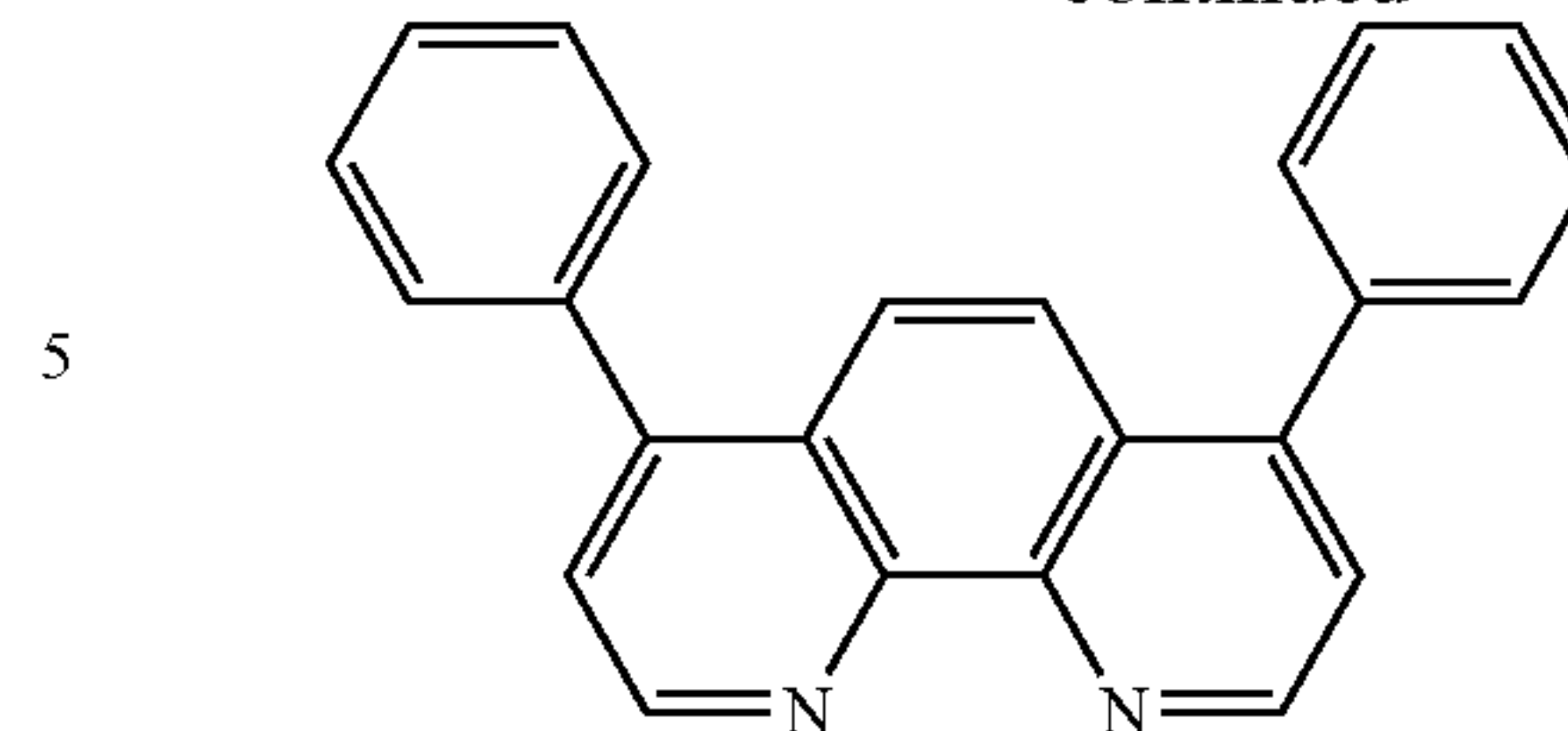
Bphen
