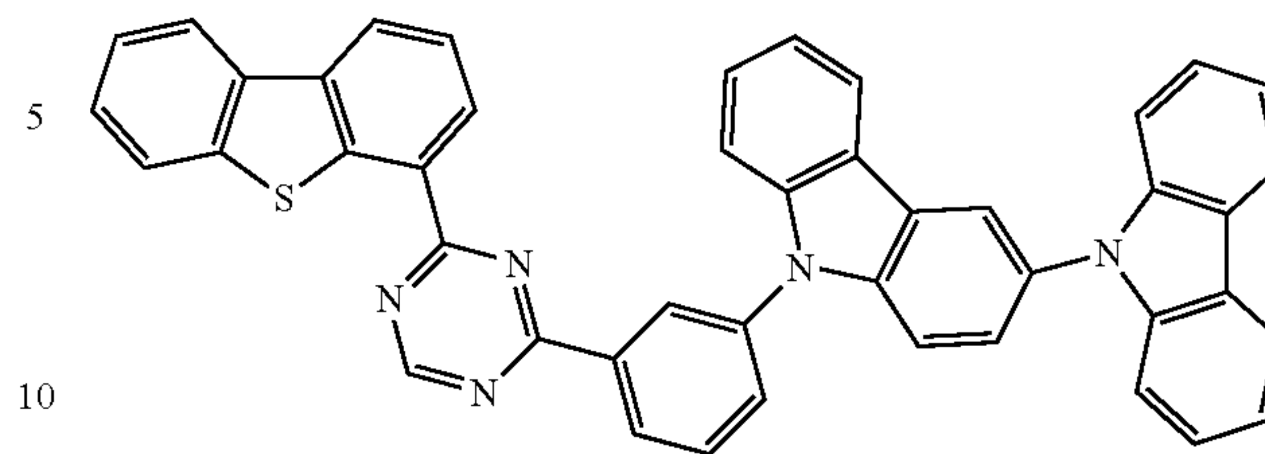
Compound A
