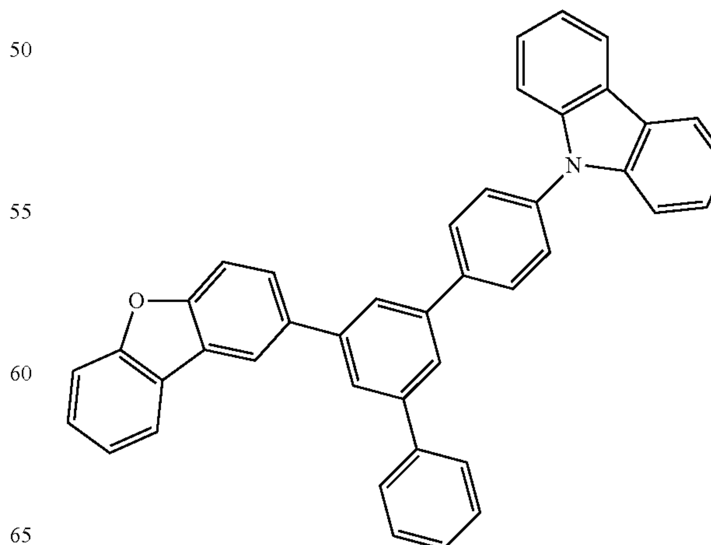
Compound C
