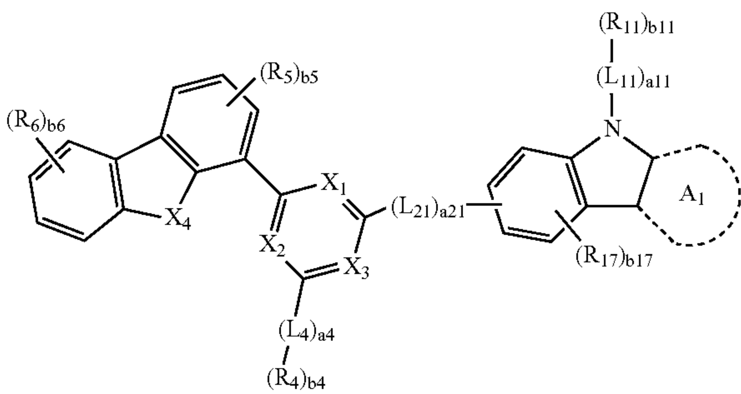
Formula 1B(1)
