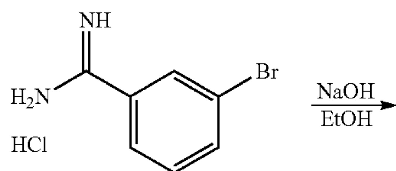
Molecular Weight: 235.51
