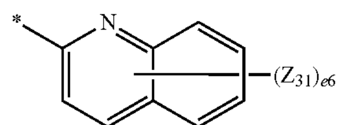
Formula 4-3 35
