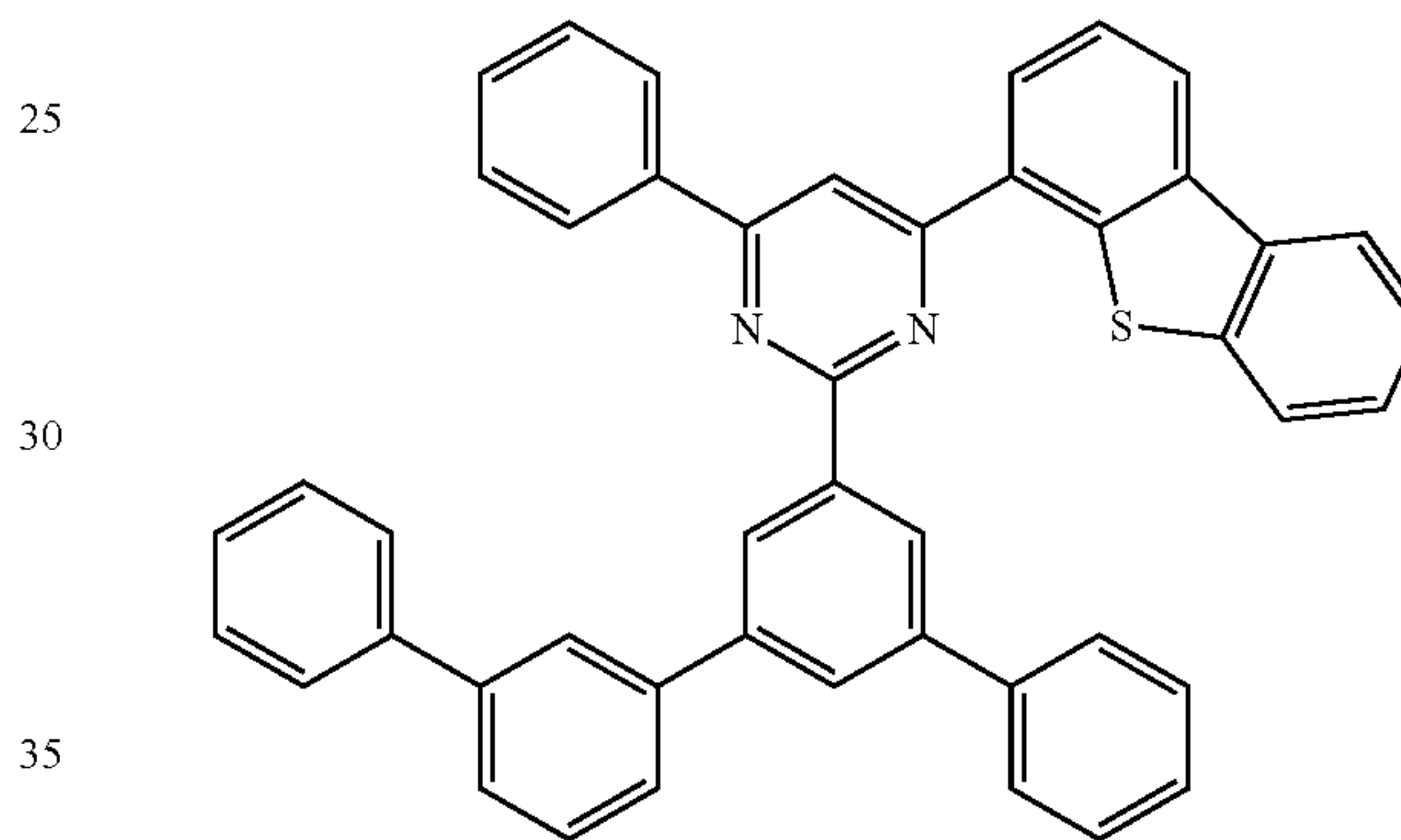
Compound B
