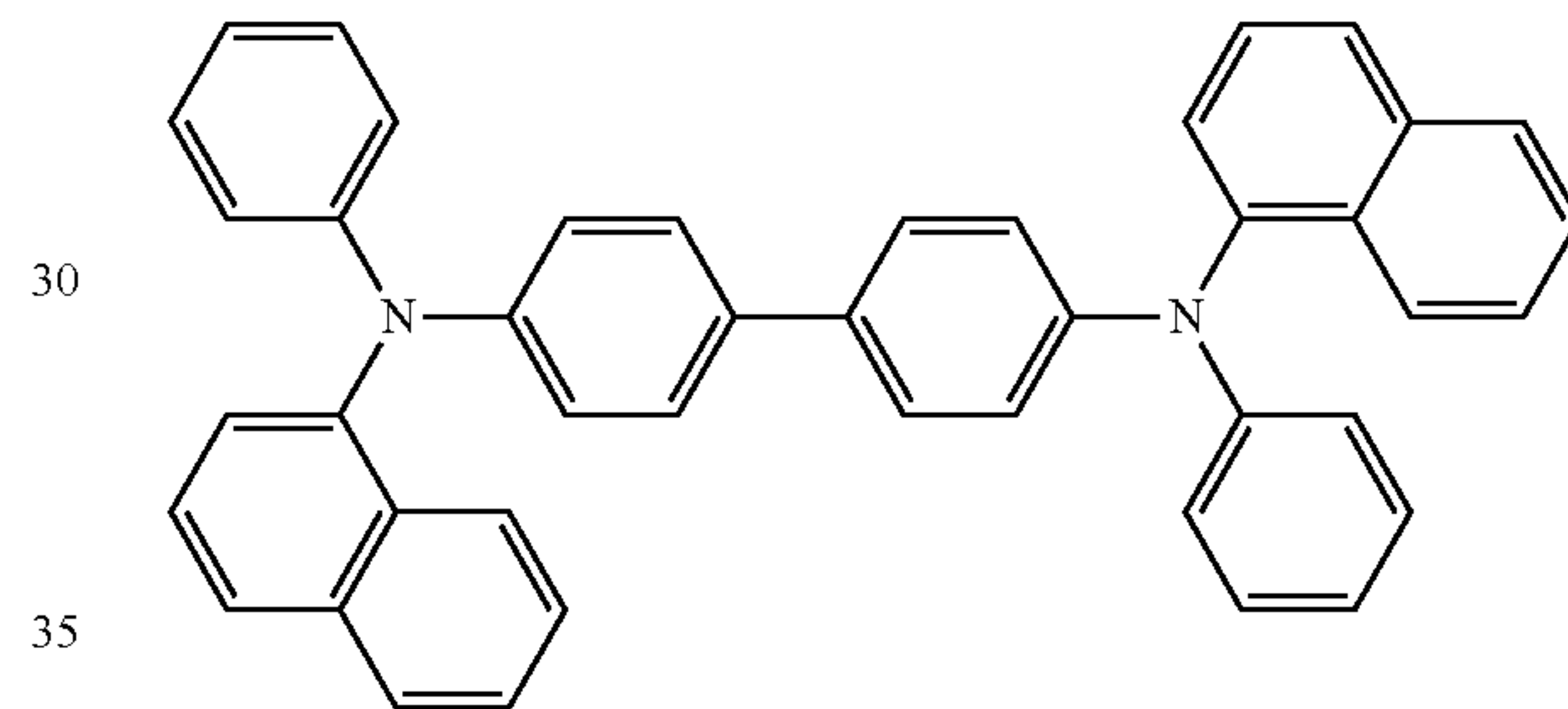
NPB
