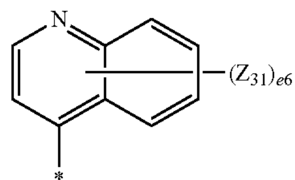
Formula 4-5 45
