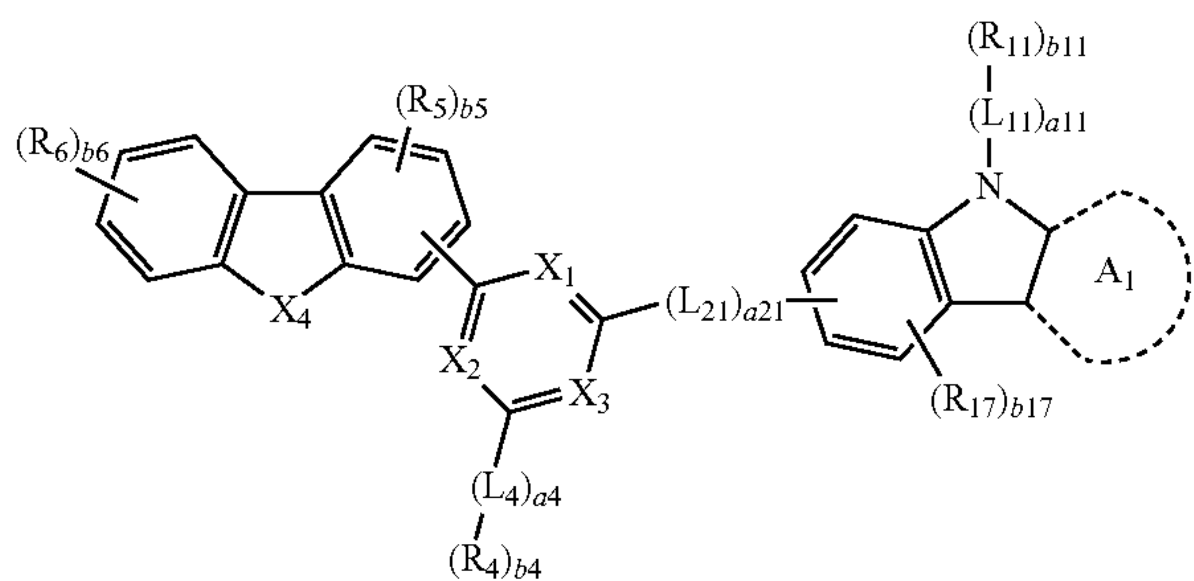
Formula 1B
