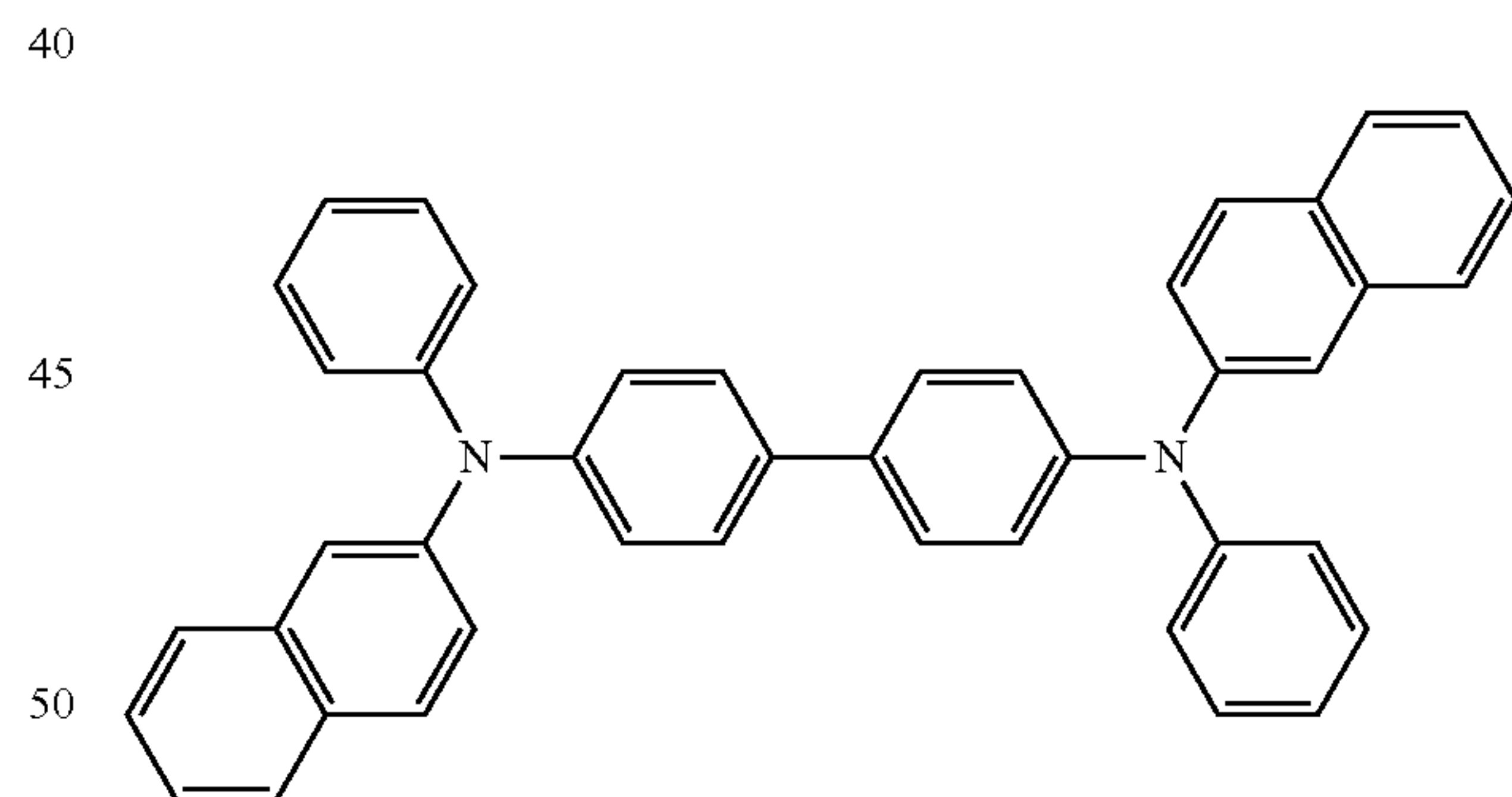
\beta -NPB
