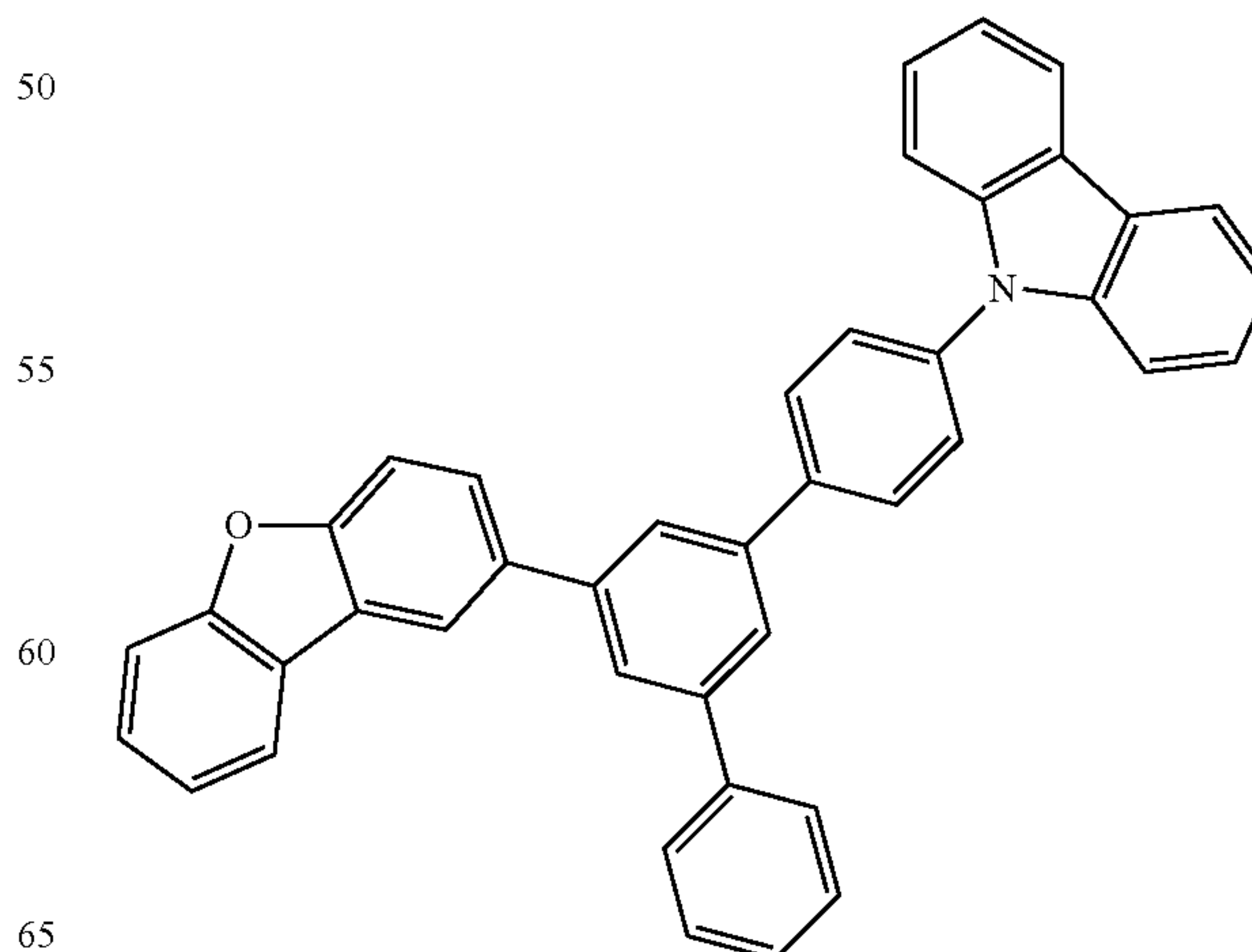
Compound C
