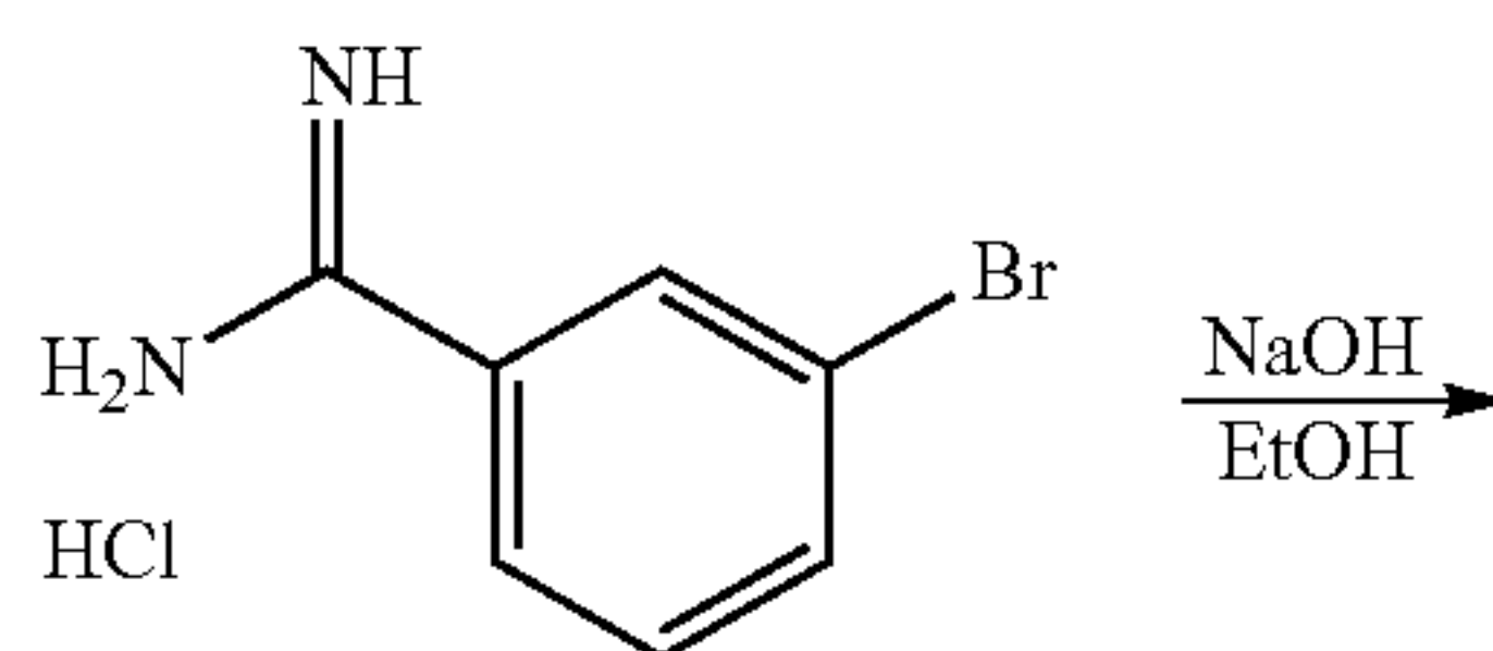
Molecular Weight: 235.51
