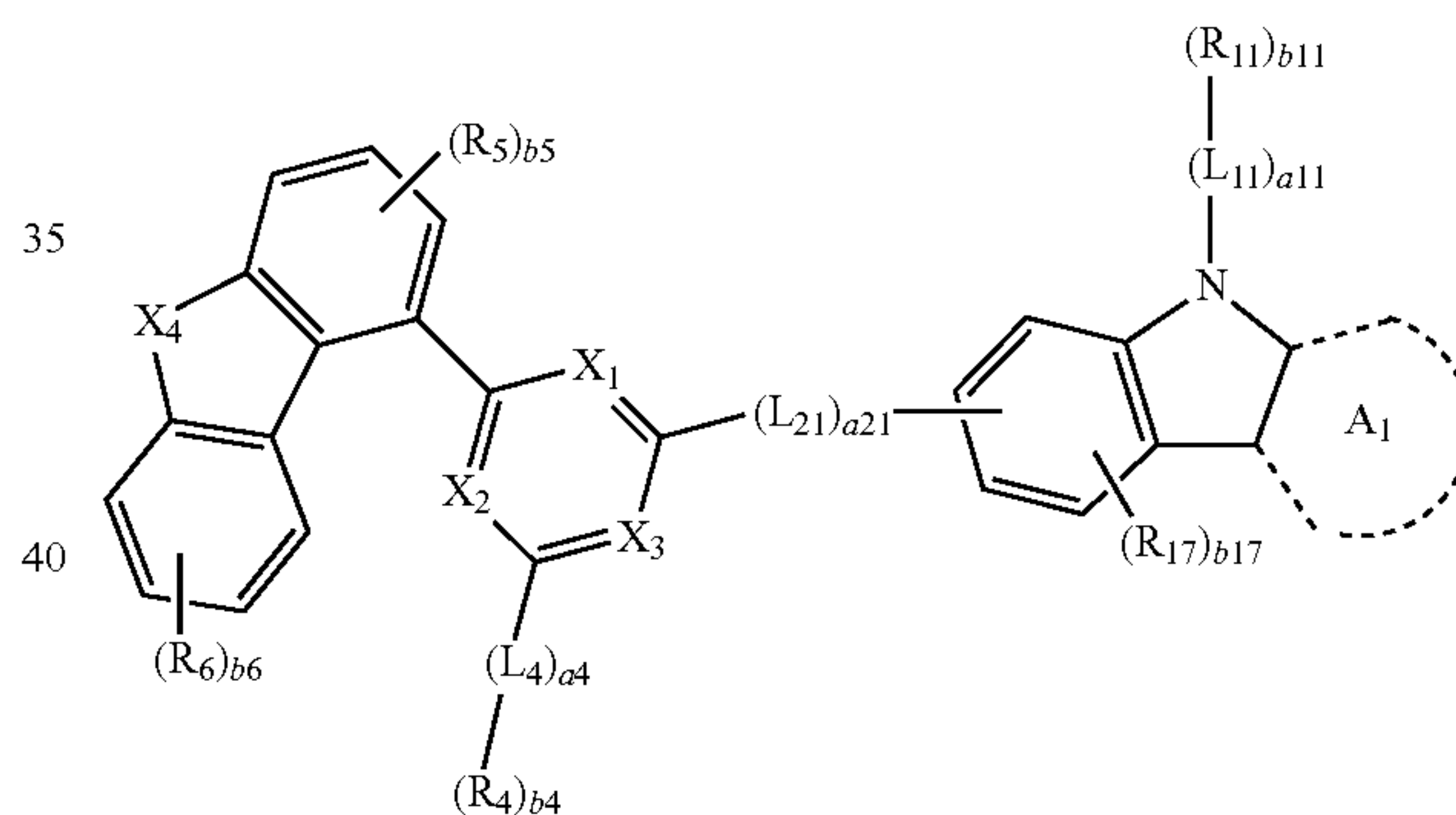
Formula 1B(4)
