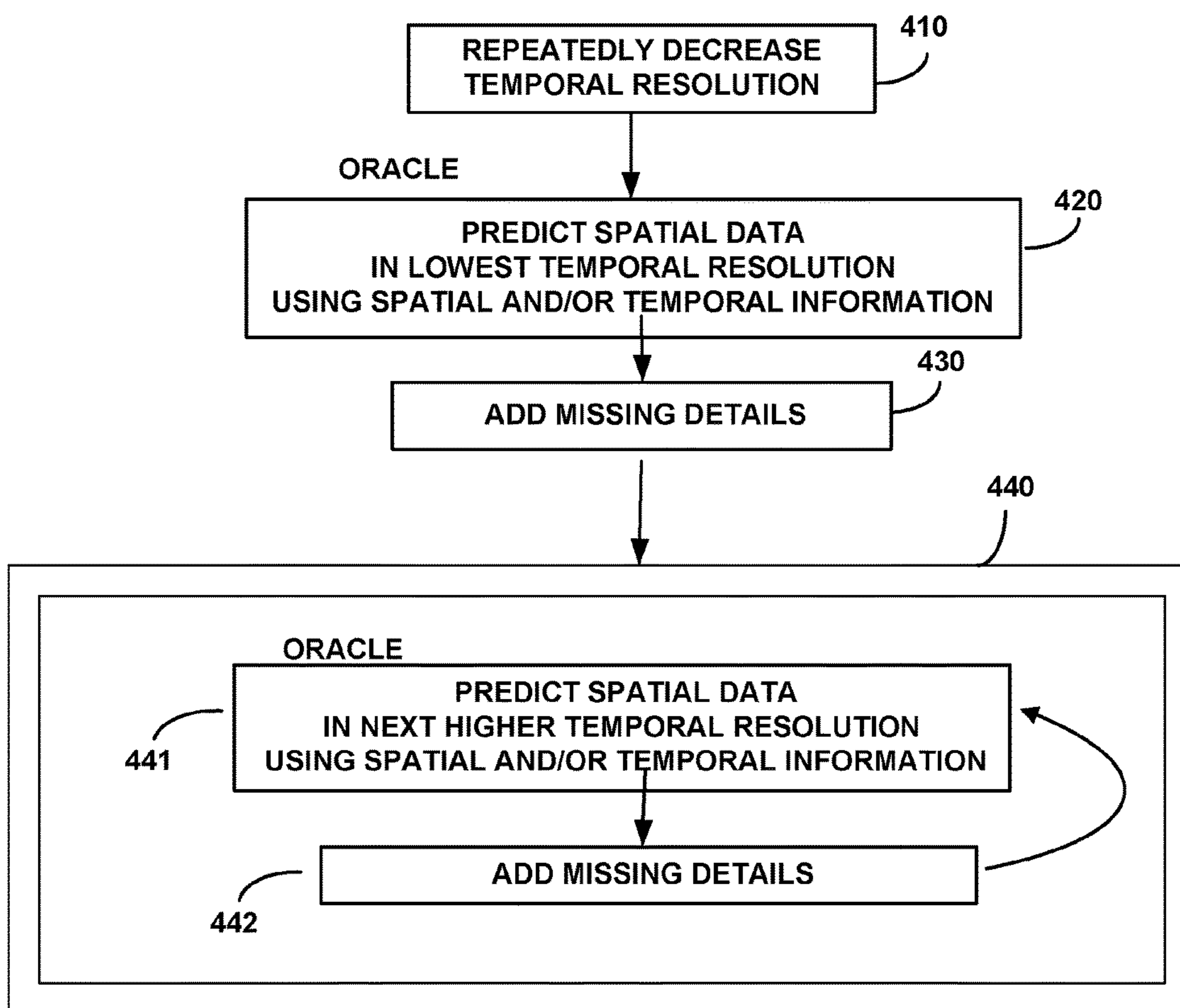
Fig. 4S – SPATIAL RESOLUTION INCREASE OF VIDEO
