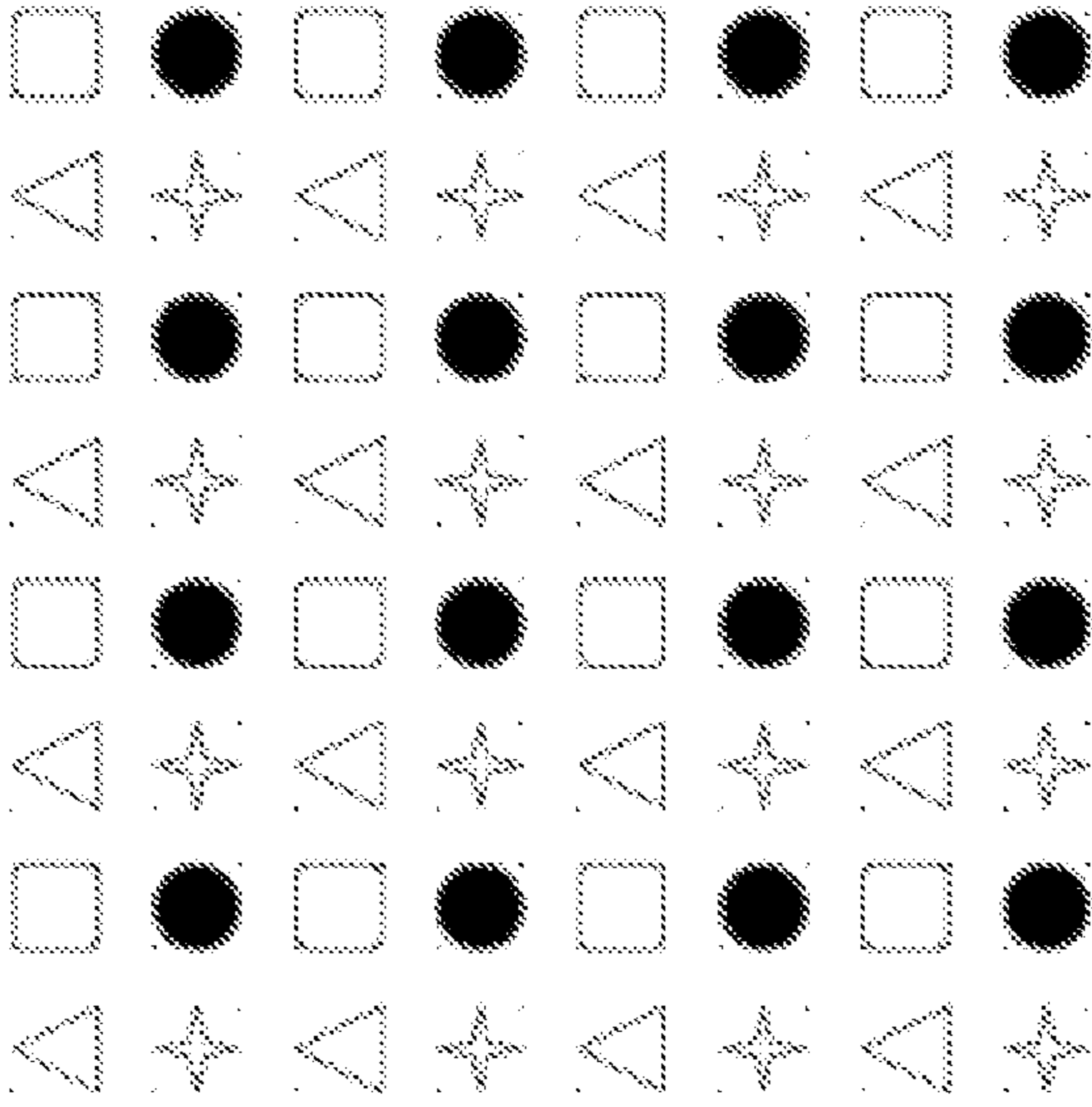
120 Dyadic sub-lattices
