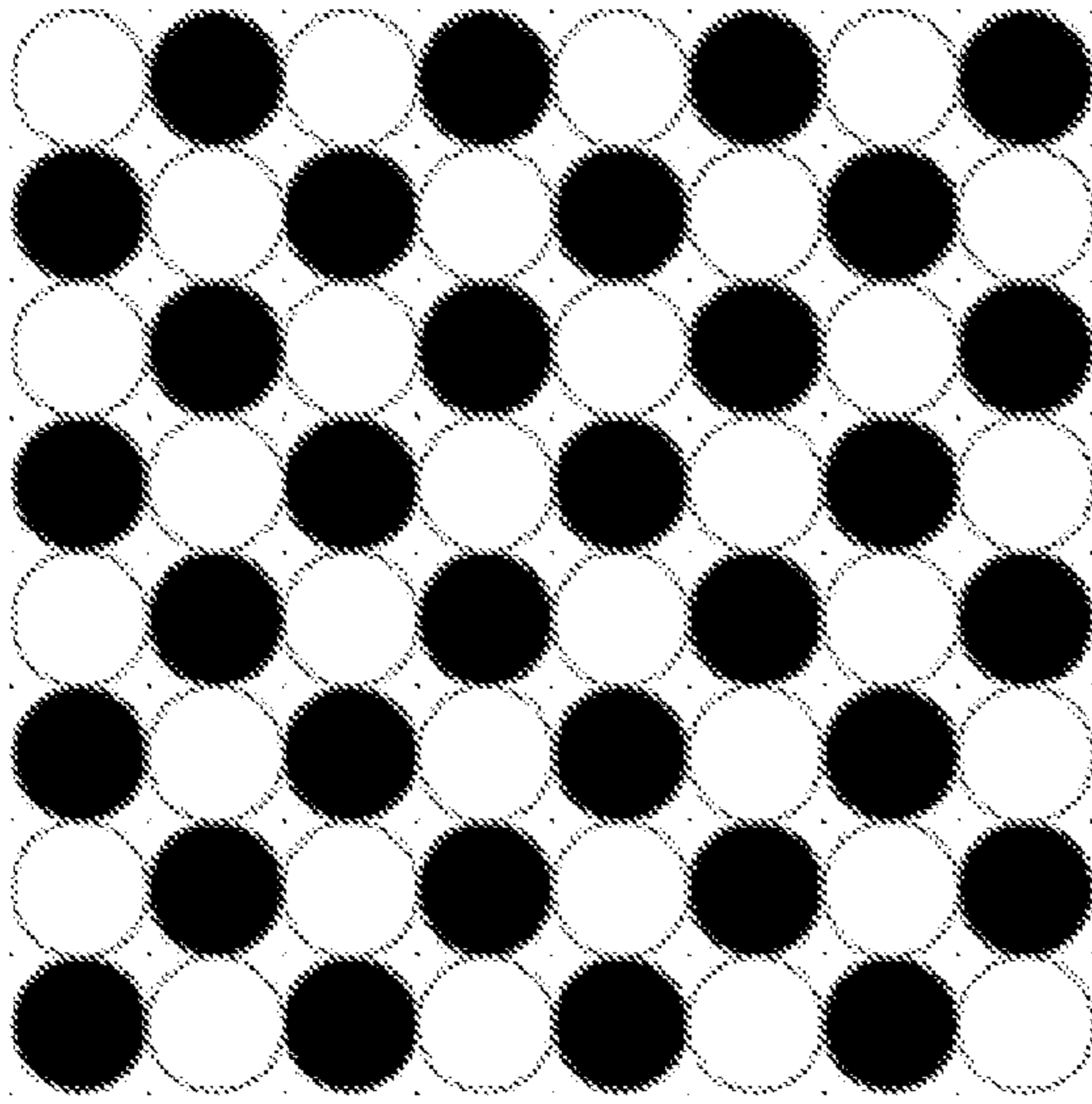
110 Quincunx sub-lattices
