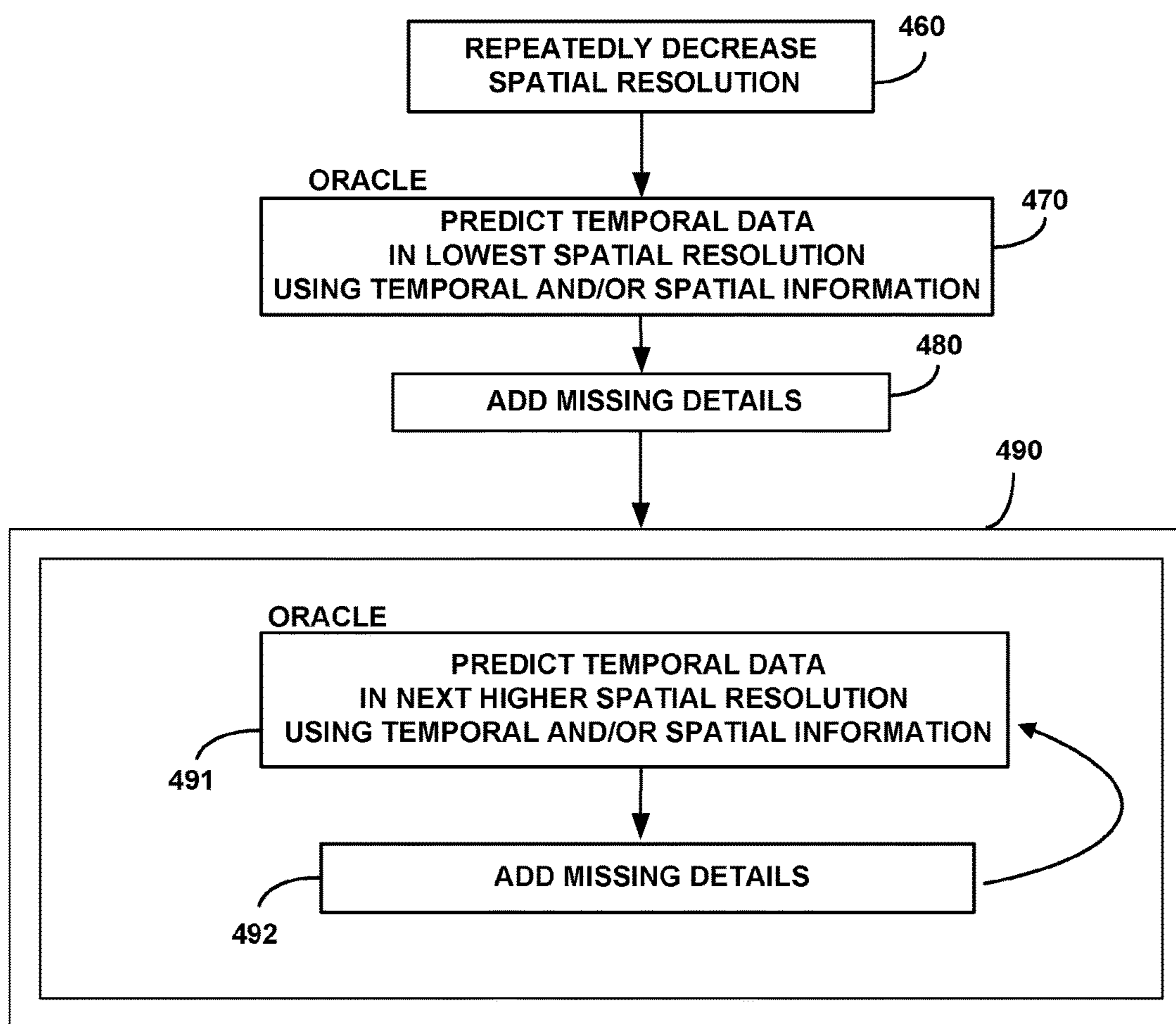
Fig. 4T – TEMPORAL RESOLUTION INCREASE OF VIDEO
