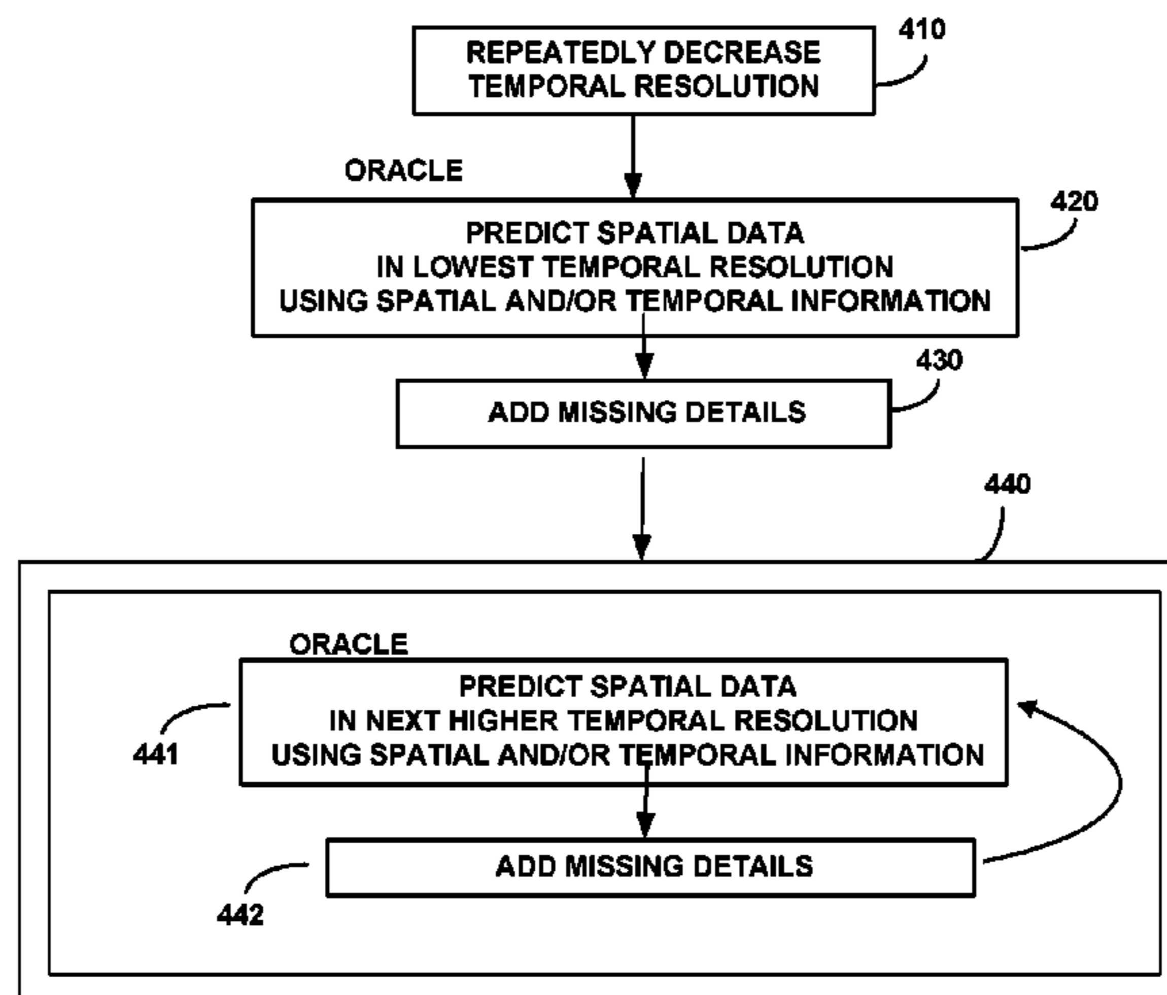
SPATIAL RESOLUTION INCREASE OF VIDEO
