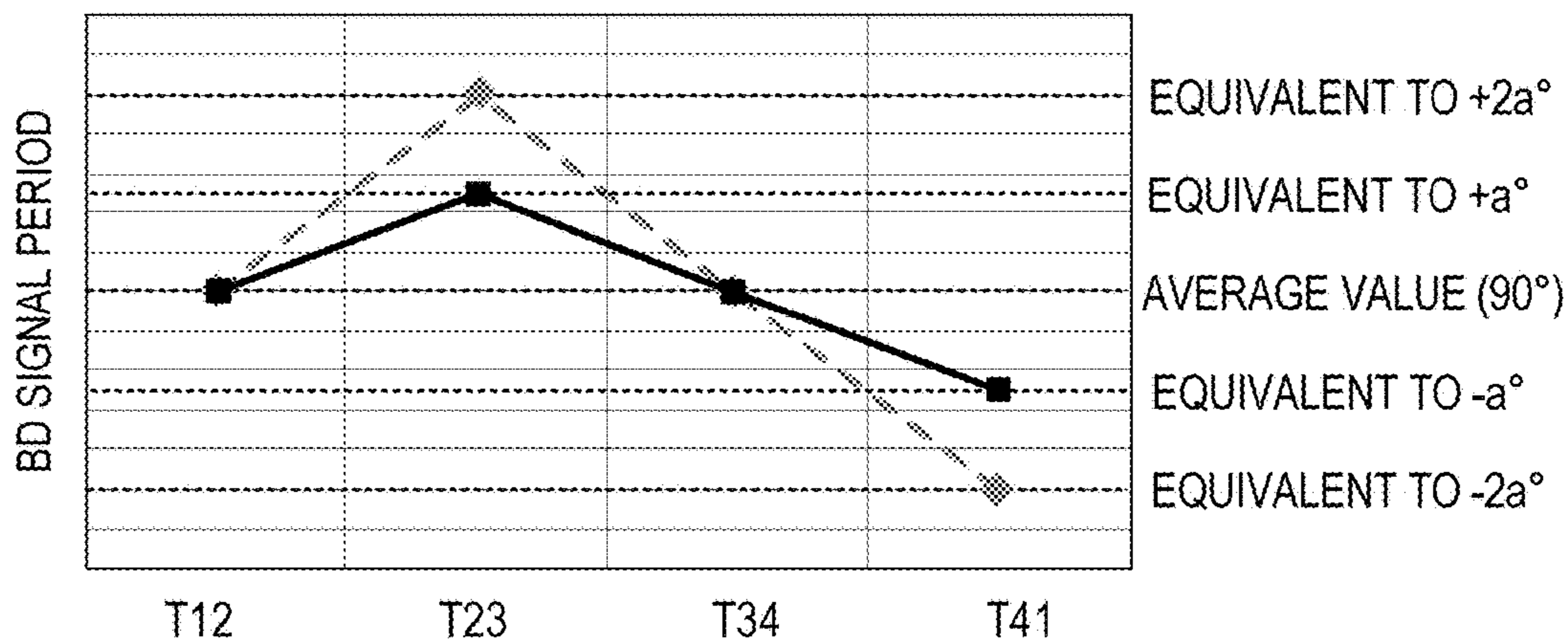
MANUFACTURING ERROR TOLERANCE OF DEFORMED ROTARY POLYGON MIRROR 113
