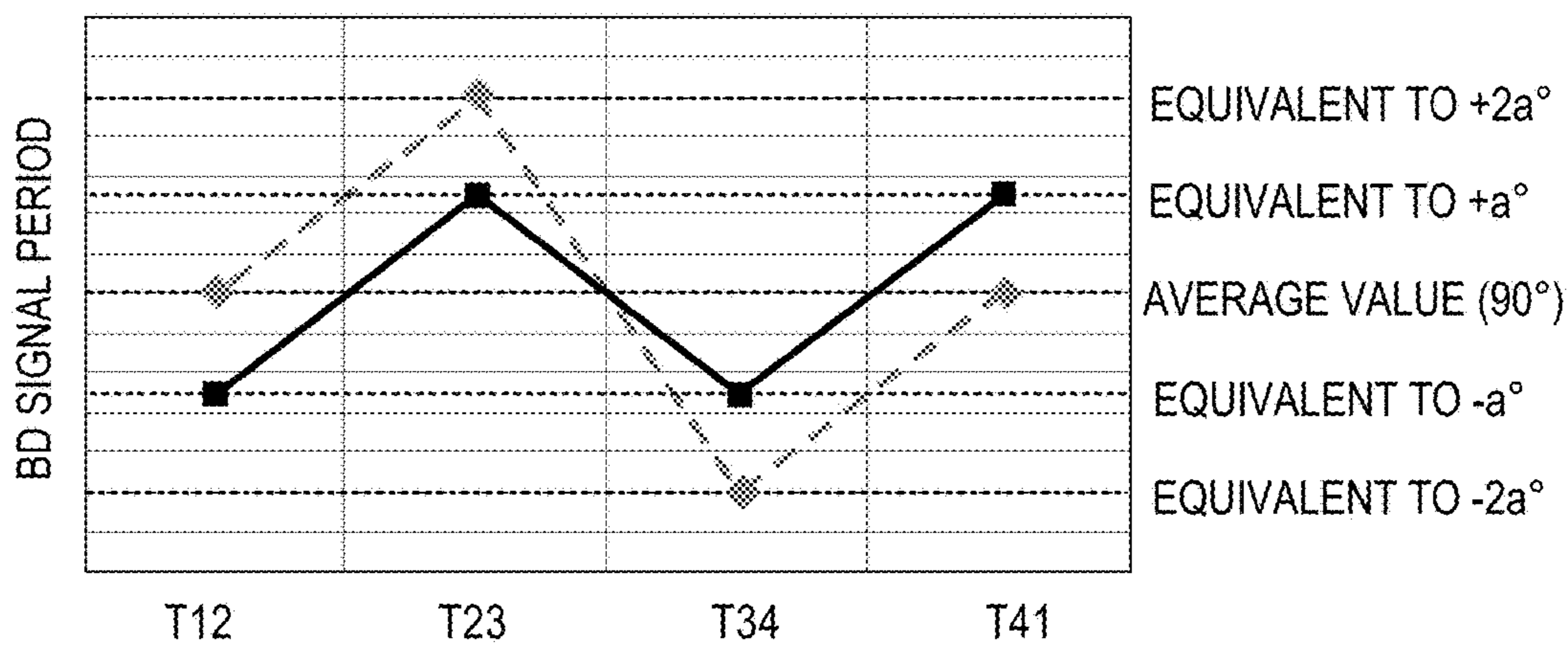
MANUFACTURING ERROR TOLERANCE OF TRAPEZOID ROTARY POLYGON MIRROR 114
