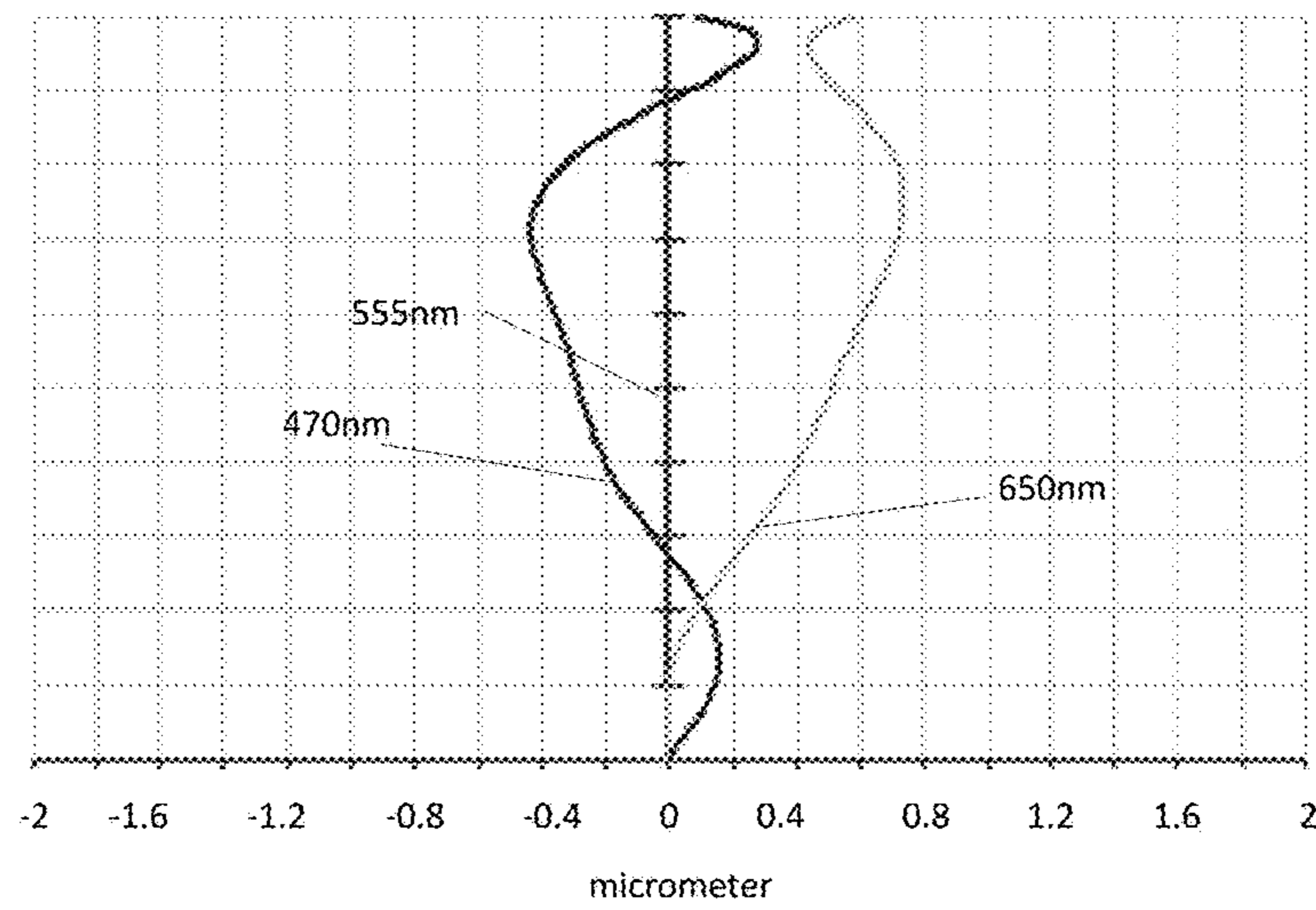
Lateral color
