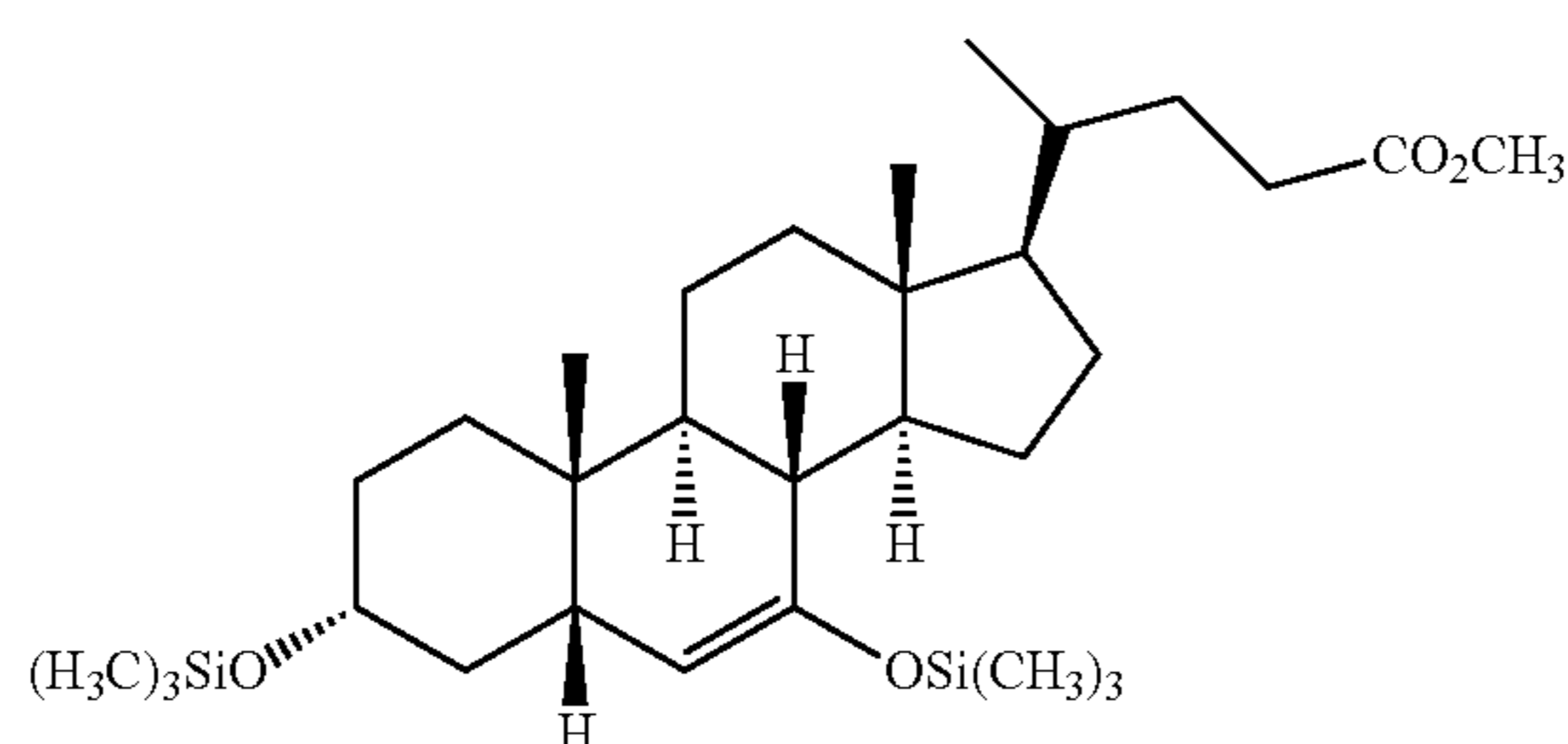
3 \alpha ,7-ditrimethylsilyloxy-5 \beta -chol-6-en-24-oic acid methyl ester
