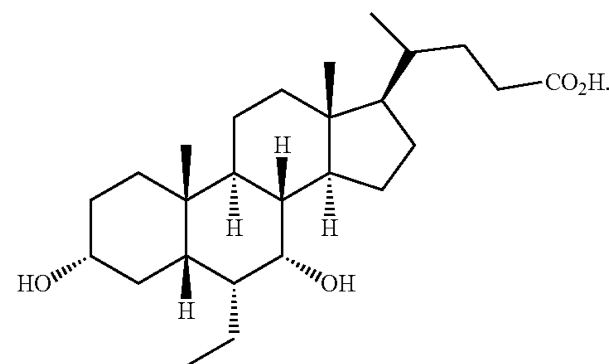
obeticholic acid (also known as INT-747)
