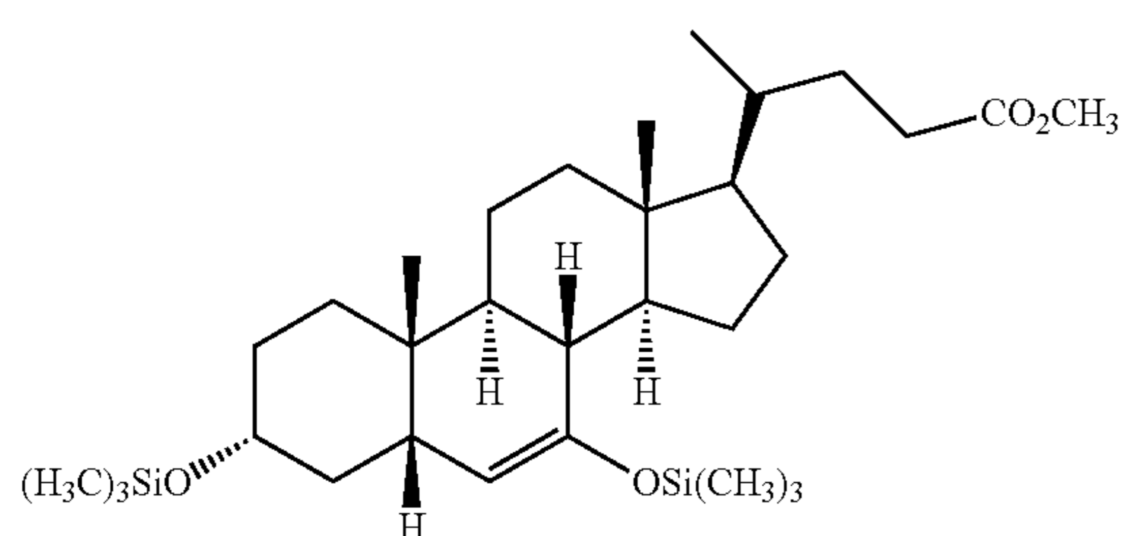
3 \alpha ,7-ditrimethylsilyloxy-5 \beta -chol-6-en-24-oic acid methyl ester
