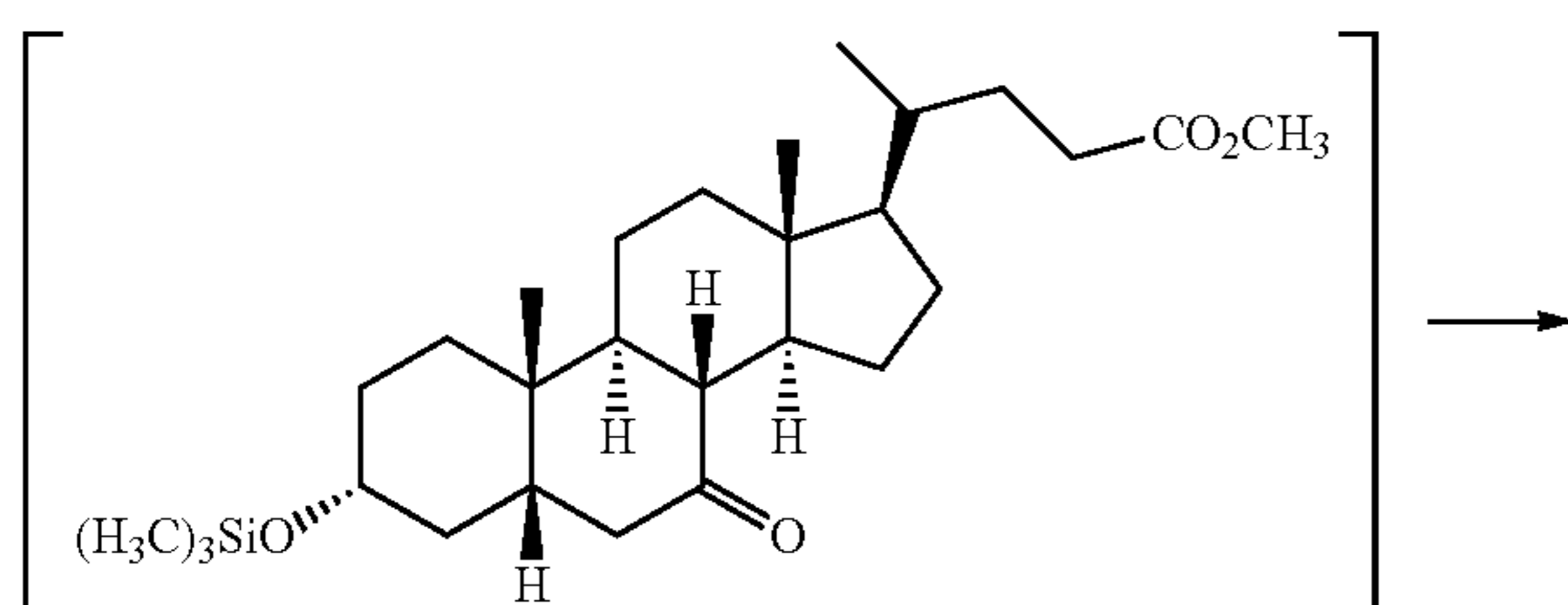
3 \alpha -trimethylsilyloxy-7-keto-5 \beta -cholan-24-oic acid methyl ester 2 (not isolated)
