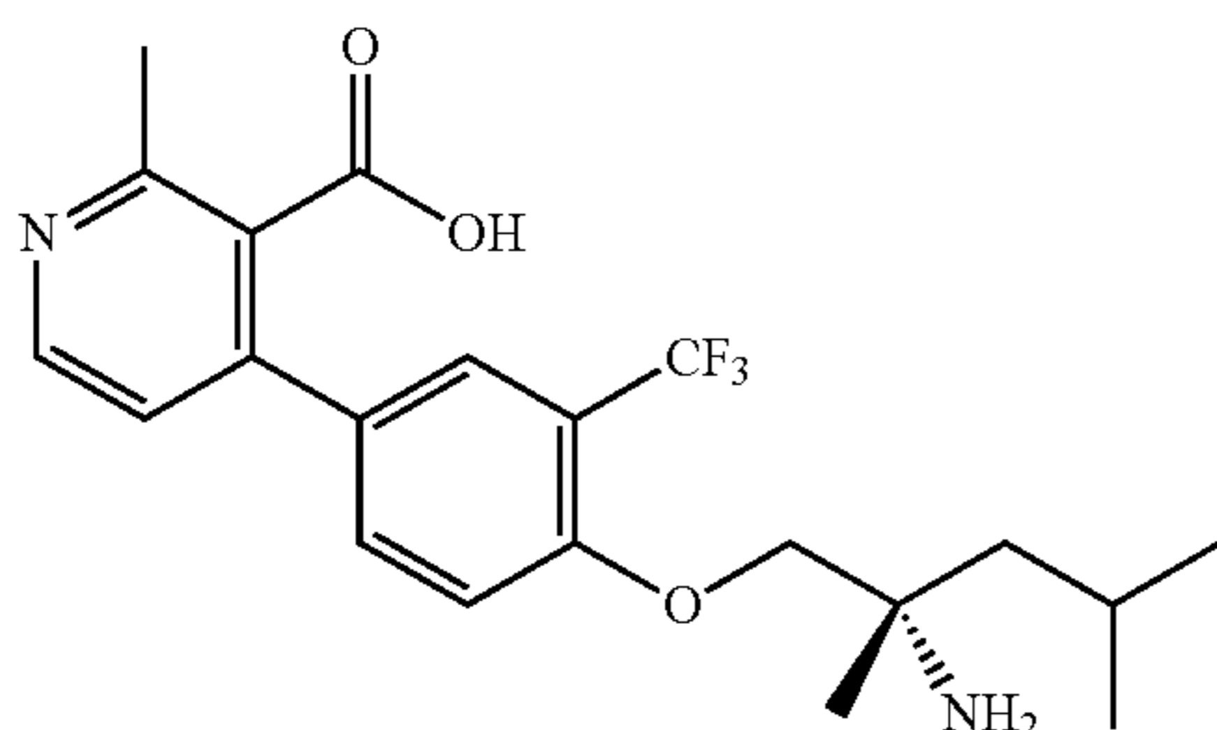
Part B: (S)-4-(4-((2-amino-2,4-dimethylpentyl)oxy)-3-(trifluoromethyl)phenyl)-2-methylnicotinic acid
