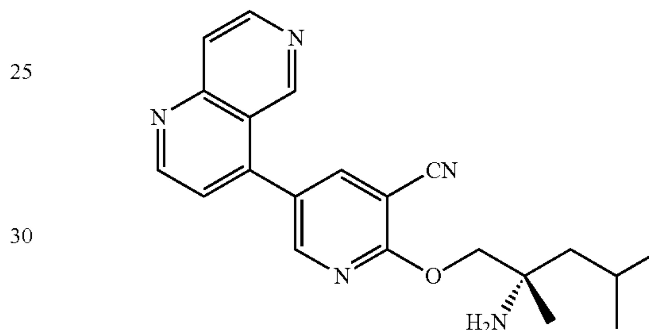
Part B: (S)-2-((2-amino-2,4-dimethylpentyl)oxy)-5-(1,6-naphthyridin-4-yl)nicotinonitrile
