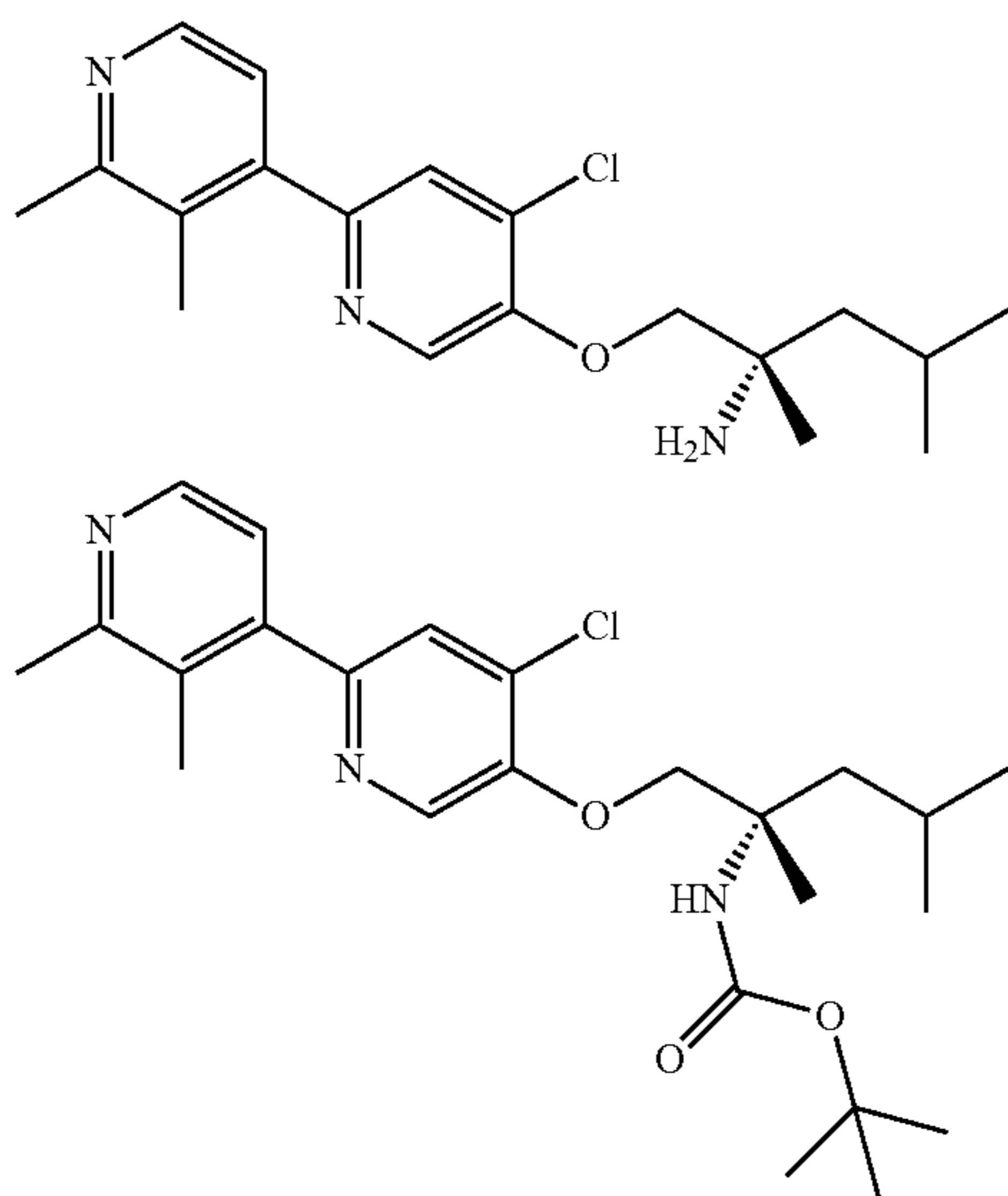
Part A: (S)-tert-butyl (1-((4-chloro-2',3'-dimethyl-[2,4'-bipyridin]-5-yl)oxy)-2,4-dimethylpentan-2-yl) carbamate
