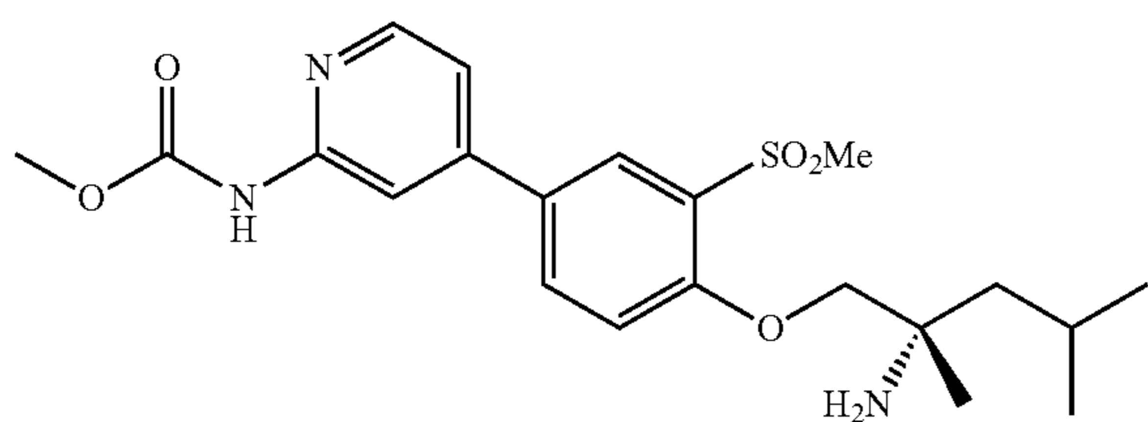
Part B: (S)-methyl(4-(4-((2-amino-2,4-dimethylpentyl)oxy)-3-(methylsulfonyl)phenyl)pyridin-2-yl)carbamate
