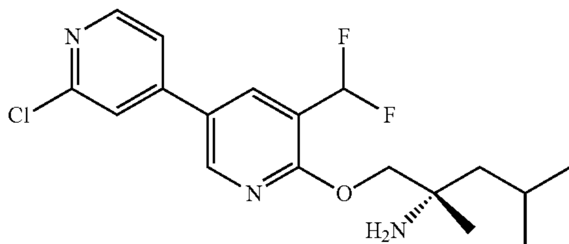
Part C: (S)-1-((2'-chloro-5-(difluoromethyl)-[3,4'-bipyridin]-6-yl)oxy)-2,4-dimethylpentan-2-amine
