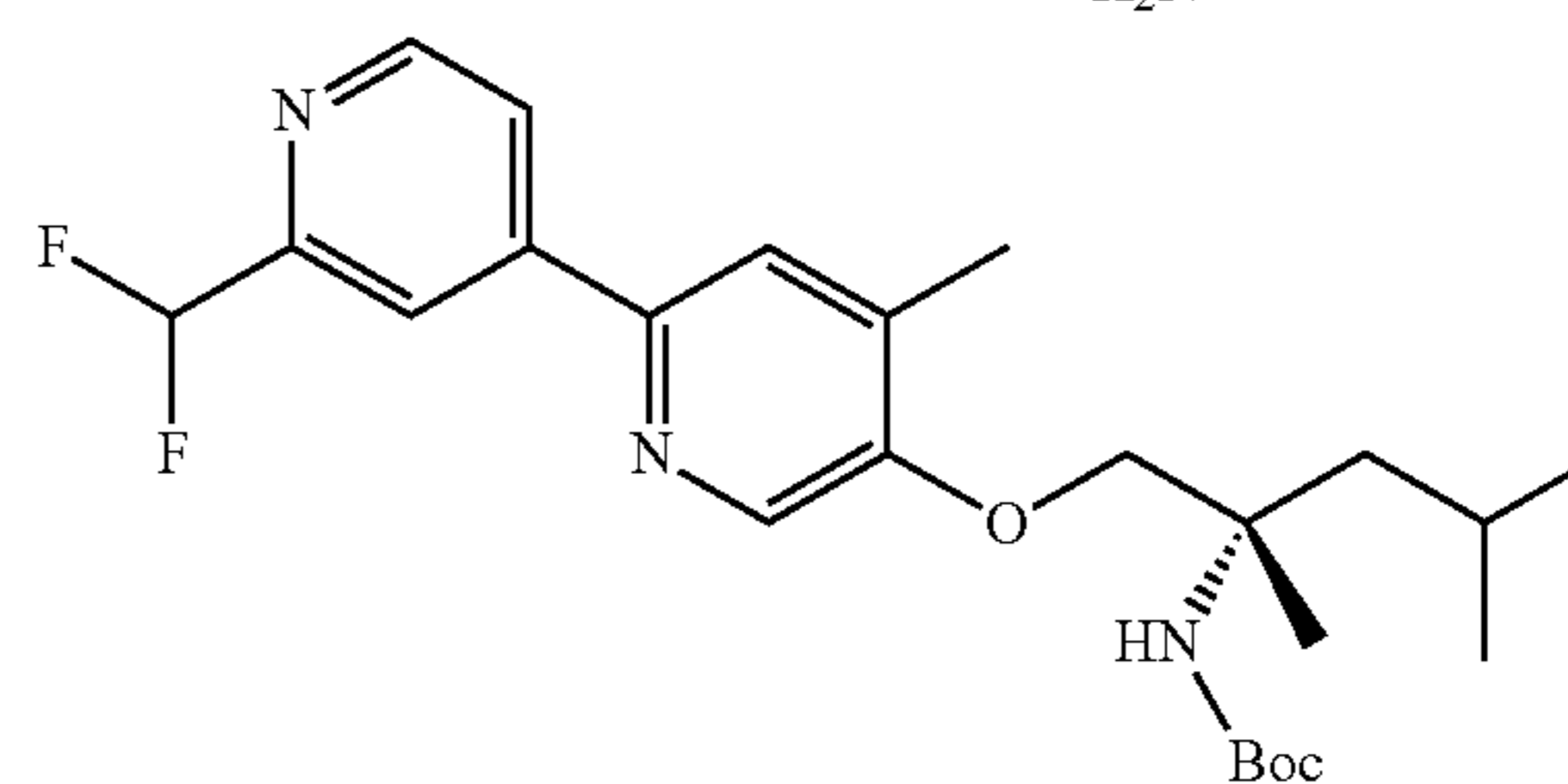
Part A: (S)-tert-butyl (1-((2'-(difluoromethyl)-4-methyl-[2,4'-bipyridin]-5-yl)oxy)-2,4-dimethylpentan-2-yl)carbamate
