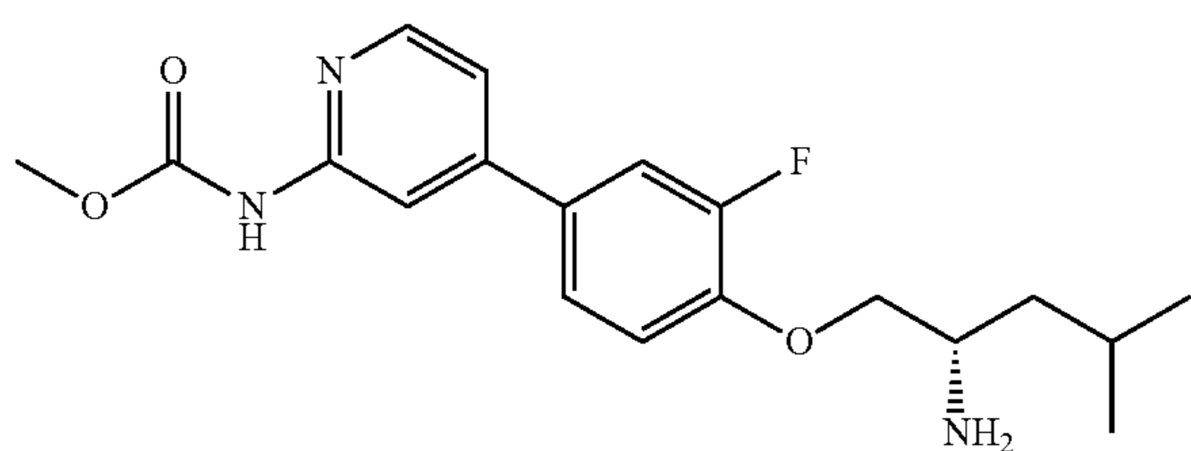
Part C: (S)-methyl (4-(4-((2-amino-4-methylpentyl)oxy)-3-fluorophenyl)pyridin-2-yl)carbamate
