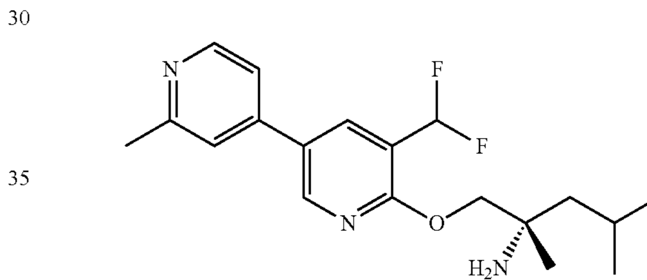
(S)-1-((5-(difluoromethyl)-2'-methyl-[3,4'-bipyridin]-6-yl)oxy)-2,4-dimethylpentan-2-amine
