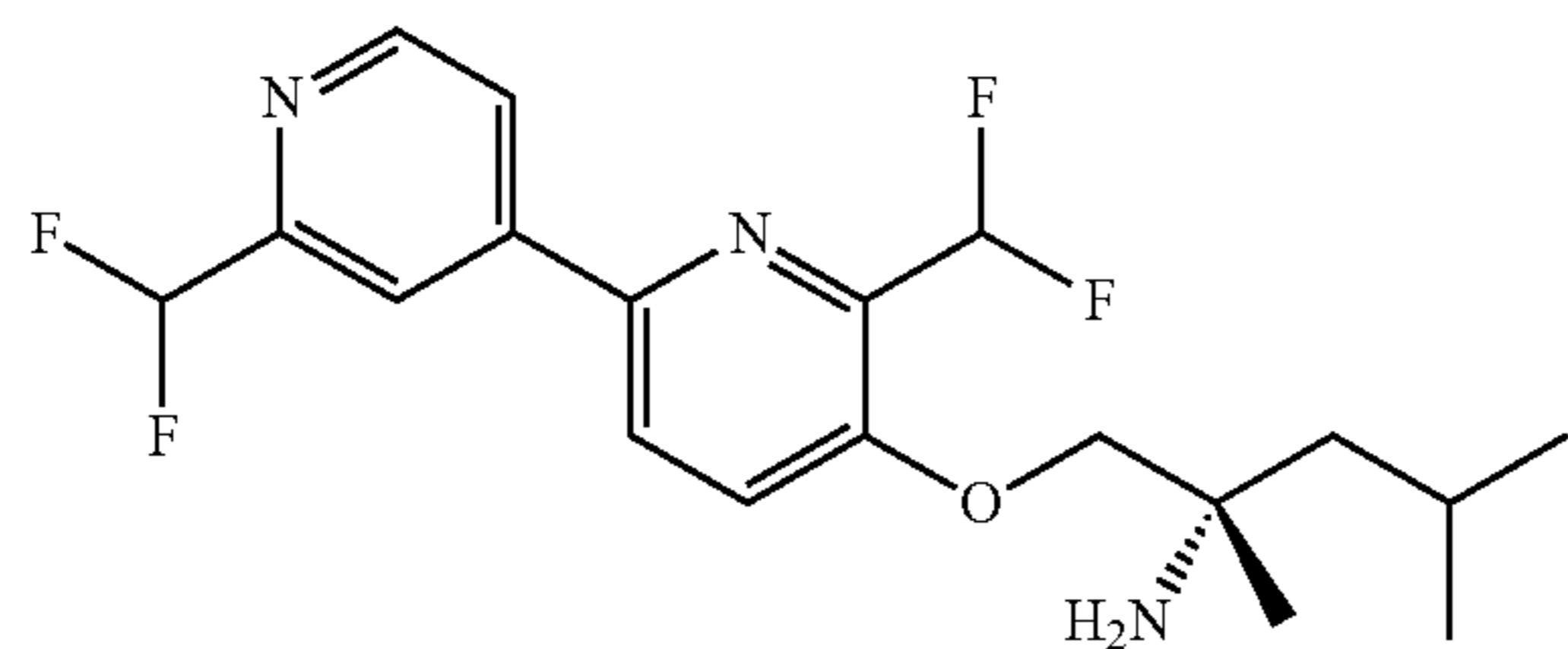
Part B: (S)-1-((2',6-bis(difluoromethyl)-[2,4'-bipyridin]-5-yl)oxy)-2,4-dimethylpentan-2-amine
