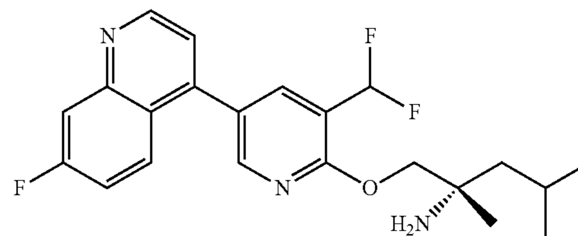
Part A: (S)-1-((3-(difluoromethyl)-5-(7-fluoroquinolin-4-yl)pyridin-2-yl)oxy)-2,4-dimethylpentan-2-amine
