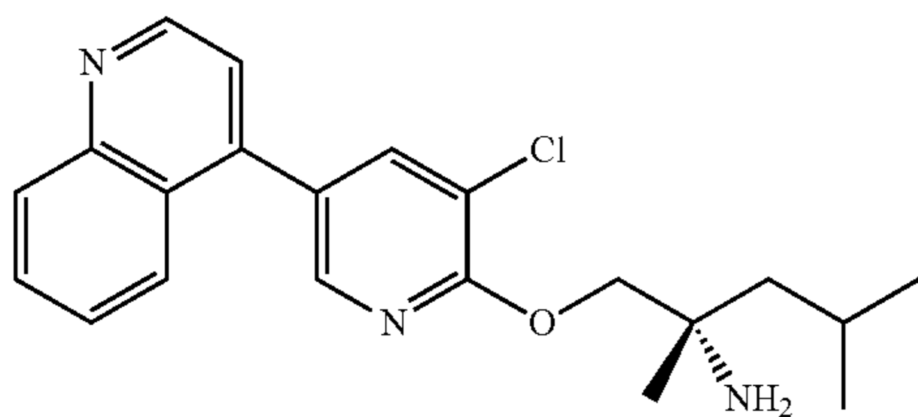
Part B: (S)-1-((3-chloro-5-(quinolin-4-yl)pyridin-2-yl)oxy)-2,4-dimethylpentan-2-amine
