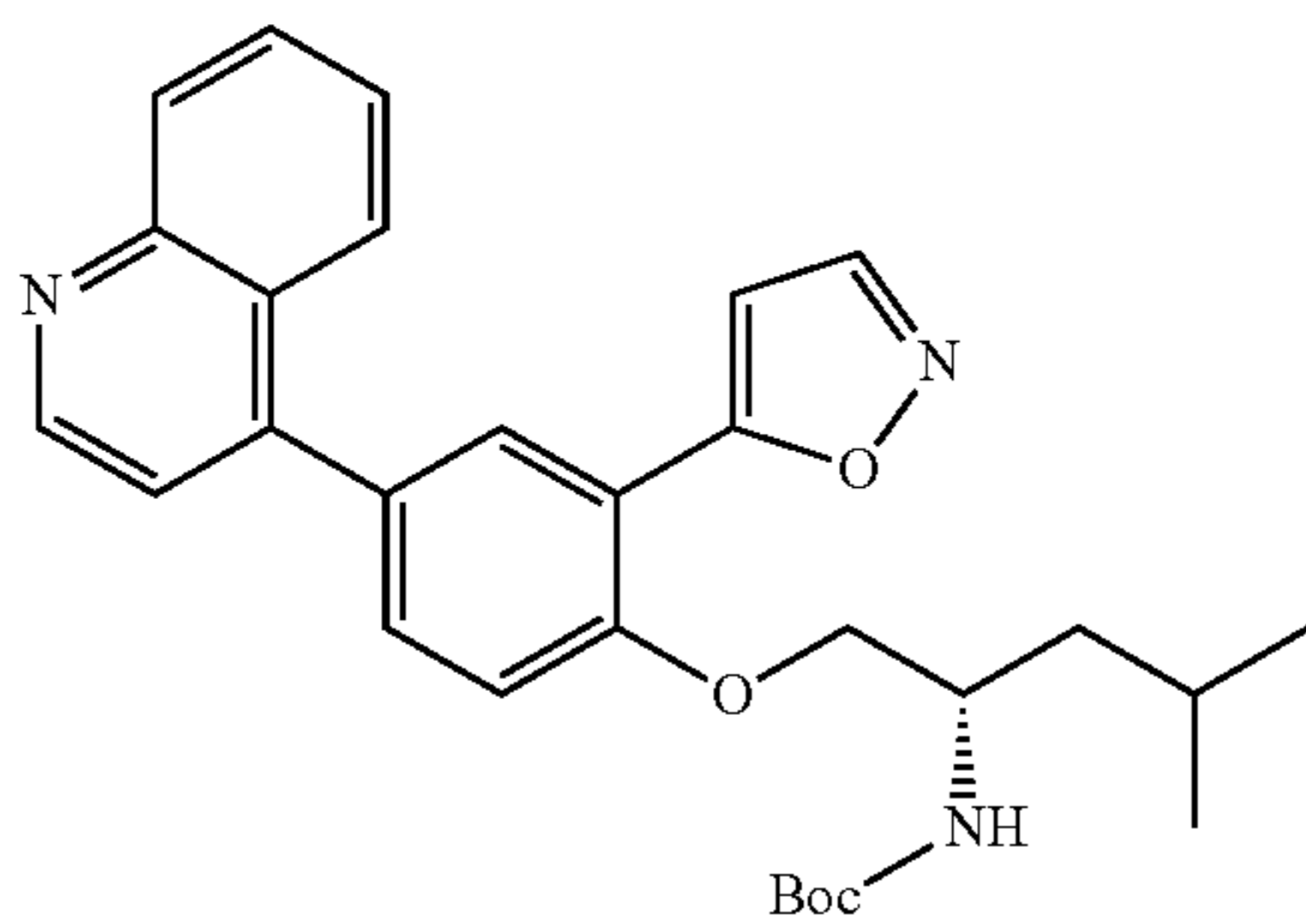
Part B: (S)-tert-butyl (1-(2-(isoxazol-5-yl)-4-(quinolin-4-yl)phenoxy)-4-methylpentan-2-yl)carbamate
