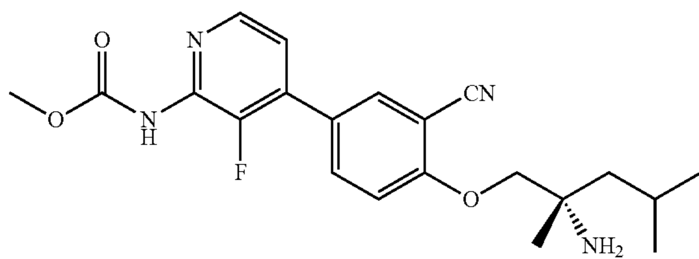
Part E: (S)-methyl (4-(4-((2-amino-2,4-dimethylpentyl)oxy)-3-cyanophenyl)-3-fluoropyridin-2-yl)carbamate
