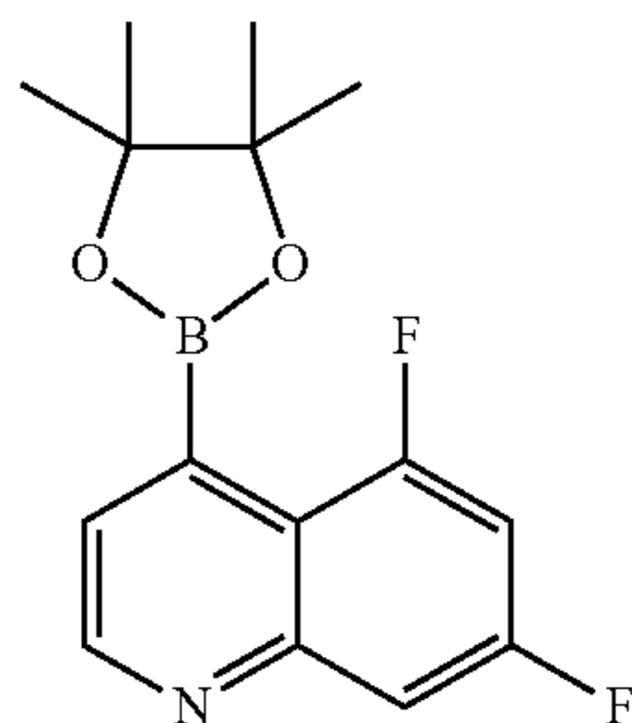
Part C: 5,7-difluoro-4-(4,4,5,5-tetramethyl-1,3,2-dioxaborolan-2-yl)quinoline
