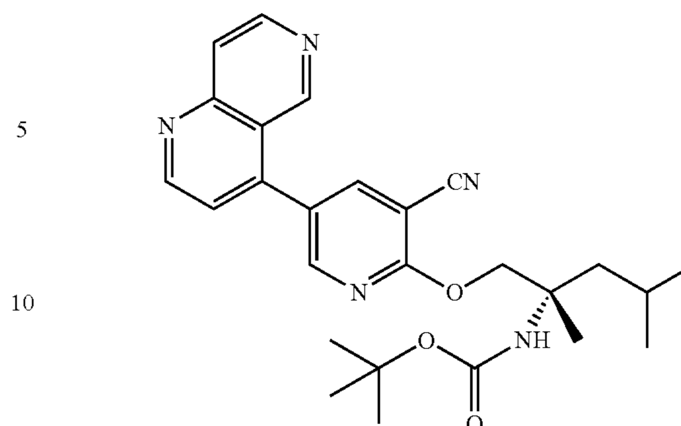
Part A: (S)-tert-butyl (1-((3-cyano-5-(1,6-naphthyridin-4-yl)pyridin-2-yl)oxy)-2,4-dimethylpentan-2-yl)carbamate
