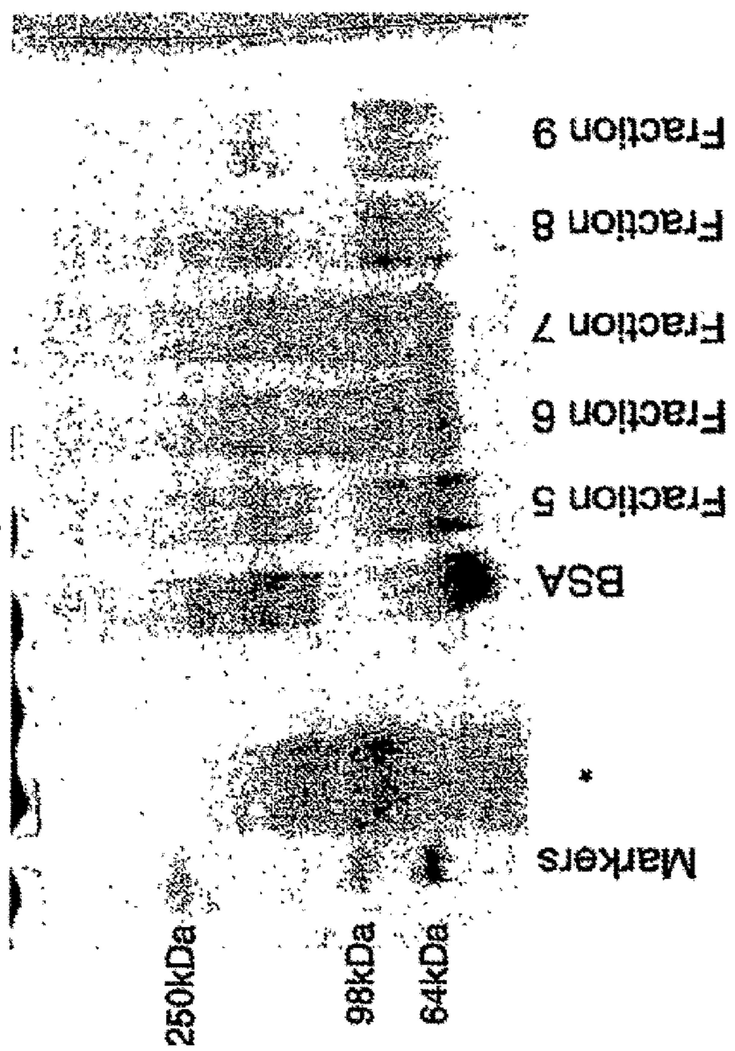
Figure 15 SDS-PAGE analysis of the CAH-NHS reactions
