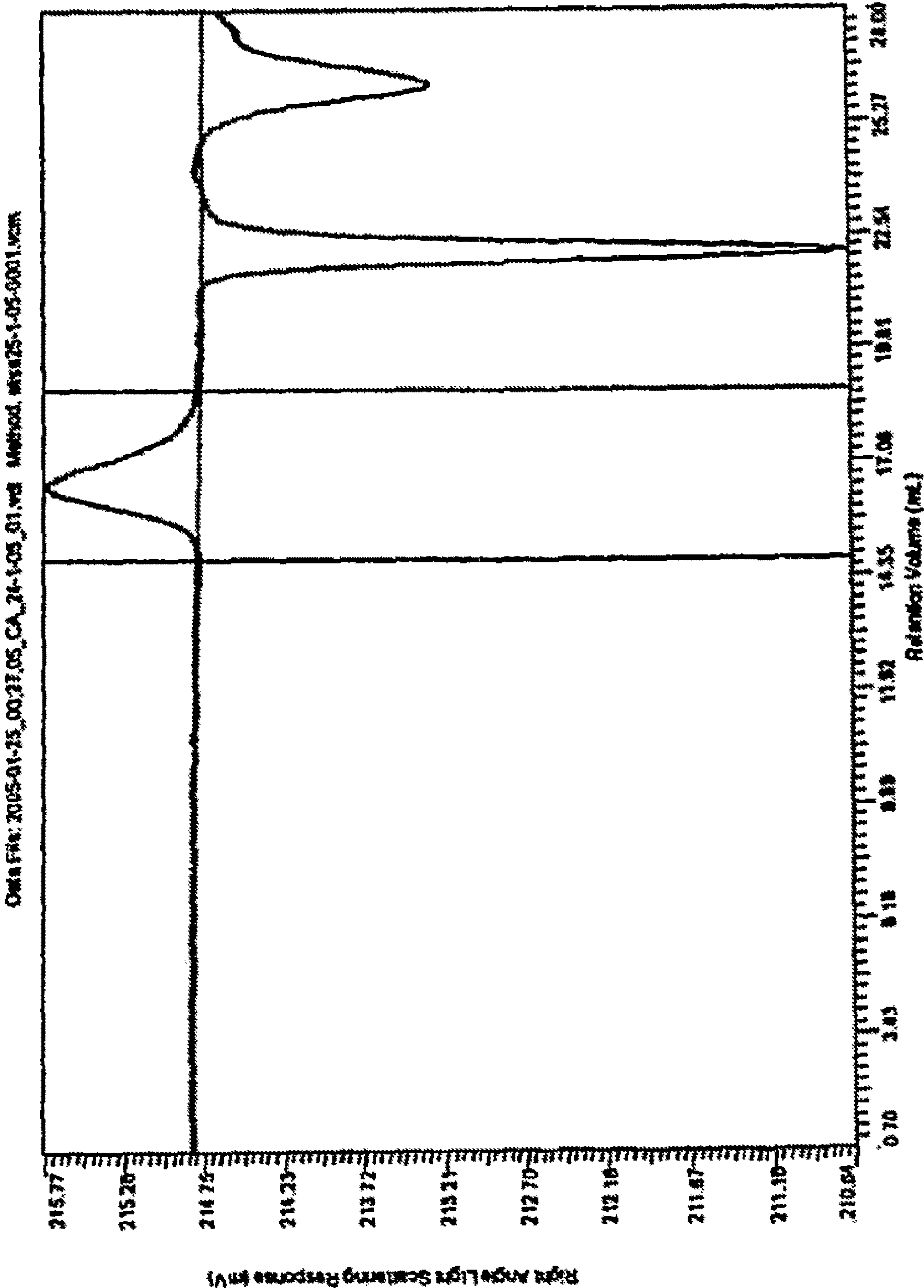
Figure 11a: RI scan on GPC of unreacted 35kDa CA-NH 2
