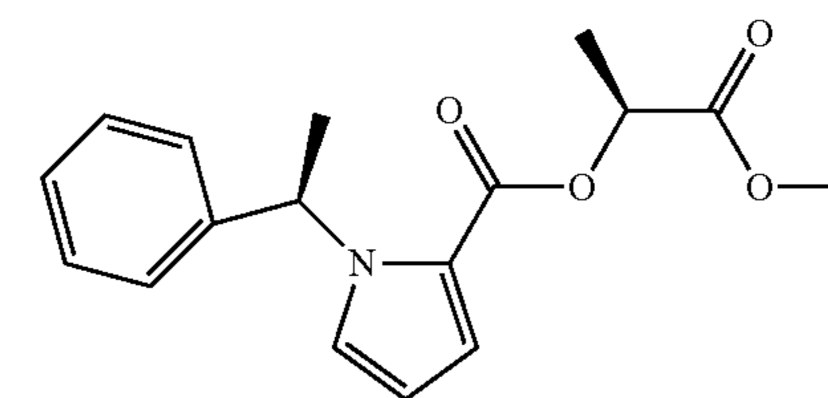
35 (R-methyl-MOC-carbometomidate),
