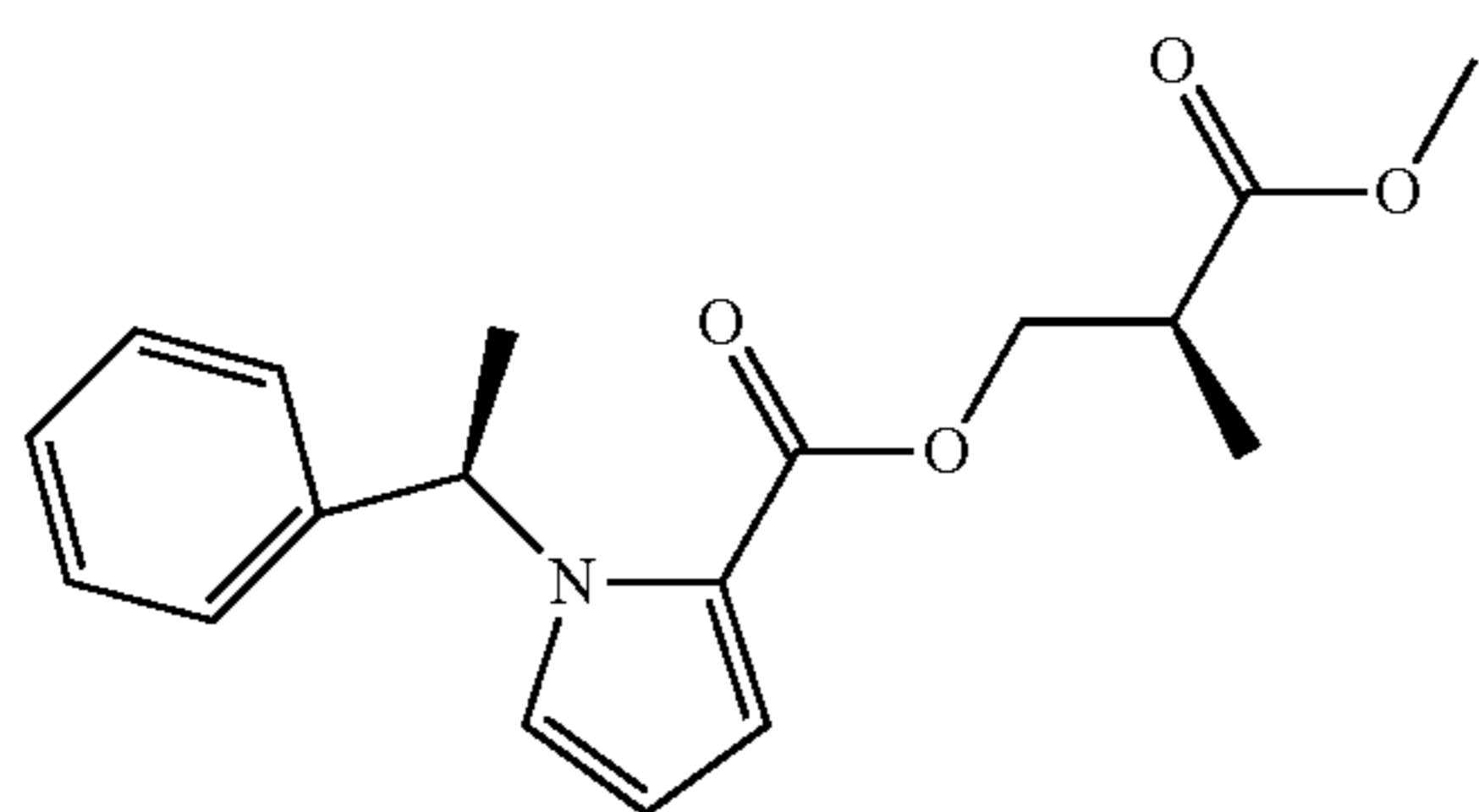
( \alpha -R-methyl-MOC-carboetomidate),
