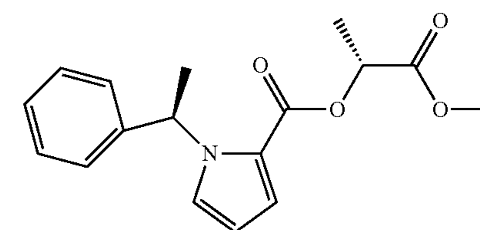
45 (S-methyl-MOC-carbometomidate),
