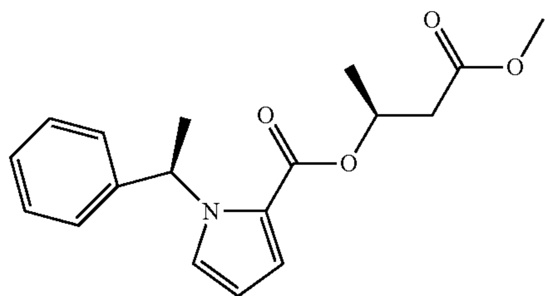
( \beta -R-methyl-MOC-carboetomidate),
