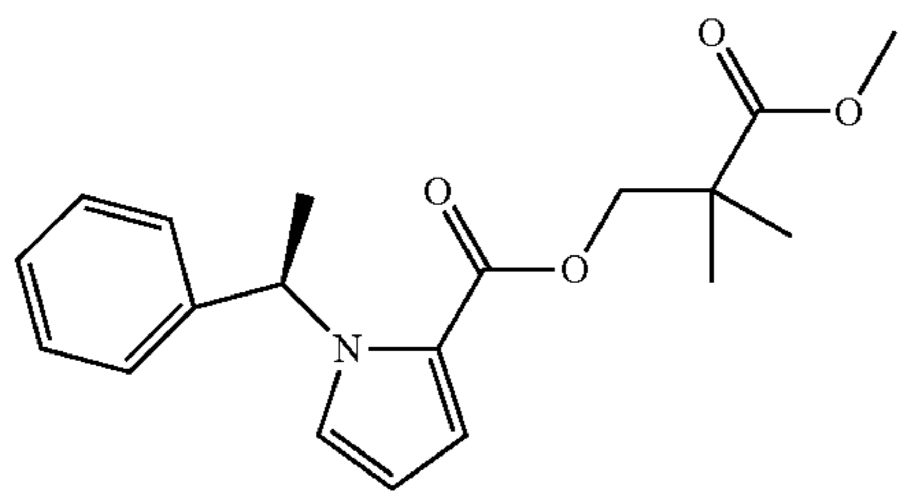
( \alpha -dimethyl-MOC-carboetomidate),
