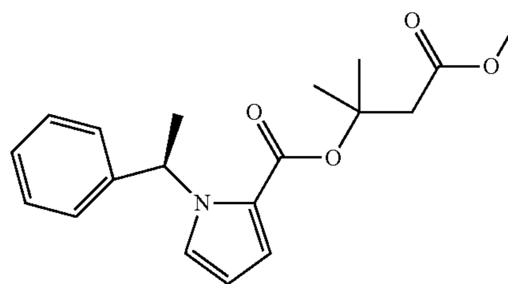
20 (β-dimethyl-MOC-carboetomidate),
