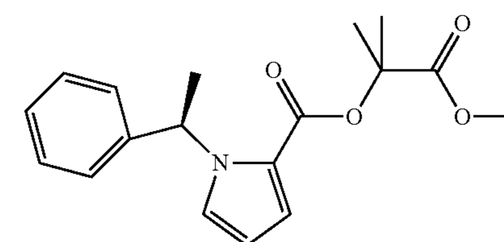
60 (dimethyl-MOC-carbometomidate),
