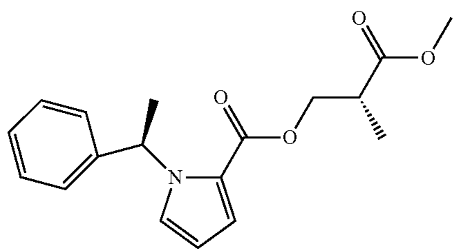
( \alpha -S-methyl-MOC-carboetomidate),
