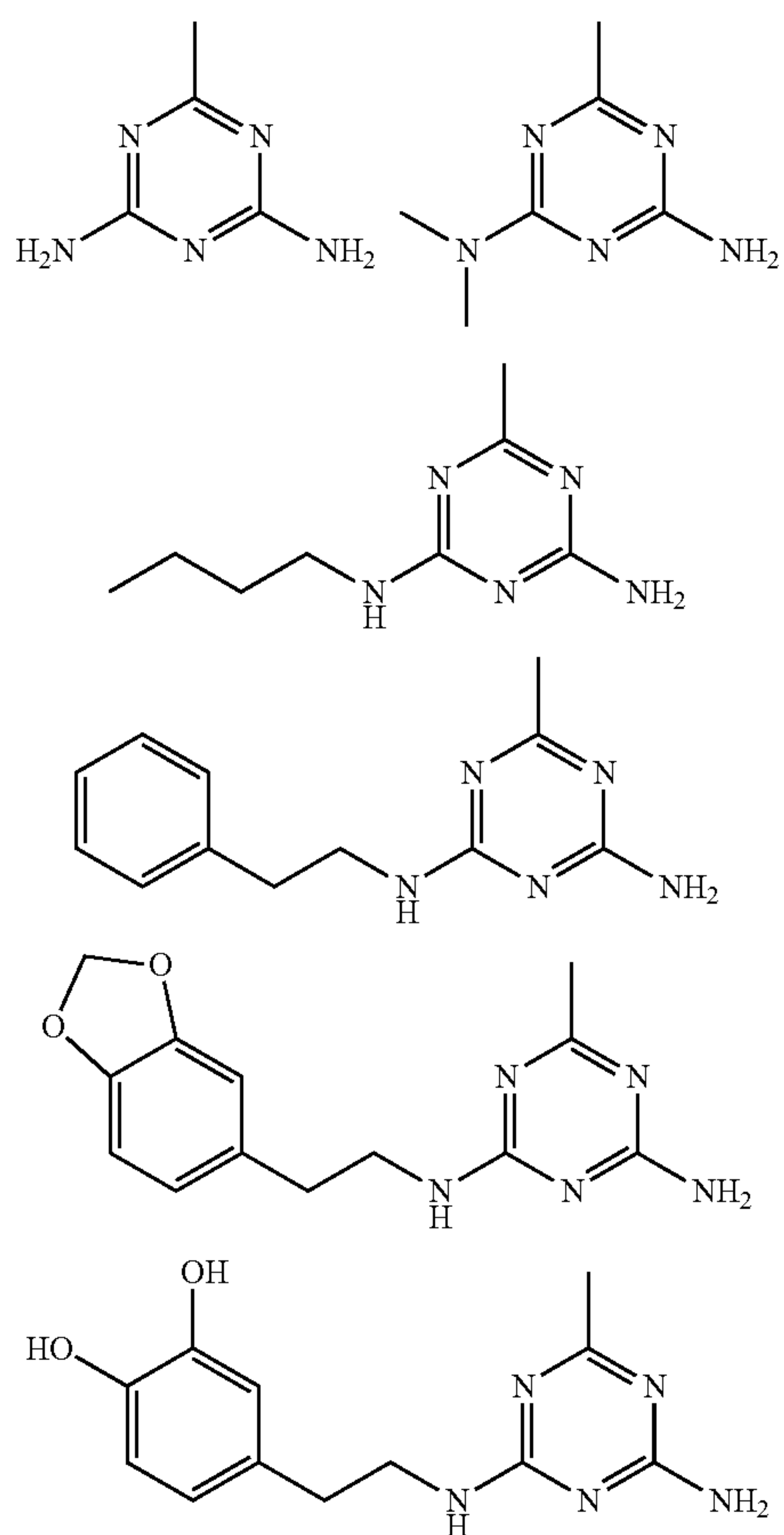
Triazines: Formula (II)
