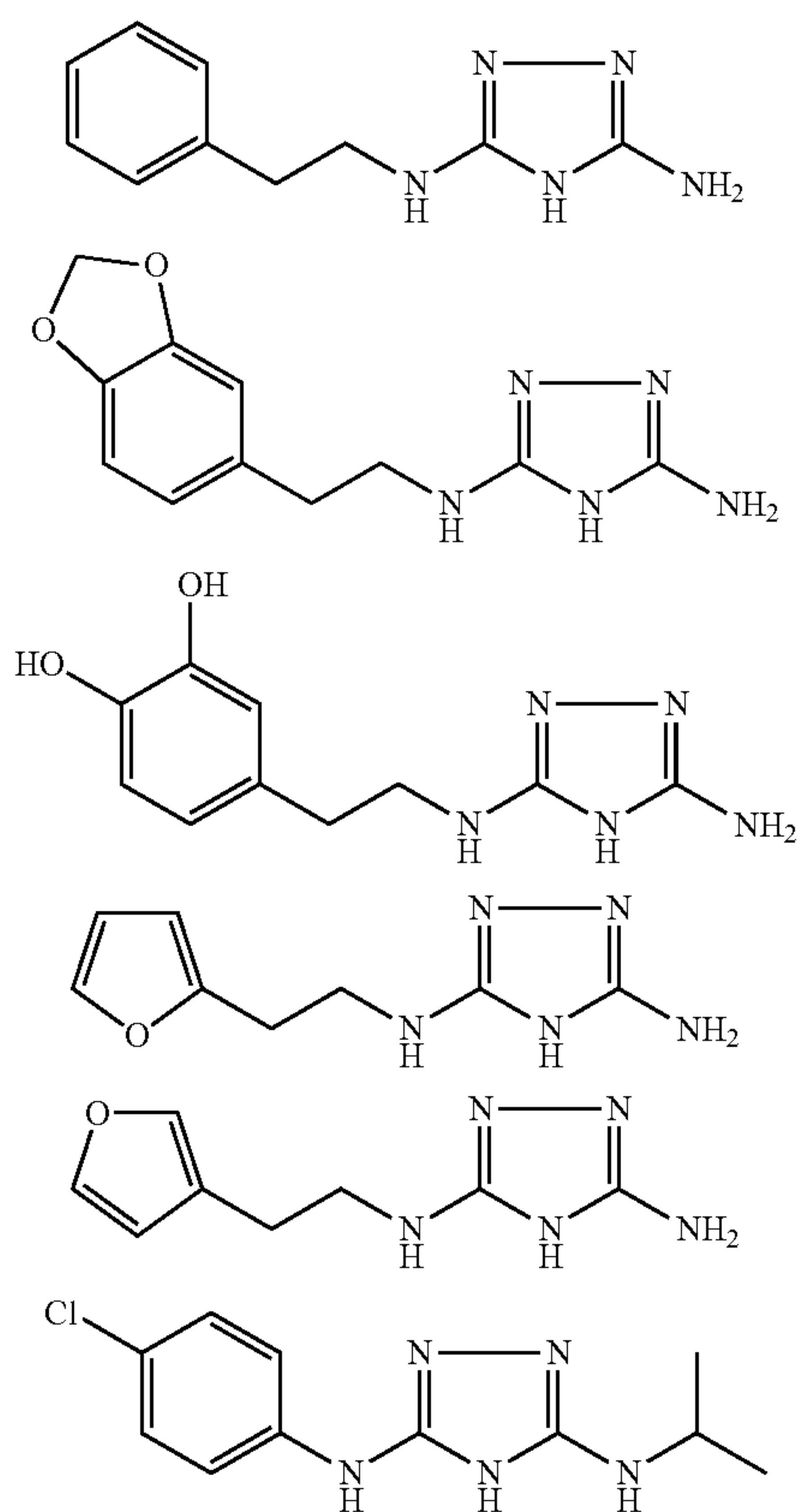
Triazines: Formula (II)
