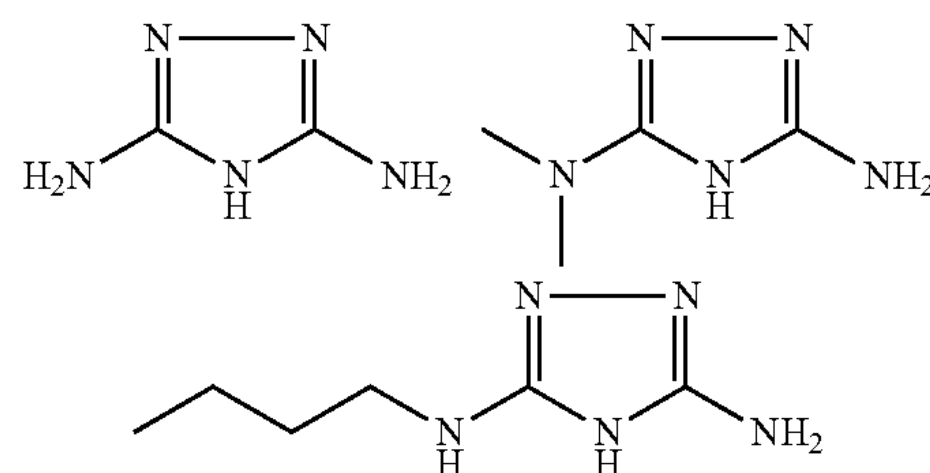
Triazoles: Formula (IA)
