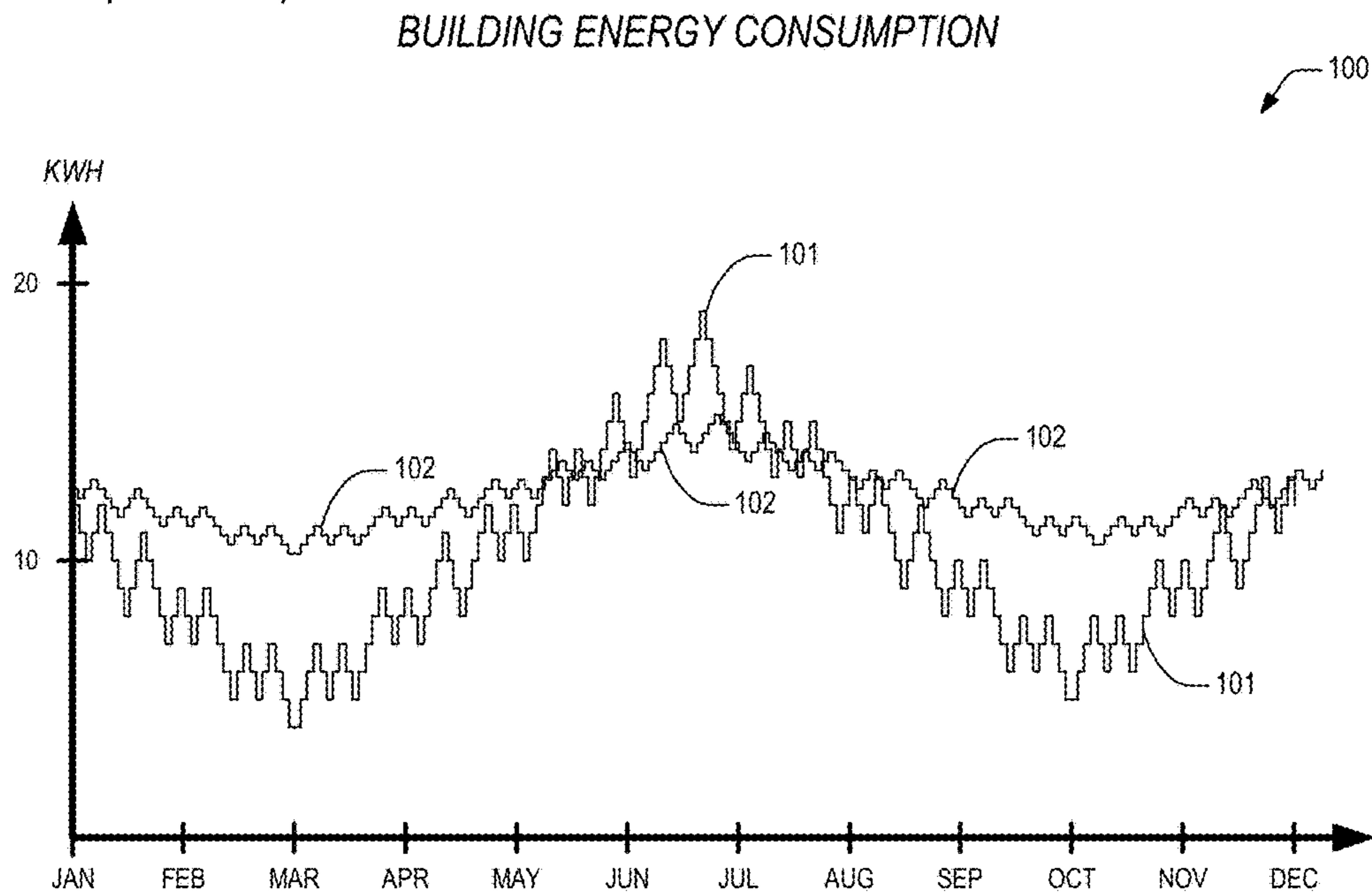
FIG. 1 (Prior Art)
