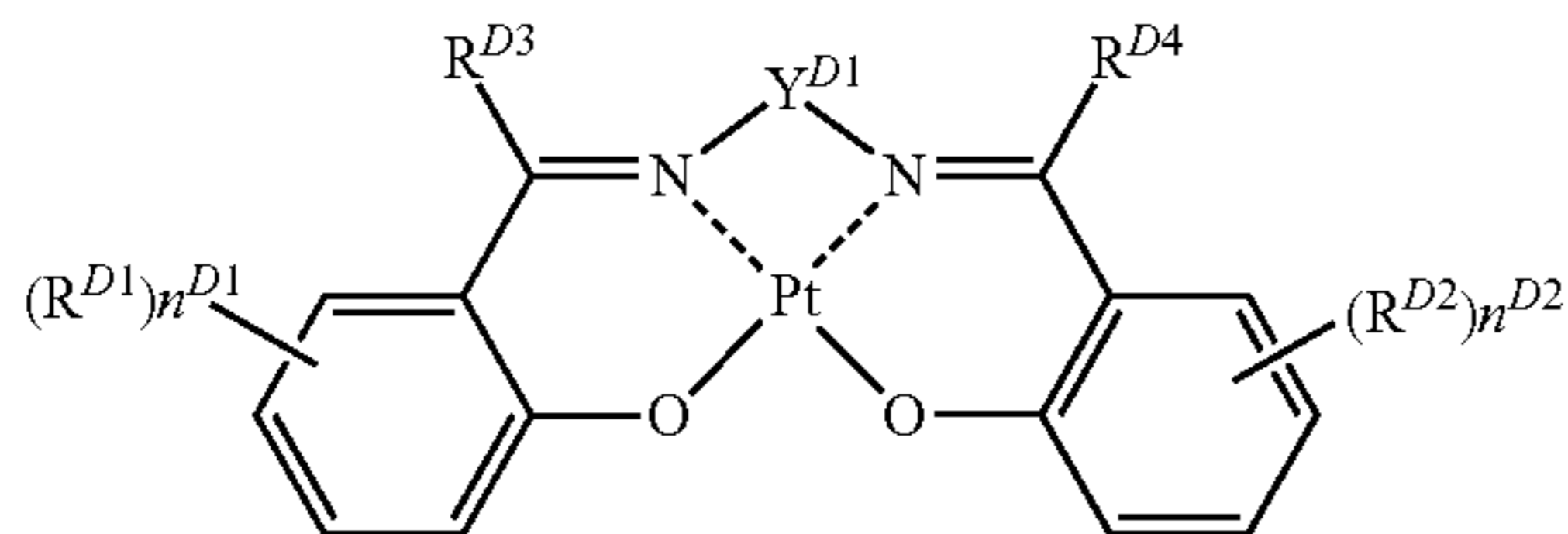
Formula (12)
