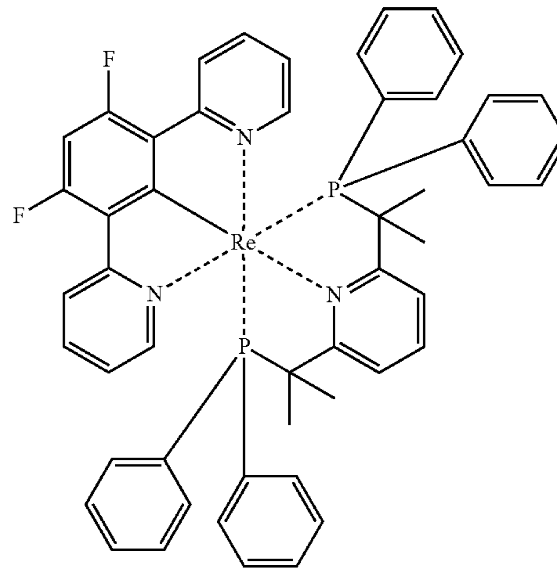
Compound (164)
