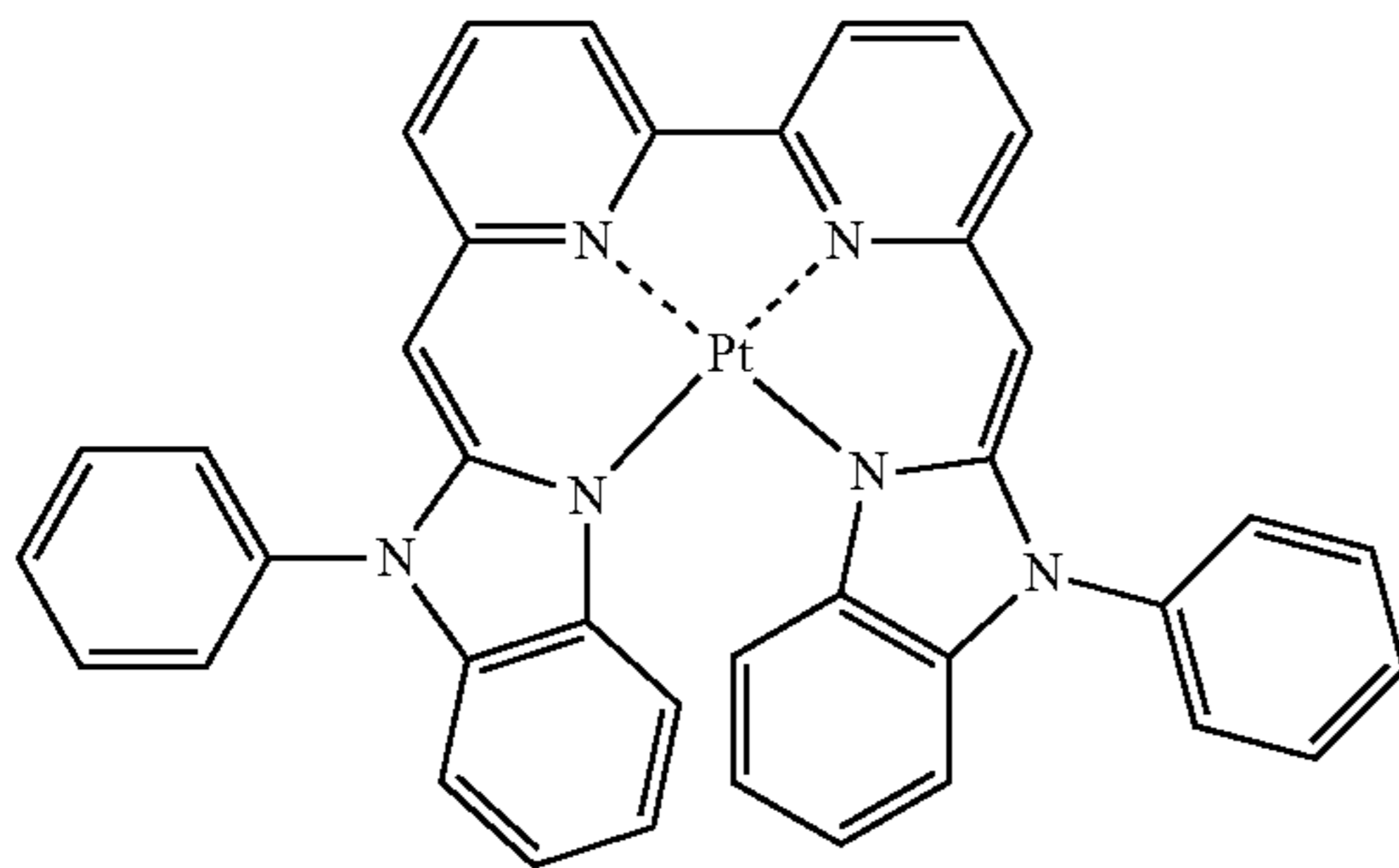
Compound (29)
