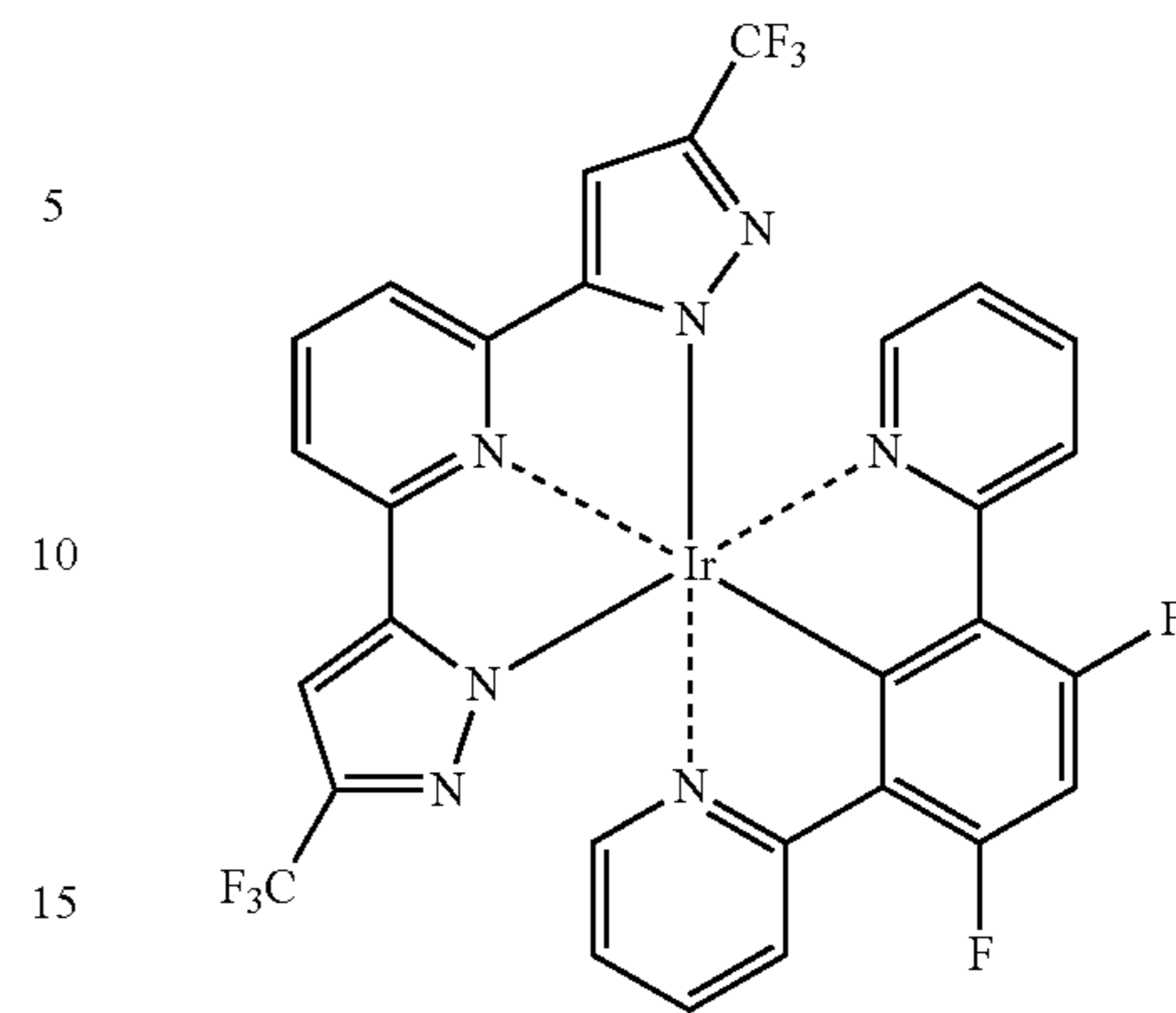
Compound (102)
