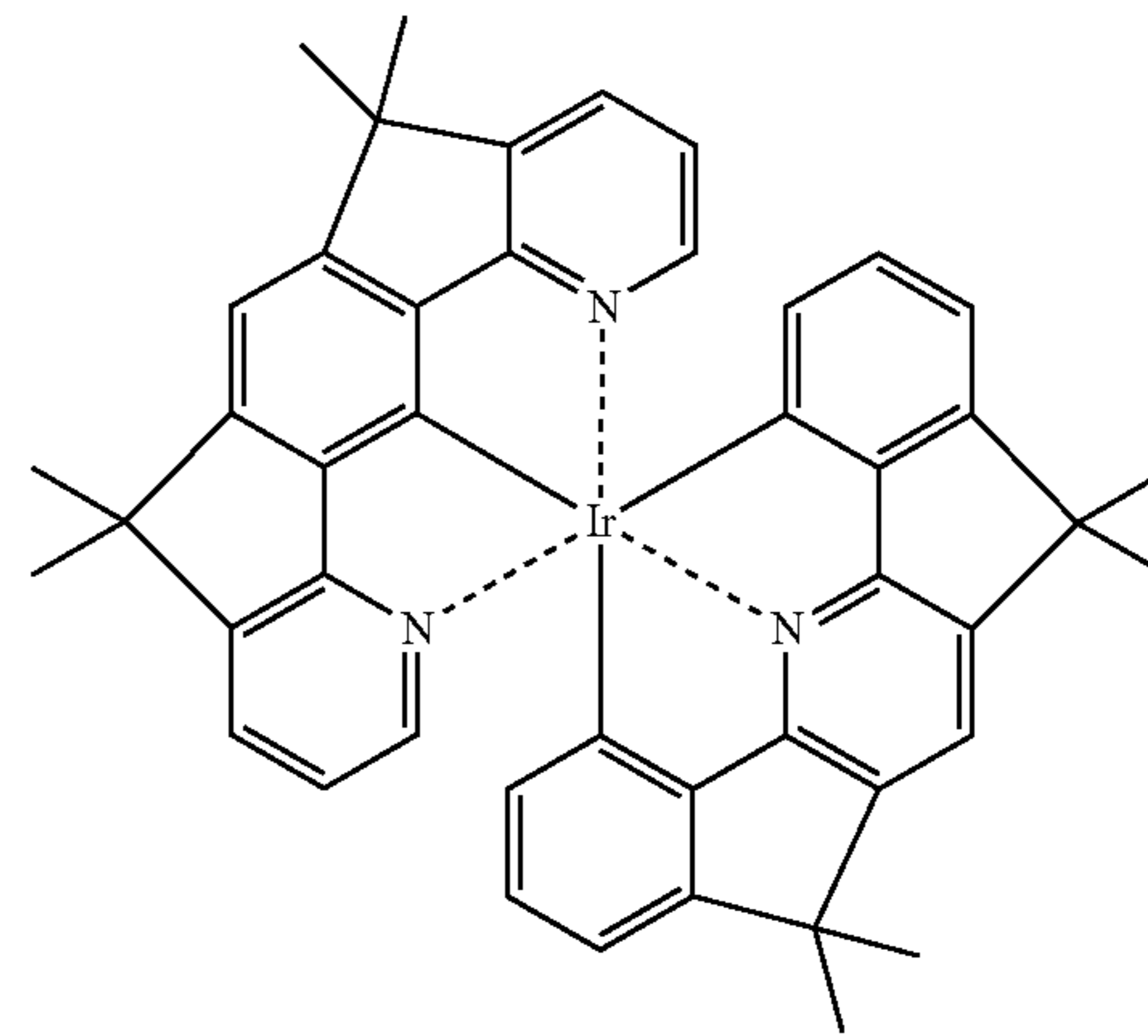
Compound (99)
