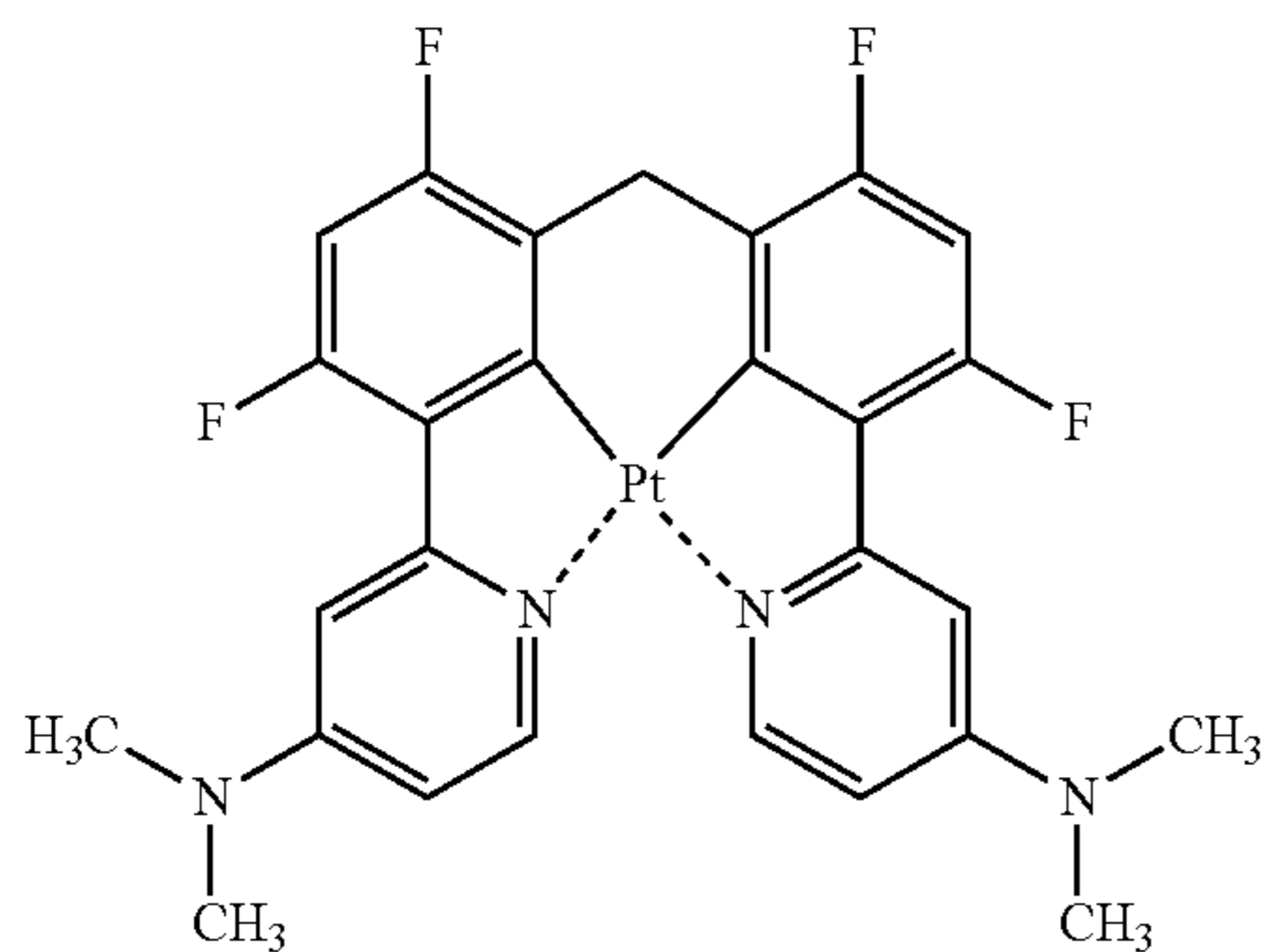
Compound (41)
