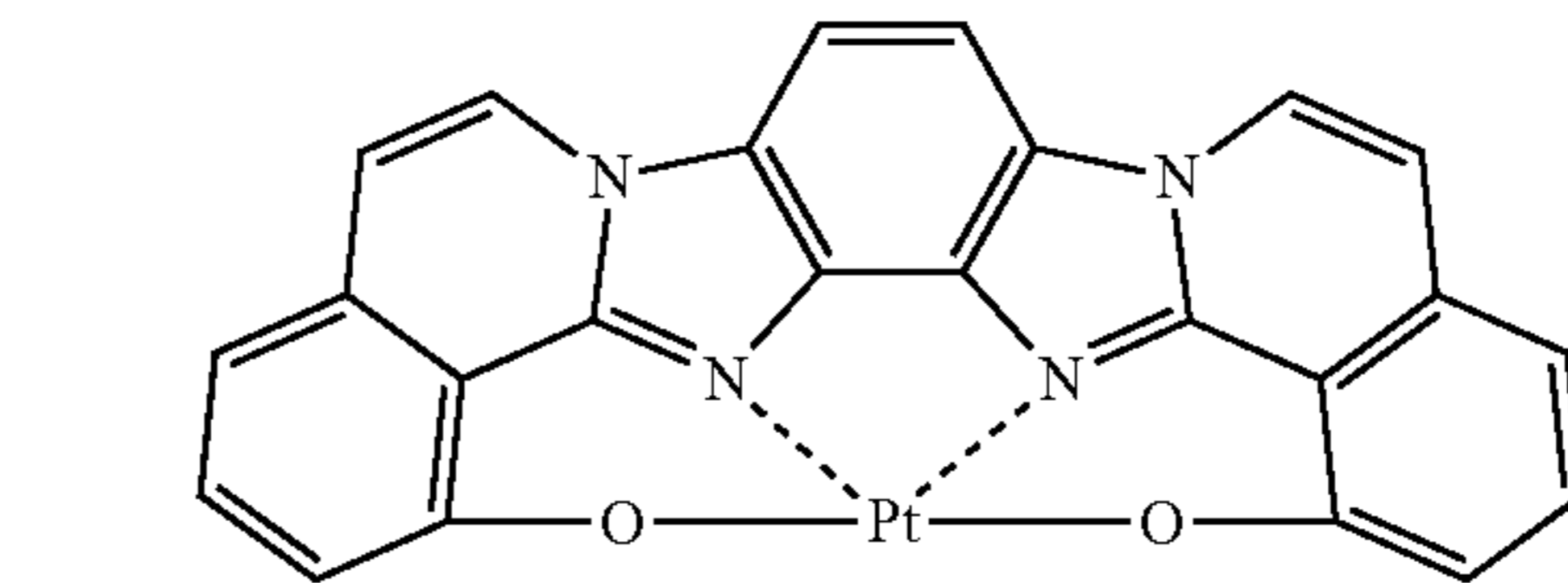
Compound (184)
