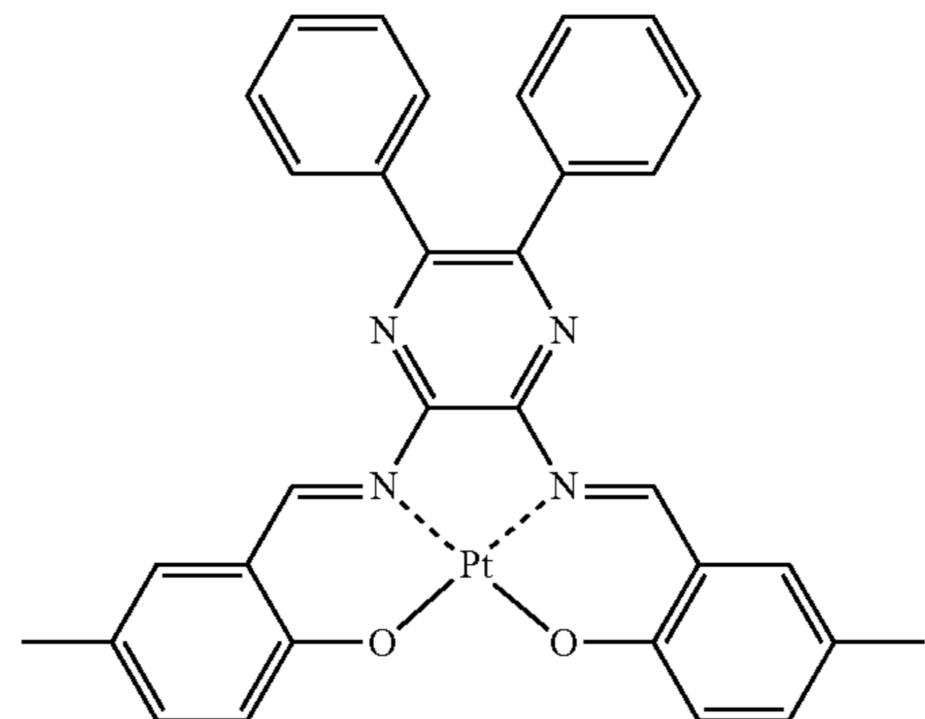
Compound (94)
