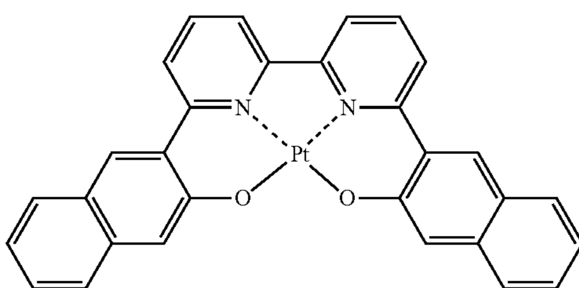
Compound (22)
