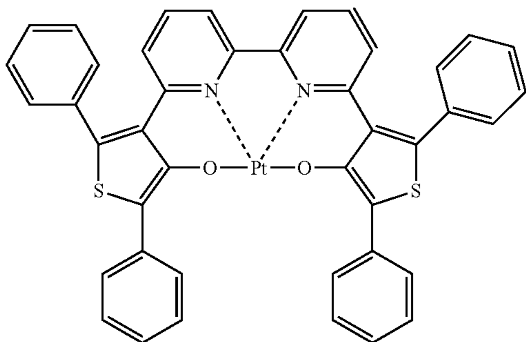
Compound (211)
