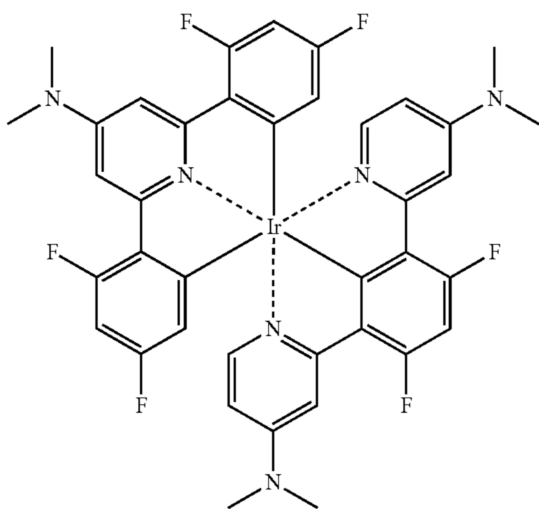
Compound (105)
