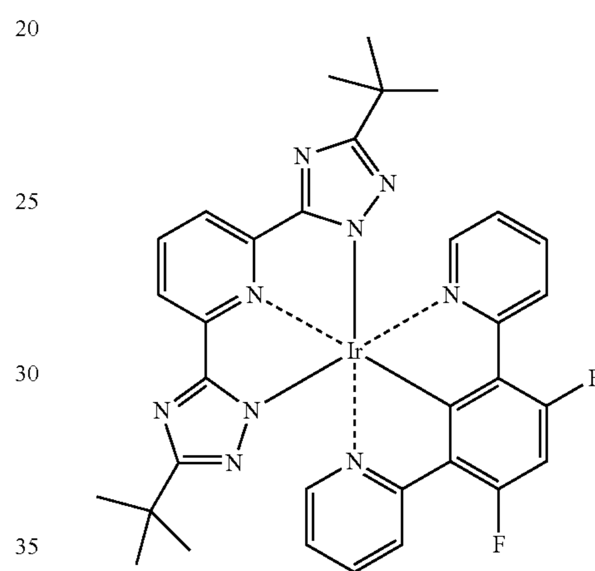
Compound (107)
