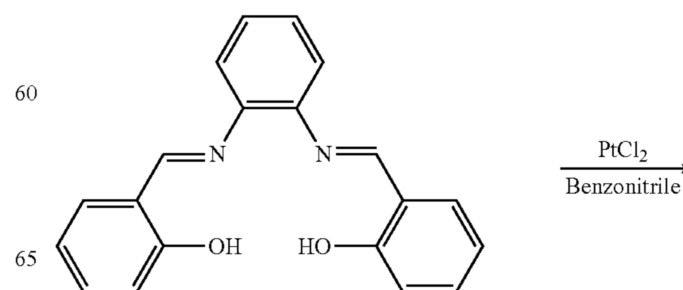
Synthesis scheme-2
