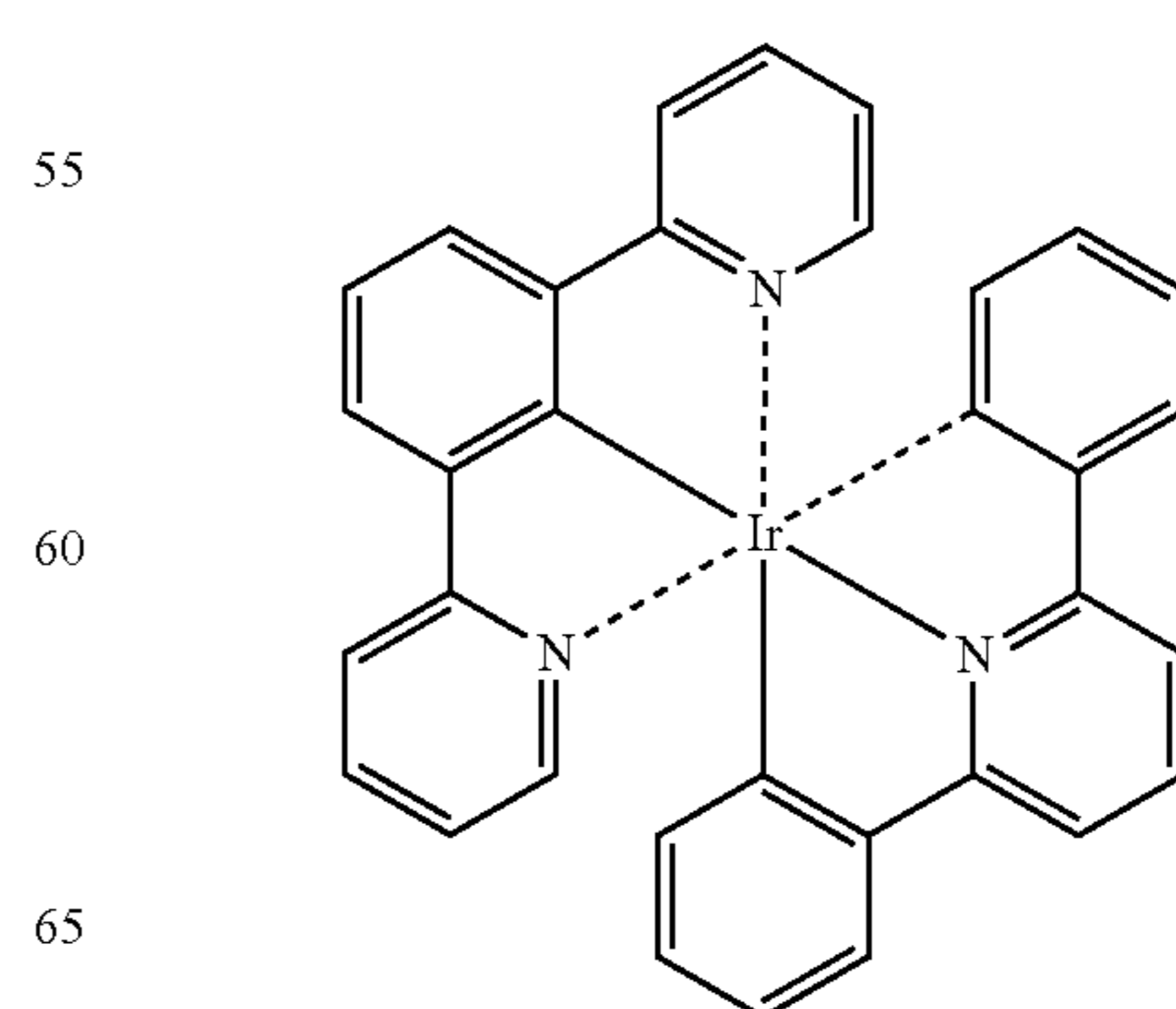
Compound (105)
