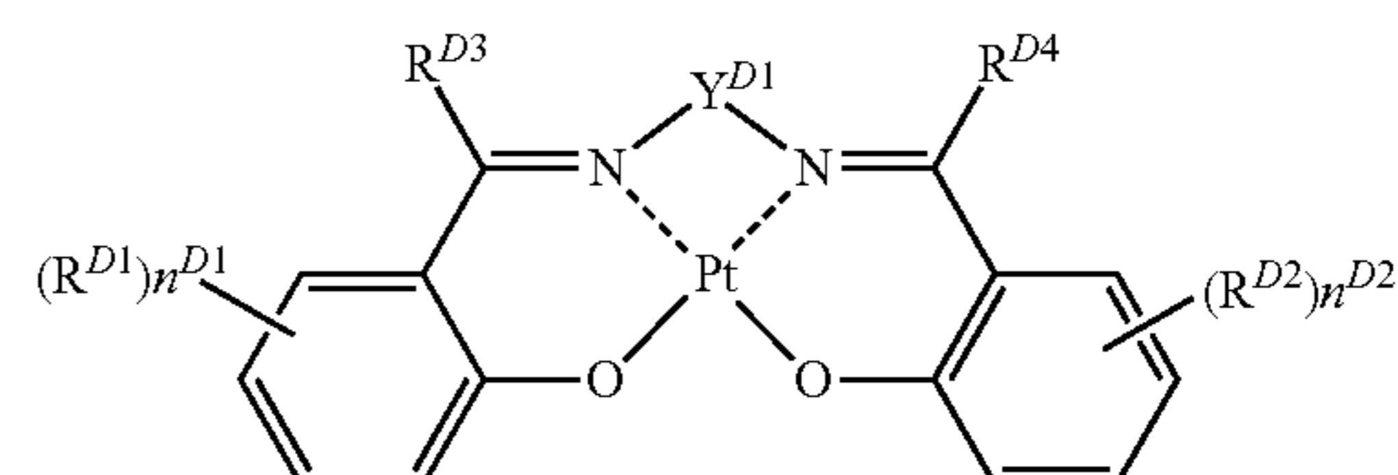
Formula (12)
