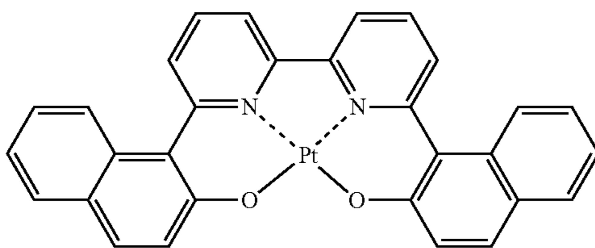
Compound (22)
