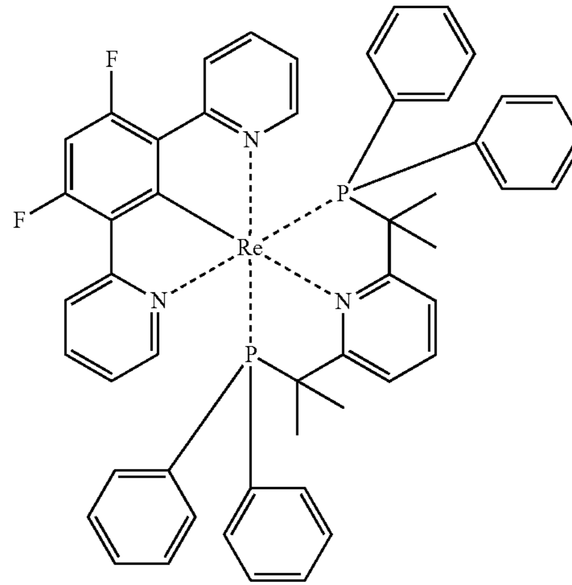
Compound (165)
