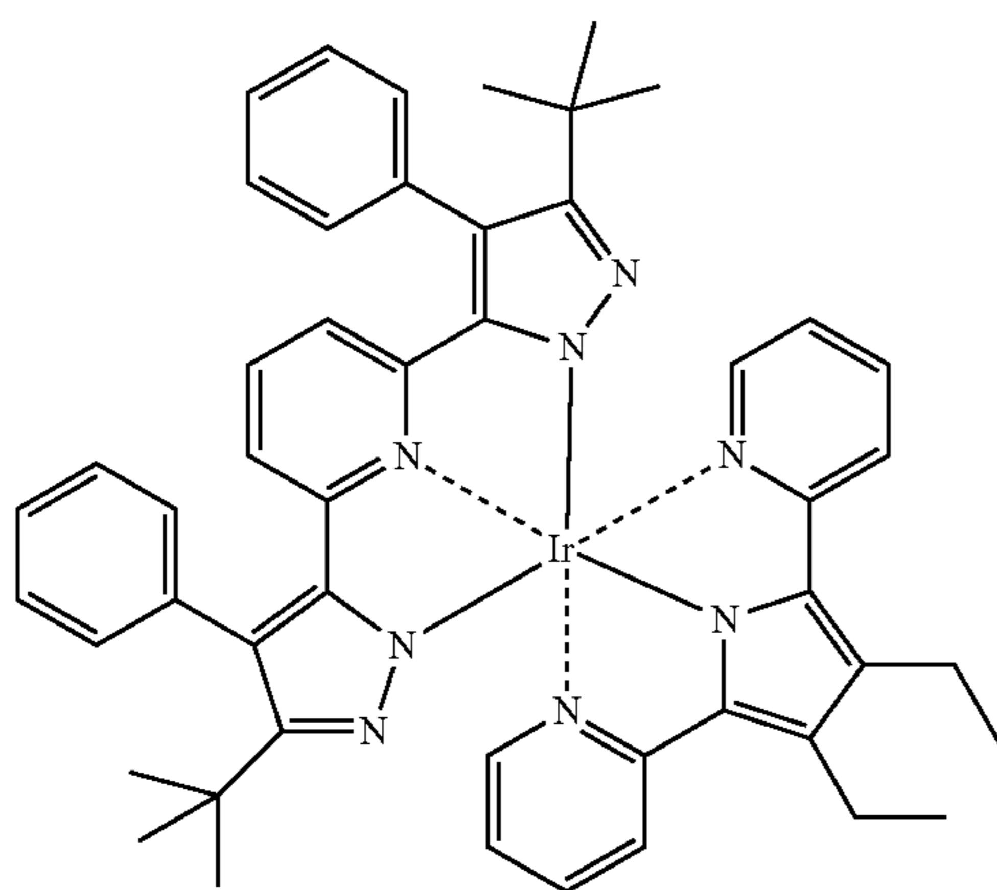
Compound (154)
