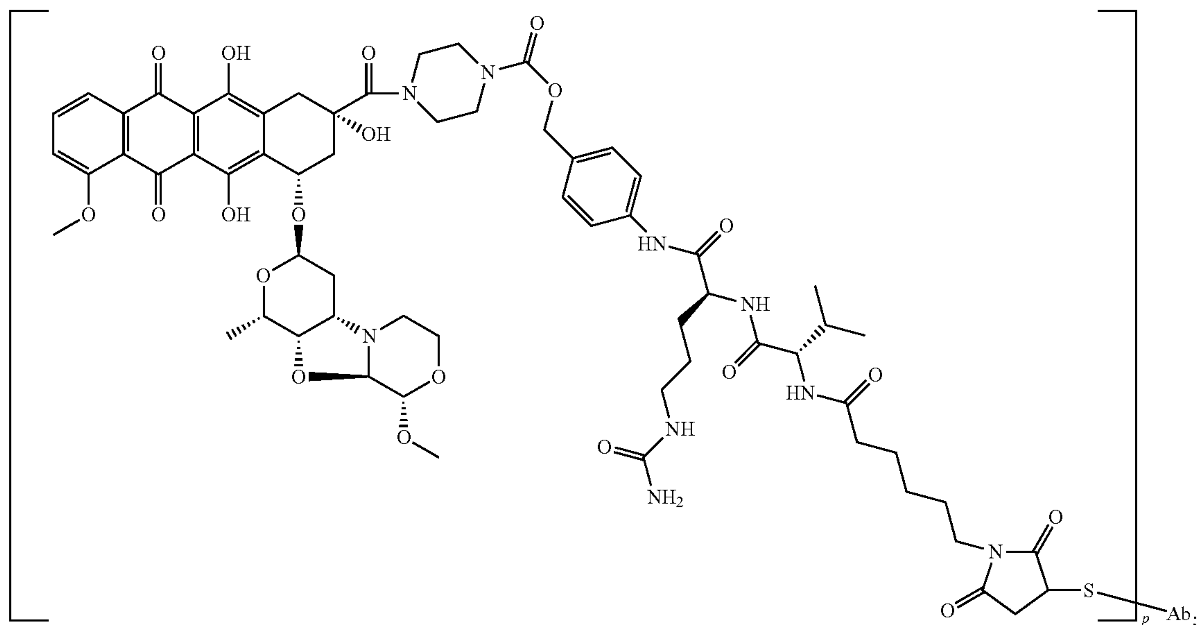
PNU-159682-val-cit-PAB-Ab
