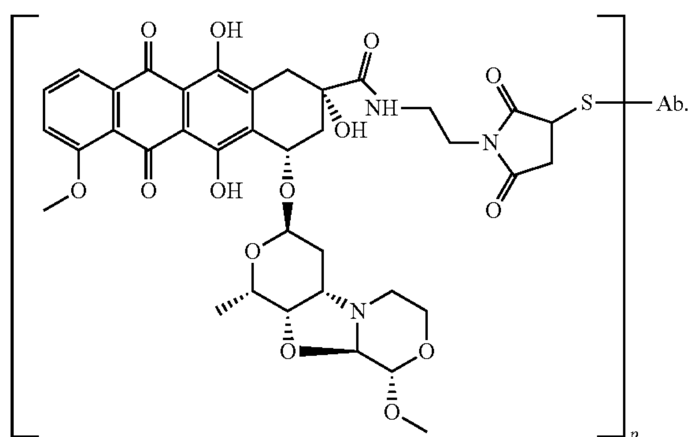
PNU-159682-maleimide-Ab
