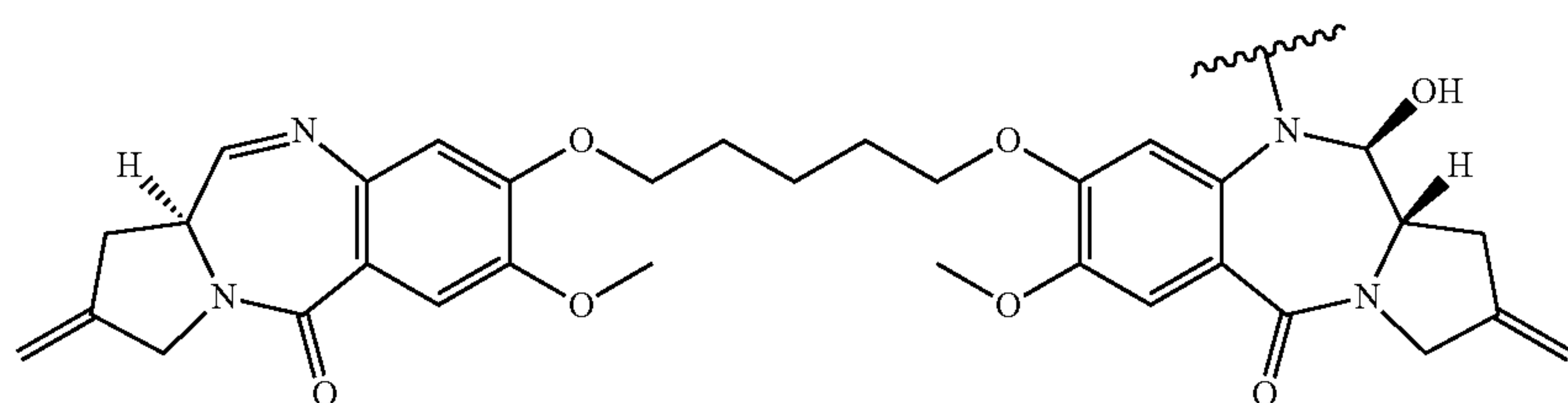
PBD dimer
