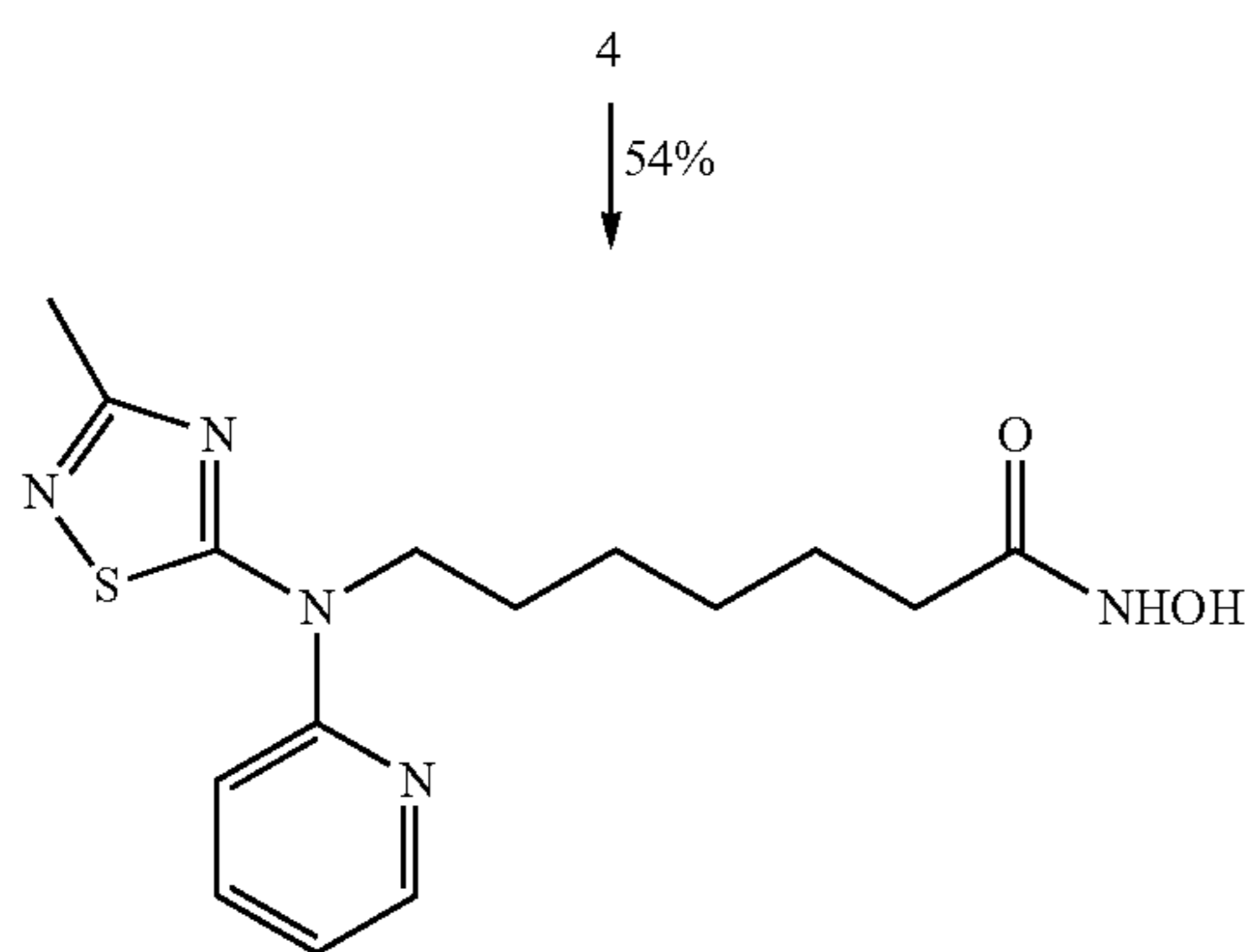
Compound A
