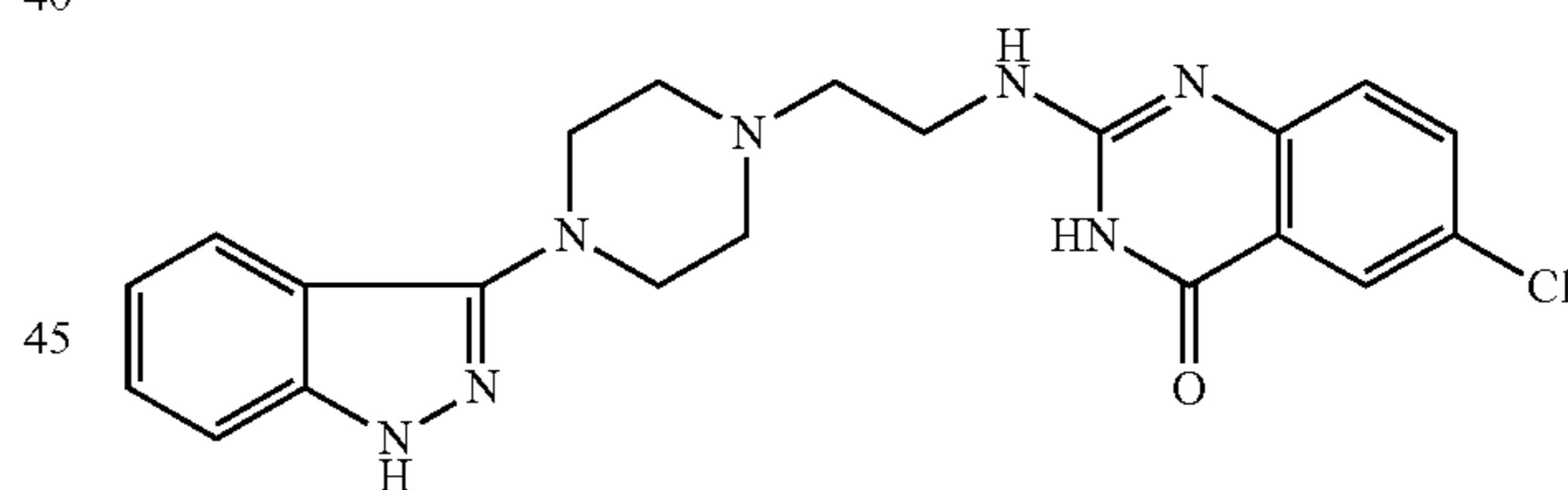
Compound 43
