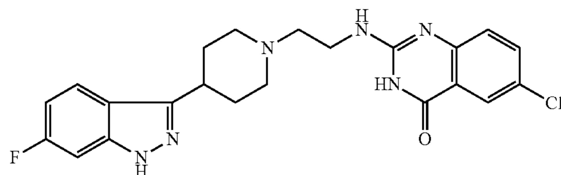
Compound 39
