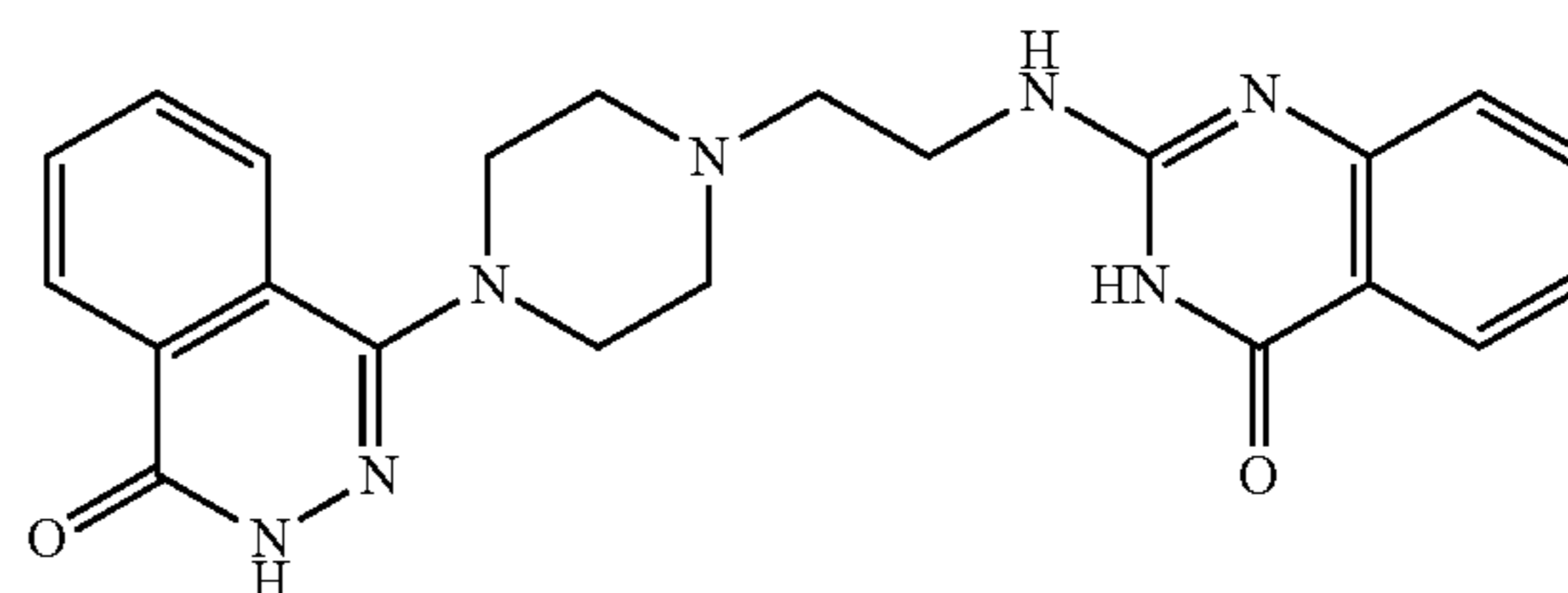
Compound 36
