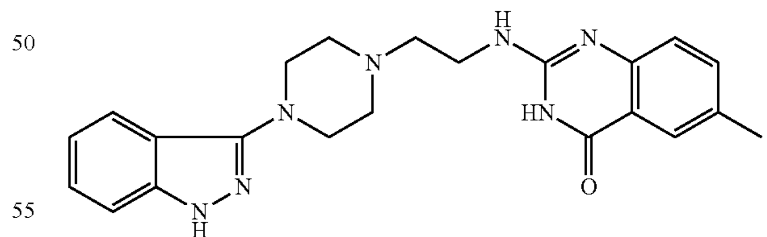
Compound 43
