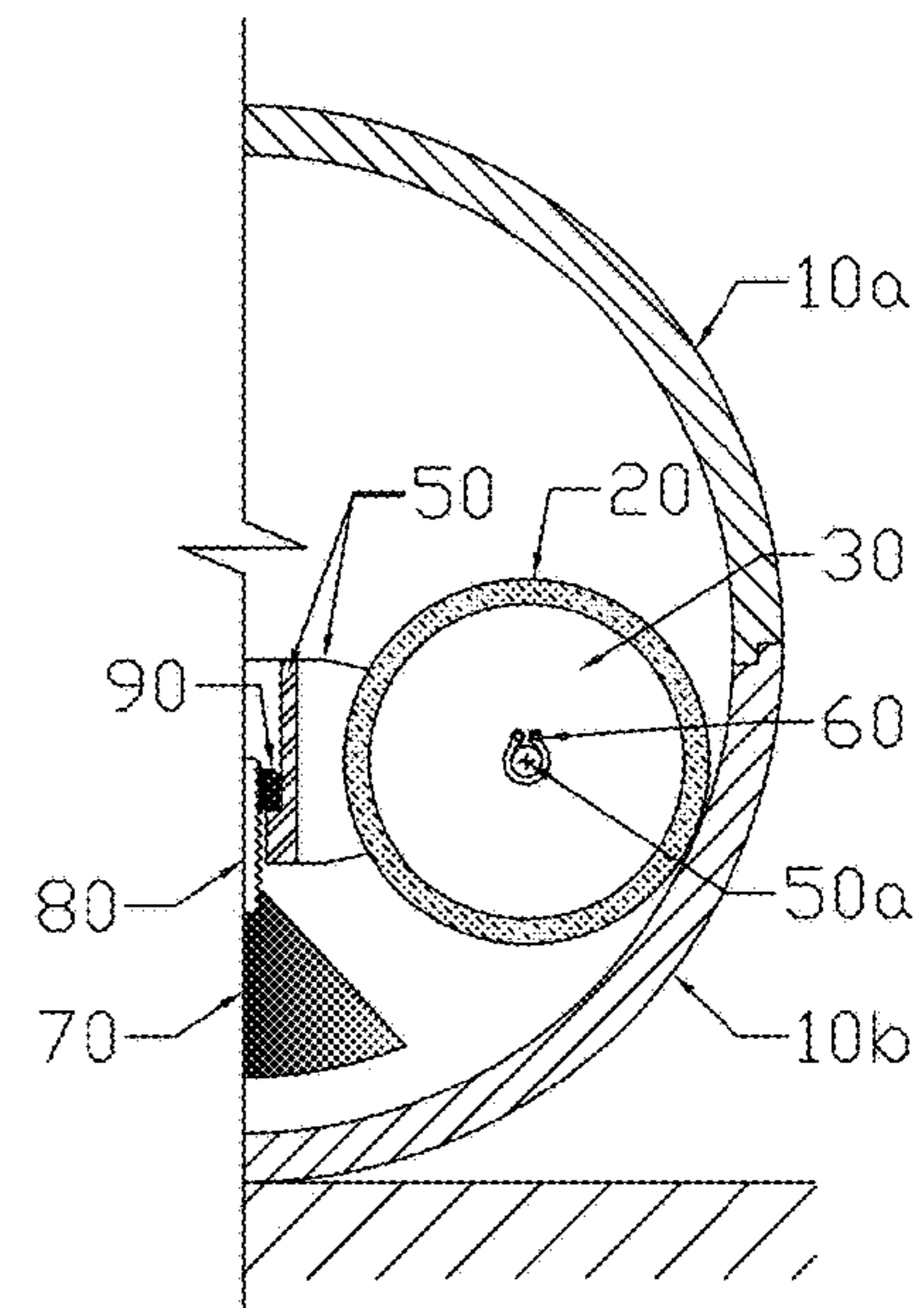
Section B-B
