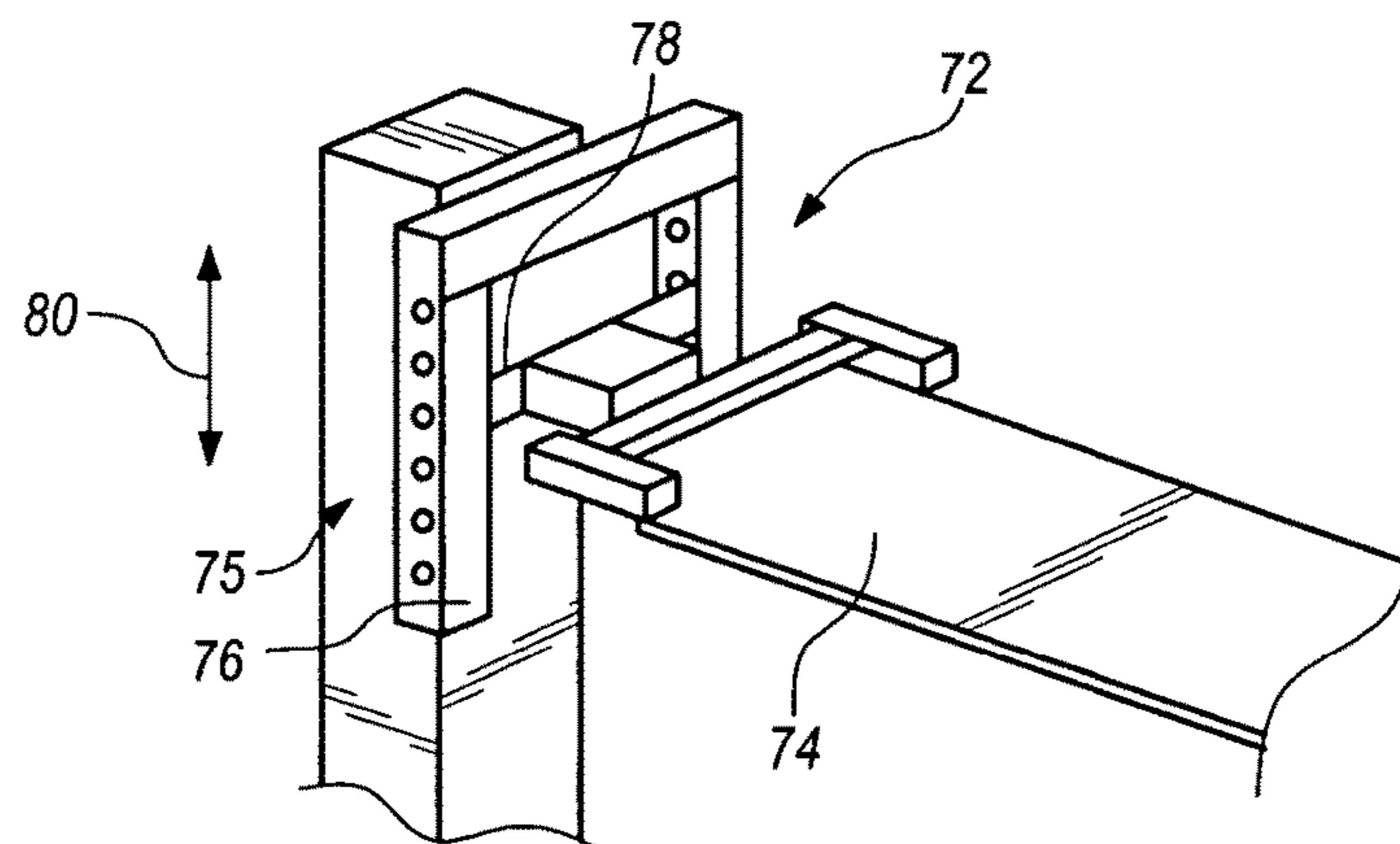
PRIOR ART FIG. 5
