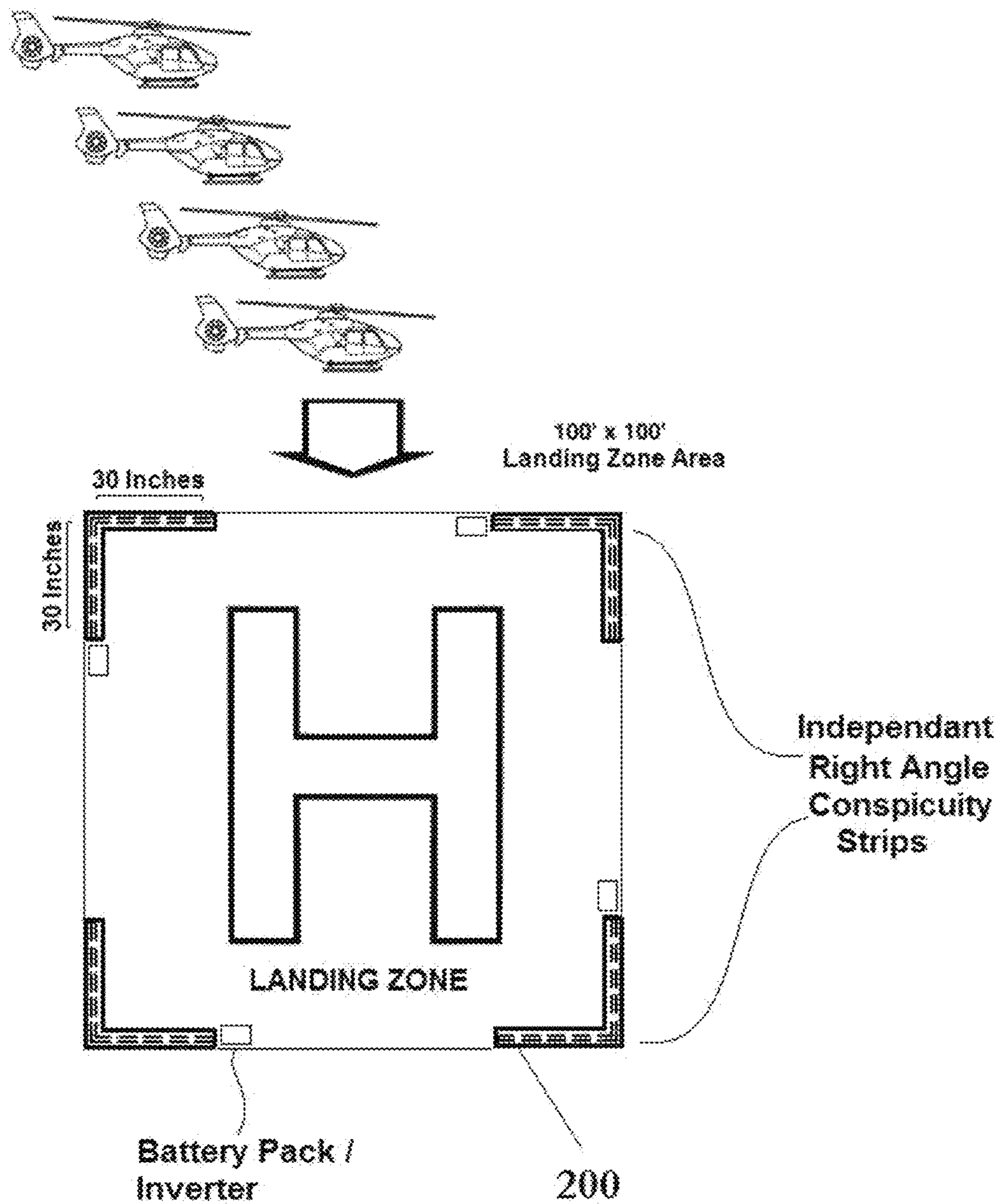
Transportable Helipad Landing Zone Demarcation (Anchored w/ Tent Spikes)
