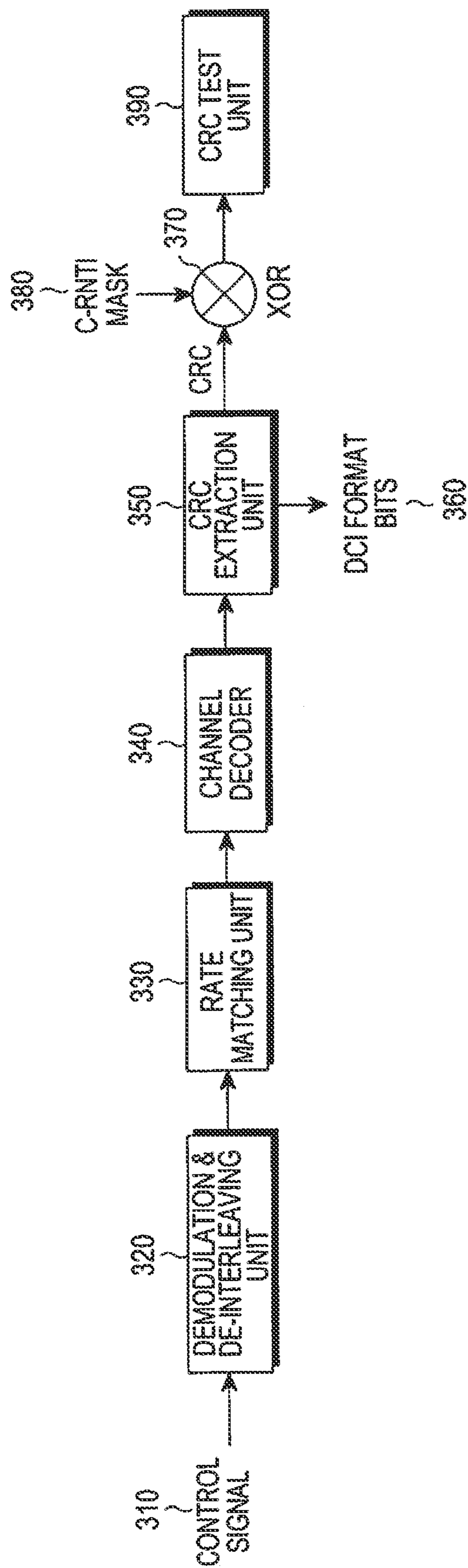
FIG.3 (PRIOR ART)
